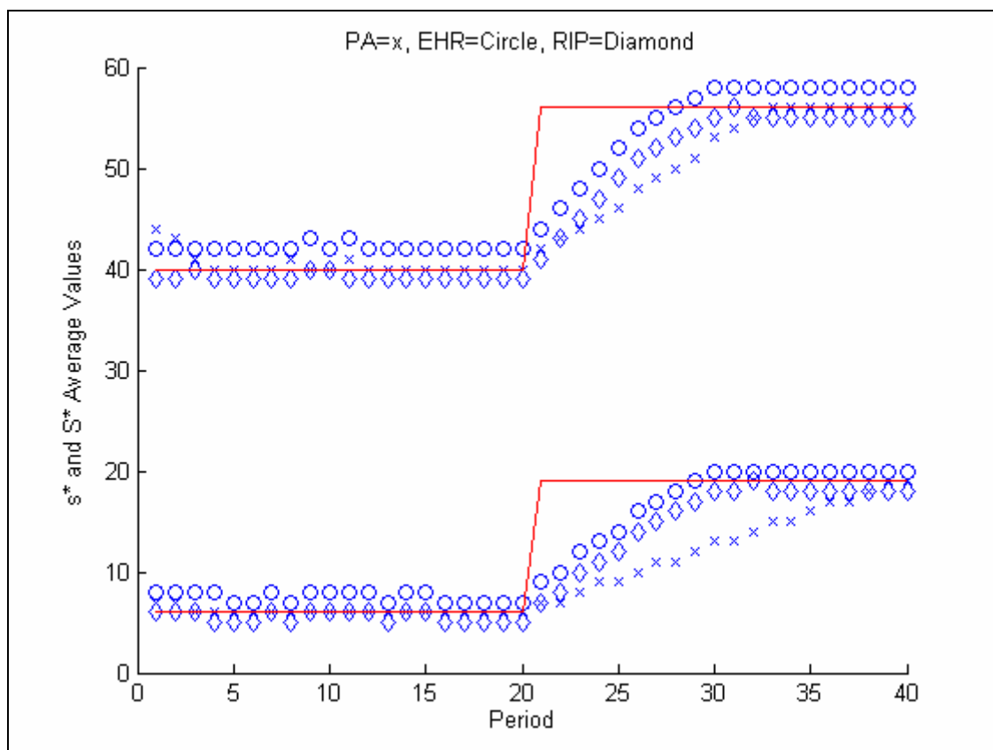
Fig. J.34. Comparison of (s^*, S^*) Graphs, \delta=15 , \gamma=\text{ALL HISTORY}
