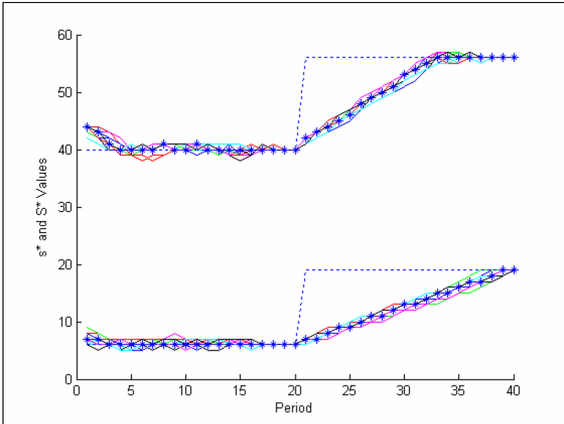
Fig. J.31. (s^*, S^*) Graph for PA Alg. , \delta=15 , \gamma=\text{ALL HISTORY}
