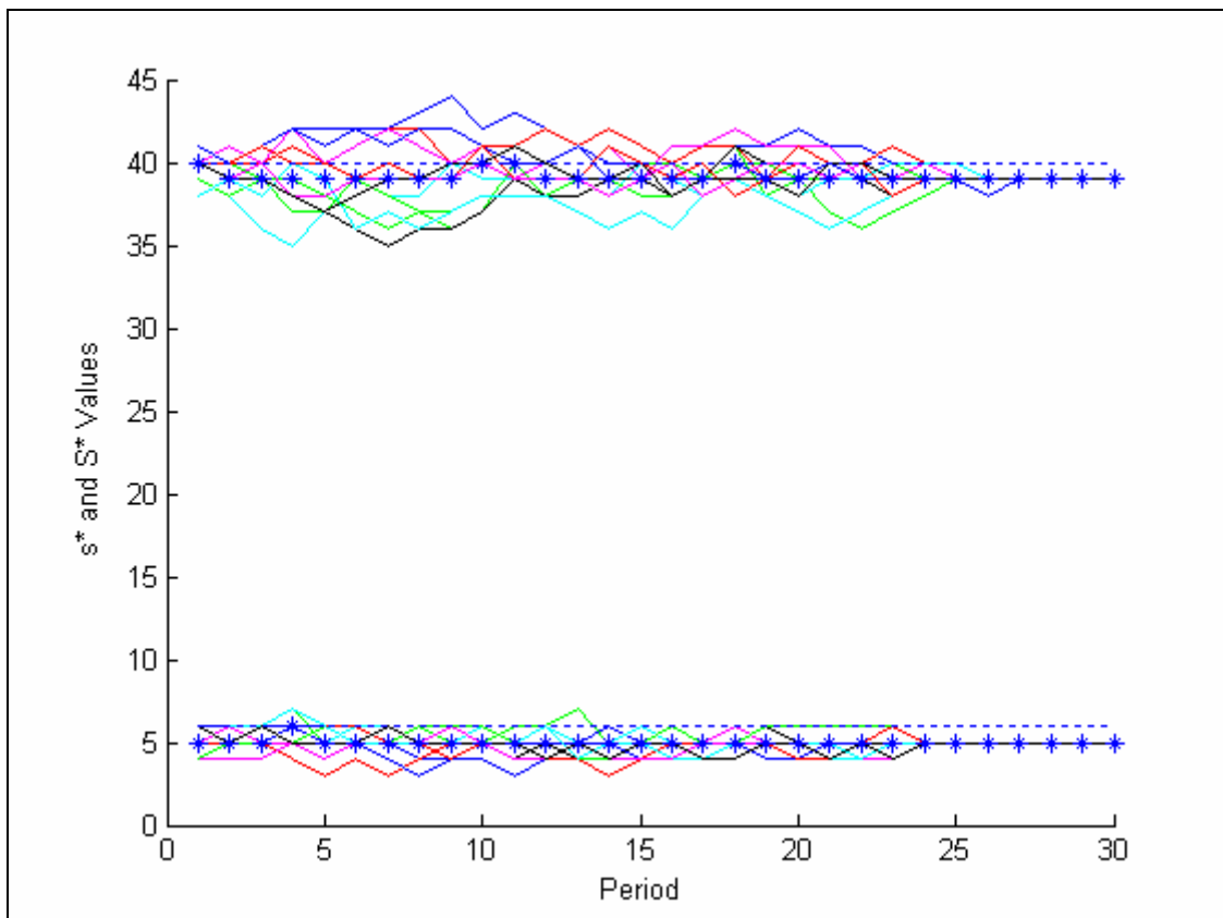
Fig. J.6. (s^*, S^*) Graph for RIP Alg. \text{POI}(10) , \gamma = 3
