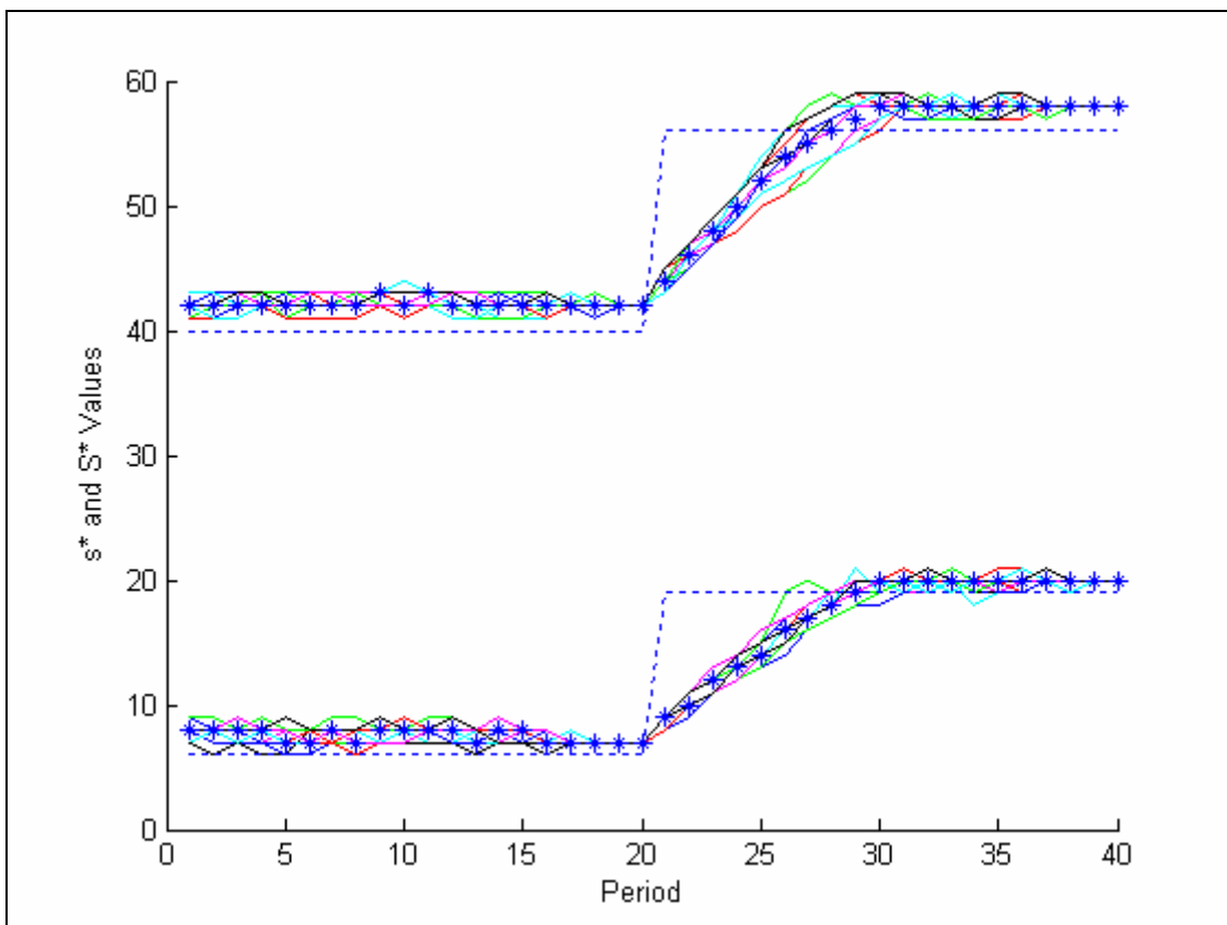
Fig. J.32. (s^*, S^*) Graph for EHR Alg. , \delta=15 , \gamma=\text{ALL HISTORY}
