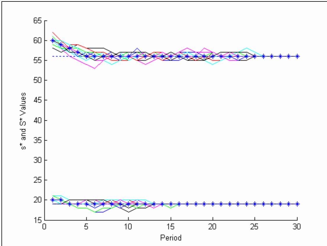
Fig. J.11. (s^*, S^*) Graph for PA Alg. POI(25), \gamma = \text{ALL HISTORY}
