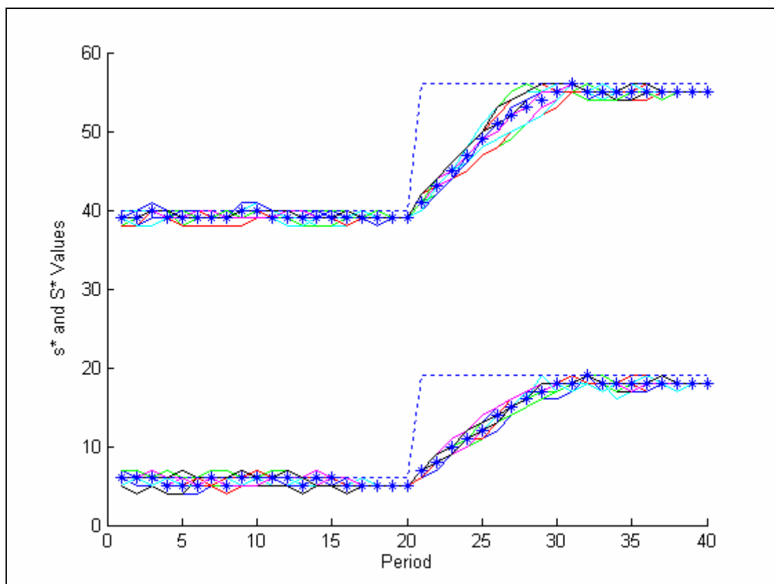
Fig. J.33. (s^*, S^*) Graph for RIP Alg. , \delta=15 , \gamma=\text{ALL HISTORY}
