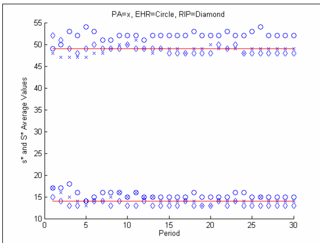
Fig. J.25. Comparison of ( s^* , S^* ) Graphs for Empirical Distribution
