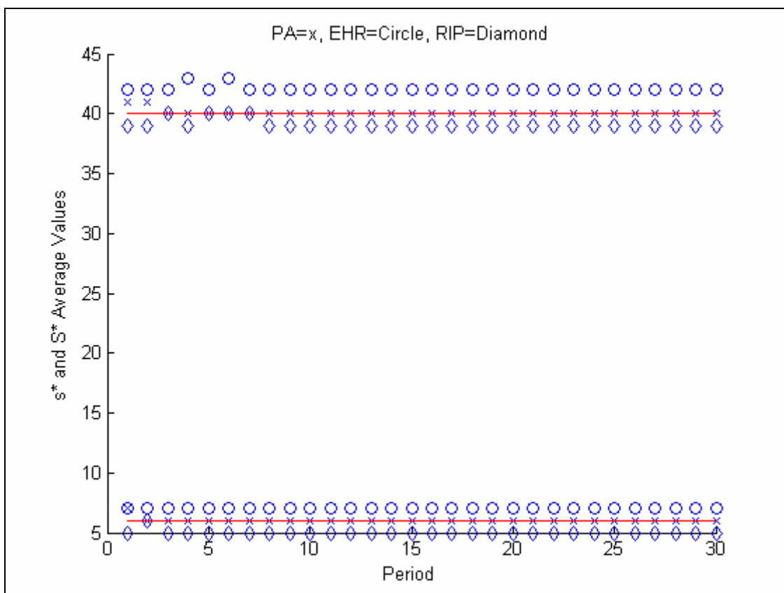
Fig. J.7. Comparison of (s^*, S^*) Graphs for POI(10), \gamma=\text{ALL HISTORY}
