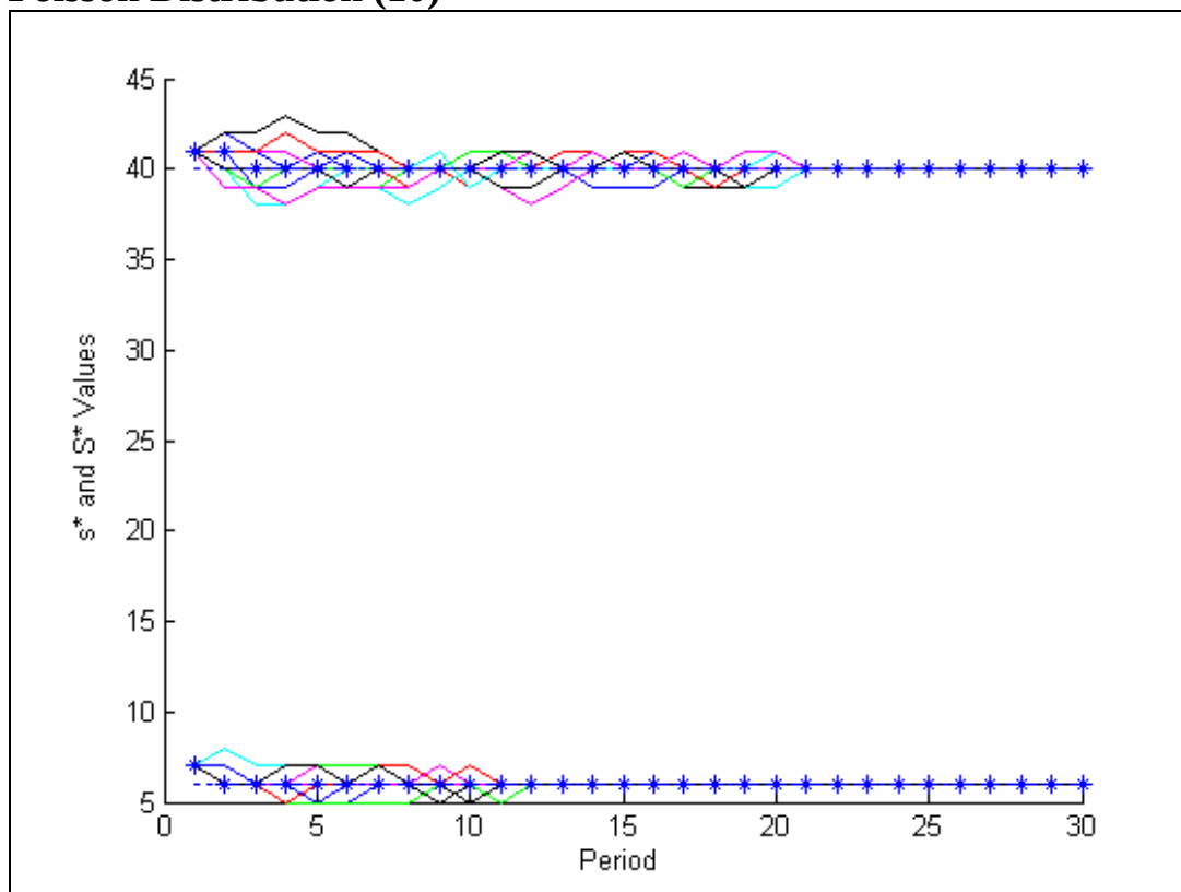
Fig. J.1. ( s^* , S^* ) Graph for PA Alg. POI(10), \gamma = \text{ALL HISTORY}
