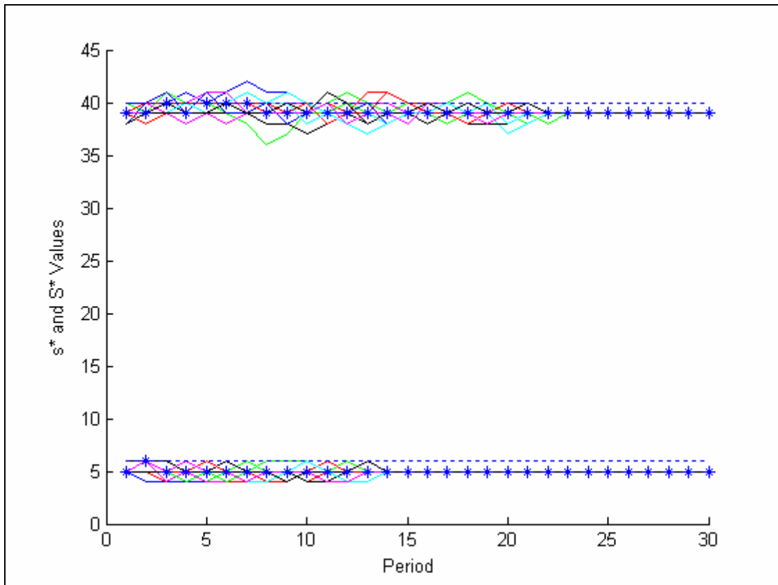
Fig. J.5. (s^*, S^*) Graph for RIP Alg. \text{POI}(10) , \gamma = \text{ALL HISTORY}
