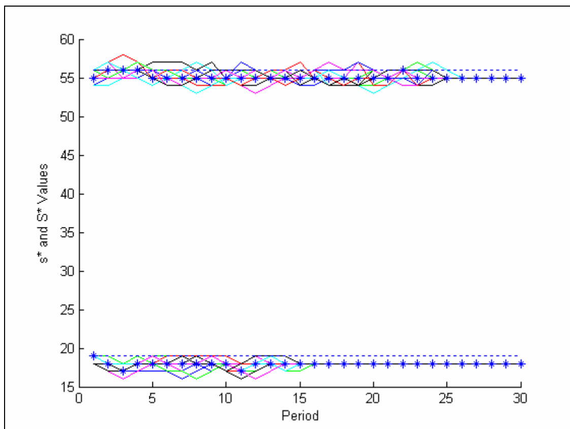
Fig. J.15. (s^*, S^*) Graph for RIP Alg. POI(25), \gamma = \text{ALL HISTORY}
