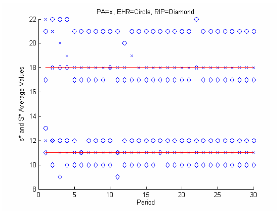
Fig. J.23. Comparison of (s^*, S^*) Graphs for NOR(5,1)
