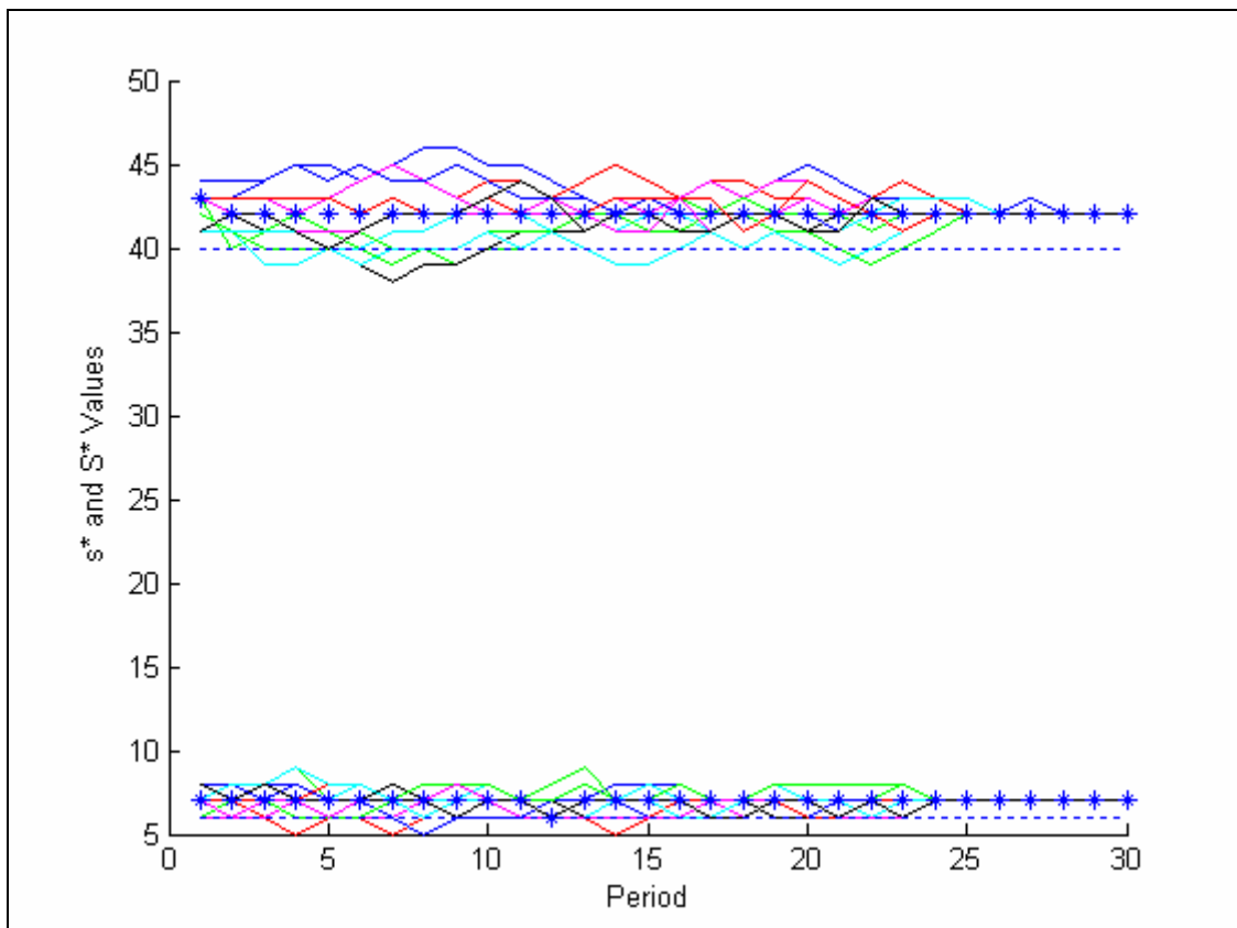
Fig. J.4. (s^*, S^*) Graph for EHR Alg. \text{POI}(10) , \gamma = 3
