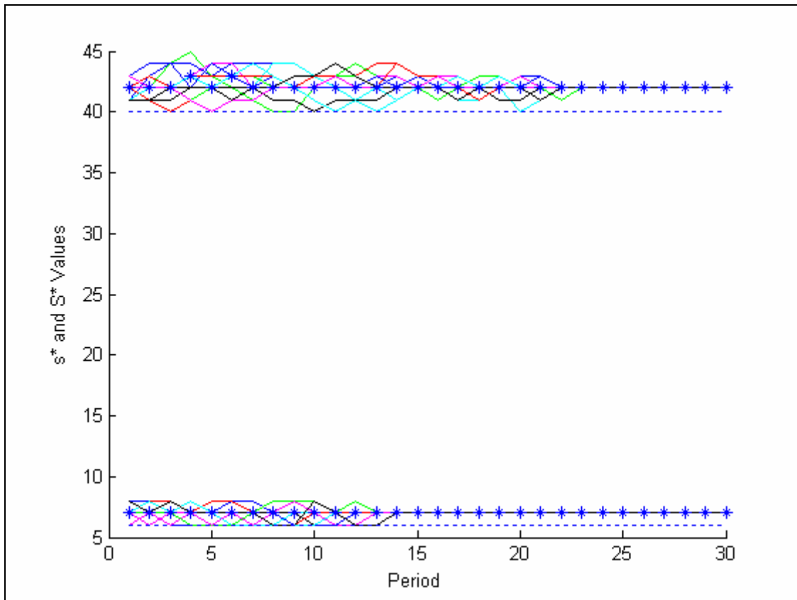
Fig. J.3. (s^*, S^*) Graph for EHR Alg. \text{POI}(10) , \gamma = \text{ALL HISTORY}
