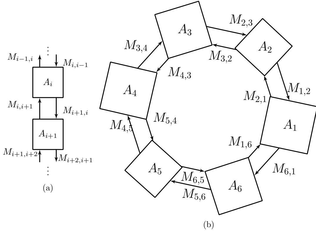
Figure 6.2: Example 5: (6.2a) Interconnection of the subsystems at discrete positions. (6.2b) The circular interconnection of subsystems.
