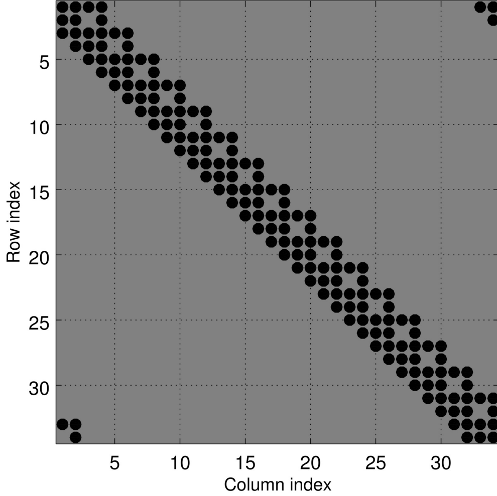
Figure 6.3: Example 5: The nonzero structure of the system matrix A_{cont} for the ring shaped structure where N = 17 .
