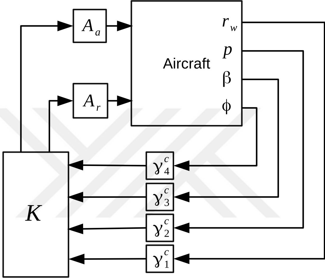
Figure 5.2: In the aircraft model, A_a and A_r are aileron and rudder actuators. \gamma_i^c \in \{0, 1\} determines that corresponding output is used for feedback.
