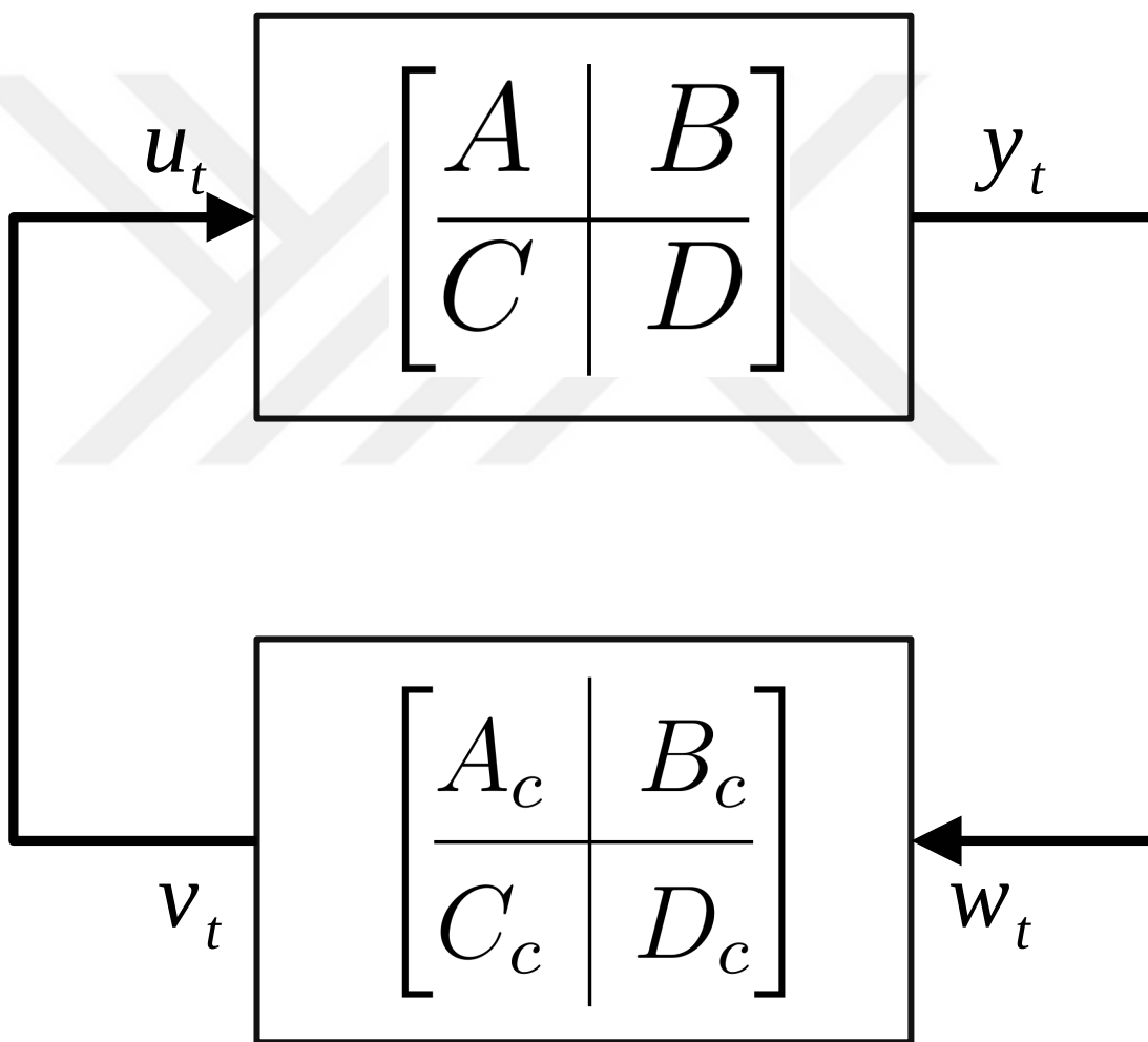
Figure 5.1: The closed loop system diagram with the fixed-order controller.
