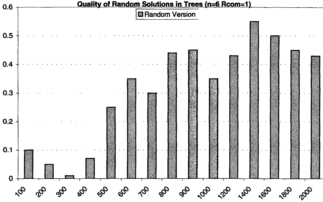
Figure 5.1: Percent relative distance of the best solutions provided by 100000 runs of the randomized multilevel assignment algorithm on trees
