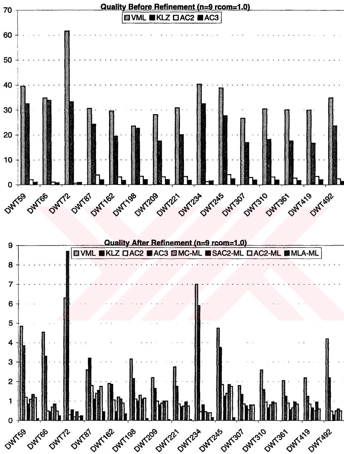
Figure 5.8: Percent qualities of algorithms for 9-processor systems in general graphs
