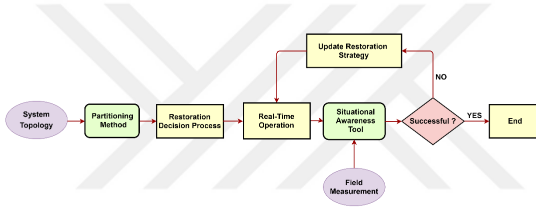
Figure 1.1. The flow chart of the restoration procedure.
