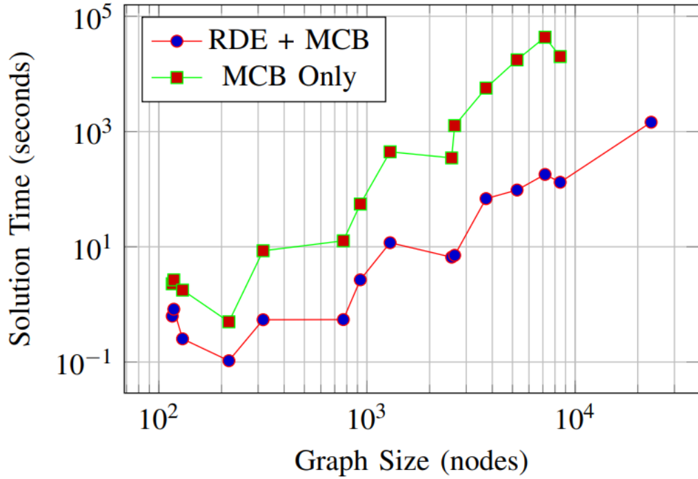
Figure 5.2. Performance of IRS using (i) MCB only, and (ii) RDE followed by MCB
