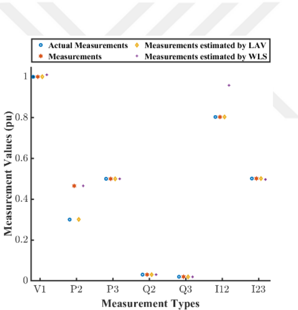
Figure 5.4. Comparison of WLS and LAV estimation under biased measurements
