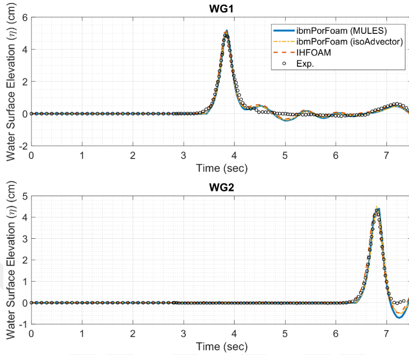
Figure 6.16. Comparison of water surface elevations of the numerical models with the experimental data: ibmPorFoam (MULES) (solid blue line), ibmPorFoam (isoAdvector) (dotdashed yellow line), IHFOAM (dashed orange line), Experiment (black circles)
