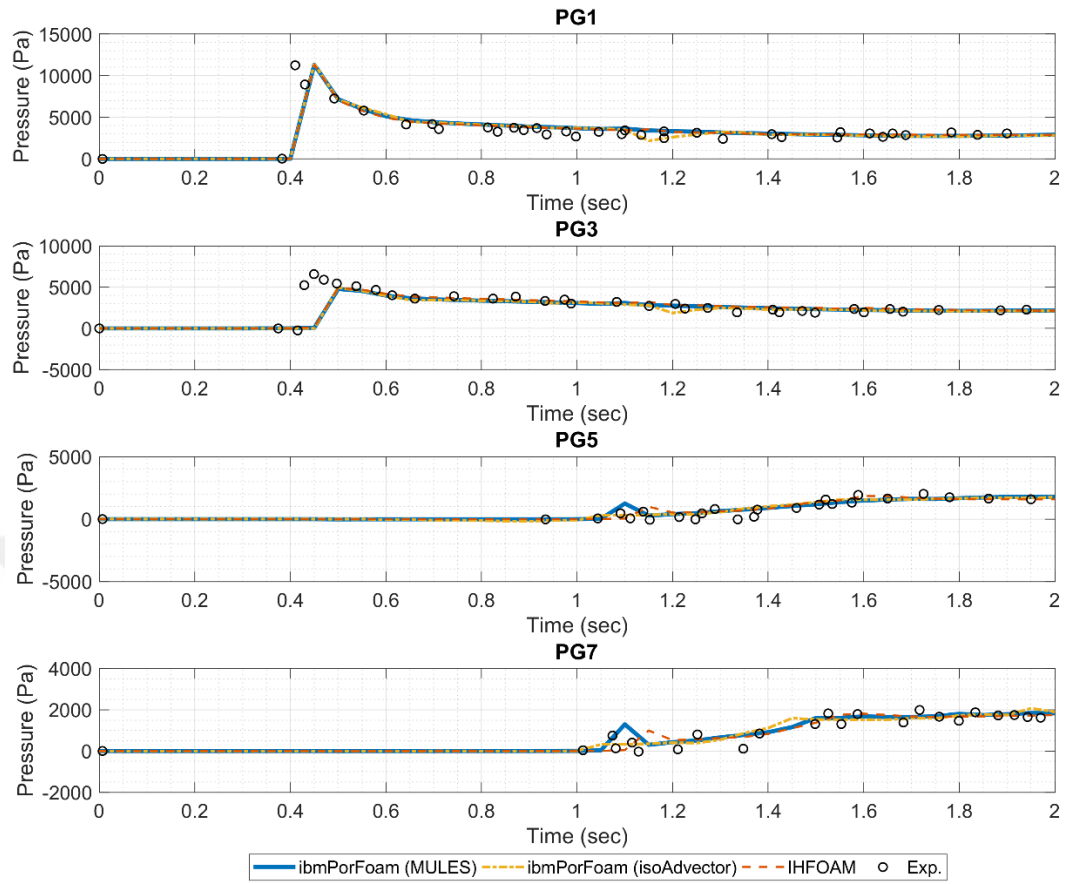
Figure 6.4. Comparison of pressure values of the numerical models with the experimental data: ibmPorFoam (MULES) (solid blue line), ibmPorFoam (isoAdvector) (dotdashed yellow line), IHFOAM (dashed orange line), Experiment (black circles)
