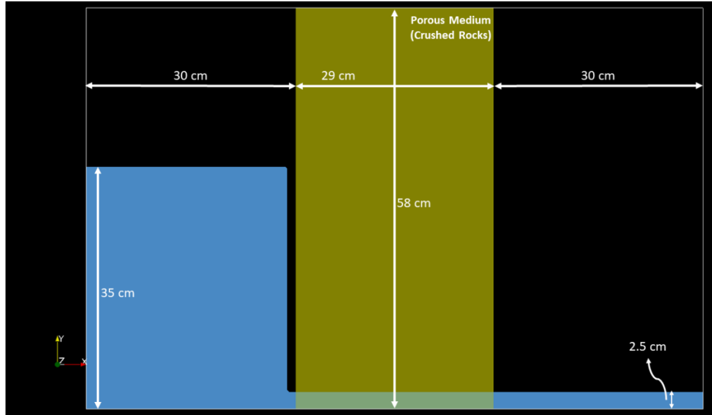
Figure 6.9. Experimental setup
