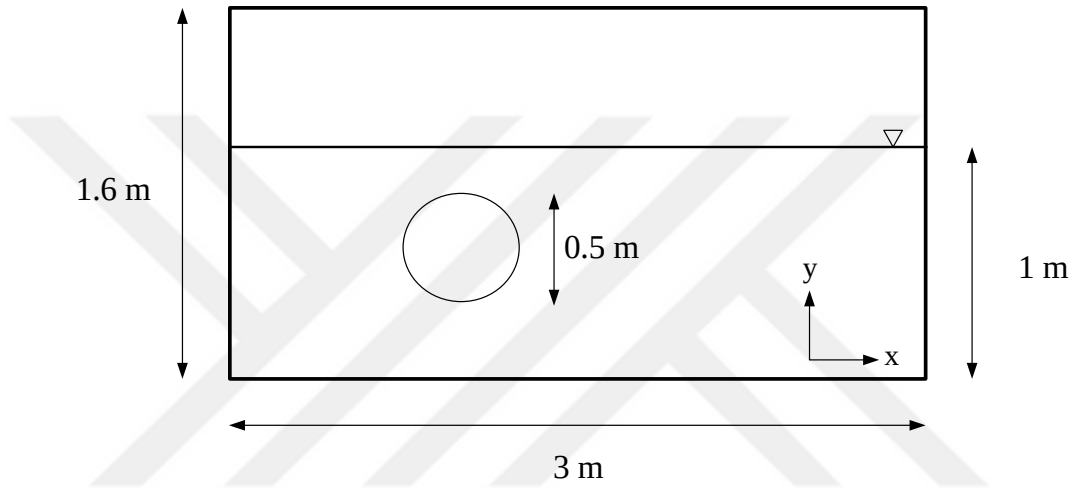
Figure 6.23. Dimensions of the computational domain
