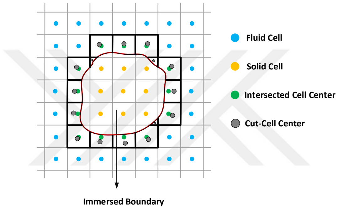
Figure 5.4. Schematic representation of the cut-cell immersed boundary method
