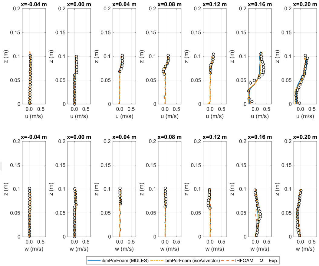
Figure 6.19. Comparison of the velocity profiles along the selected lines of the numerical models with the experimental data at t=6.1 sec: ibmPorFoam (MULES) (solid blue line), ibmPorFoam (isoAdvector) (dotdashed yellow line), IHFOAM (dashed orange line), Experiment (black circles)
