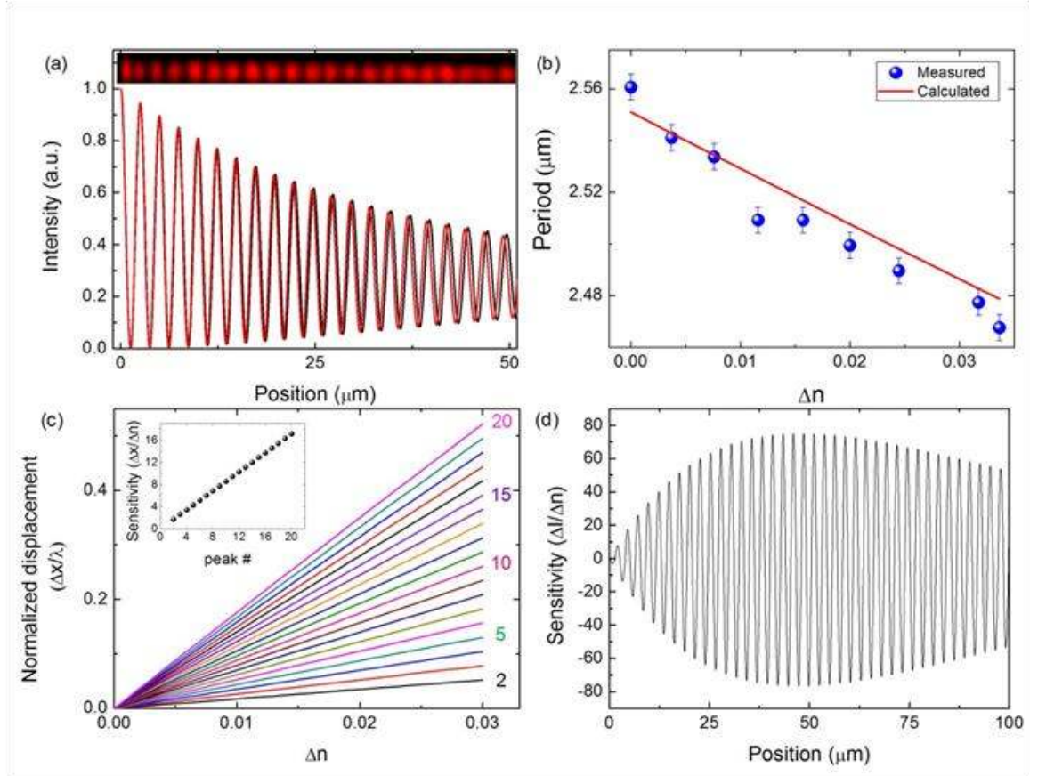
Figure 5.6 (a) Calculated interference fringes for two different index of refraction ( n=1.33 , black curve, n=1.34 , red curve) generated by a plasmon interferometer with a length of 50 \mu\text{m} and a slit-groove angle of 10 \text{ deg} . The inset shows the CCD image of the interference fringes. (b) Measured and calculated period of the fringe pattern as a function of change of index of refraction. (c) Normalized displacement of the fringes as a function of change of index of refraction. The inset shows the sensitivity as a function of fringe index. (d) Normalized intensity change along the slit position.
