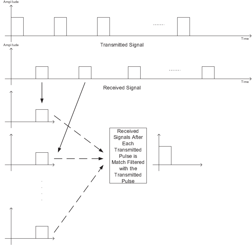
Figure 2.3: Match filtering process for pulse burst waveforms.
