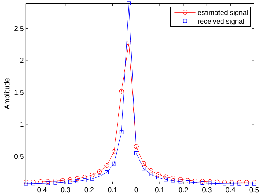
Figure 5.9: Received signal from one VAB armored vehicle and estimated signal found by using the optimal solution or successive cancelation.
