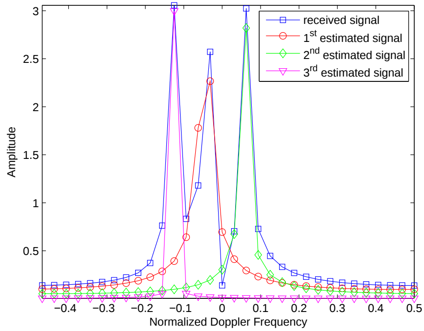
Figure 5.15: Received signal from three VAB armored vehicles and estimated signal found by using successive cancelation.
