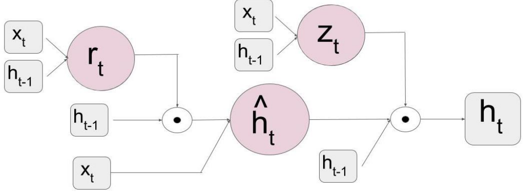
Figure 3: The GRU architecture
