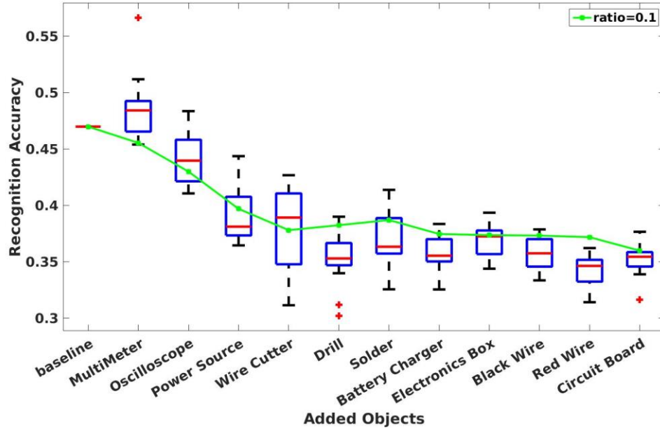
Figure 22: Recognition success in an gradual learning environment in the first step. The robot takes pictures and adds new objects one by one. The displayed values are the highest accuracy.
