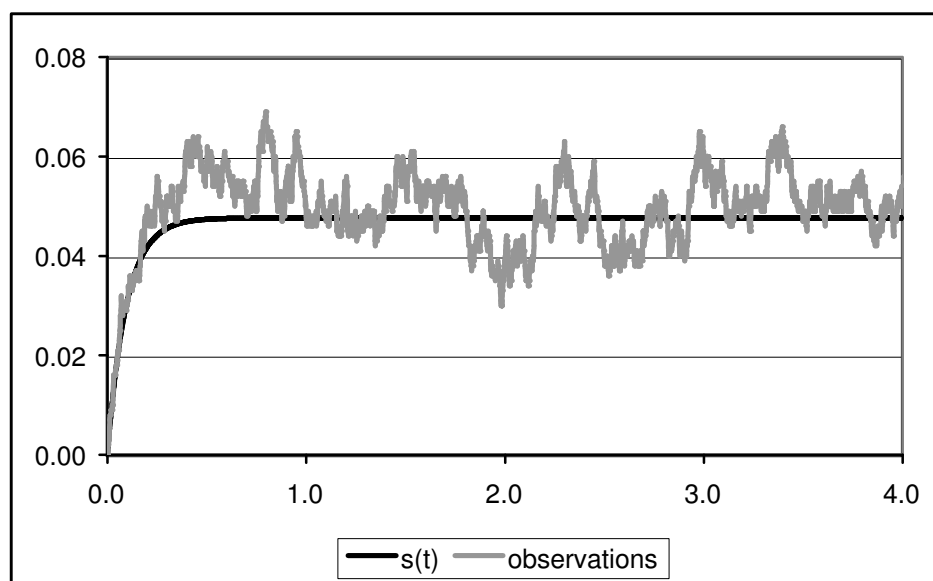
Figure A.1: Model 2: Simulation of trajectory of failed devices for reliability model with replacement ( \lambda_0 = 0.5 , \beta_0 = 1 , T = 5 , m = 10 )
