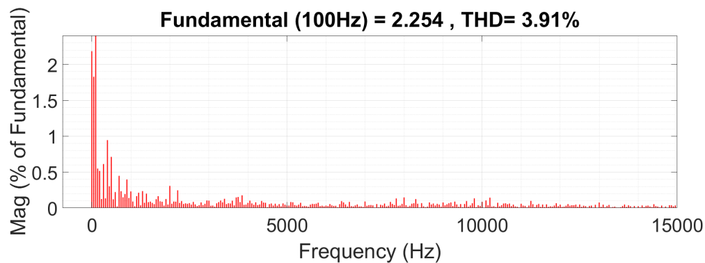
Figure 5.14: NTV Phase B Current FFT Result
