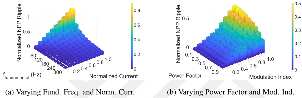
Figure 3.12: SVPWM Low Frequency NPP Ripple
