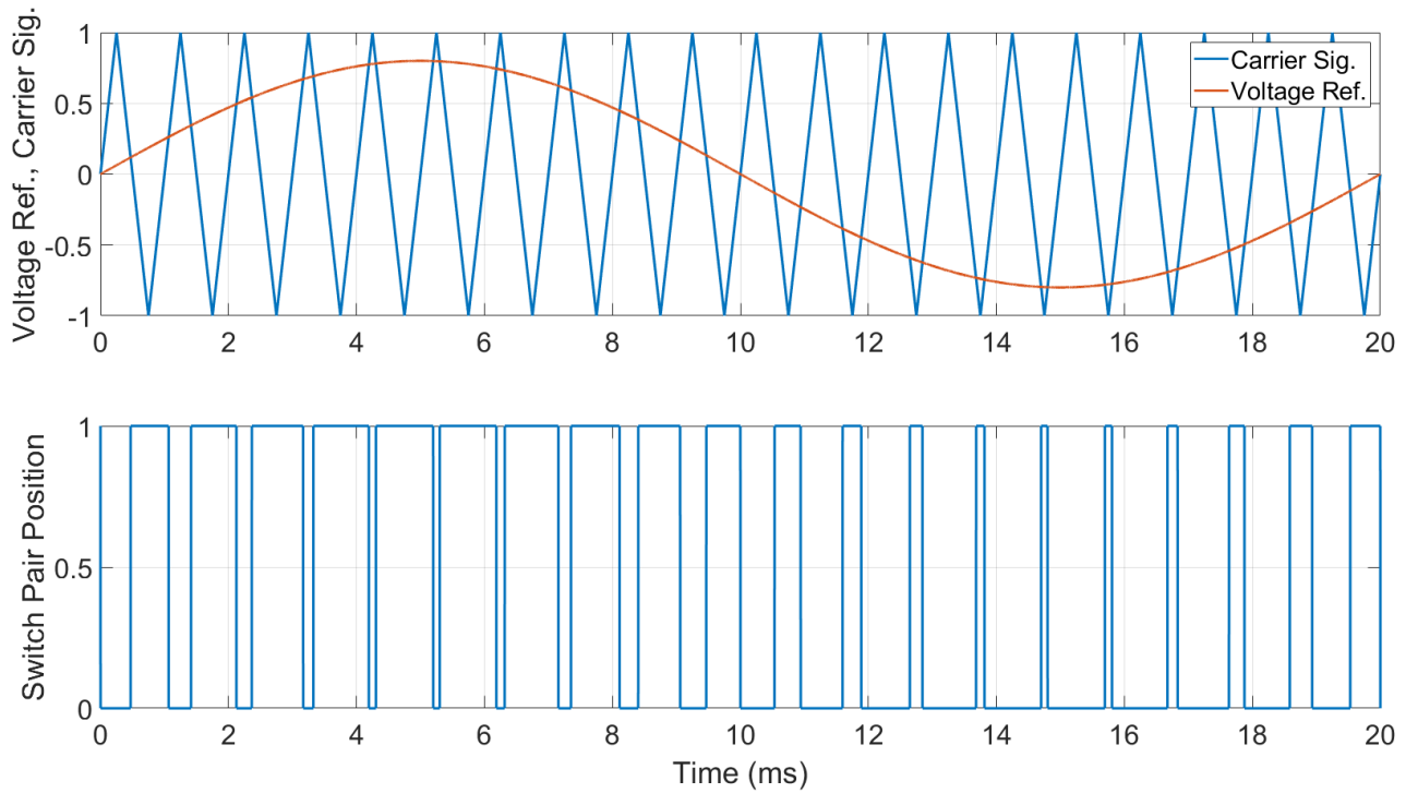
Figure 2.2: Illustration of Comparison Step of SPWM Method
