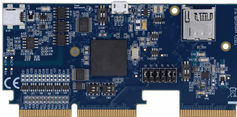
Figure 5.7: Digital Control Card (TMDSCNCD28379D)[54]
