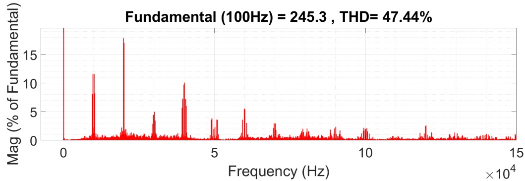
Figure 5.19: Carrier Based Method Line-to-Line Voltage FFT Result
