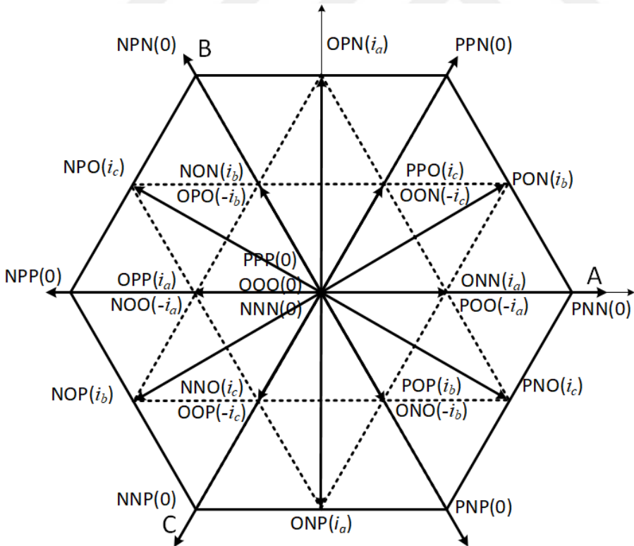
Figure 3.5: Equivalent Neutral Current of Each Vector
