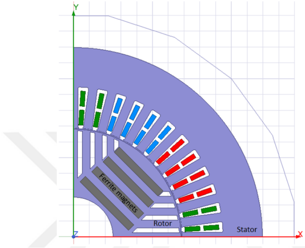
Figure 4.1: Structure of the PMaSynRM
