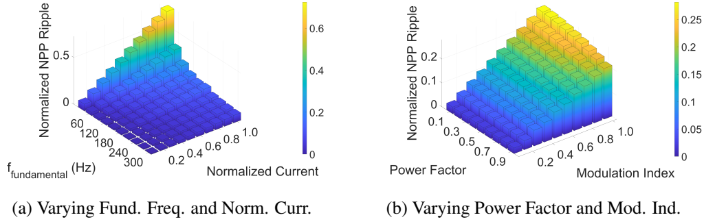
Figure 3.11: SPWM Low Frequency NPP Ripple
