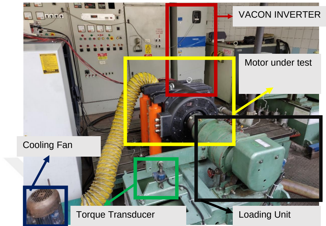
Figure 2.5. Test Setup, Including the Load System, Inverter, and the Motor Under Test
