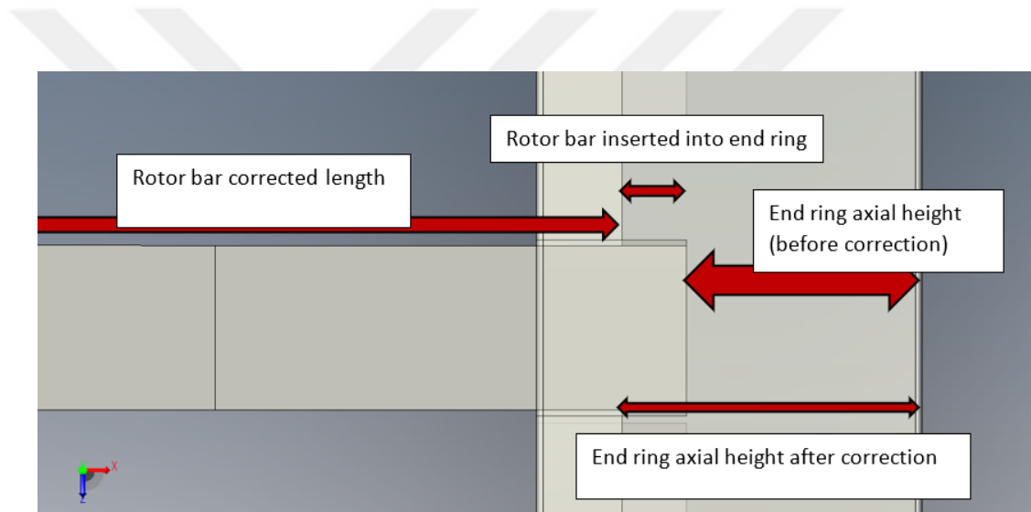
Figure 3.12. 2D Schematic of the Rotor Bar and Rotor End Ring Connection of the Actual Motor
