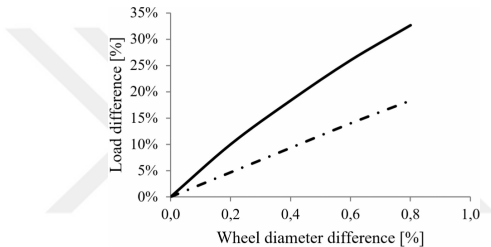
Figure 1.10. The Load Sharing Between Two Parallel Connected Motors Using either an Aluminum Rotor (Dashed Line) or a Copper Rotor (Solid Line)
