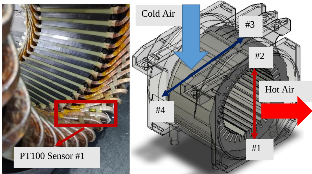
Figure 4.3. PT100 Locations
