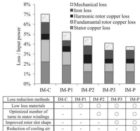
Figure 1.1. FEA Results for Losses in Traction Motors
