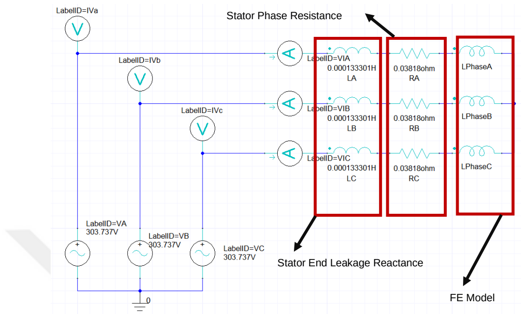
Figure 2.10. A Typical External Circuit with End Winding Parameters Used by FE Calculations
