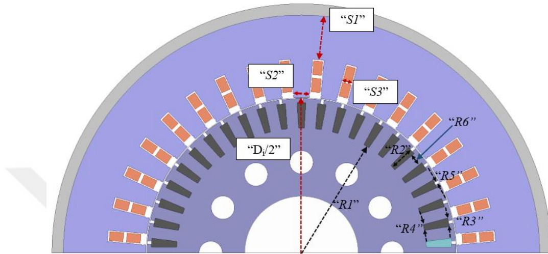
Figure 3.11. Stator and Rotor Lamination Schematics in Prototype-006
