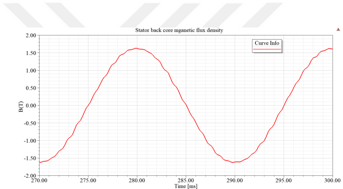
Figure 2.15. Averaged Stator Back Core Flux Density Along the “S1”Cross Section” w.r.t Time
