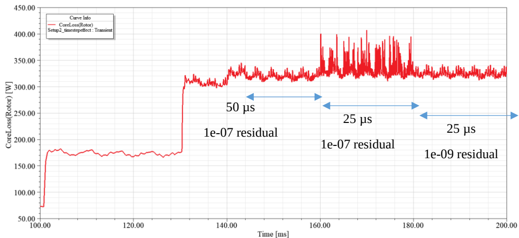
Figure 3.1. Effect of Time Step and Convergence Criteria on Transient Solution
