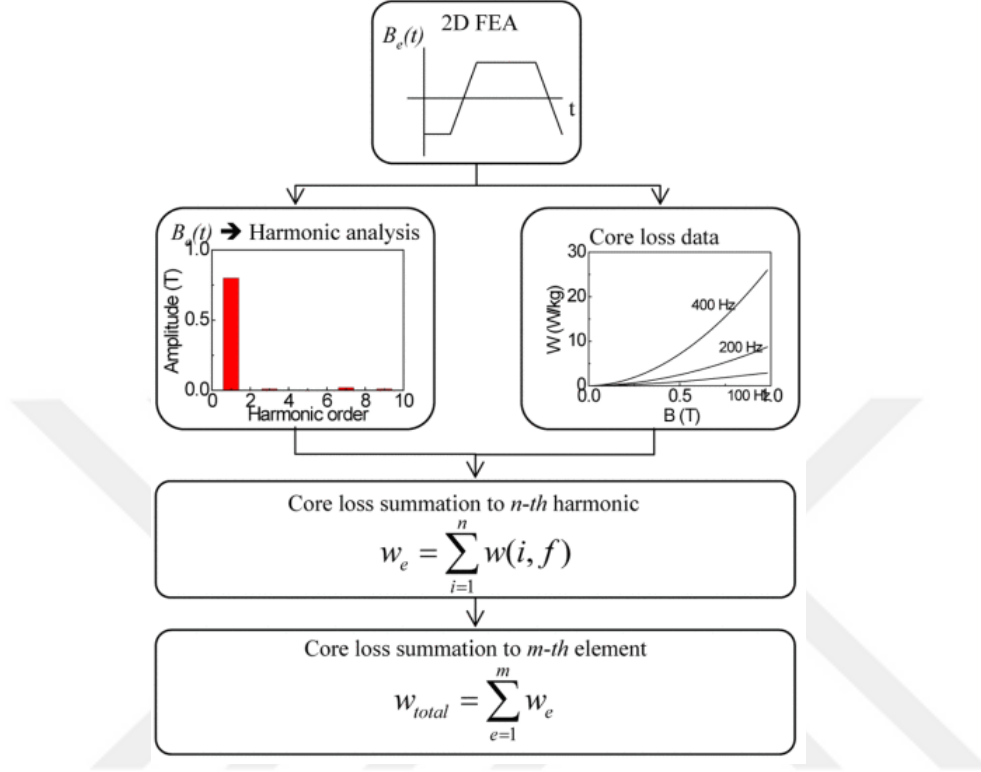
Figure 1.12. Core Loss Calculation Process
