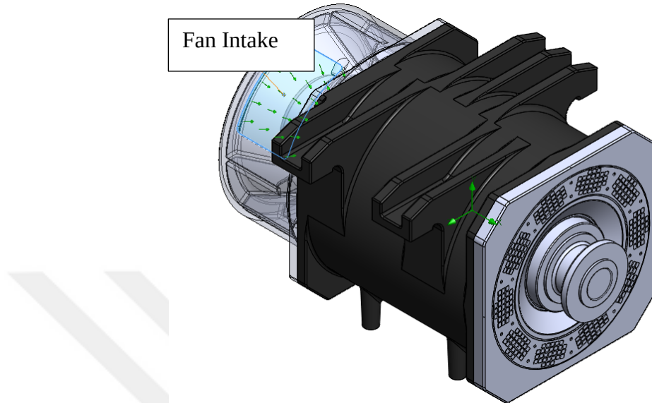
Figure 3.7. Motor's Geometry
