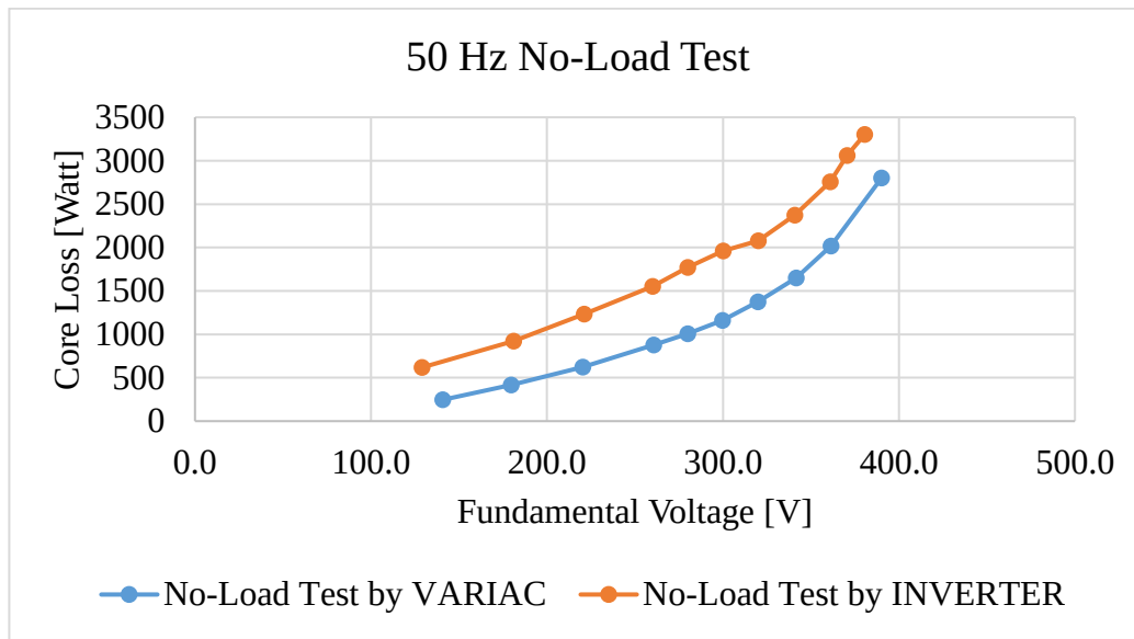
Figure 4.5. 2 nd Prototype- 50 Hz No-Load Test comparison Plot, Inverter Vs. Sinusoidal source
