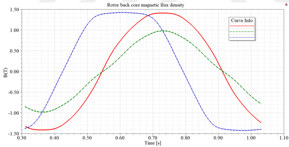
Figure 2.17. “Averaged Rotor Yoke Flux Density along the Cross Sections” w.r.t Time (Solid Red- R.1, Dot Dash Blue- R2.2, and Dashed Green- R2.3)
