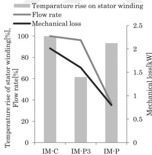
Figure 1.3. Reduction of Mechanical Loss
