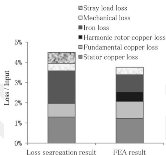
Figure 1.4. Determination of Losses
