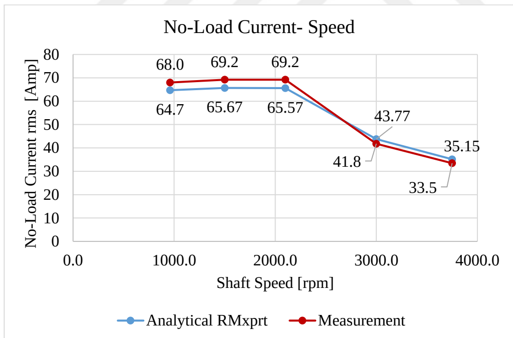
Figure 4.11. No-Load Current– Speed Characteristics. RMxpirt vs. Measurements
