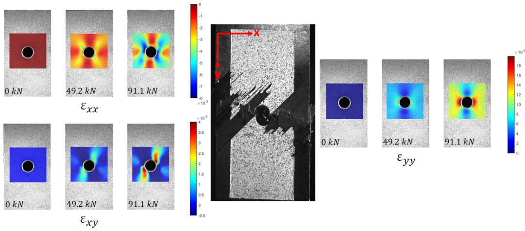
Figure 5.12: Change of strain distribution on the OHT3-3-2 test specimen up to the failure.
