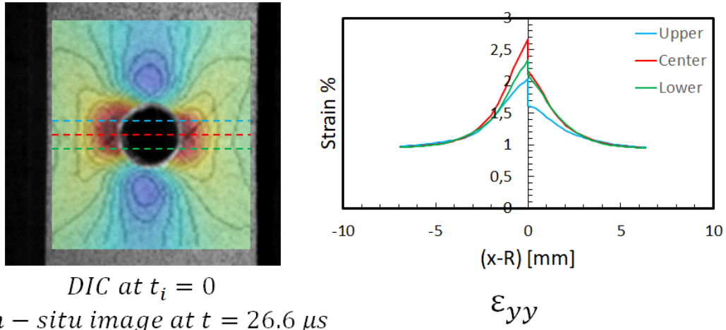
Figure 5.8: Strain field and strain plot along the paths shown by dashed lines.
