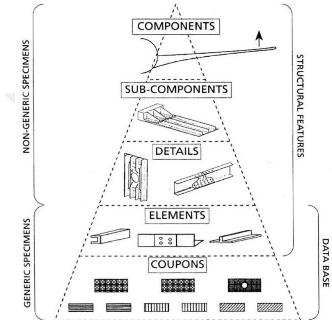
Figure 1.3: Schematic diagram of certification tests [5].
