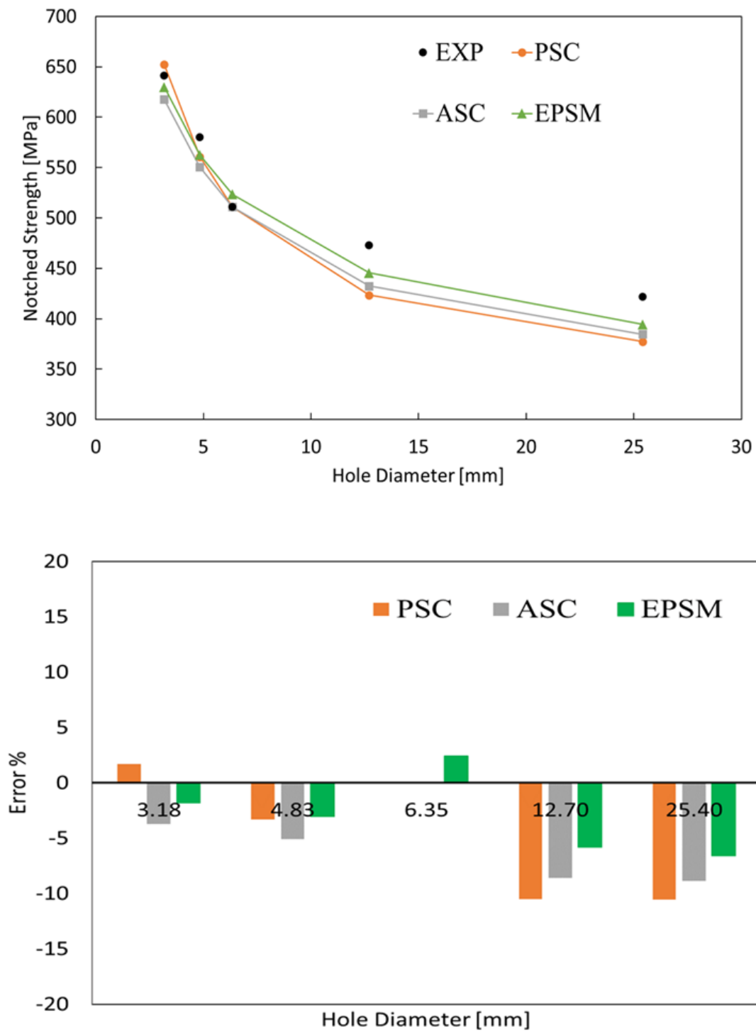
Figure 5.14: Comparison of experimental and analytical results of OHT2 family specimens.
