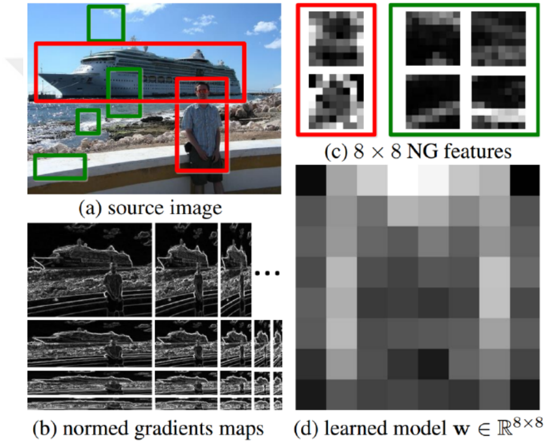
Figure 2.1: BING Algorithm. (a) Red boxes present objects while green ones present non-objects. (b) Image are resized with different scales and ratios, normed gradient maps are extracted for each scale. (c) normed gradient features for boxes given in (a). (d) linear model weights for normed gradient features. Taken from [25].
