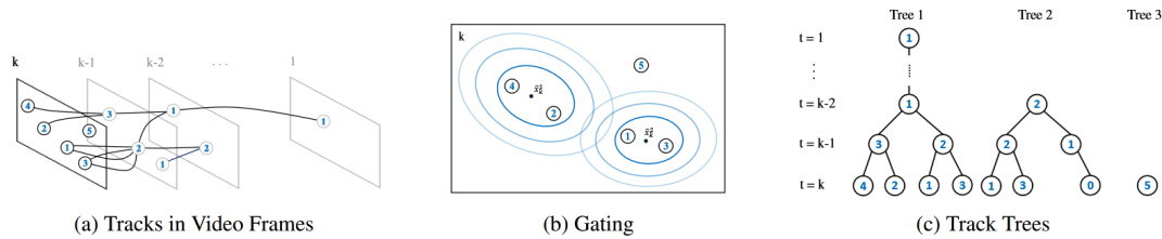
Figure 5.1: MHT. (a) (A subset of) tracklets (hypotheses) at time k . (b) Sample gating areas for two tracklets with different thresholds. (c) Respective track trees whose nodes are related with an examination in (a). Taken from [14].
