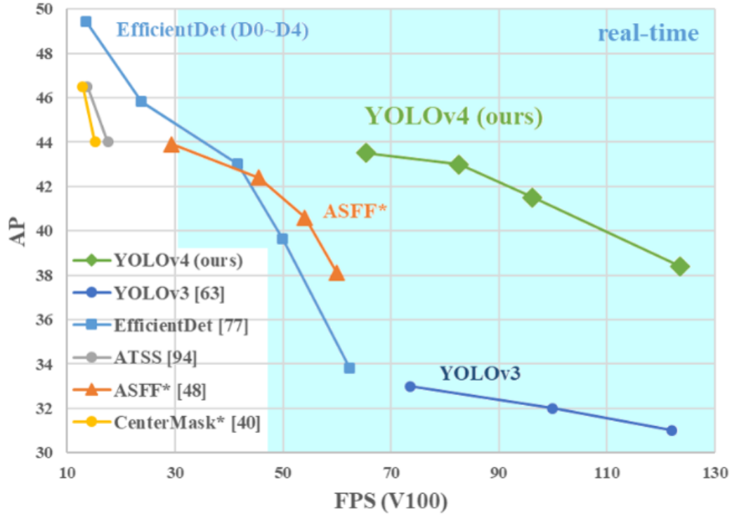
Figure 2.13: Comparison of YOLOv4 and the other state-of-the-art algorithms when the paper is introduced. Taken from [46].
