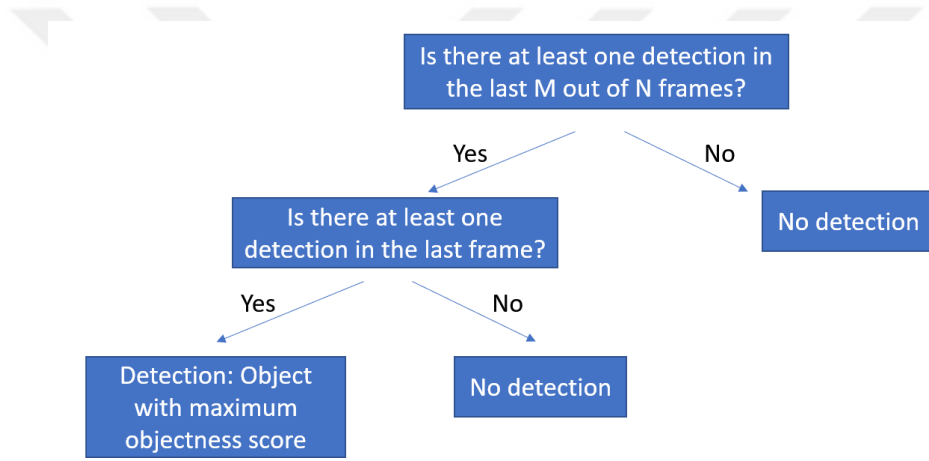
Figure 5.2: M/N (M-out-of-N) Flowchart.
