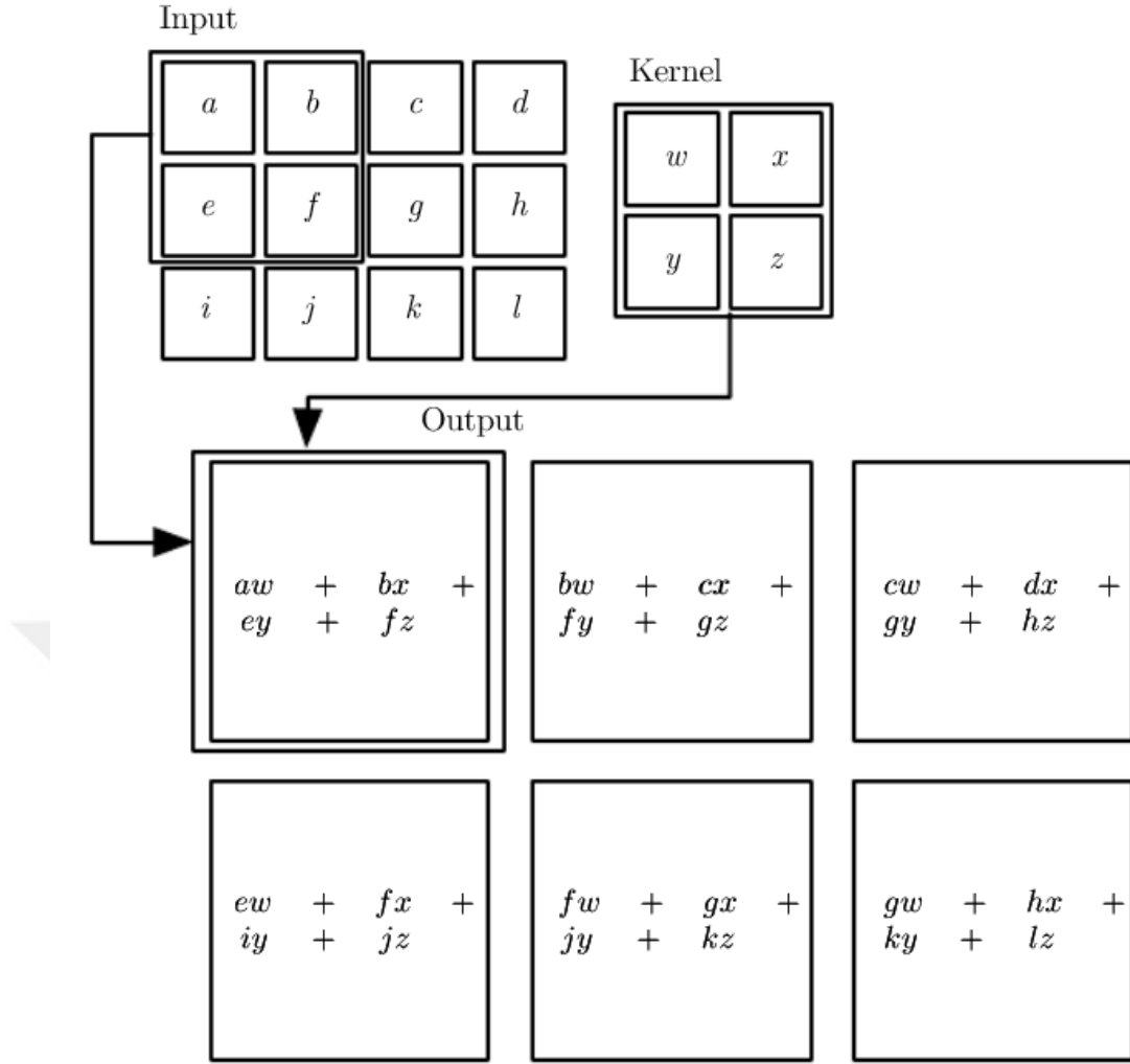
Figure 2.2: Sample 2D Convolution operation. Taken from [28].
