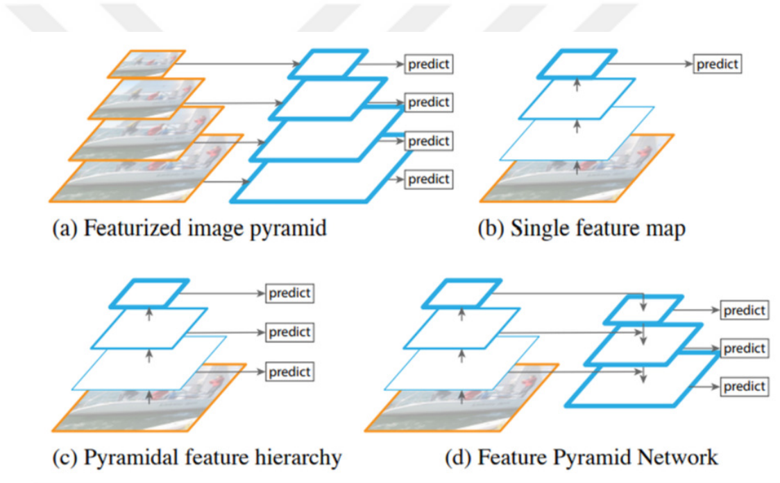
Figure 2.7: Feature pyramid alternatives. (a) Most straight forward solution since every size has its own network. Therefore, the network is very slow. Used in [42]. (b) One prediction at the end of the network. Gradients might vanish for small objects. Used in [43, 37, 38]. (c) Different predictions for different layers but previous layer prediction cannot use deeper layer information. Used in [4] (d) Feature pyramid network. Taken from [41] where this method is also proposed.
