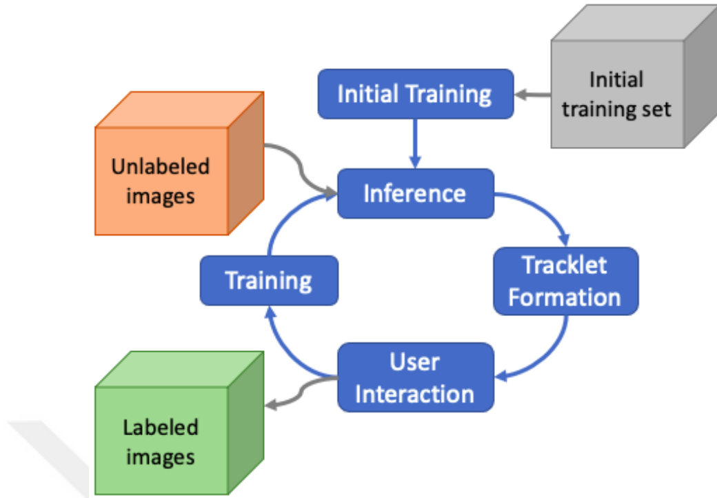
Figure 4.1: Proposed annotation scheme
