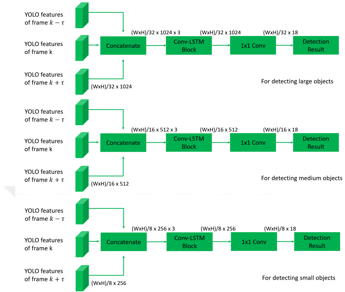
Figure 6.3: Proposed YOLOv5-LSTM Structure
