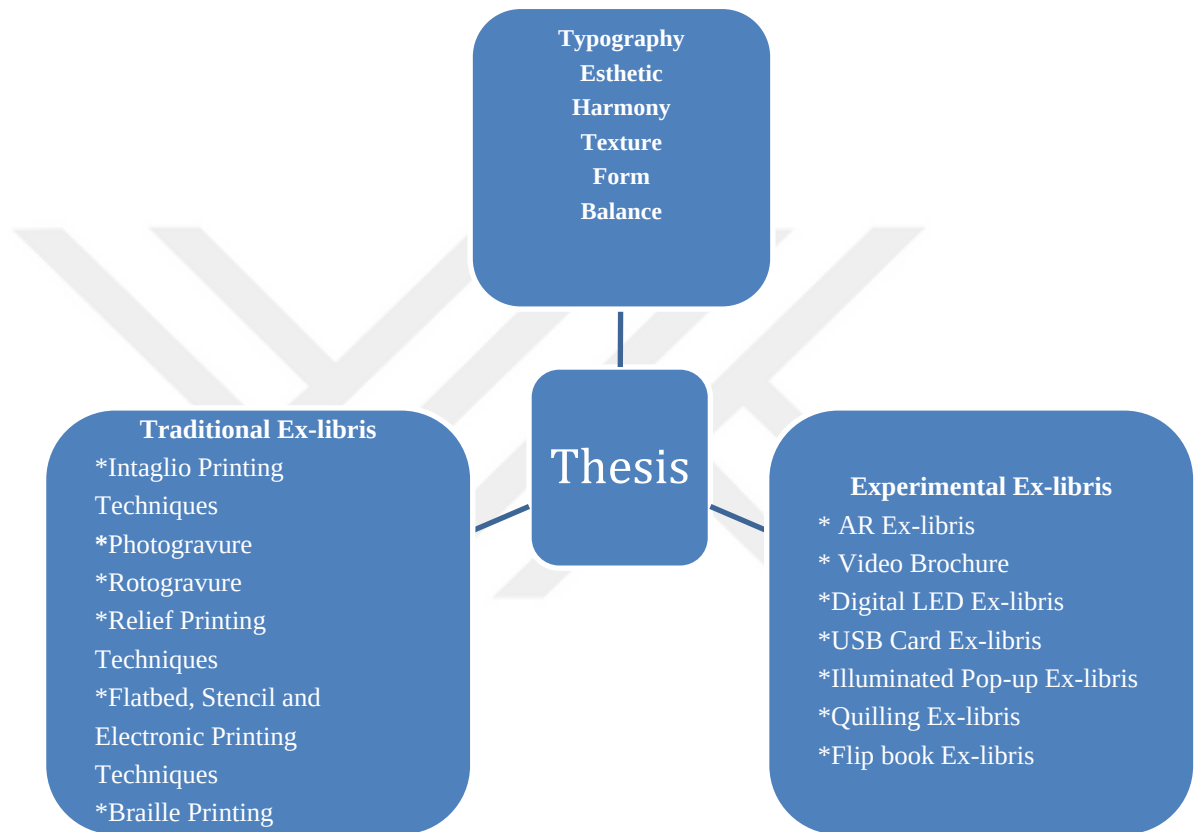
Figure 5.1. Thesis scheme
