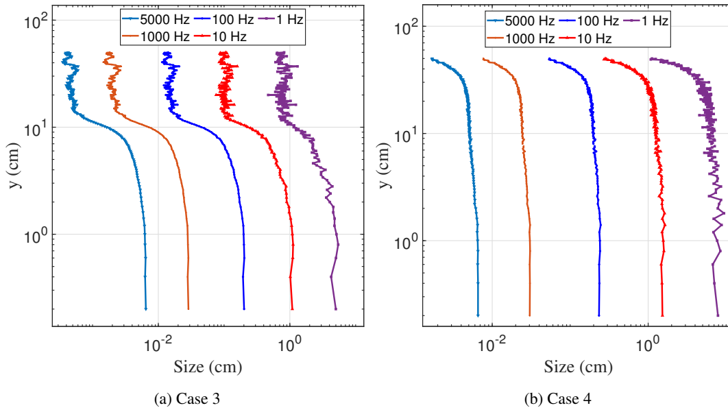
Figure 5.17: The size variation of eddies at different frequencies along the boundary layer (from raw data of Abdulrahim et al. [1])
