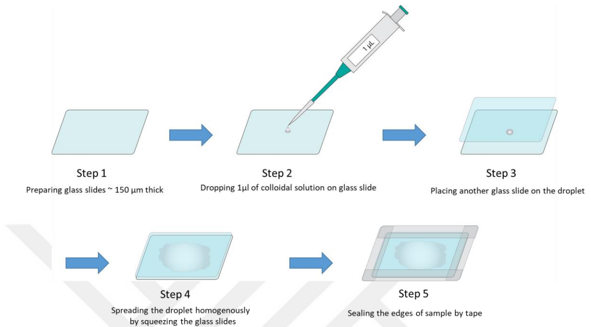
Figure 3-2 Sample preparation steps; 1 \mu\text{L} of colloidal solution was sandwiched between two thin glass slides to form a thin layer of colloidal solution, edges of the sample were sealed carefully in order to keep the sample from drying out and prevent any pressure difference throughout the sample.
