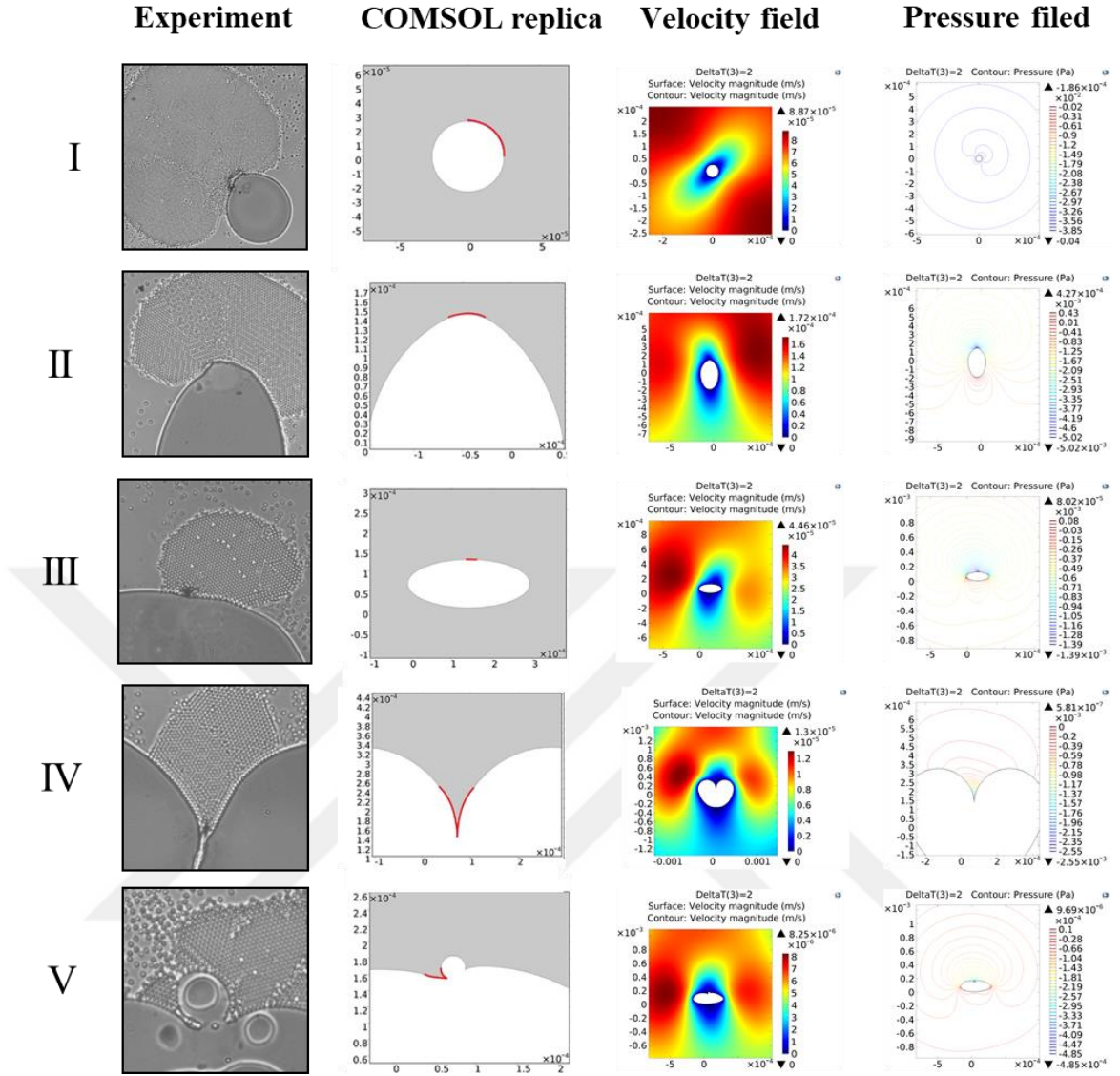
Figure 4-15 Simulated fluid velocity fields and pressure fields for replicated physical boundaries, I) Spherical bubbles; II) Elliptical bubbles; III) Flat bubbles; IV) V-shaped bubbles; V) a spherical bubble on flat bubble.
