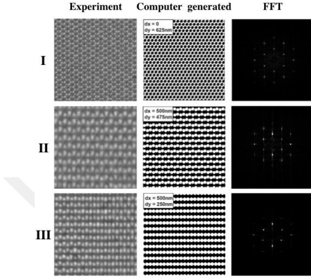
Figure 4-5 Bright field microscope images, computer generated lattices and FFTs of experimental honeycomb lattices. Depending on the shifting ratio, various types of Honeycomb patterns can be observed in the system.
