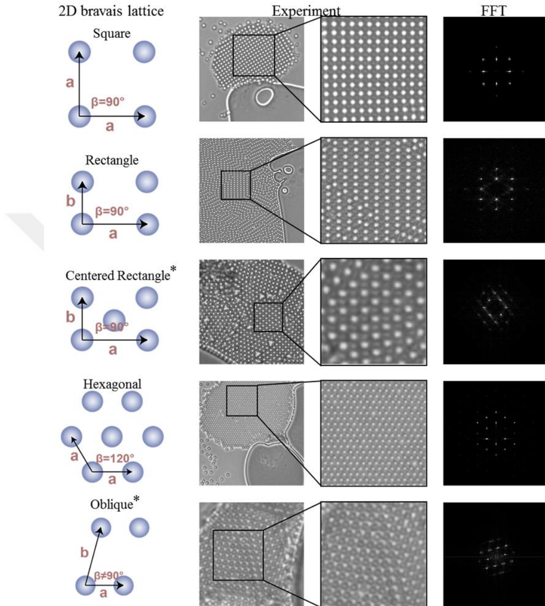
Figure 4-1 Microscope images show all 2D Bravais lattices of colloids formed in our experiments. Except hexagonal patterns that can be formed in one layer, all the other patterns are formed of at least two layers of particles therefore they are quasi 2D patterns. Centered rectangular patterns and oblique patterns were rarely observed.
