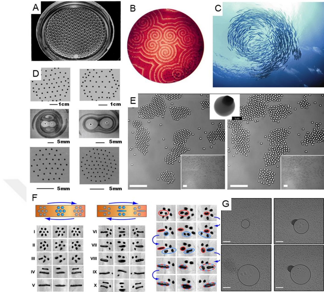
Figure 2-4 Examples of dynamic self-assembly and organization in scientific literature; A) Rayleigh-Bénard convection cells in silicone oil under an air surface 48 ; B) Belousov-Zhabotinsky reaction, a classical example of non-equilibrium self-assembly, C) Dynamic self-organization of a school of fish; D) Dynamic self-assembly of magnetically-rotating millimeter-sized disks at the liquid-air interface 11 ; E) Living crystals, dynamic self-assembly of TPM (3-methacryloxypropyl trimethoxysilane) polymeric spheres with embedded hematite cubes under the blue light (left), and melting of colloidal clusters when light is turned off (right; scale bar is \sim 10 \mu\text{m} ) 9 ; F) Switching between dynamic and static self-assembly of ferrofluid droplets on super hydrophobic surface by changing between static magnetic field to time varying magnetic fields 10 ; G) Dynamic self-assembly of pure polystyrene spheres far from equilibrium using laser-induced flows (scale bar is \sim 40 \mu\text{m} ) 4 . [Reprinted with permission from (A) Ref 48 ; (D) Ref 11 ; (E) Ref 9 ; (F) Ref 10 ; (G) Ref 4 ].
