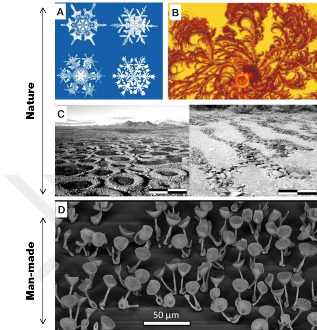
Figure 2-1 Examples of self-assembly and self-organization in nature; A) Photographs of snowflakes exhibiting various self-organized patterns (magnification \times 400 ) 23 ; B) A pseudo-colored image of patterns formed by swarming Paenibacillus Dendritiformis bacteria 23 ; C) Types of self-organized sorted pattern ground that shows circles (left; scale bar \sim 2\text{m} ) and stripes (right; scale bar \sim 1\text{m} ) 24 . Examples of self-assembly and self-organization that mimicks similar pattern formations seen in nature under laboratory conditions; D) Carbonate-silica microstructures developed in a dynamic reaction-diffusion system by carefully controlling diffusion of carbon dioxide in barium chloride and sodium metasilicate solution 25 . [Reprinted with permission from (A,B) Ref 23 ; (C) Ref 24 ; (D) Ref 25 .]
