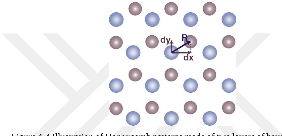
Figure 4-4 Illustration of Honeycomb patterns made of two layers of hexagonal lattices shifted on top of each other. R is the shifting vector, where dx the x component of R direction and dy is the y component of R .
