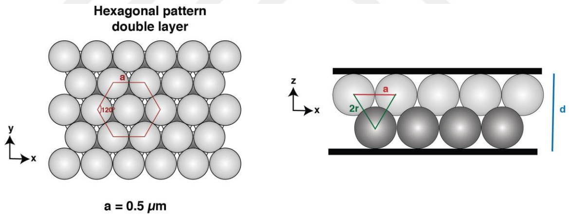
Figure 4-20 Top and cross section view of computer generated double layer hexagonal pattern.
