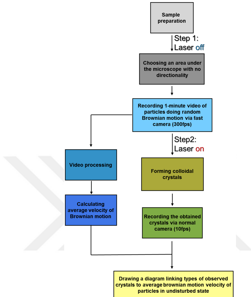
Figure 3-6 The steps taken to obtain average Brownian motion velocity for each pattern; starting with sample preparation, then finding an area under the microscope which shows no directionality (particles are doing random Brownian motion without moving toward any specific direction) and recording 1-minute video of particles doing random Brownian motion when laser is blocked, with fast camera (300fps). Next step is to create colloidal crystals in the same area and document the observed patterns. Lastly, we perform video processing on the 1-minute Brownian motion video to obtain average Brownian velocity corresponding to the observed patterns.
