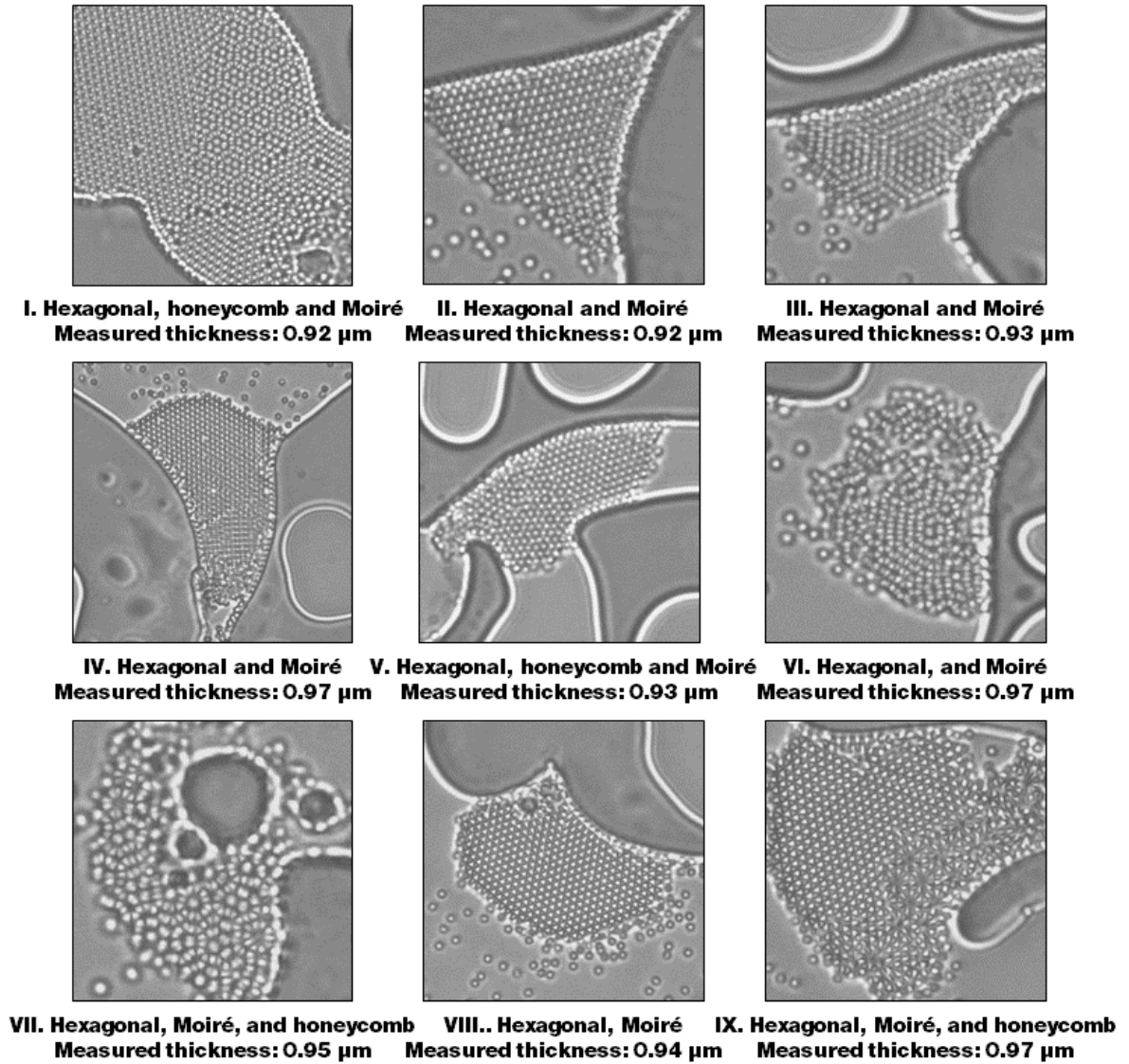
Figure 4-32 Formation of four different patterns (Double layer hexagonal, honeycomb, Moiré and Quasicrystal) one spatial area.
