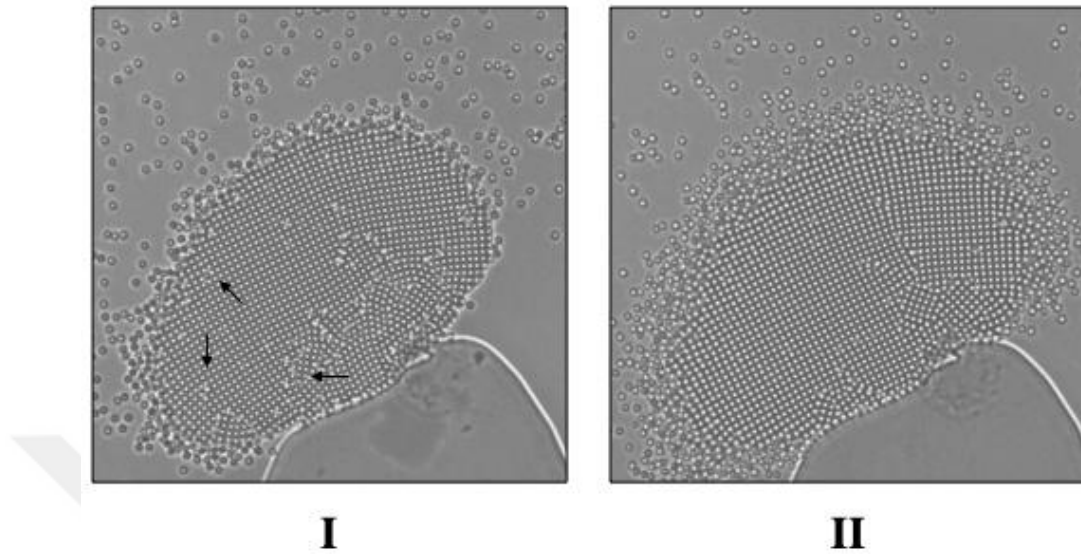
Figure 4-13 Self-healing of a square pattern; I) arrows showing vacancies and defects, II) self-healed square pattern after 10 seconds.
