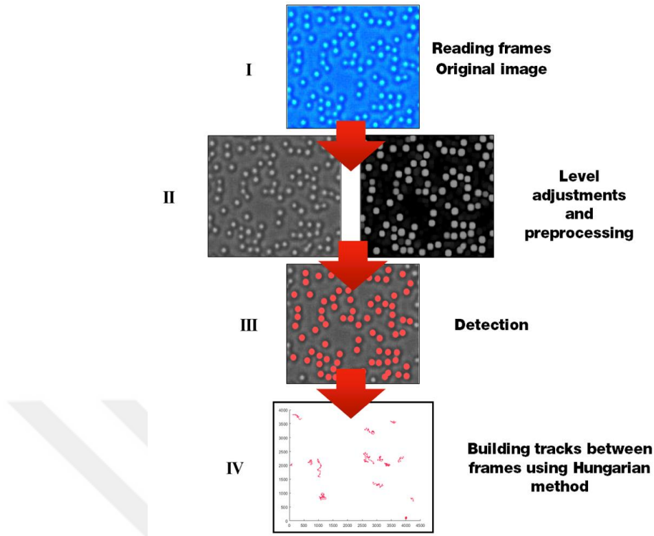
Figure 3-7 Steps of video processing algorithm, I) starting with reading the videos frame by frame; II) Next step is to adjust levels and perform some preprocessing steps; III) Detection of particles for each frame; IV) Linking the detected particles in each frame to other frames to draw the trajectories.
