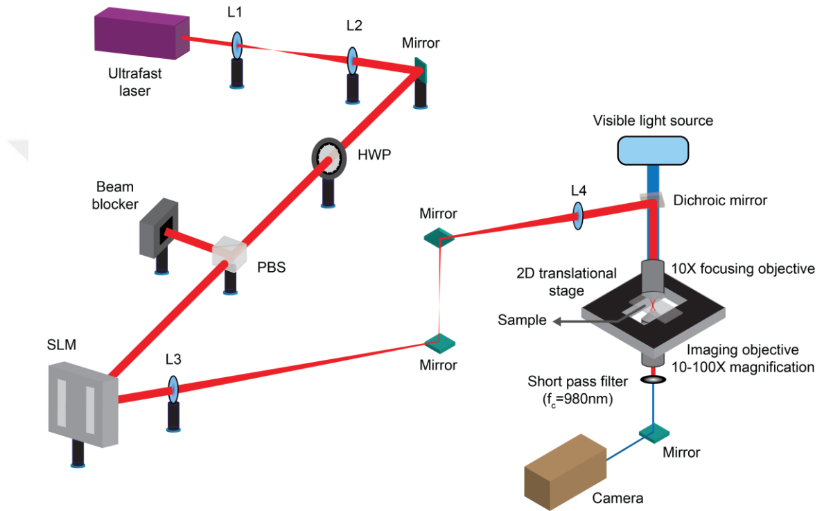
Figure 3-1 Schematic illustration of the experimental setup; An ultrafast laser beam is directed through an optical path to shine on the sample through an inverted microscope, which is connected to a camera for imaging. (Abbreviations: L: Lenses; HWP: Half-Wave Plate (the power controller); PBS: Polarizing Beam Splitter; SLM: Spatial Light Modulator).
