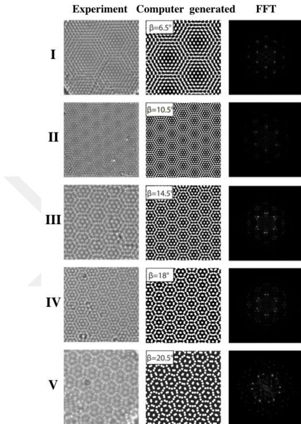
Figure 4-3 Various types of Moiré patterns can be observed depending on their misorientation angles, their computer generated replicas (drawn in Adobe illustrator 2018), and FFT pattern of experimentally obtained patterns.
