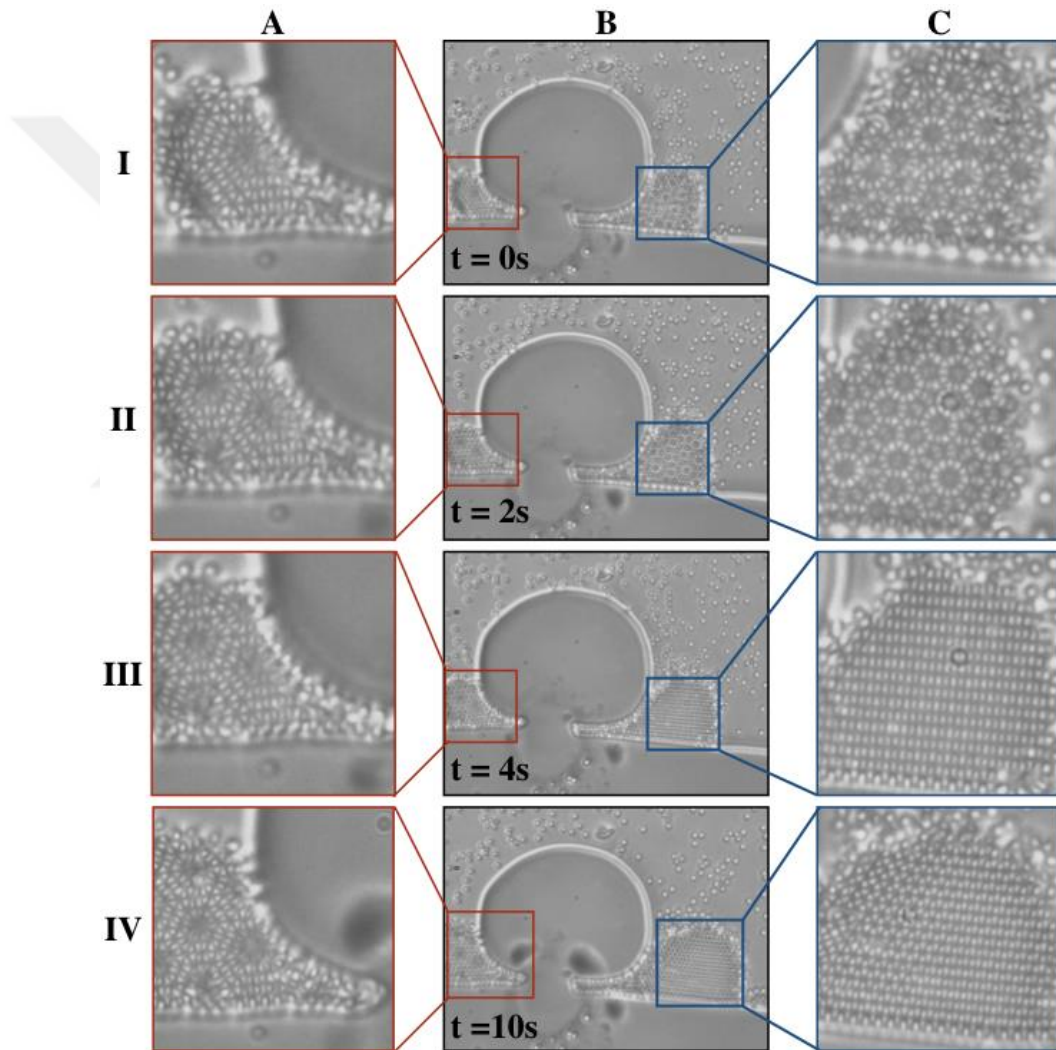
Figure 4-9 Dynamic behavior of far from equilibrium colloidal crystals; Starting with I-A) Moiré patterns, and I-C) quasicrystals at t = 0 , s which changes to II-A) another type of Moiré patterns at t = 2 s, and III-C) type three honeycomb at t = 4 s and IV-C) type two honeycomb at t = 10 s.
