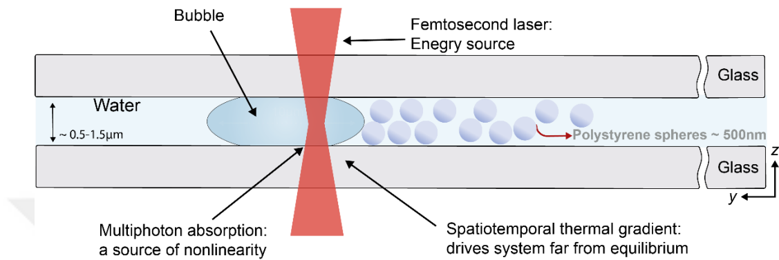
Figure 2-5 An illustration showing the cross-section arrangement of the experimental setting, where a colloidal solution is sandwiched between two thin glass slides with a femtosecond laser beam focused on the sample, due to the localized heat deposition the water boils down and creates a vapor bubble, which serves as a physical boundary for particles to hit and collect 4 .
