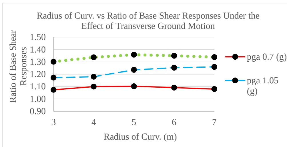
Figure 51. Radius of Curvature and Ratio of Base Shear Responses of Uplift-Restricted case to Uplift-Allowed Case (Investigated Under the Effect of Transverse Motion Considering Three Different PGA values)
