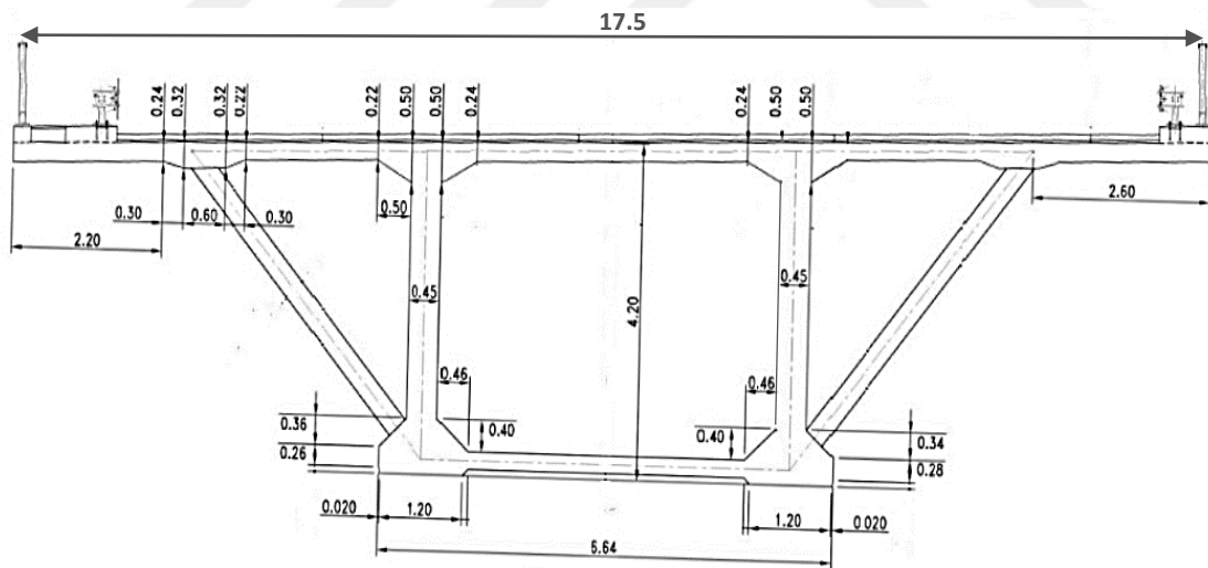
Figure. 3 Bridge Deck Cross Section
