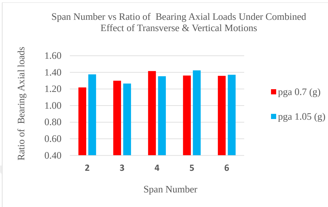
Figure 23. Span Number and Ratio of Bearing Axial Load of Uplift-Restricted Case to Uplift-Allowed Case (Investigated Under the Combined Effect of Transverse and Vertical Motions Considering Two different PGA values)
