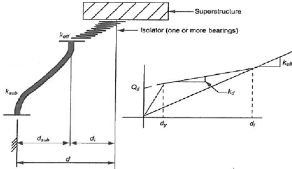
Figure 7. Sliding Isolator and Substructure Deformations Due to Lateral Load
