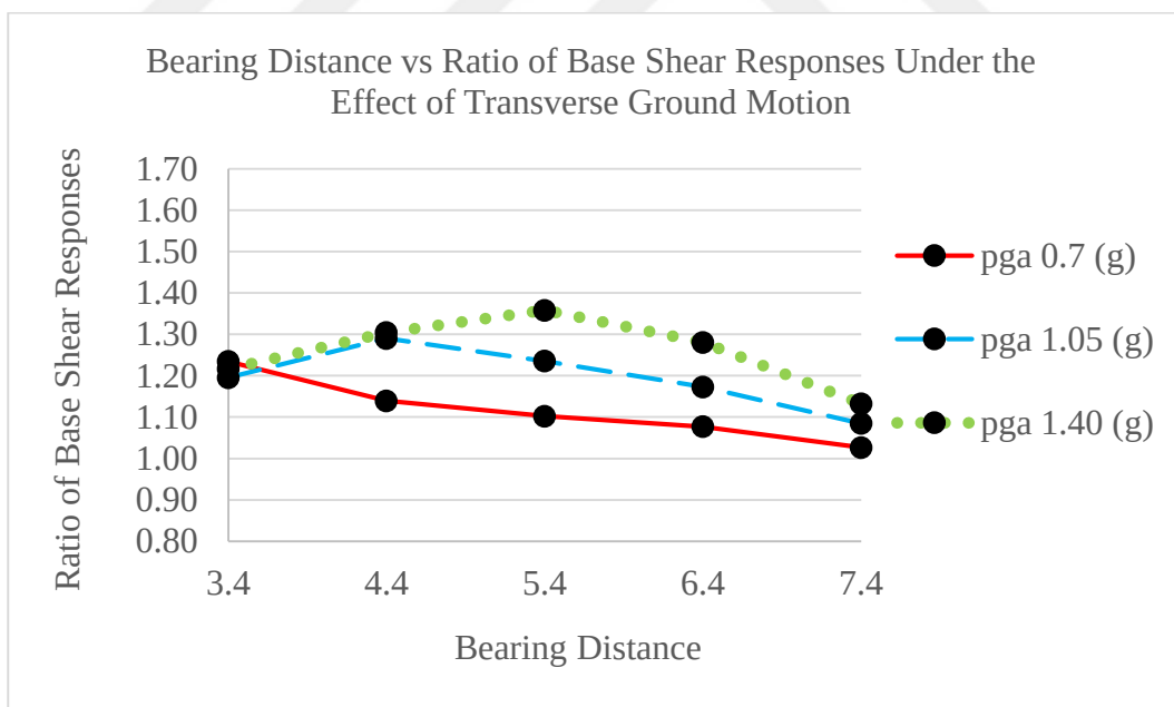
Figure 25. Bearing Distances and Ratio of Base Shear Responses of Uplift-Restricted Case to Uplift-Allowed Case (Investigated Under the Effect of Transverse Motion Considering Three Different PGA values)
