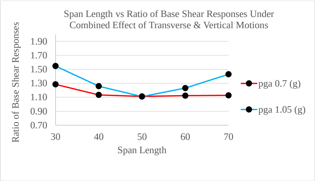
Figure 34. Span Length and Ratio of Base Shear Responses of Uplift-Restricted Case to Uplift-Allowed Case (Investigated Under the Combined Effect of Transverse and Vertical Motions Considering Two Different PGA values)
