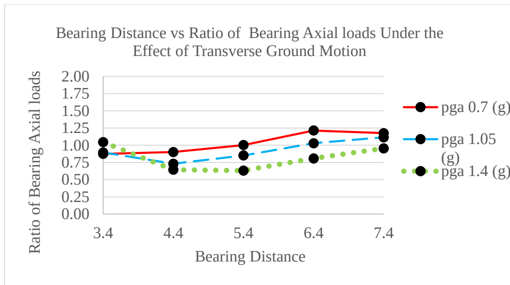
Figure 26. Bearing Distances and Ratio of Bearing Axial Loads of Uplift-Restricted Case to Uplift-Allowed Case (Investigated under the Effect of Transverse Motion Considering Three Different PGA values)
