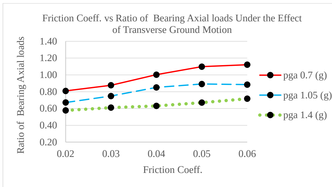
Figure 44. Friction Coefficient and Ratio of Bearing Axial Loads of Uplift-Restricted Case to Uplift-Allowed Case. (Investigated Under the Effect of Transverse Motion Considering Three Different PGA values)
