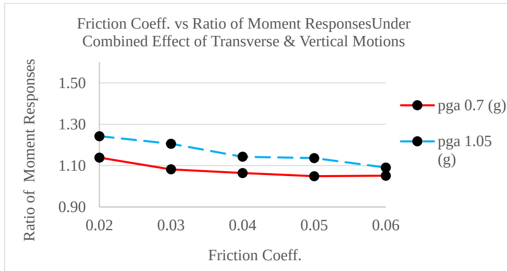
Figure 47. Friction Coefficient and Ratio of Moment Responses of Uplift-Restricted Case to Uplift-Allowed Case. (Investigated Under the Combined Effect of Transverse and Vertical Motions Considering Two Different PGA values)
