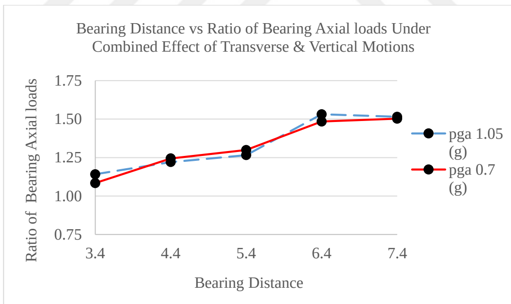
Figure 29. Bearing Distances and Ratio of Bearing Axial Load of Uplift-Restricted Case to Uplift-Allowed Case (Investigated Under the Combined Effect of Transverse and Vertical Motions Considering Two Different PGA values)
