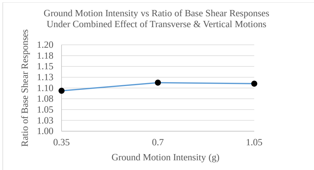
Figure 60. Ground Motion Intensity and Ratio of Base Shear Responses of Uplift-Restricted case to Uplift-Allowed case (Investigated Under the Combined Effect of Transverse and Vertical Motions)
