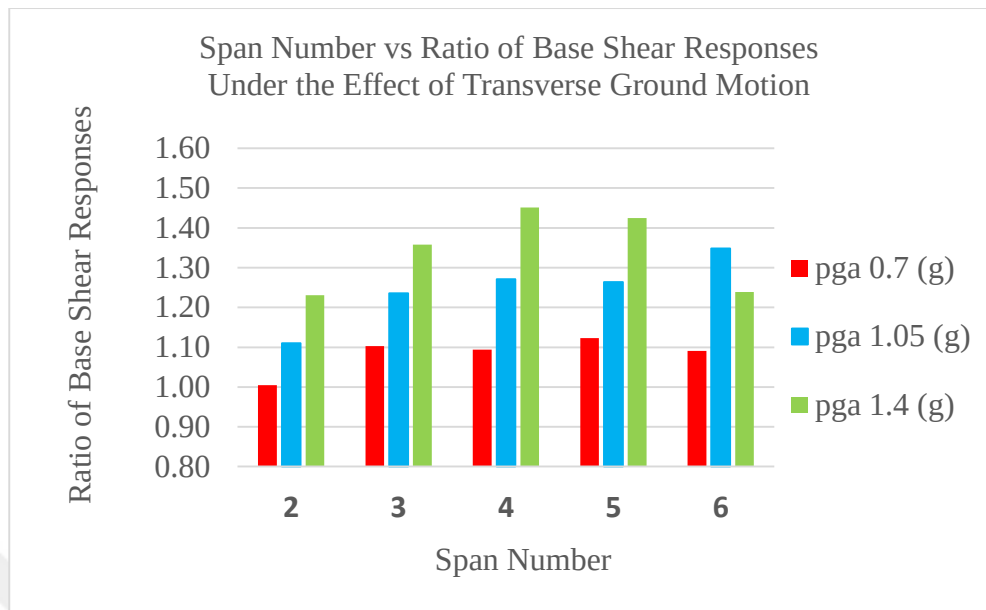
Figure 19. Span Number and Ratio of Base Shear Responses of Uplift-Restricted Case to Uplift-Allowed Case (Investigated Under the Effect of Transverse Motion Considering Three different PGA values)
