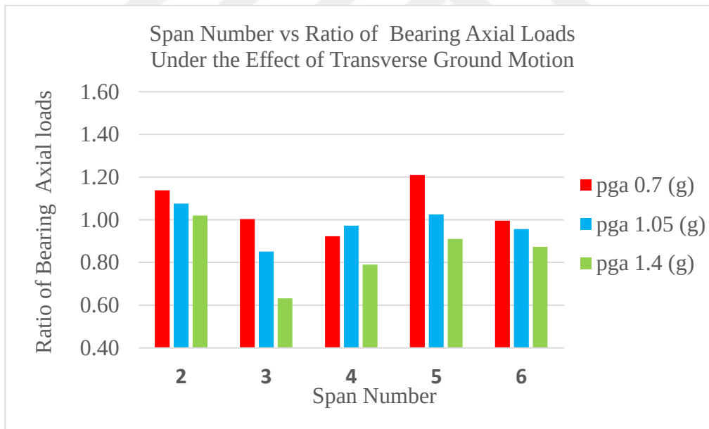
Figure 20. Span Number and Ratio of Bearing Axial Loads of Uplift-Restricted Case to Uplift-Allowed Case (Investigated Under the Effect of Transverse Motion Considering Three different PGA values)
