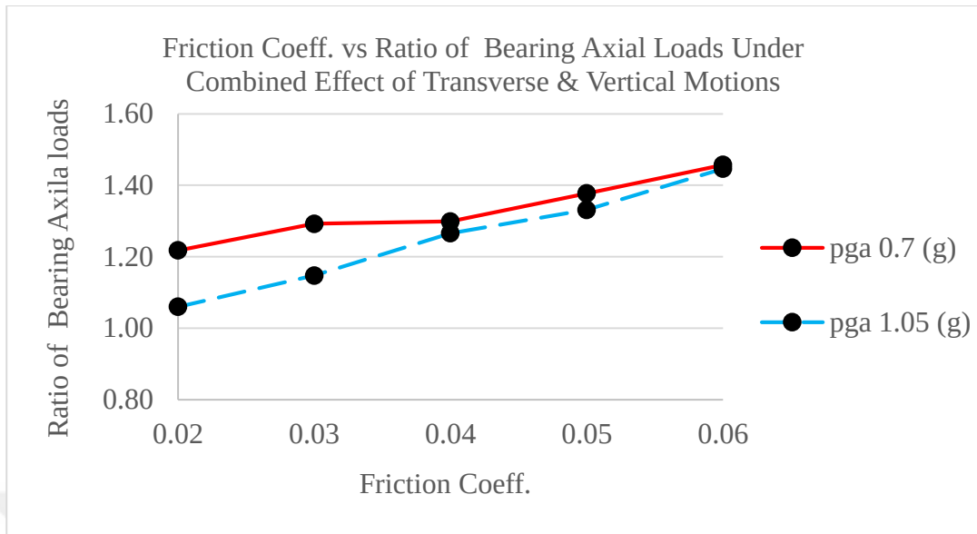
Figure 49. Friction Coefficient and Ratio of Bearing Axial Loads of Uplift-Restricted Case to Uplift-Allowed Case. (Investigated Under the Combined Effect of Transverse and Vertical Motions Considering Two Different PGA values)
