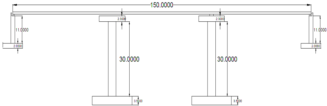
Figure .1 Elevation view of Benchmark Bridge Considered for the Purpose of Study
