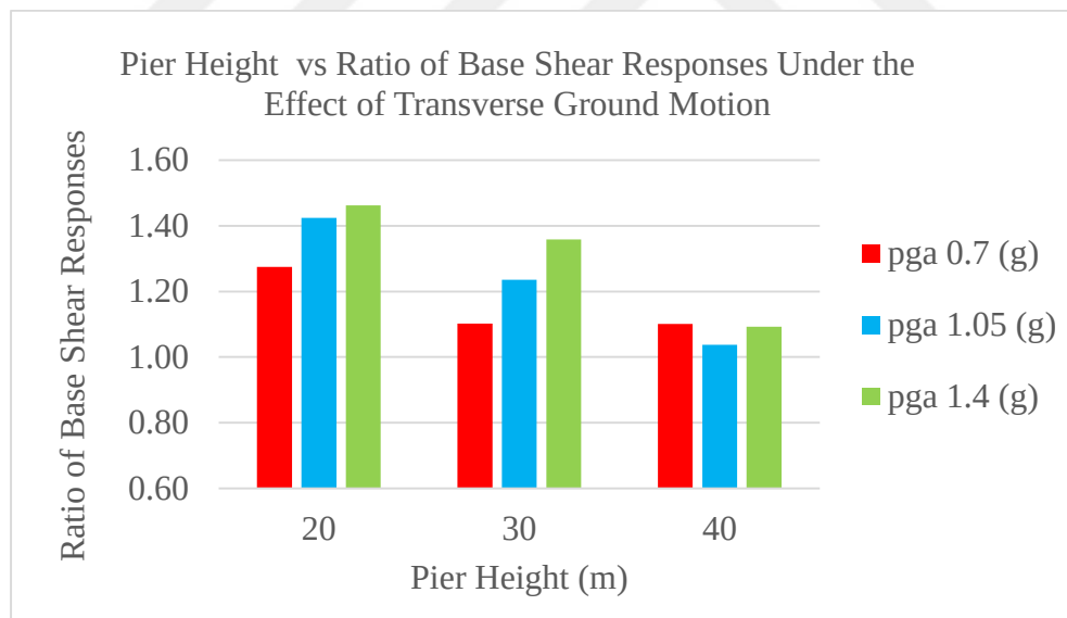
Figure 37. Pier Height and Ratio of Base Shear Responses of Uplift-Restricted Case to Uplift-Allowed Case (Investigated Under the Effect of Transverse Motion Considering Three Different PGA values)
