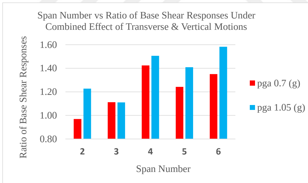
Figure 22. Span Number and Ratio of Base Shear Responses of Uplift-Restricted Case to Uplift-Allowed Case (Investigated Under the Combined Effect of Transverse and Vertical Motions Considering Two different PGA values)
