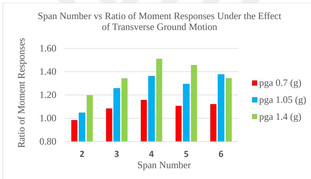
Figure 18. Span Number and Ratio of Moment Responses of Uplift-Restricted Case to Uplift-Allowed Case (Investigated Under the Effect of Transverse Motion Considering Three different PGA values)
