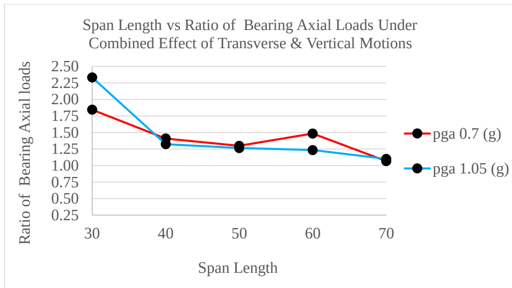
Figure 35. Span Length and Ratio of Bearing Axial Loads of Uplift-Restricted Case to Uplift-Allowed Case (Investigated Under the Combined Effect of Transverse and Vertical Motions Considering Two Different PGA values)
