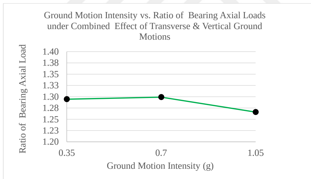
Figure 61. Ground Motion Intensity and Ratio of Bearing Axial Loads of Uplift-Restricted case to Uplift-Allowed case (Investigated Under the Combined Effect of Transverse and Vertical Motions)
