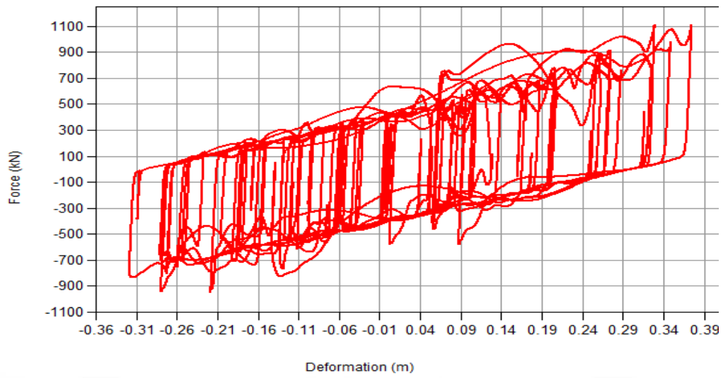
Figure 45. Force-Deformation Graph of FPS Isolator Having Friction Coefficient Equal to 0.06 Obtained Under RSN5778 Transverse Ground Motion with 1.05 (g) PGA
