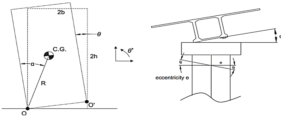
Figure. 4 Free body Diagram of Rocking Body Together with Cross Section of the Rocking Superstructure or Bridge Deck
