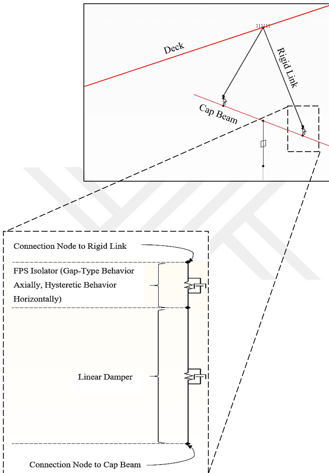
Figure 12. Connection Interphase of Linear Damper with FPS Isolator at MIDAS CIVIL
