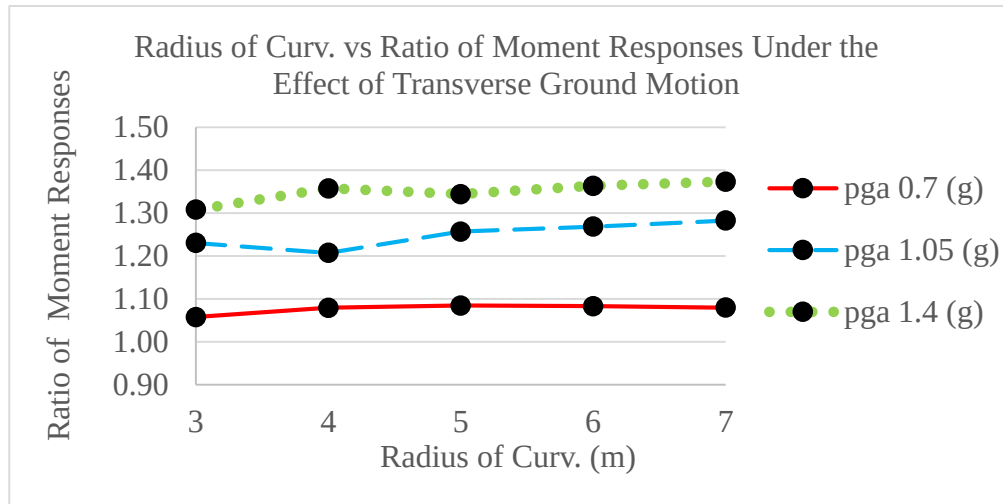
Figure 50. Radius of Curvature and Ratio of Moment Responses of Uplift-Restricted Bridge Model to Uplift-Allowed Case. (Investigated Under the Effect of Transverse Motion Considering Three Different PGA values)
