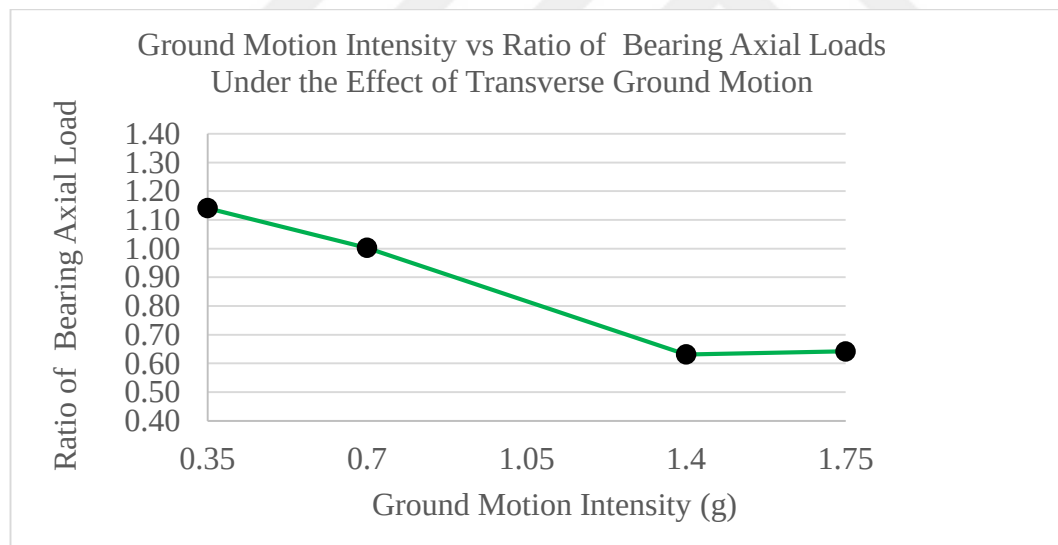
Figure 58. Ground Motion Intensity and Ratio of Bearing Axial Loads of Uplift-Restricted Case to Uplift-Allowed Case (Investigated Under the Effect of Transverse Motion)
