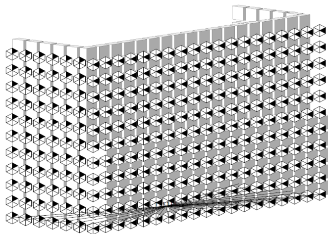
Figure 16. Abutment Model Designed Using Thickness Elements at MIDAS Civil.
