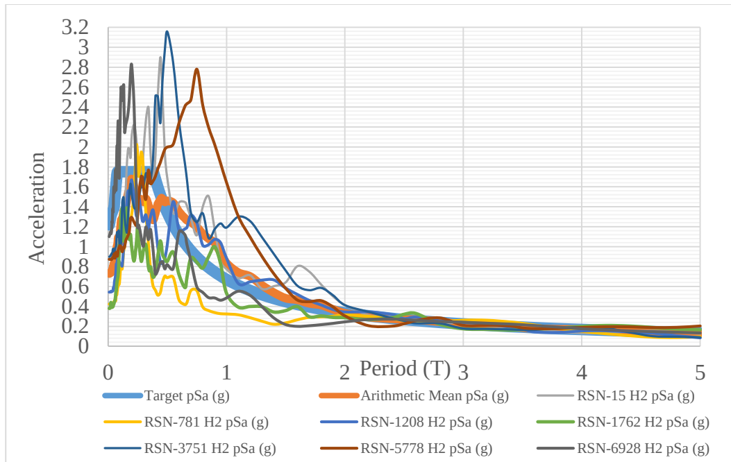
Figure. 17 Target Design Spectrum and Average of Response Spectra of Selected Ground Motions
