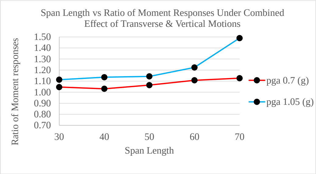
Figure 33. Span Length and Ratio of Moment Responses of Uplift-Restricted Case to Uplift-Allowed Case (Investigated Under the Combined Effect of Transverse and Vertical Motions Considering Two Different PGA values)
