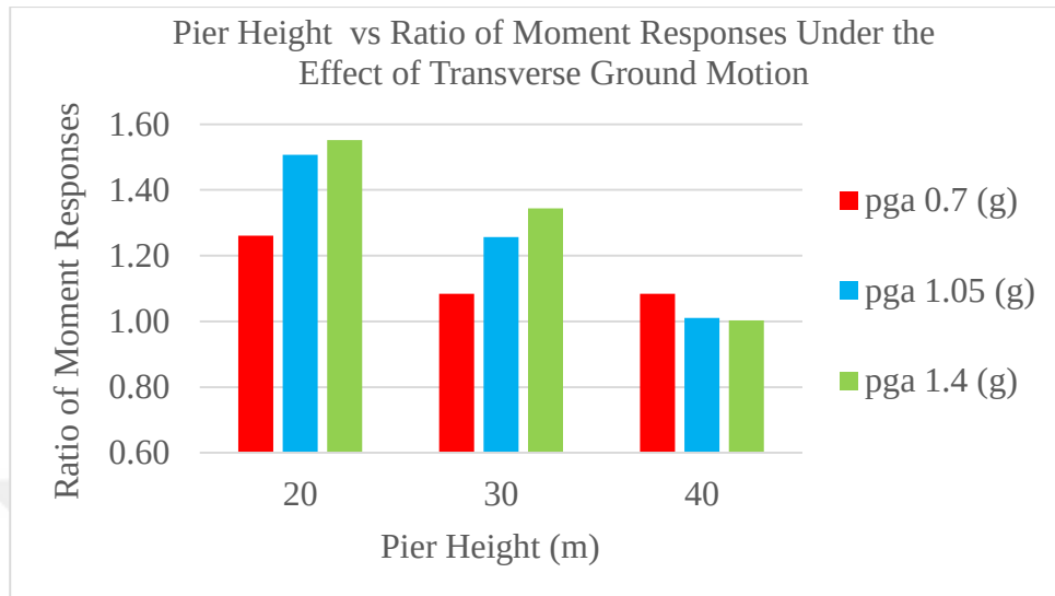
Figure 36. Pier Height and Ratio of Moment Responses of Uplift-Restricted Case to Uplift-Allowed Case (Investigated Under the Effect of Transverse Motion Considering Three Different PGA values)
