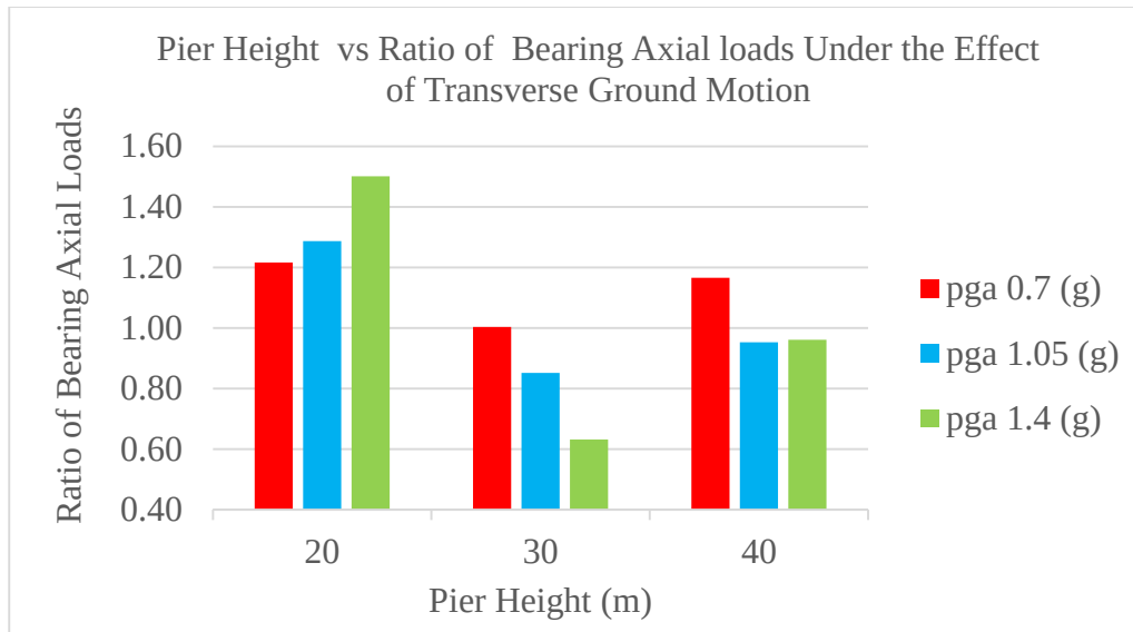
Figure 38. Pier Height and Ratio of Bearing Axial Loads of Uplift-Restricted Case to Uplift-Allowed Case (Investigated Under the Effect of Transverse Motion Considering Three Different PGA values)
