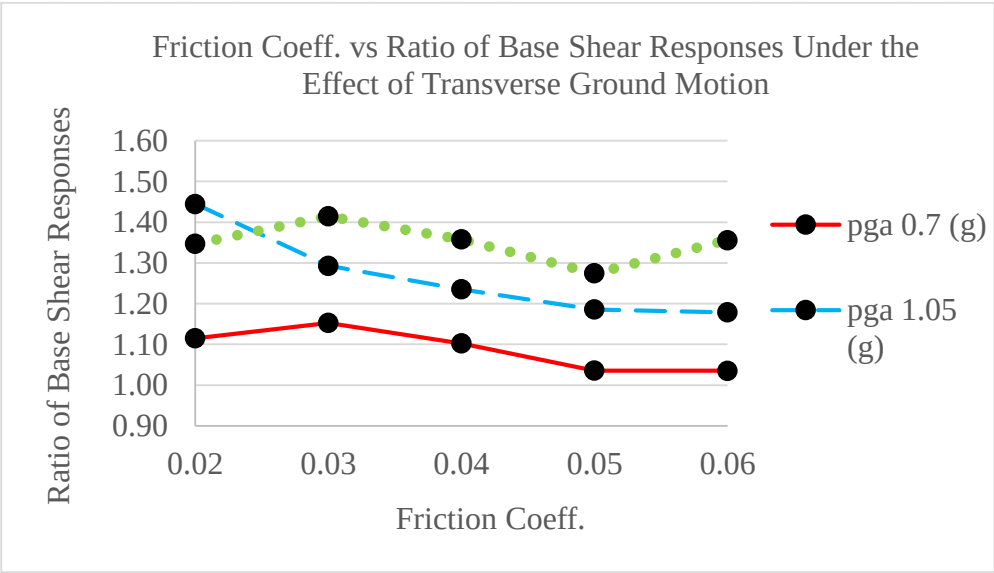
Figure 43. Friction Coefficient and Ratio of Base Shear Responses of Uplift-Restricted Case to Uplift-Allowed Case (Investigated Under the Effect of Transverse Motion Considering Three Different PGA values)
