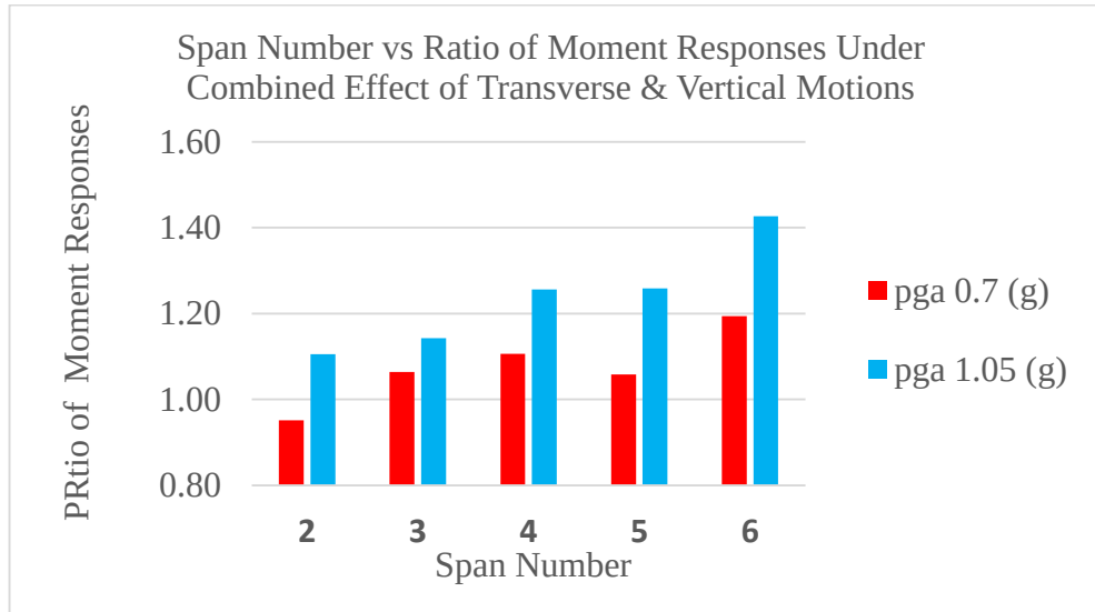
Figure 21. Span Number and Ratio of Moment Responses of Uplift-Restricted Case to Uplift-Allowed Case (Investigated Under the Combined Effect of Transverse and Vertical Motions Considering Two different PGA values)
