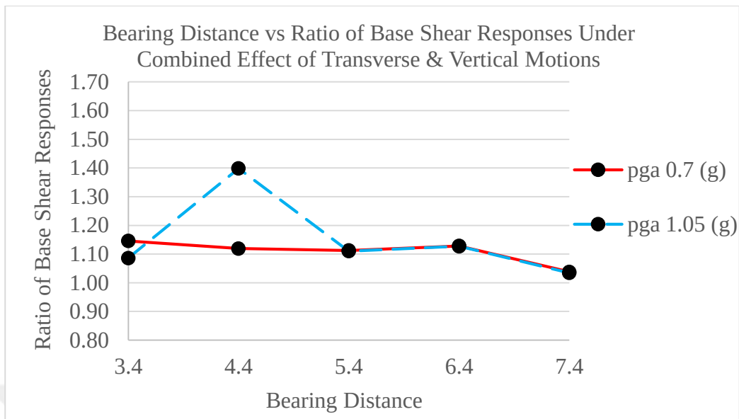
Figure 28. Bearing Distances and Ratio of Base Shear Responses of Uplift-Restricted Case to Uplift-Allowed Case (Investigated Under the Combined Effect of Transverse and Vertical Motions Considering Two Different PGA values)
