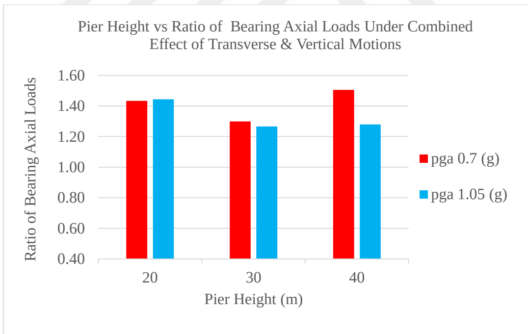
Figure 41. Pier Height and Ratio of Bearing Axial Loads of Uplift-Restricted Case to Uplift-Allowed Case (Investigated Under the Combined Effect of Transverse and Vertical Motions Considering Two Different PGA values)
