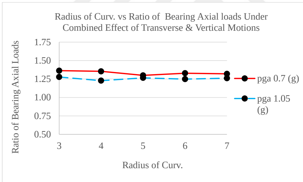
Figure 55. Radius of Curvature and Ratio of Bearing Axial Loads of Uplift-Restricted case to Uplift-Allowed case (Investigated Under the Combined Effect of Transverse and Vertical Motions Considering Two Different PGA values)
