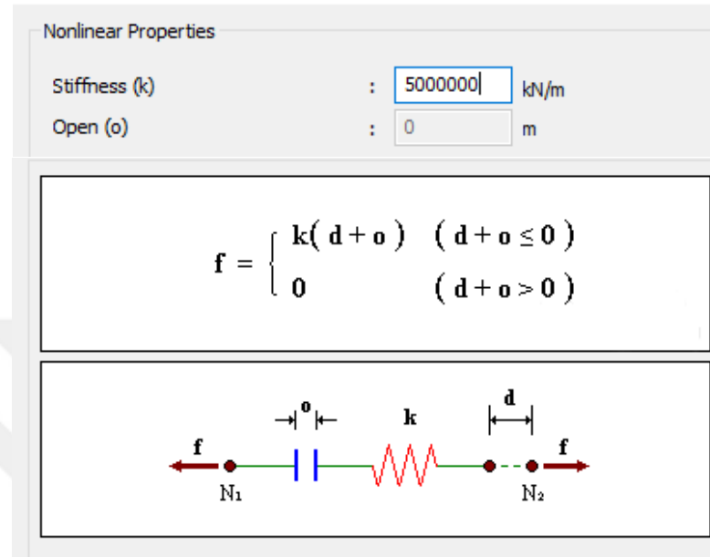
Figure 10. Axial Spring Property of FPS Bearing
