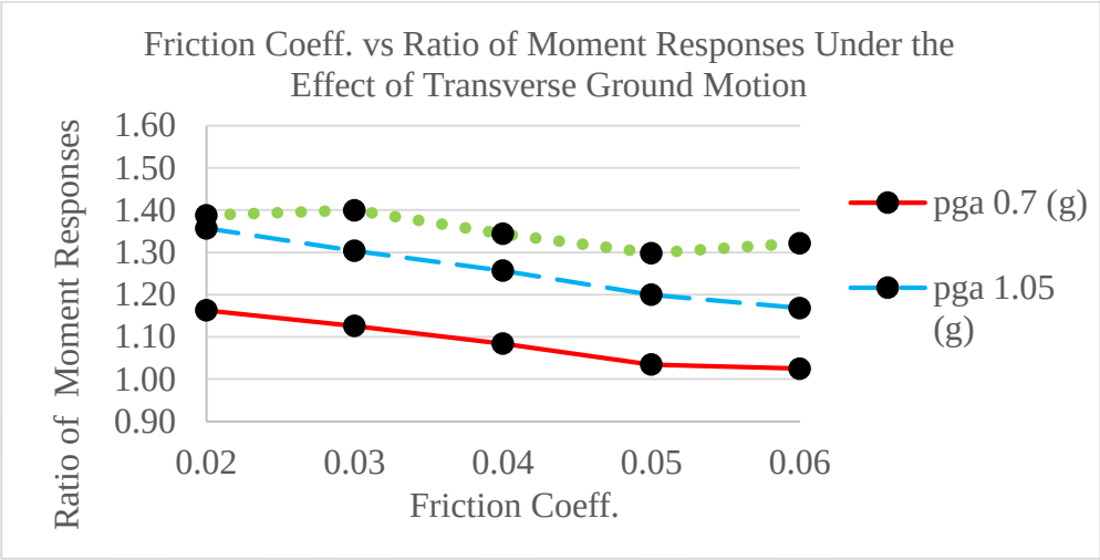
Figure 42. Friction Coefficient and Ratio of Moment Responses of Uplift-Restricted Case to Uplift-Allowed Case. (Investigated Under the Effect of Transverse Motion Considering Three Different PGA values)
