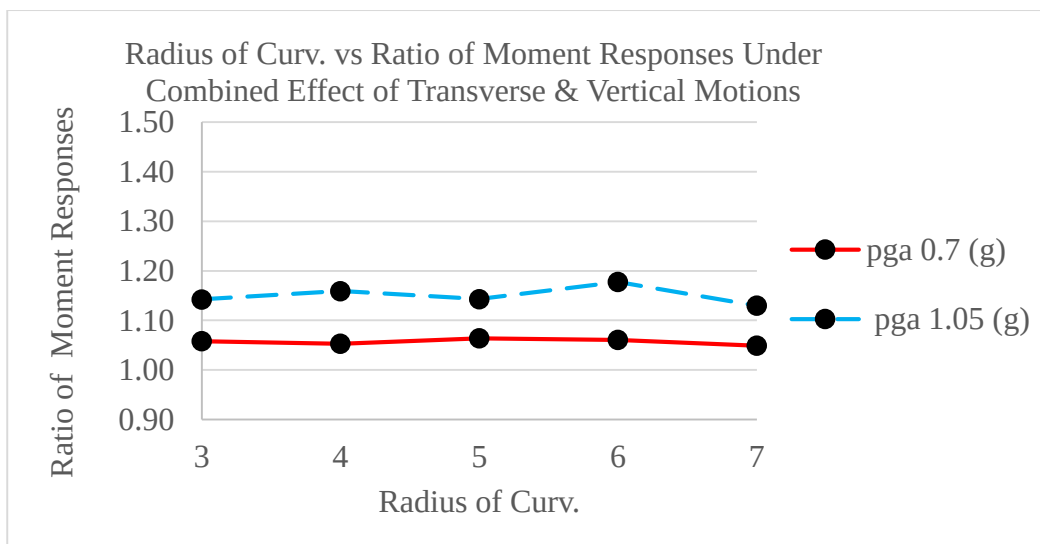
Figure 53. Radius of Curvature and Ratio of Moment Responses of Uplift-Restricted Bridge Model to Uplift-Allowed Case. (Investigated Under the Combined Effect of Transverse and Vertical Motions Considering Two Different PGA values)
