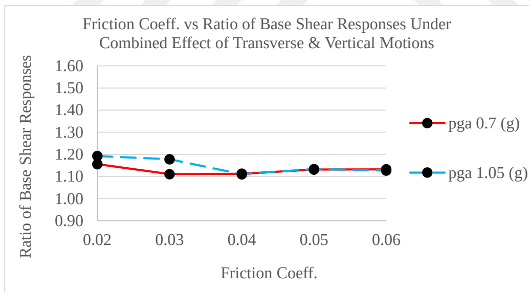
Figure 48. Friction Coefficient and Ratio of Base Shear Responses of Uplift-Restricted Case to Uplift-Allowed Case (Investigated Under the Combined Effect of Transverse and Vertical Motions Considering Two Different PGA values)
