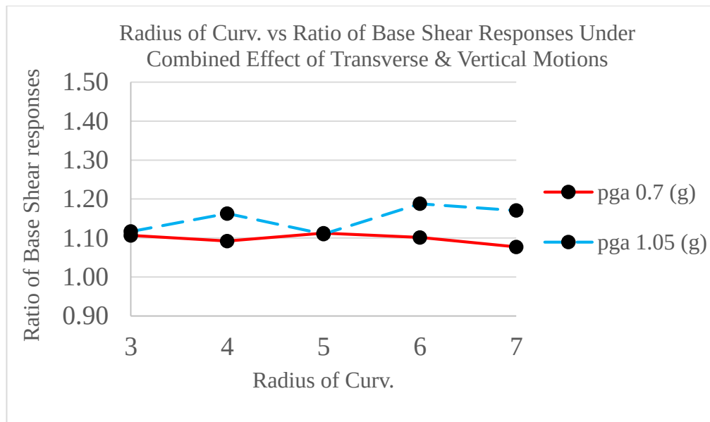
Figure 54. Radius of Curvature and Ratio of Base Shear Responses of Uplift-Restricted case to Uplift-Allowed Case (Investigated Under the Combined Effect of Transverse and Vertical Motions Considering Two Different PGA values)
