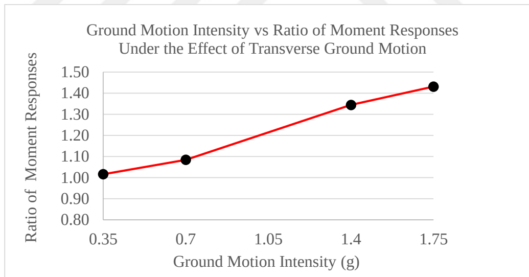
Figure 56. Ground Motion Intensity and Ratio of Moment Responses of Uplift-Restricted Case to Uplift-Allowed Case (Investigated Under the Effect of Transverse Motion)
