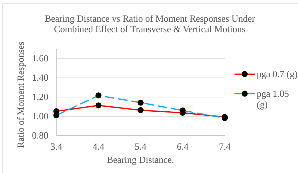
Figure 27. Bearing Distances and Ratio of Moment Responses of Uplift-Restricted Case to Uplift-Allowed Case (Investigated Under the Combined Effect of Transverse and Vertical Motions Considering Two Different PGA values)
