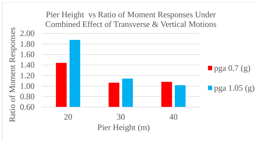
Figure 39. Pier Height and Ratio of Moment Responses of Uplift-Restricted Case to Uplift-Allowed Case (Investigated Under the Combined Effect of Transverse and Vertical Motions Considering Two Different PGA values)
