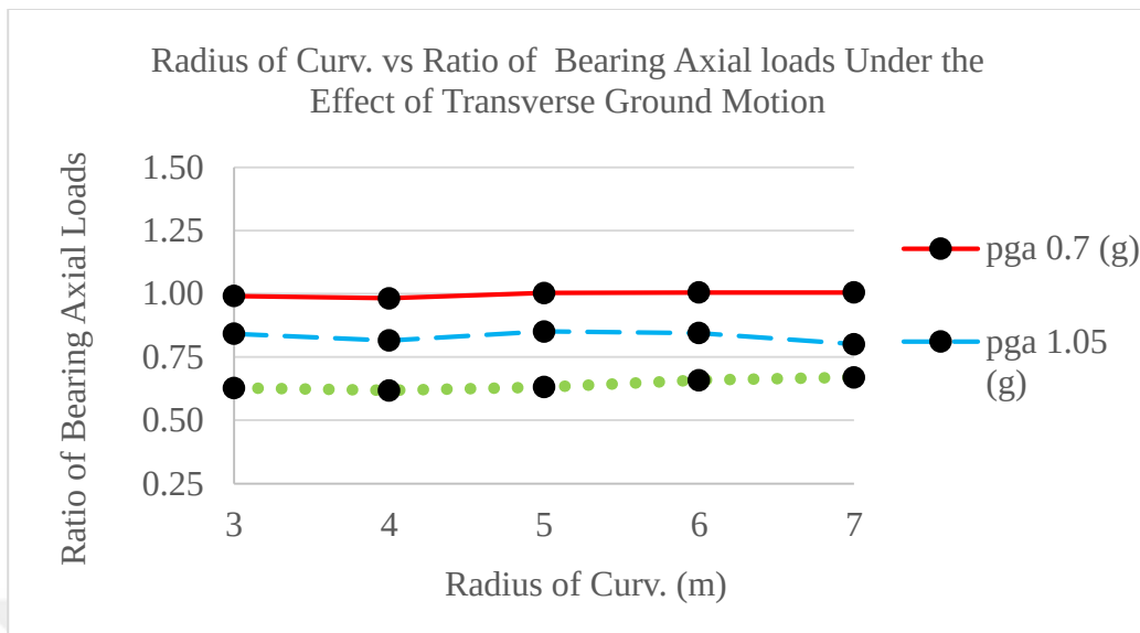
Figure 52. Radius of Curvature and Ratio of Bearing Axial Loads of Uplift-Restricted case to Uplift-Allowed case (Investigated Under the Effect of Transverse Motion Considering Three Different PGA values)
