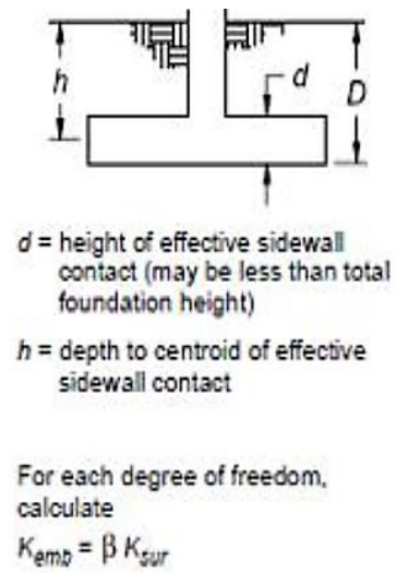
Figure 14. Footing with specified Dimensions at Embedment Depth
