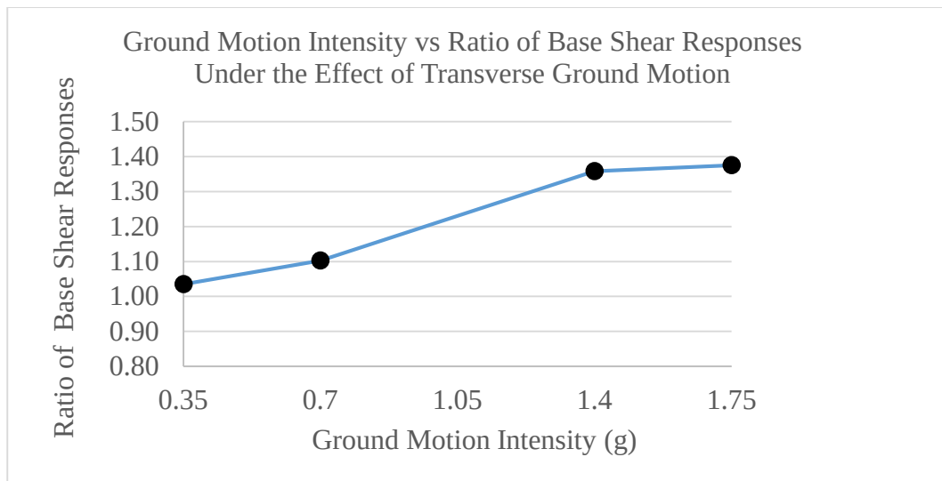
Figure 57. Ground Motion Intensity and Ratio of Base Shear Responses of Uplift-Restricted Case to Uplift-Allowed Case (Investigated Under the Effect of Transverse Motion)
