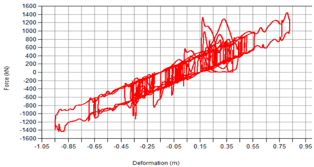
Figure 46. Force-Deformation Graph of FPS Isolator Having Friction Coefficient Equal to 0.02 Obtained Under RSN5778 Transverse Ground Motion with 1.05 (g) PGA
