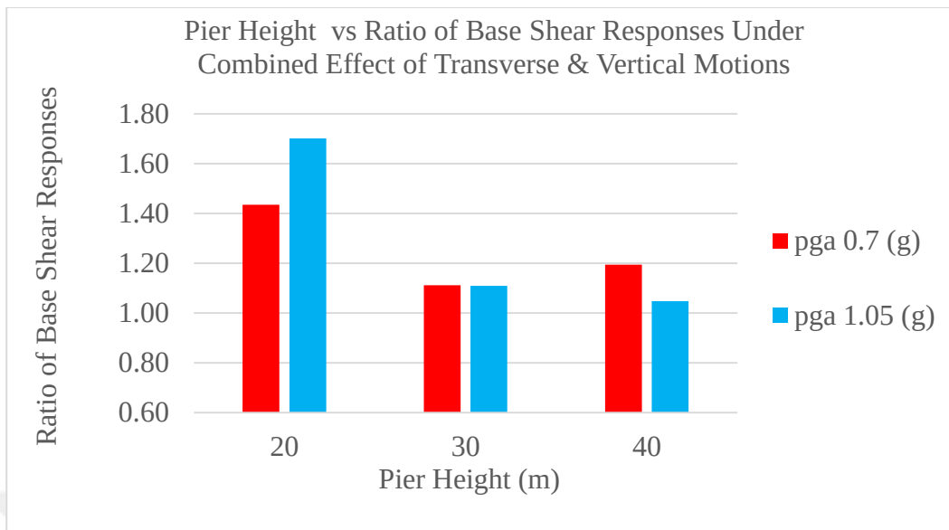
Figure 40. Pier Height and Ratio of Base Shear Responses of Uplift-Restricted Case to Uplift-Allowed Case (Investigated Under the Combined Effect of Transverse and Vertical Motions Considering Two Different PGA values)
