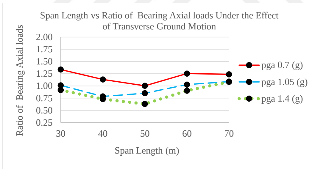
Figure 32. Span Length and Ratio of Bearing Axial Loads of Uplift-Restricted Case to Uplift-Allowed Case (Investigated Under the Effect of Transverse Motion Considering Three Different PGA values)
