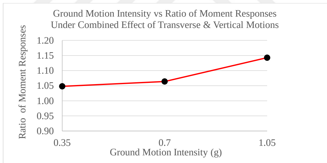
Figure 59. Ground Motion Intensity and Ratio of Moment Responses of Uplift-Restricted case to Uplift-Allowed Case (Investigated Under the Combined Effect of Transverse and Vertical Motions)
