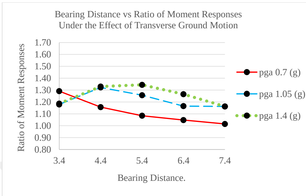
Figure 24. Bearing Distances and Ratio of Moment Responses of Uplift-Restricted Case to Uplift-Allowed Case. (Investigated Under the Effect of Transverse Motion Considering Three Different PGA values)
