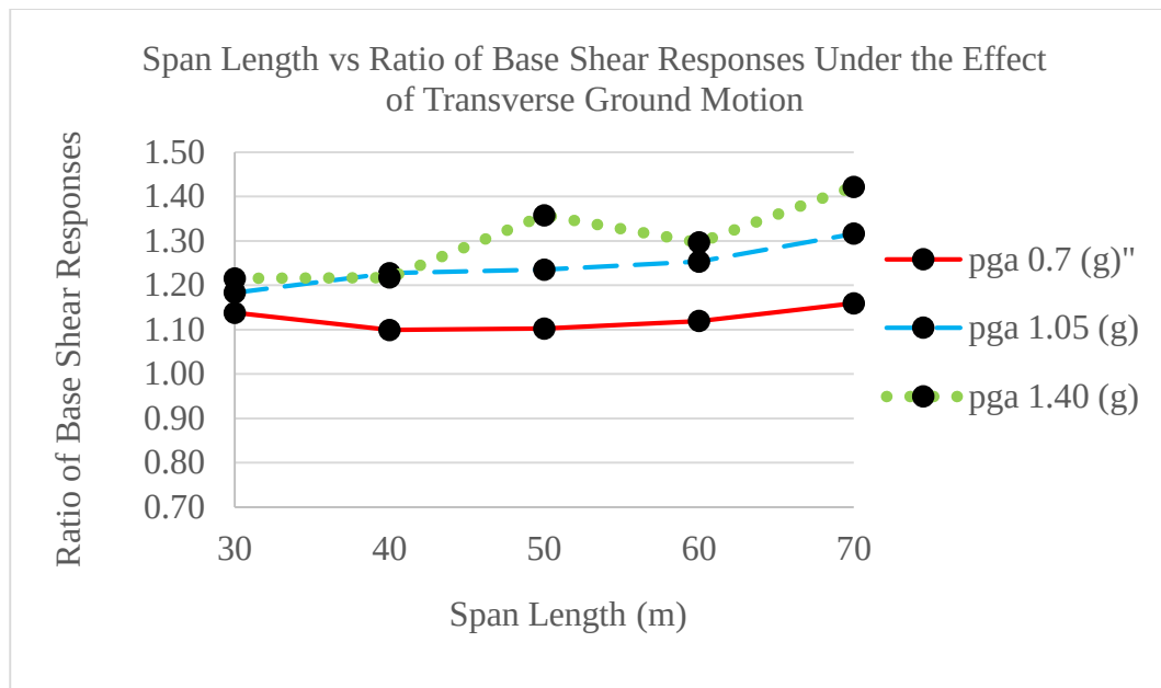
Figure 31. Span Length and Ratio of Base Shear Responses of Uplift-Restricted Case to Uplift-Allowed Case (Investigated Under the Effect of Transverse Motion Considering Three Different PGA values)
