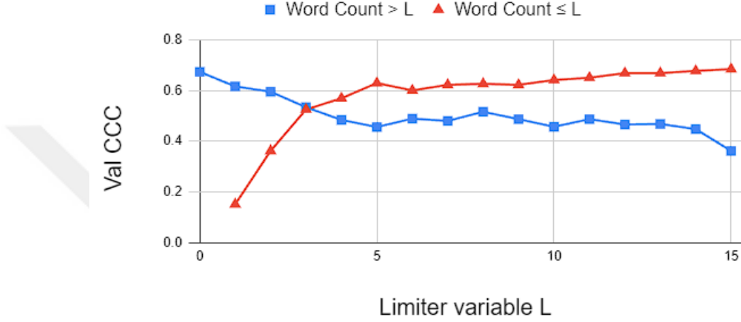
Figure 3.9: Additive (Red-Triangle) and Subtractive (Blue-Square) experiments on word count, using NT-MEAN model. For Limiter variable L , Additive experiment evaluates NT-MEAN on all sentences with word count \leq L . Subtractive experiments do the same for word count > L .
