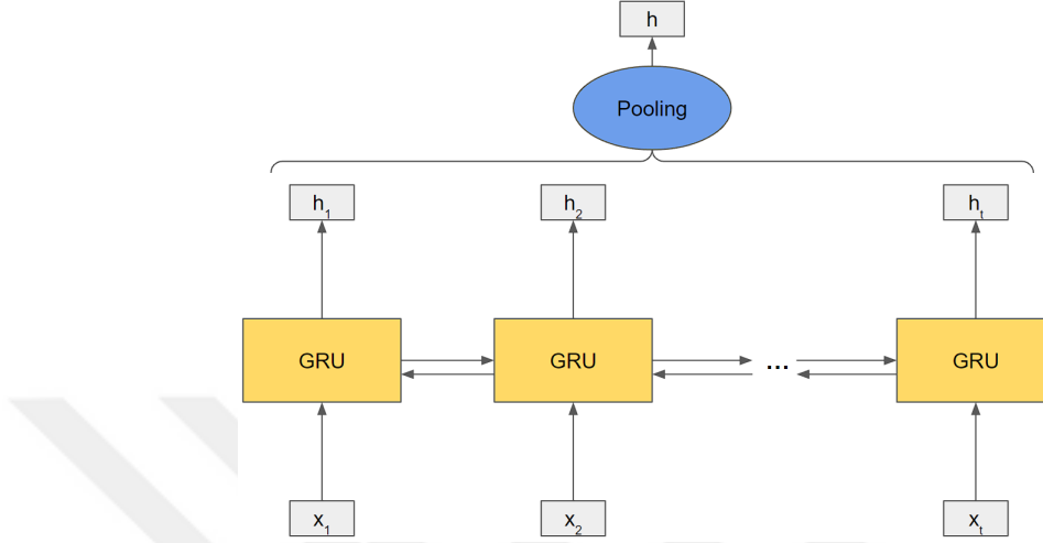
Figure 2.4: Unrolled architecture for the single-level GRU. Each GRU box depicts the same network at different timesteps. Output for each time step is stored and pooled into a single representation.
