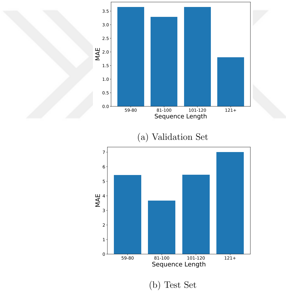
Figure 3.7: Visualization of MAE per sequence length for TS-MEAN model. The value of each bin is the average MAE for participants with that sequence length in (a) validation and (b) test sets.
