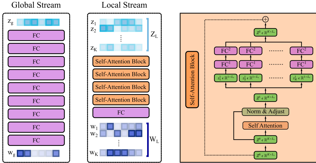
Supp. Fig. A.1: Mapper is a multi-layered architecture comprising two separate processing streams: a global stream dedicated to the global latent variable w_g , and a local stream dedicated to the local latent variables W_l = \{w_1, w_2, \dots, w_K\} . The global stream contains a cascade of fully-connected sub-blocks. Meanwhile, the local stream is a cascade of self-attention sub-blocks followed by a fully-connected sub-block (see rightmost panel for the architecture of the self-attention sub-block). Self-attention sub-blocks enable interactions among individual local latents.
