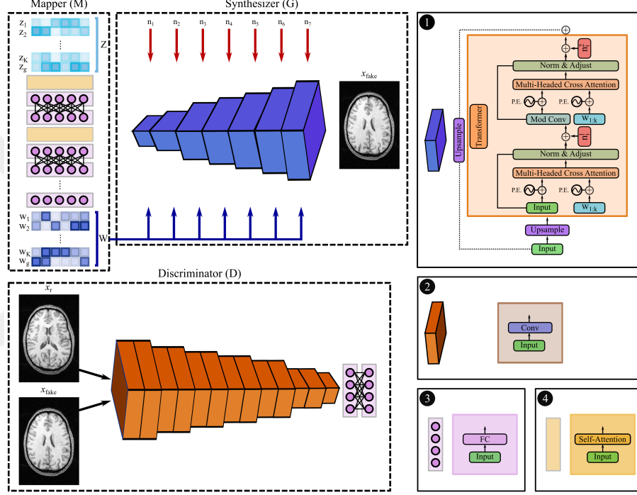
Figure 4.2: SLATER is based on an unconditional adversarial architecture with a synthesizer (G), a discriminator (D), and a mapper (M). G is a multi-layer architecture where image resolution is progressively increased across layers. Within intermediate layers, a convolutional upsampling block is followed by a cross-attention transformer block (see 1). The transformer block receives global and local latent variables, noise variables and positional encoding (P.E.) for latents and image features. D enables adversarial learning while it receives as input synthetic and actual MR images. It is composed of convolutional and fully-connected (FC) blocks (see 2, 3). M projects raw latent variables ( Z ) onto k local ( w_1, \dots, w_K ) variables and one global ( w_g ) latent variable. It is composed of self-attention and FC blocks (see 3, 4, and Supp. Fig. A.1 for details). An unsupervised generative modeling task is performed using the SLATER model to capture high-quality MRI priors.
