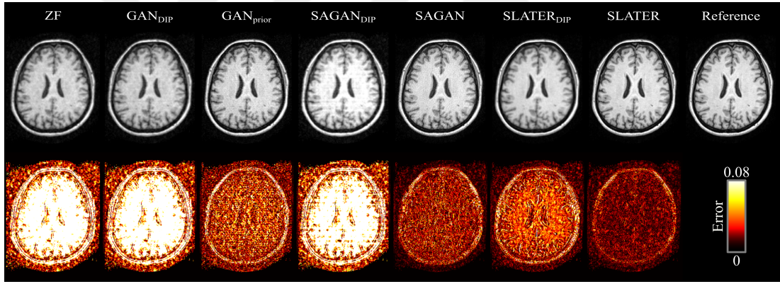
Supp. Fig. A.5: Reconstructions of a representative T_1 -weighted acquisition at R=4 are shown for the Fourier method (ZF), DIP methods (GAN DIP , SAGAN DIP , SLATER DIP ) and zero-shot reconstructions (GAN prior , SAGAN, SLATER) along with the reference image. Corresponding error maps are underneath the images for each method.
