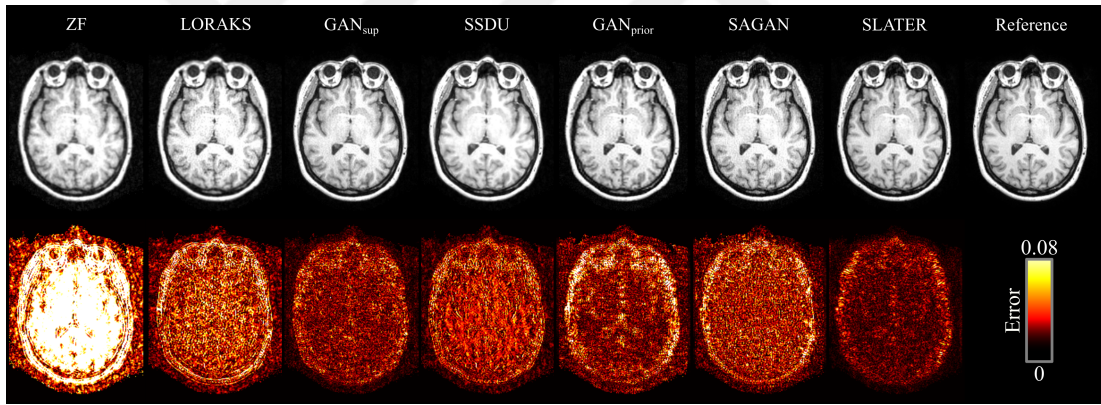
Supp. Fig. A.10: Across-domain reconstructions of a T 1 -weighted acquisition in the IXI dataset at R=4. Results are shown for ZF, LORAKS, GAN sup , SSDU, GAN prior , SAGAN and SLATER along with the reference image. Corresponding error maps are underneath the images for each method.
