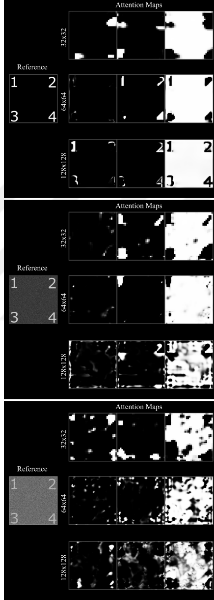
Supp. Fig. A.4: Cross-attention maps in SLATER for a simulated digit phantom with varying levels of noise. Relative to a peak signal intensity of 1, top, middle and bottom panels display sample attention maps for no noise, noise variance of 0.01, and noise variance of 0.1, respectively. Within each panel, maps from the first cross-attention sub-block are shown at three resolutions (i.e., 32x32, 64x64, 128x128 at network layers 4-6), along with the reference phantom images.
