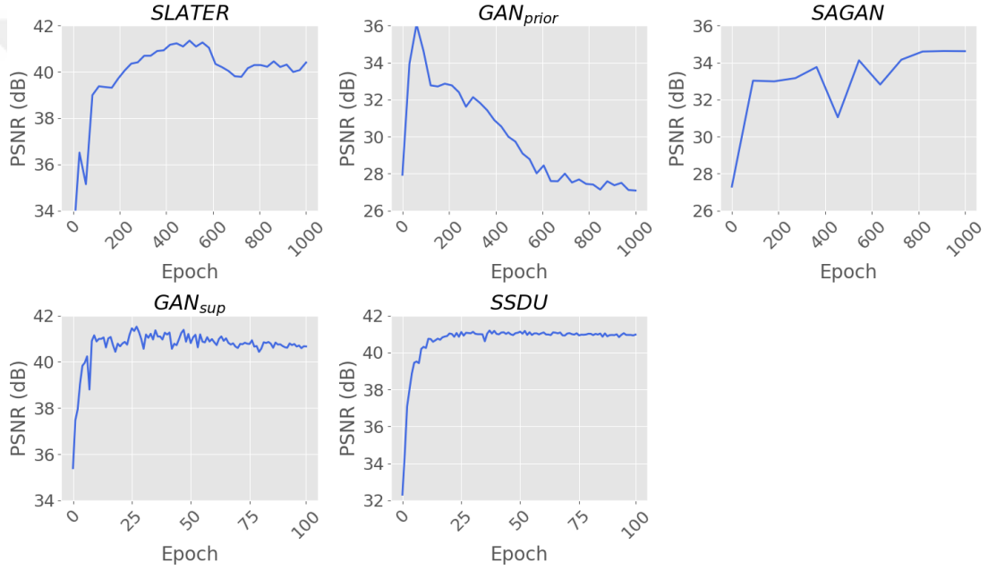
Supp. Fig. A.3: Reconstruction performance in the validation set as a function of number of training epochs. Results from supervised ( \text{GAN}_{\text{sup}} ) and unsupervised models (SSDU, \text{GAN}_{\text{prior}} , SAGAN and SLATER) are shown for T_1 -weighted acquisitions in IXI at R=4 . For unsupervised models, hyperparameter selection in the validation set was actually performed based on the difference between recovered and acquired k-space samples in undersampled data. However, to facilitate interpretation, here performance for all methods is displayed as PSNR between reconstructed and ground-truth images.
