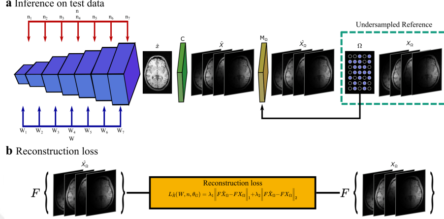
Figure 4.1: (a) The generative model in SLATER is adapted to perform zero-shot reconstruction for accelerated MRI. To do this, the generator output is back-projected onto individual coils (C), and masked with the same sampling pattern as in the undersampled acquisition ( M_\Omega ). (b) The network prior consisting of noise (n), latent variables (W) and weights ( \theta_G ) is then optimized to maximize consistency between the reconstructed and acquired k-space data.
