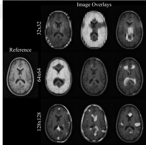
Figure 3.1: Cross-attention maps in SLATER for a T_1 -weighted acquisition. Sample maps from the first CA sub-block are displayed by overlay onto the respective MR image across three resolutions (i.e., at network layers 4-6). Attention maps for separate latents typically show segregated spatial distribution, and tend to group tissue clusters with similar signal intensity and texture broadly distributed across the image.
