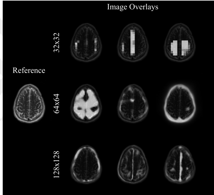
Supp. Fig. A.2: Cross-attention maps in SLATER for a T_2 -weighted acquisition. Sample attention maps from the first cross-attention transformer block are displayed across three resolutions (i.e., 32 \times 32 , 64 \times 64 , 128 \times 128 at network layers 4-6). At each resolution, respective maps are displayed in overlaid format onto the MR image, and the reference MR image is also shown. Attention maps for separate latents show segregated spatial distribution. They also tend to group tissue clusters with similar signal intensity and texture, where the clusters are broadly distributed across the image and they are often spatially noncontiguous.
