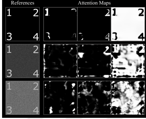
Figure 3.2: Cross-attention maps in SLATER for a simulated phantom with varying levels of normally-distributed white noise. Sample maps from the first CA sub-block are displayed at 128x128 resolution (network layer 6). Relative to a peak signal intensity of 1, top, middle and bottom rows show results for no noise, noise variance of 0.01, and noise variance of 0.1, respectively.
