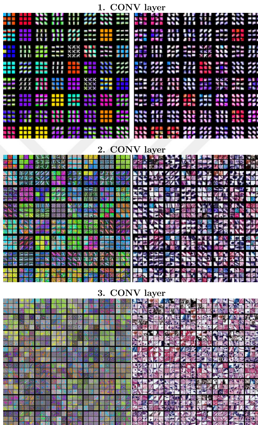
Figure 5.16: Visualization of the first three convolutional layers of the trained CNN model by the deconvolution method. For each layer, the top-9 activations of 64 neurons (left) and their corresponding original image patches (right) are shown as 3 \times 3 groups. Color in left squares does not represent natural spectrum, but the activation projection and the color contrast artificially enhanced for better view. Best viewed in color and with zoom.
