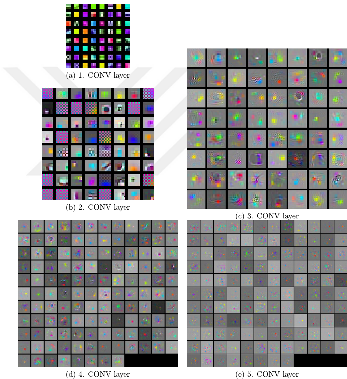
Figure 5.19: The synthesized images that activate neurons the most. Best viewed in color and with zoom.
