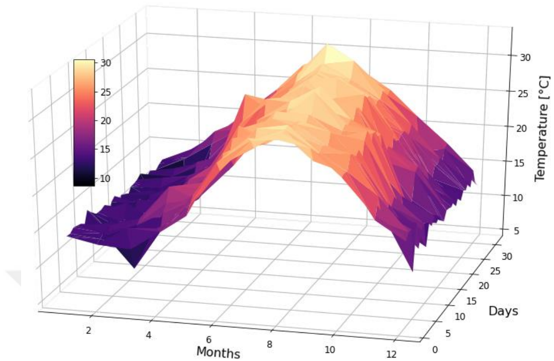
Figure 3.5. Temporal distribution of temperature over NASA dataset
