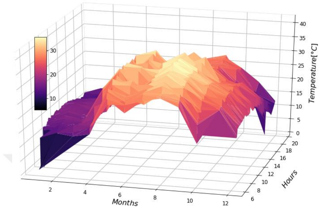
Figure 3.10. Temporal distribution of temperature over METU NCC dataset
