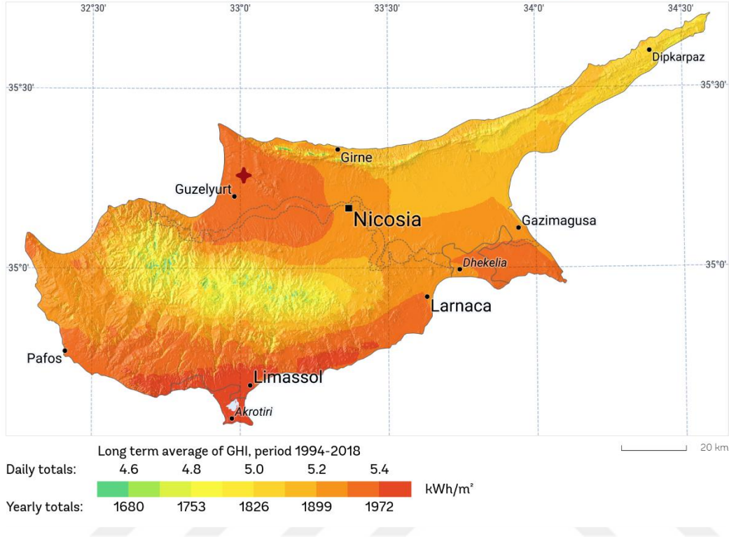
Figure 3.1. The spatial distribution of GHI over Cyprus island [33]
