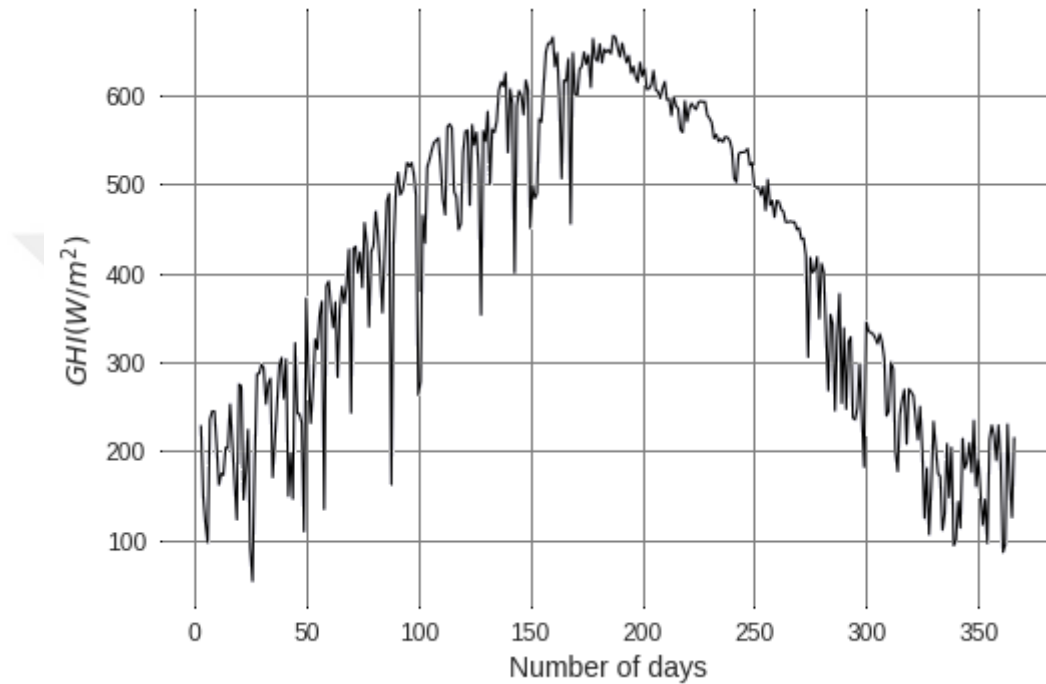
Figure 3.3. Change in GHI values over the year 2018
