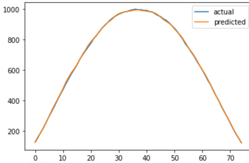
Figure 4.6. CM-SVR model prediction fitted over the actual data for the summer season for a clear-sky condition
