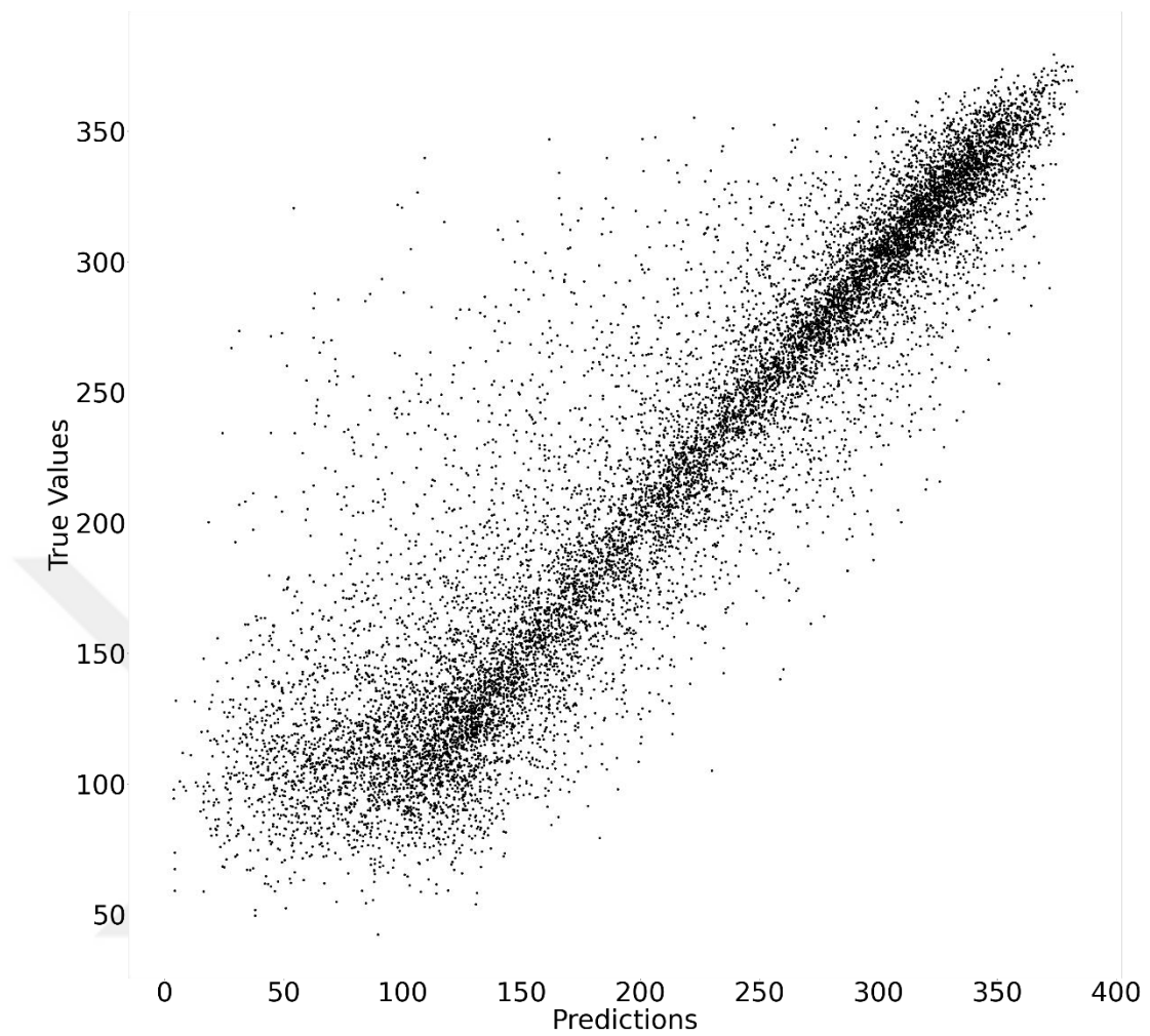
Figure A.9. Predicted and actual GHI values on a scattered plot for endogenous CNN over the testing set
