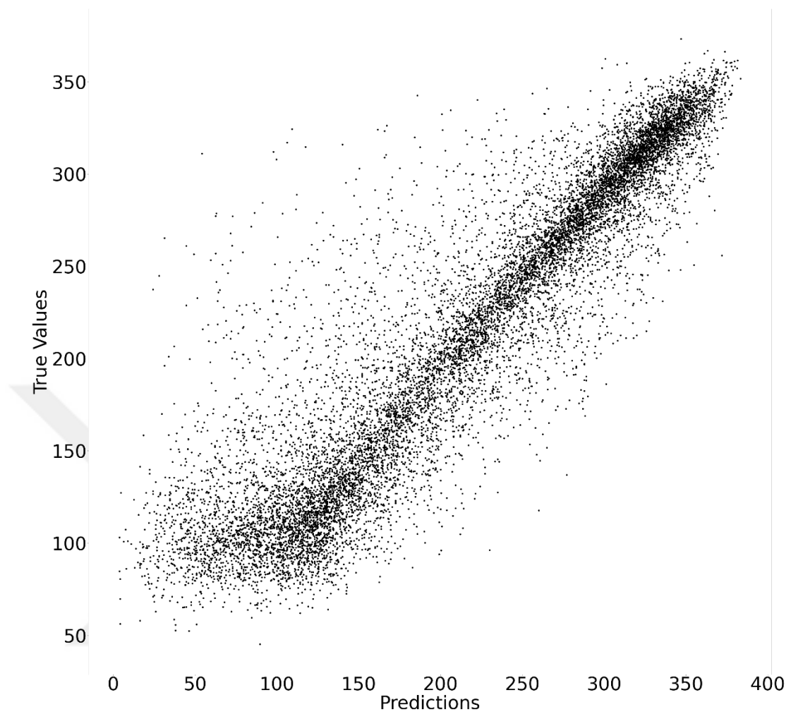
Figure A.7. Predicted and actual GHI values on a scattered plot for endogenous LSTM over the testing set
