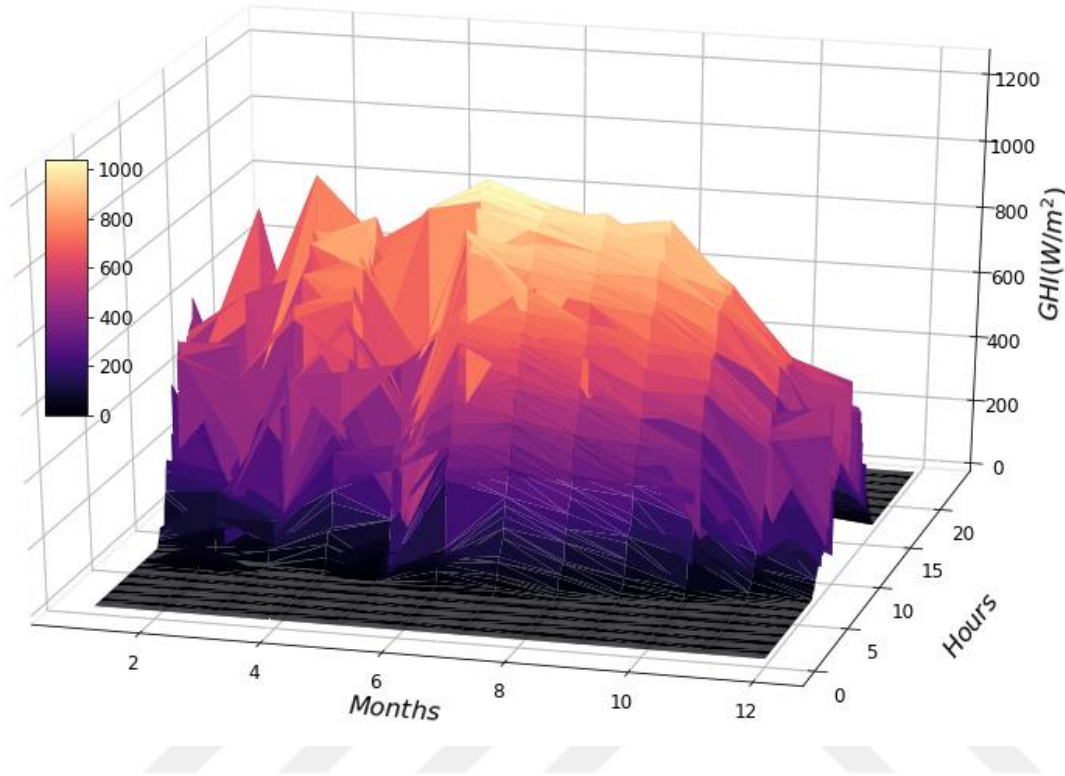
Figure 3.7. Temporal distribution of GHI throughout the METU NCC dataset
