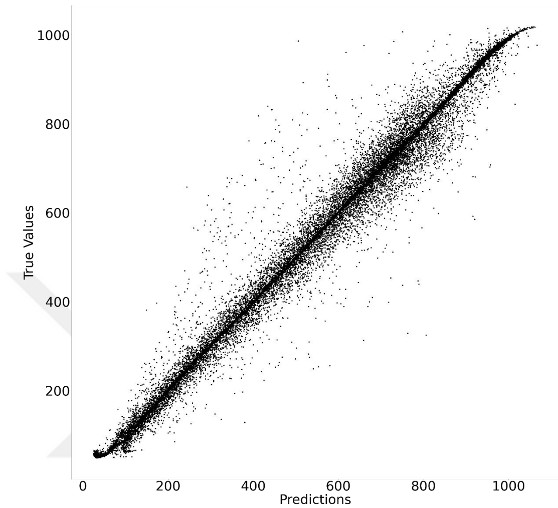
Figure B.7. Predicted and actual GHI values on a scattered plot for the summer season over the testing set
