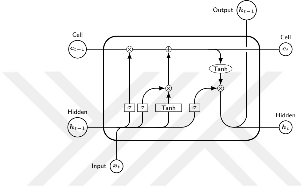
Figure 2.1: Memory cell for Long-Short term memory neural networks.
