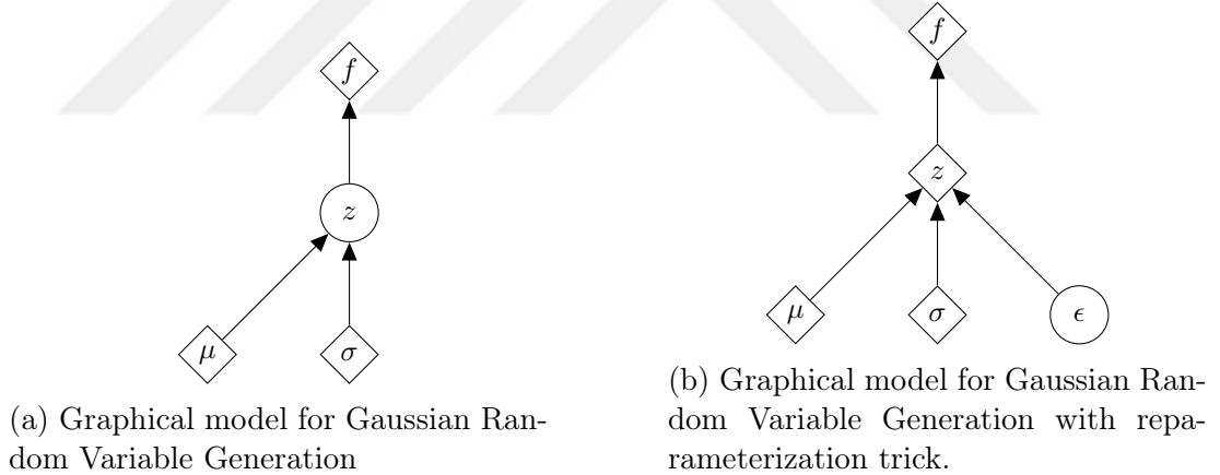
Figure 2.5: Reparameterization Trick for Deep Latent Variable Models.
