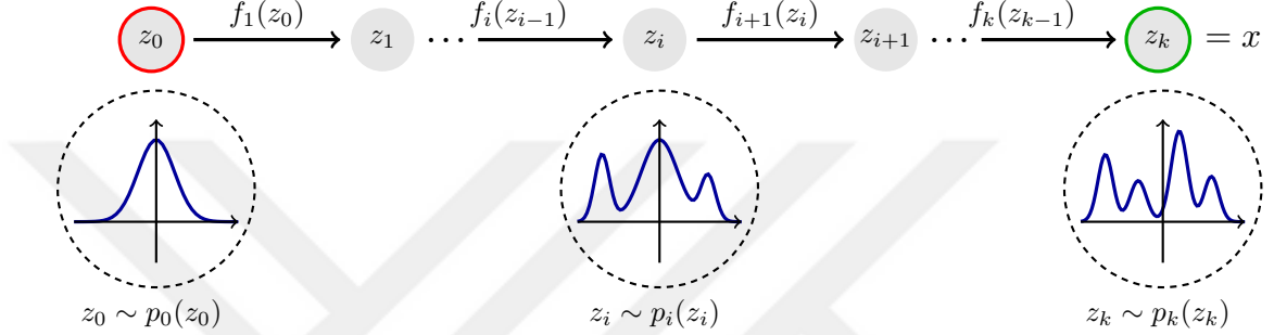
Figure 2.6: Normalizing flows transforms a simple density such as Gaussian, to a complicated multi-modal density via a series of invertible transformations.
