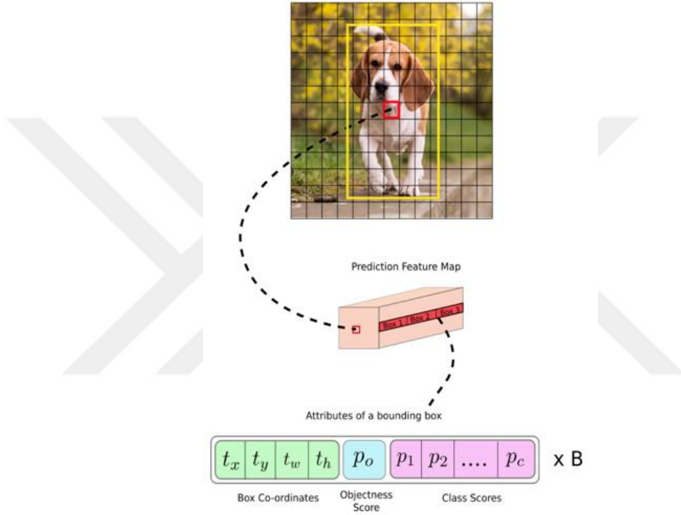
Figure 4.2. Attributes of the bounding boxes of YOLOv3.
