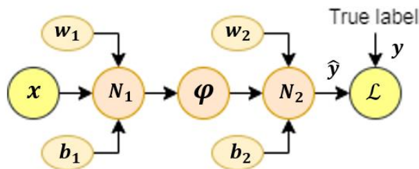
Figure 2.7. Simple two-layer NN with input x , activation \phi , loss \mathcal{L} functions.
