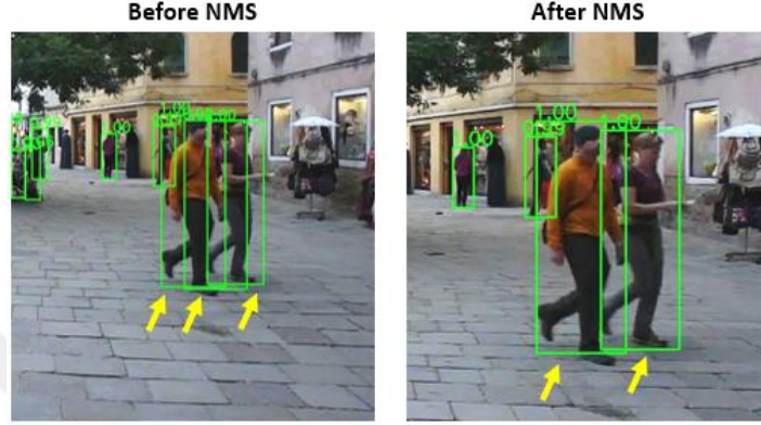
Figure 6.2. On the left: the middle detection combines both pedestrians. On the right: NMS filtering the overlapped detection.
