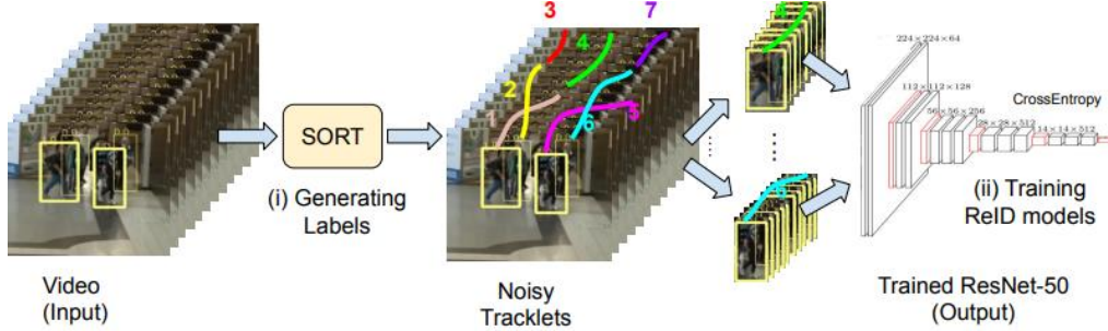
Figure 5.6. The tracker's pipeline proposed by [83].
