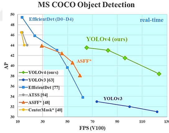
Figure 7.2. Comparison of Yolo-v4 to other popular detection models [118].
