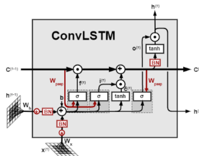
Figure 7.11. ConvLSTM2D layer architecture.
