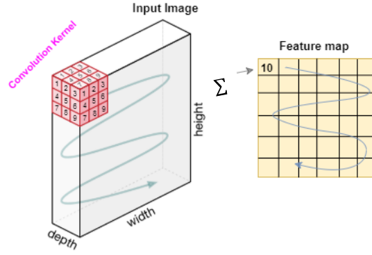
Figure 2.8. Movements path of the convolution kernel operating on the input image to output feature map [32].
