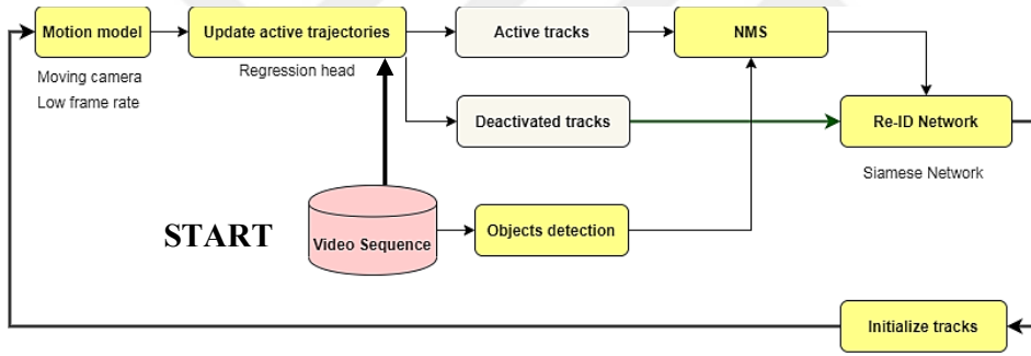
Figure 6.3. Summary of Tractor tracking pipeline [74].
