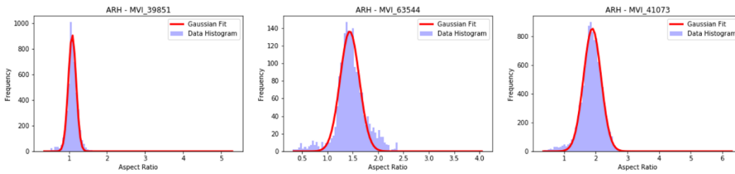
Figure 7.8. Sample AR plots for three UA-DETRAC [46] videos.
