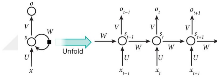
Figure 2.11. Sample RNN architecture on the left and the unfolded time representation. i.e., write the network for the full sequence [35].
