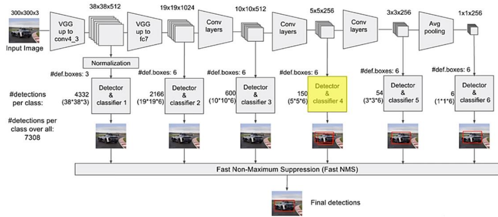
Figure 4.3. SSD network architecture [67].
