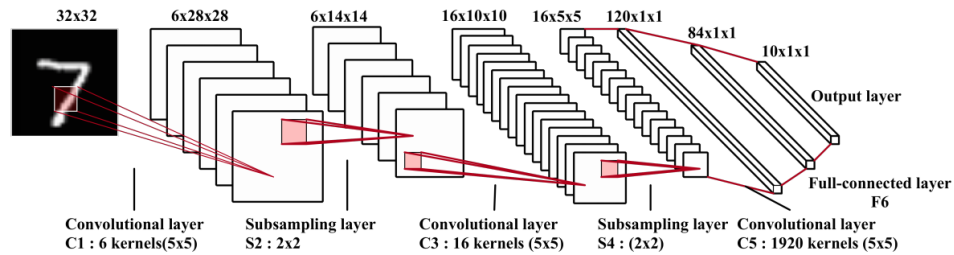
Figure 2.10. LeNet-5 network [32].
