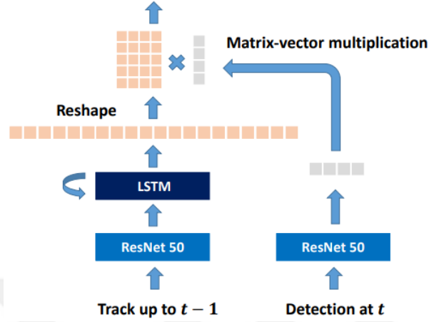
Figure 5.1. Proposed bLSTM topology [96].
