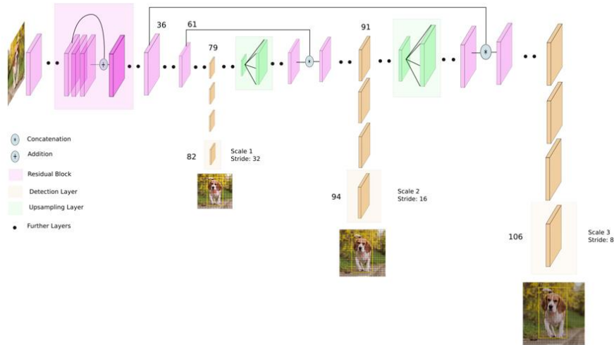
Figure 4.1. YOLOv3 architecture.
