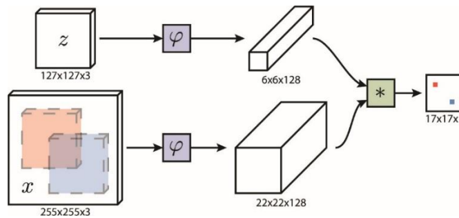
Figure 4.7. SiameseFC architecture [85].
