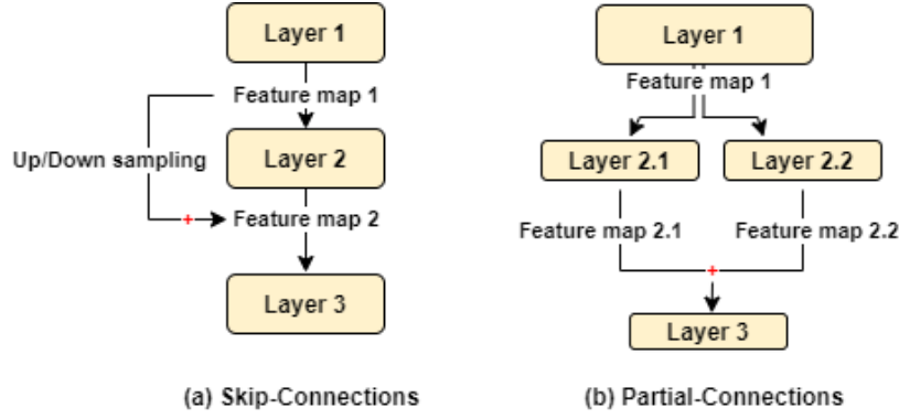
Figure 7.1. Example diagram for partial and skip connections.
