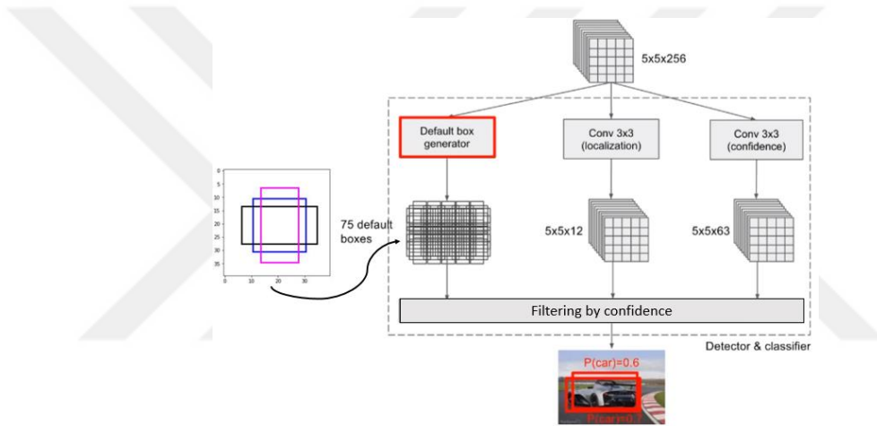
Figure 4.4. Fourth D&C network in the SSD network [67].
