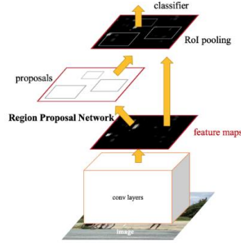
Figure 4.5. Faster R-CNN architecture overview [28].
