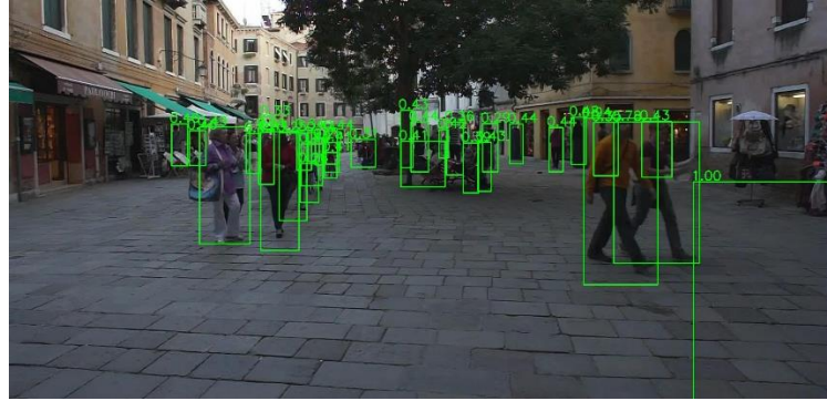
Figure 7.4. Sample Yolo-v4 detection output from sequence MOT17-02 frame 1.
