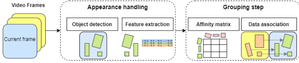
Figure 1.3. DL based trackers pipeline.
