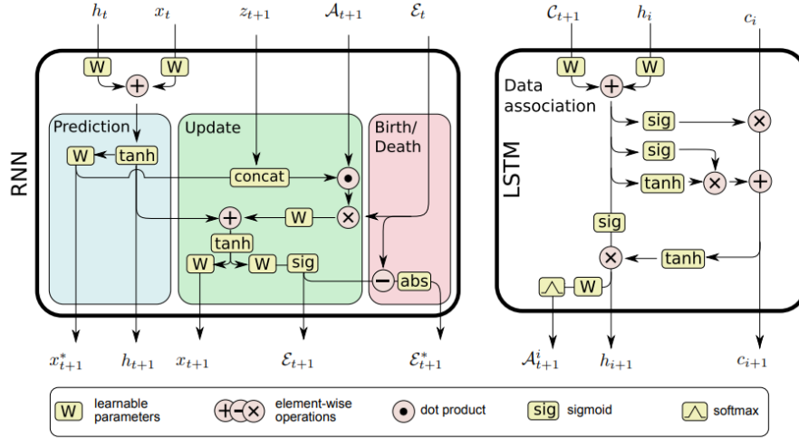
Figure 5.4. Summary of the tracker proposed in [99].
