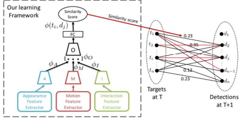
Figure 5.5. Summary of [100] end-to-end DL based affinity computation.
