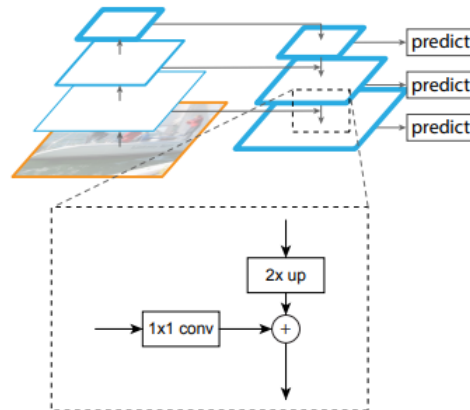
Figure 6.1. Faster R-CNN Feature Pyramid building block [116].
