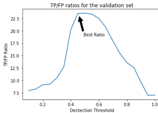
Figure 7.5. TP/FP ratios of Yolo-V4 detections on the validation set.
