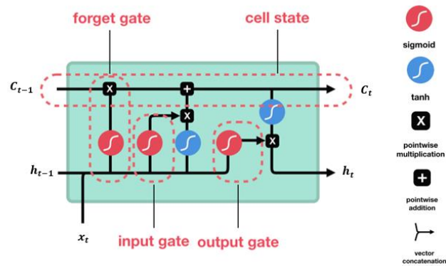
Figure 2.12. Standard LSTM cell [38].
