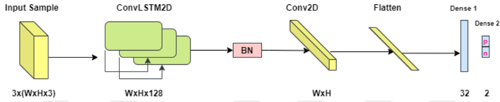
Figure 7.12. The graphical representation of the proposed CLSN.
