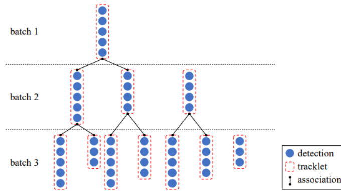
Figure 5.7. Tracklets association framework. It constructs a tree which is updated while tracking with a window of 3-5 frames [106]. A batch refers to the recent 3-5 consecutive frames detections associated together.
