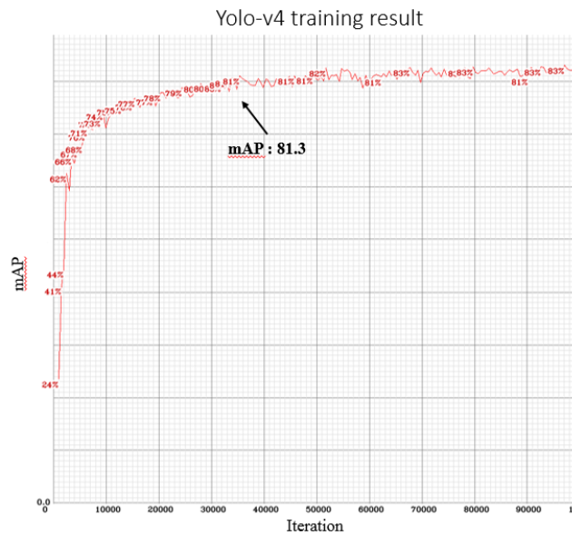
Figure 7.3. Yolo-v4 performance after training.
