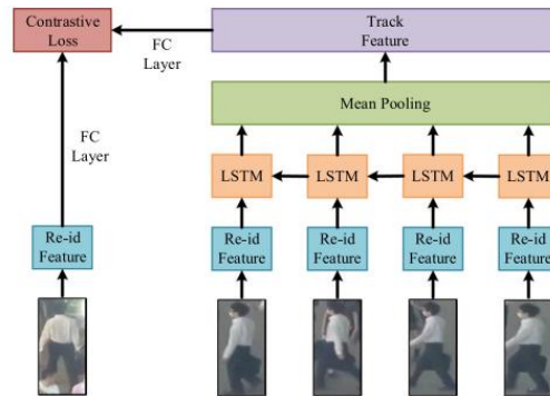
Figure 5.2. Enhanced bLSTM topology by [97]. Re-ID features are collected from the LOMO appearance model proposed by S. Liao et al. [98].
