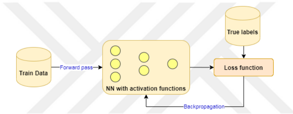
Figure 2.5. Supervised learning based NN pipeline.
