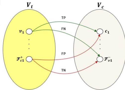
Figure 3.12. Example ID Bipartite graph with one tracklet for demonstration.
