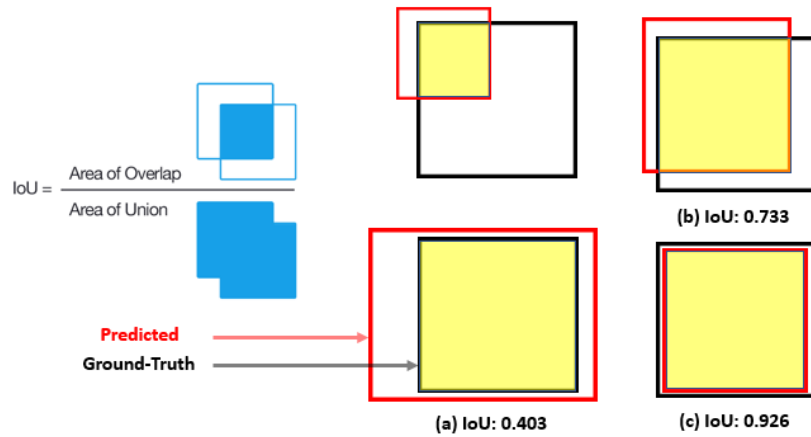
Figure 3.9. An example of computing IoU for various bounding boxes.
