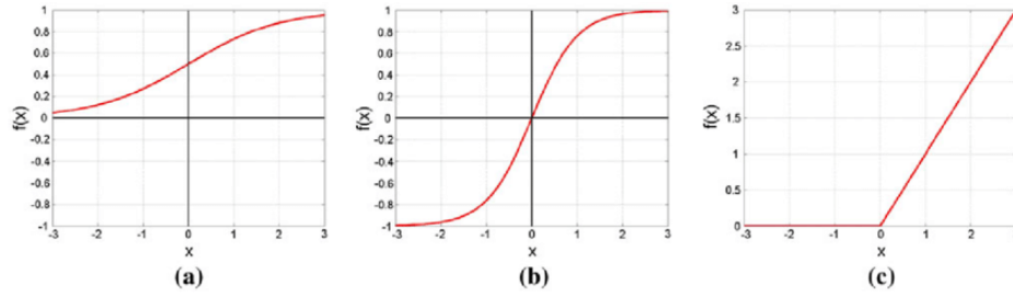
Figure 2.6. (a) Sigmoid function, (b) Tanh function, (c) ReLU function.
