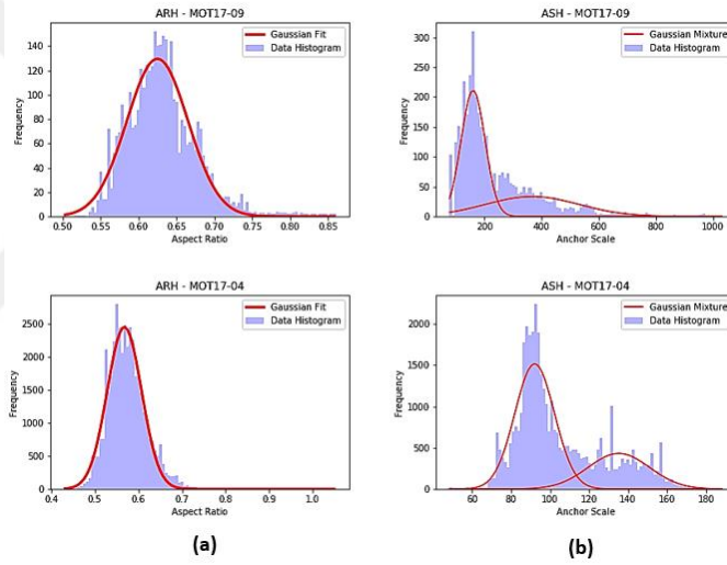
Figure 7.7. Sample AR and AS histograms for both MOT17-09 & 04 sequences.
