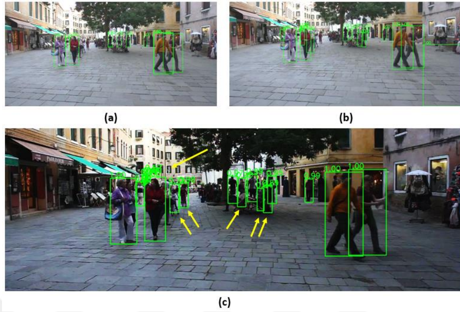
Figure 7.6. (a) original Faster R-CNN detection with a 0.5 filtering threshold. (b) Yolo-v4 experiment 2 example output. (c) Integrated Yolo + Faster R-CNN output.
