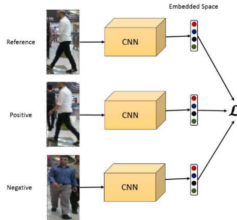
Figure 7.9. Sample training cycle where input x is fed to shared weights CNNs and the resultant features are used to compute the triplet loss \mathcal{L} .
