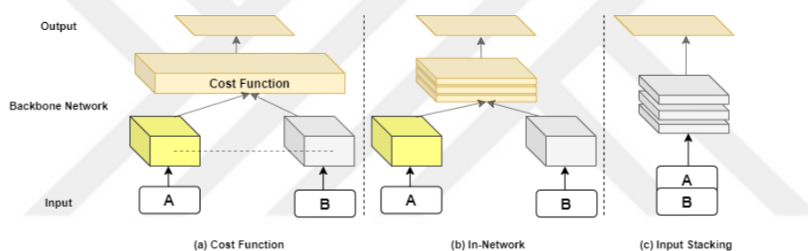
Figure 4.8. Summary of common Siamese topologies.
