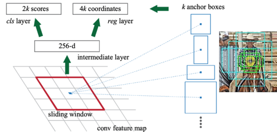
Figure 4.6. Region Proposal Network (RPN) [28].
