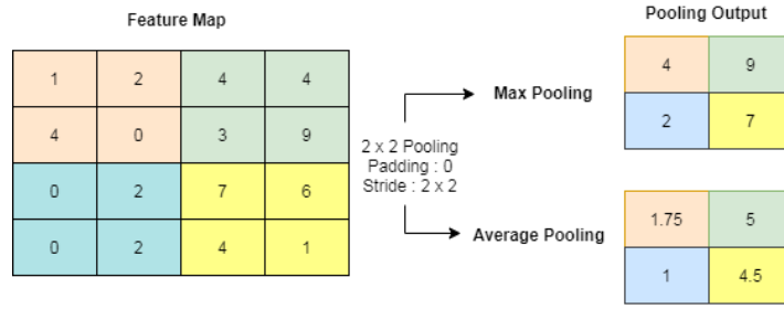
Figure 2.9. Average and max-pooling example. Better viewed with colors.
