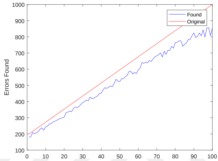
Figure 4.4: err found lin
