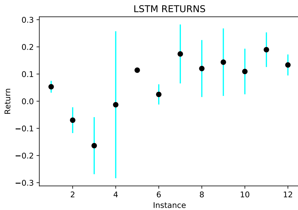
Figure 3.12: LSTM Returns with Std Error on Dataset4
