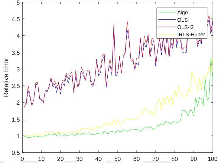
Figure 4.1: Relative Err Lin
