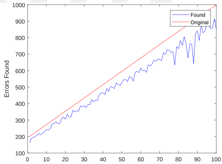
Figure 4.8: err found nonlin
