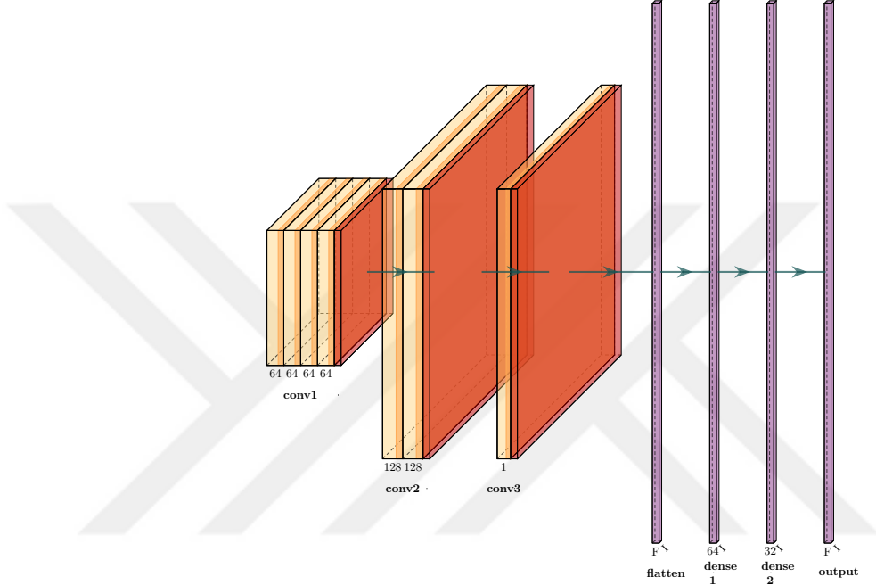
Figure 3.2: Proposed GNN Architecture
