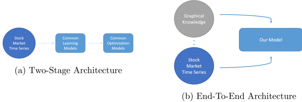
Figure 3.1: Deep Learning Architectures for Portfolio Optimization
