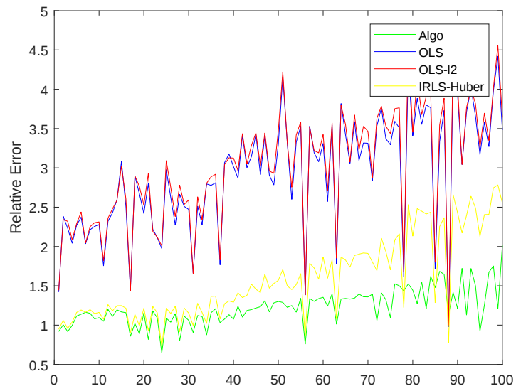
Figure 4.5: relative err nonlin
