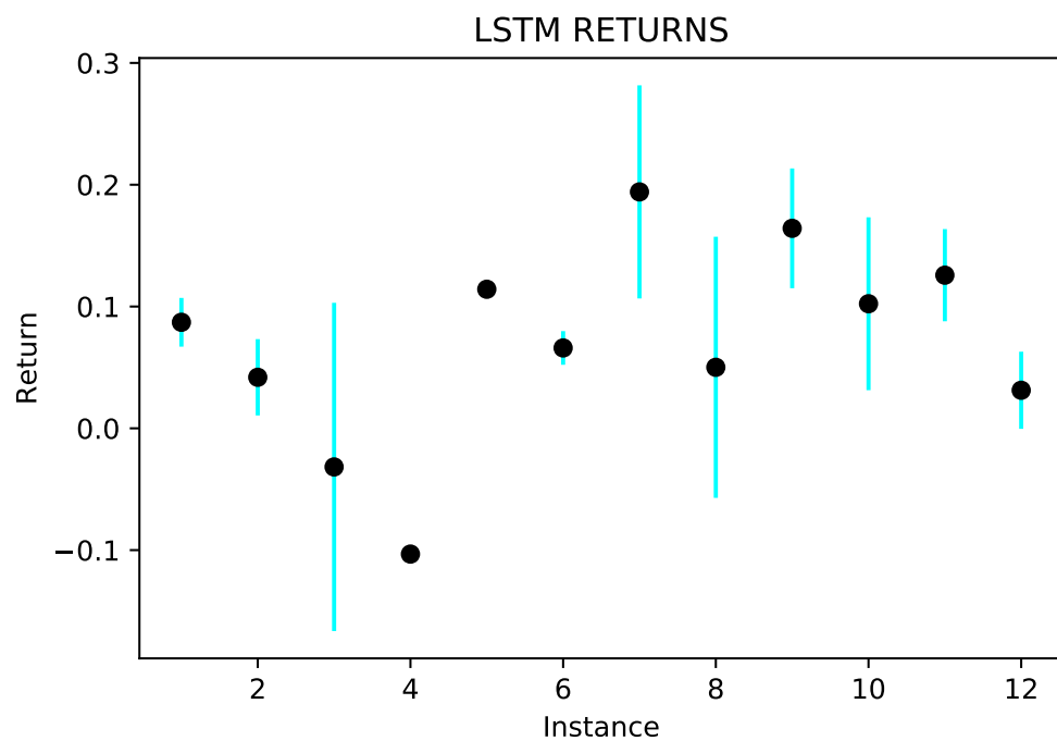
Figure 3.8: LSTM Returns with Std Error on Dataset2
