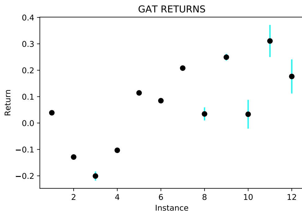
Figure 3.7: GAT Returns with Std Error on Dataset2
