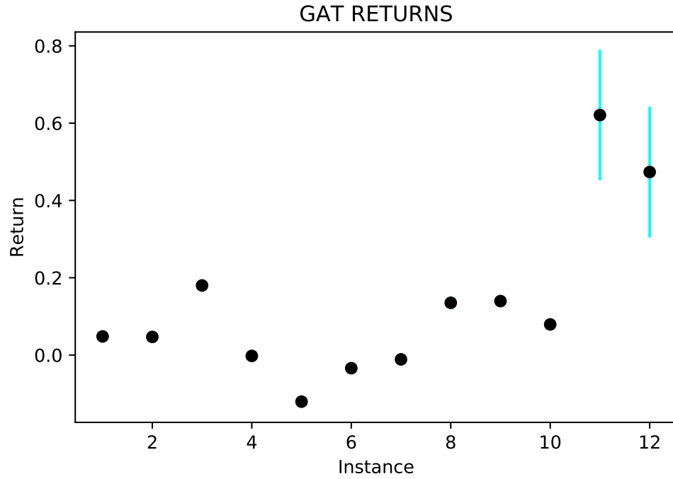
Figure 3.3: GAT Returns with Std Error on Dataset1
