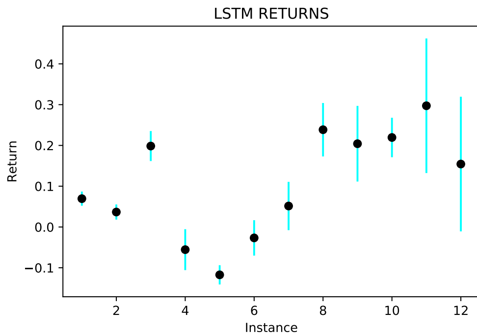
Figure 3.4: LSTM Returns with Std Error on Dataset1
