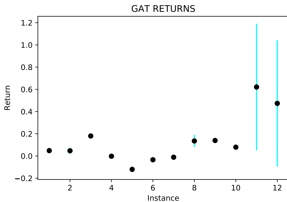
Figure 3.5: GAT Returns with Max Error on Dataset1
