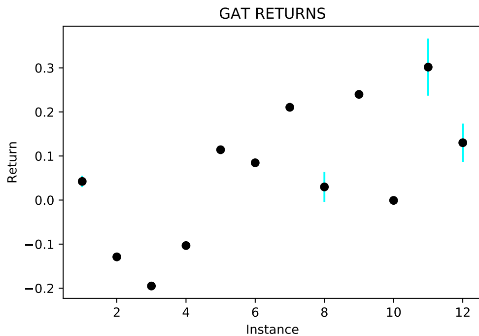
Figure 3.11: GAT Returns with Std Error on Dataset4
