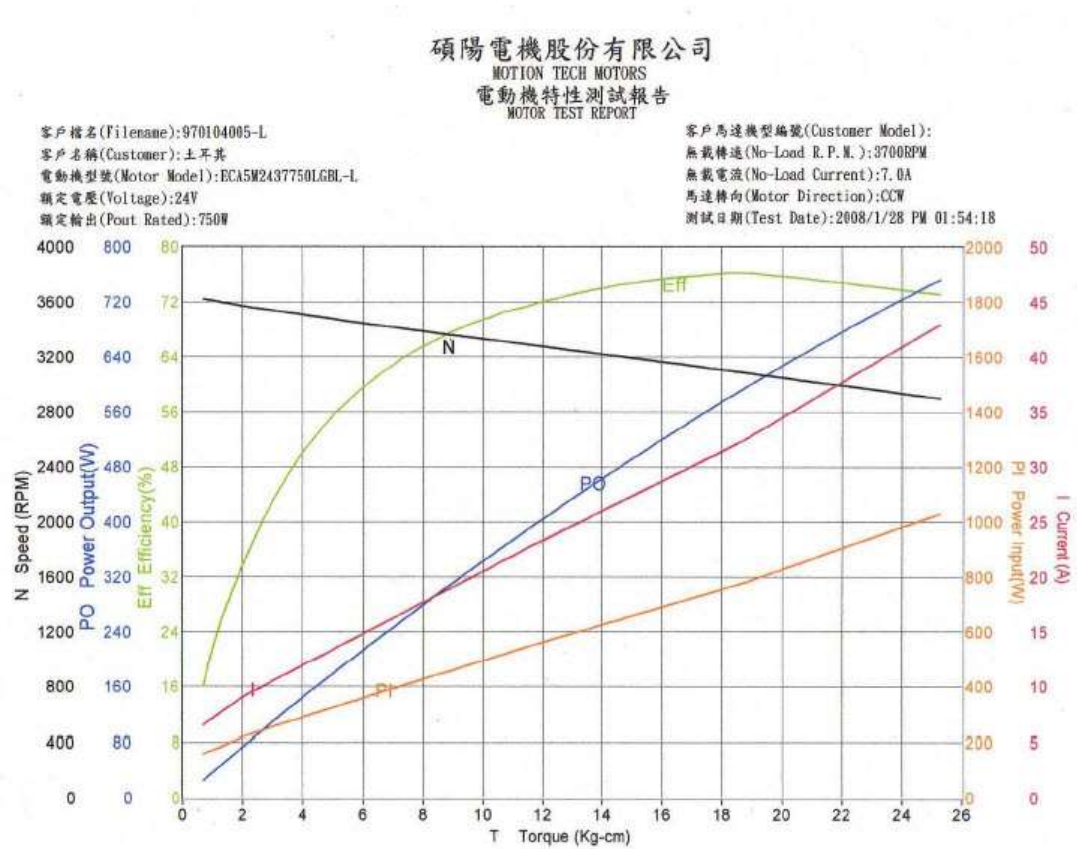
Figure 7.2 Motor test diagram
