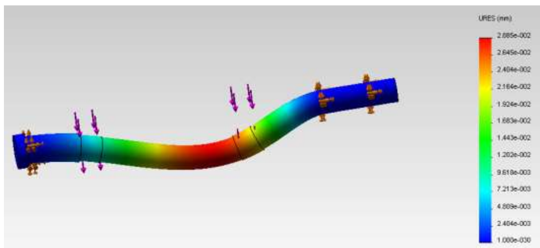
Figure 3.7 Front axle displacement results
