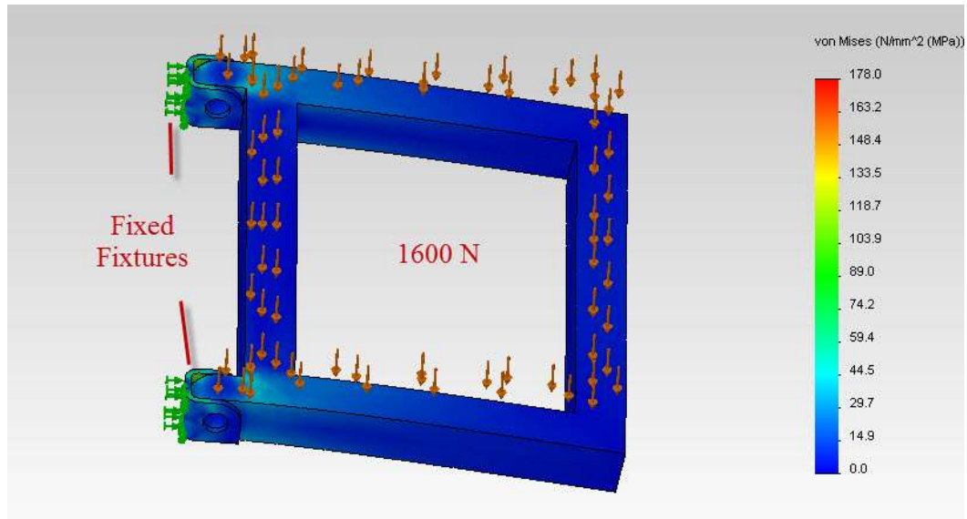
Figure 3.18 Manual ladder Von-Mises stress results
