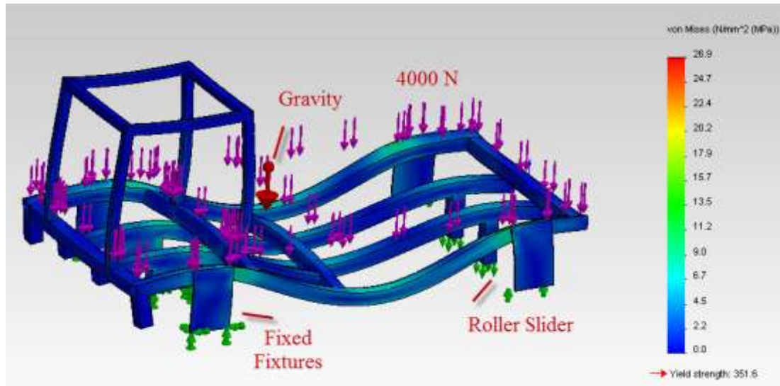
Figure 3.10 Main chassis Von-Mises stress results
