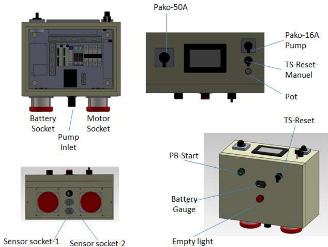
Figure 4.1 Control panel
