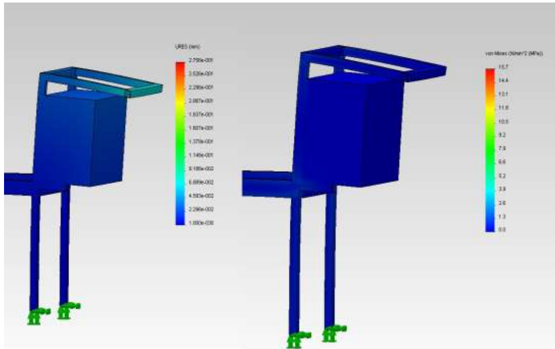
Figure 5.11 Fixed panel static analysis
