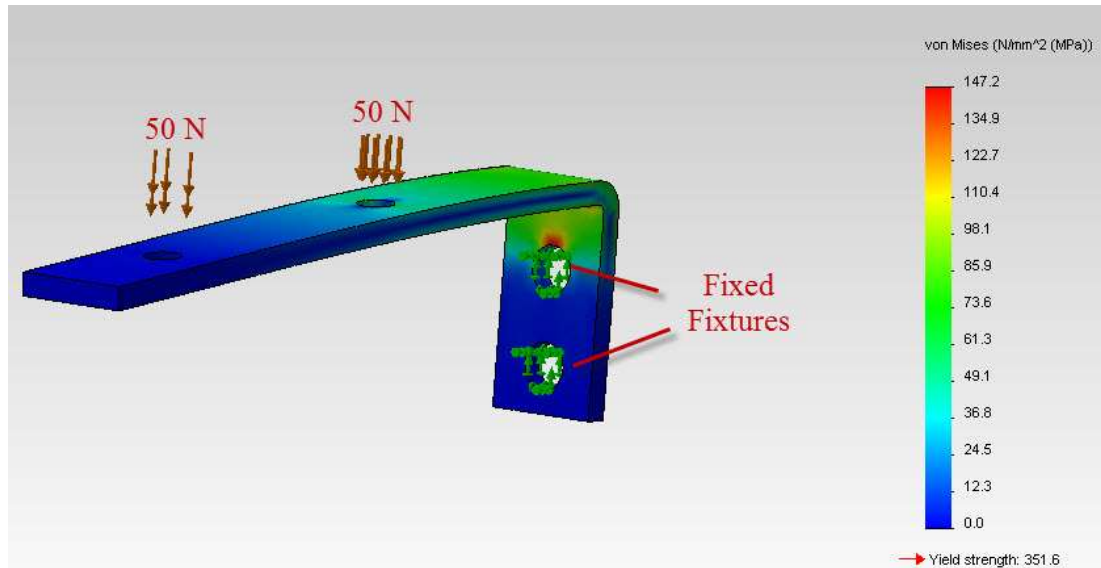
Figure 3.16 Panel flexible beam Von-Mises stress results
