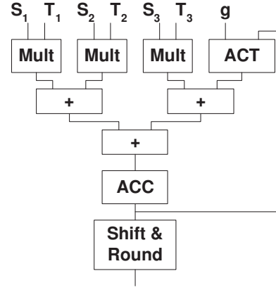
Figure 3.17 Arithmetic unit of a CASTLE processor [6]
