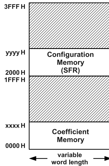
Figure 4.6 Memory map of a block with a serial communication interface
