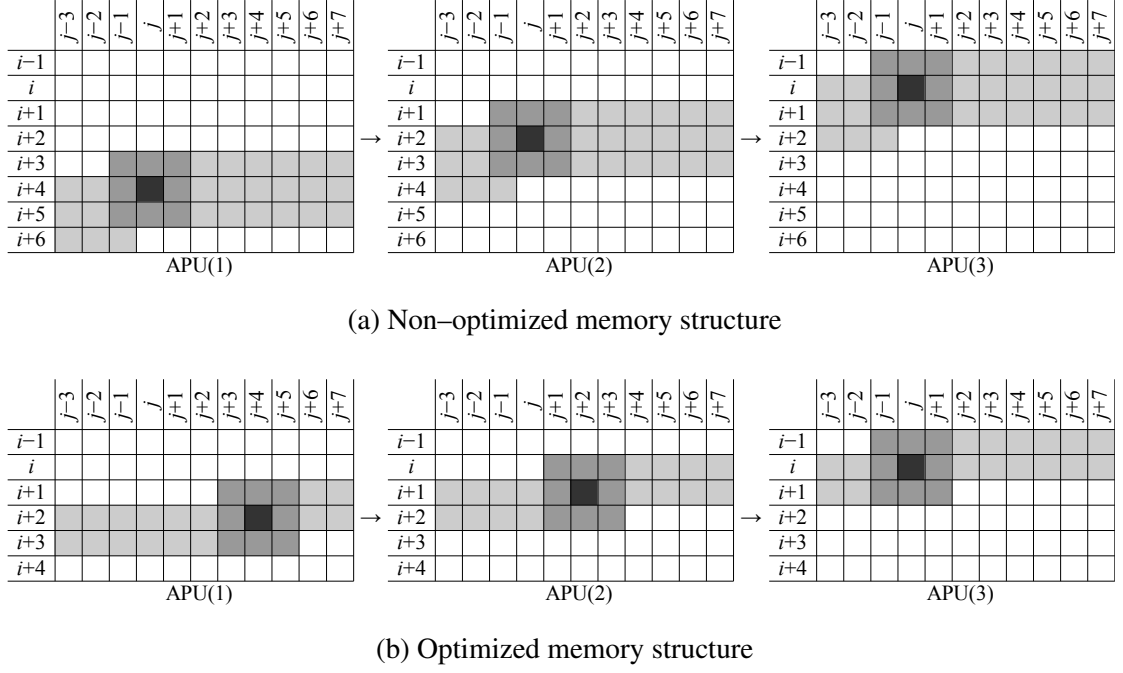
Figure 4.3 Memory usage of consequent APUs (light gray), and pixels that are being processed (dark gray)
