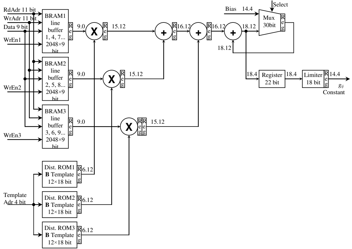
Figure 3.27 Block diagram of BPU of Steadfast-I [13]
