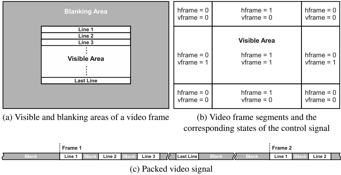
Figure 4.4 Video frame structure defined by video display interfaces and its packing scheme
