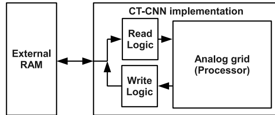
Figure 3.2 Block diagram of a CT CNN implementation
