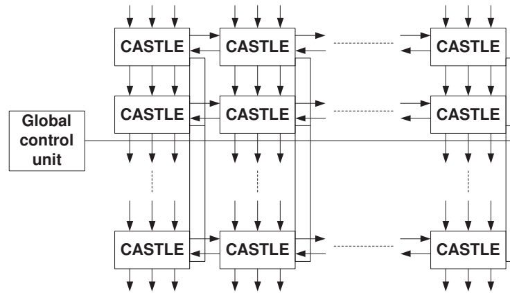
Figure 3.14 Processor organization of the CASTLE architecture [6]
