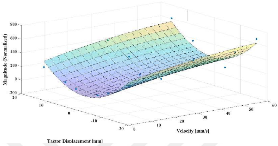
Figure 4.5: The skin stretch intensity perceived by the participants is modeled as a function of tactor displacement and velocity, utilizing the second order model given in (4.4). R^2 of the fit is 0.88.
