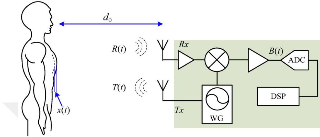
Figure 2.9. Simplified block diagram of CW/FMCW radar sensor and the mechanism of noncontact vital sign detection.
