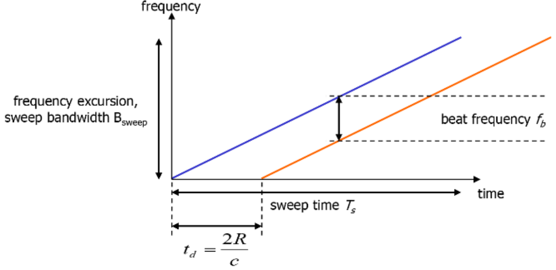
Figure 2.11. Sawtooth modulated chirp
