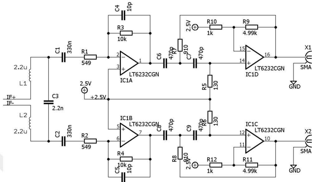
Figure 3.7. Baseband circuit schematic diagram
