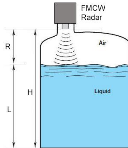
Figure 2.7. Fluid level sensor based on FMCW radar
