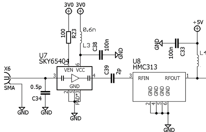
Figure 3.6. LNA circuit schematic diagram
