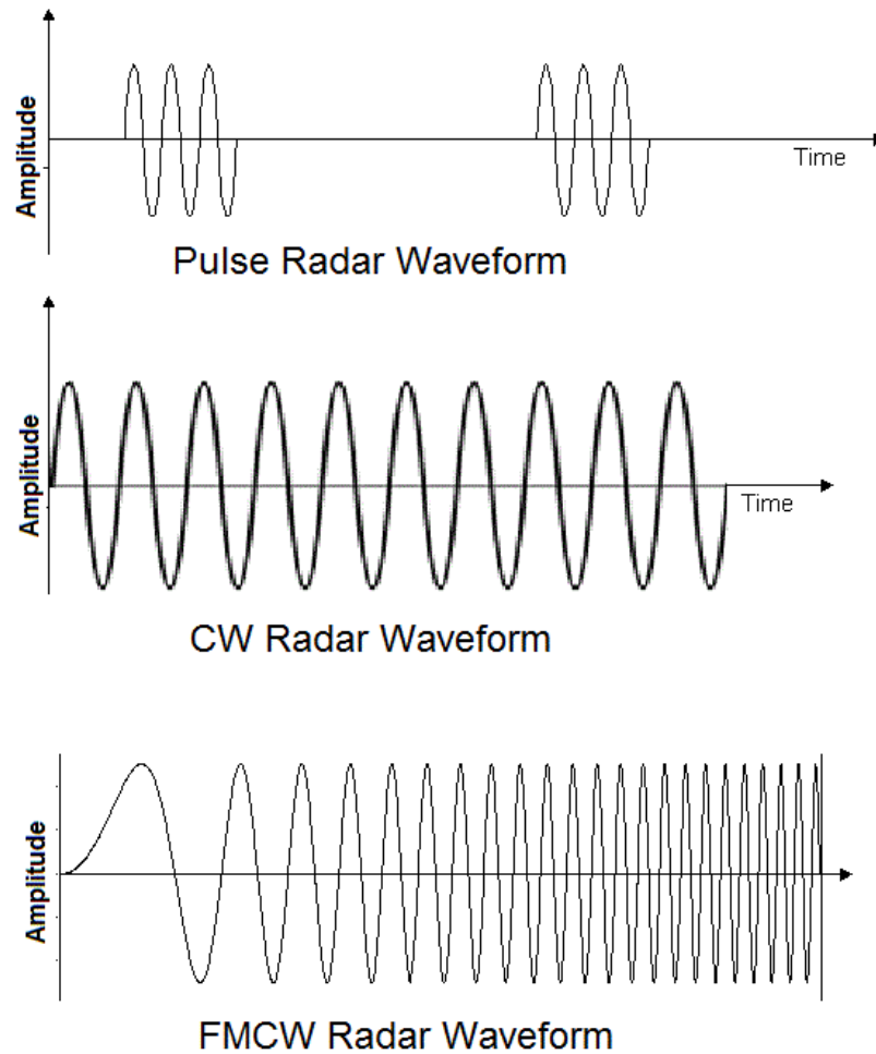
Figure 1.3. Waveform of pulse, CW, and FMCW radars
