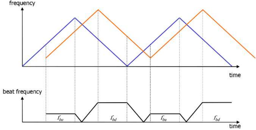
Figure 2.12. Triangular modulated chirp
