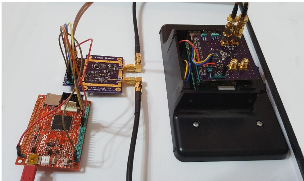
Figure 4.2. System modules connection
