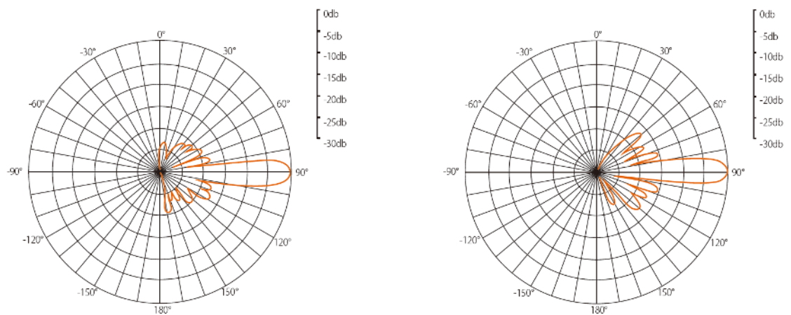
Figure 3.14. TL-ANT5823B antenna radiation patterns
