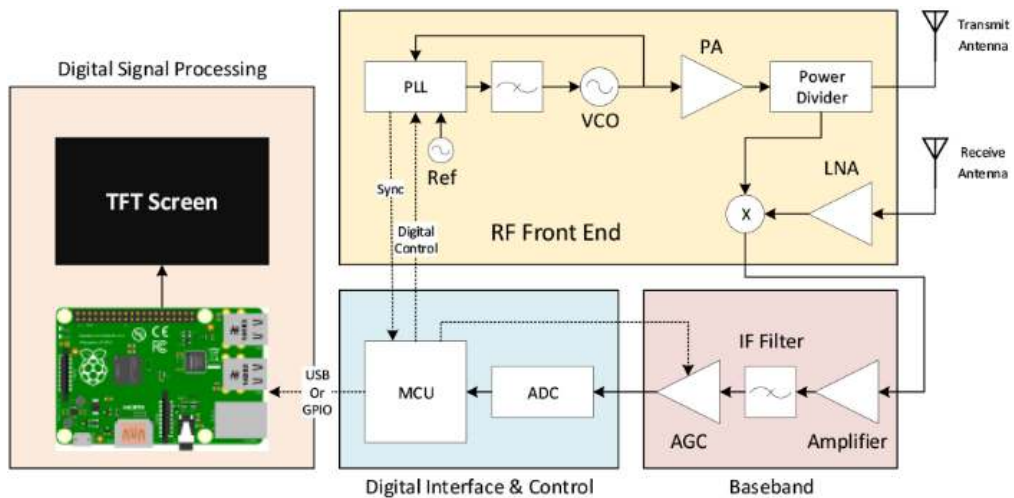
Figure 3.1. Block diagram of proposed FMCW radar
