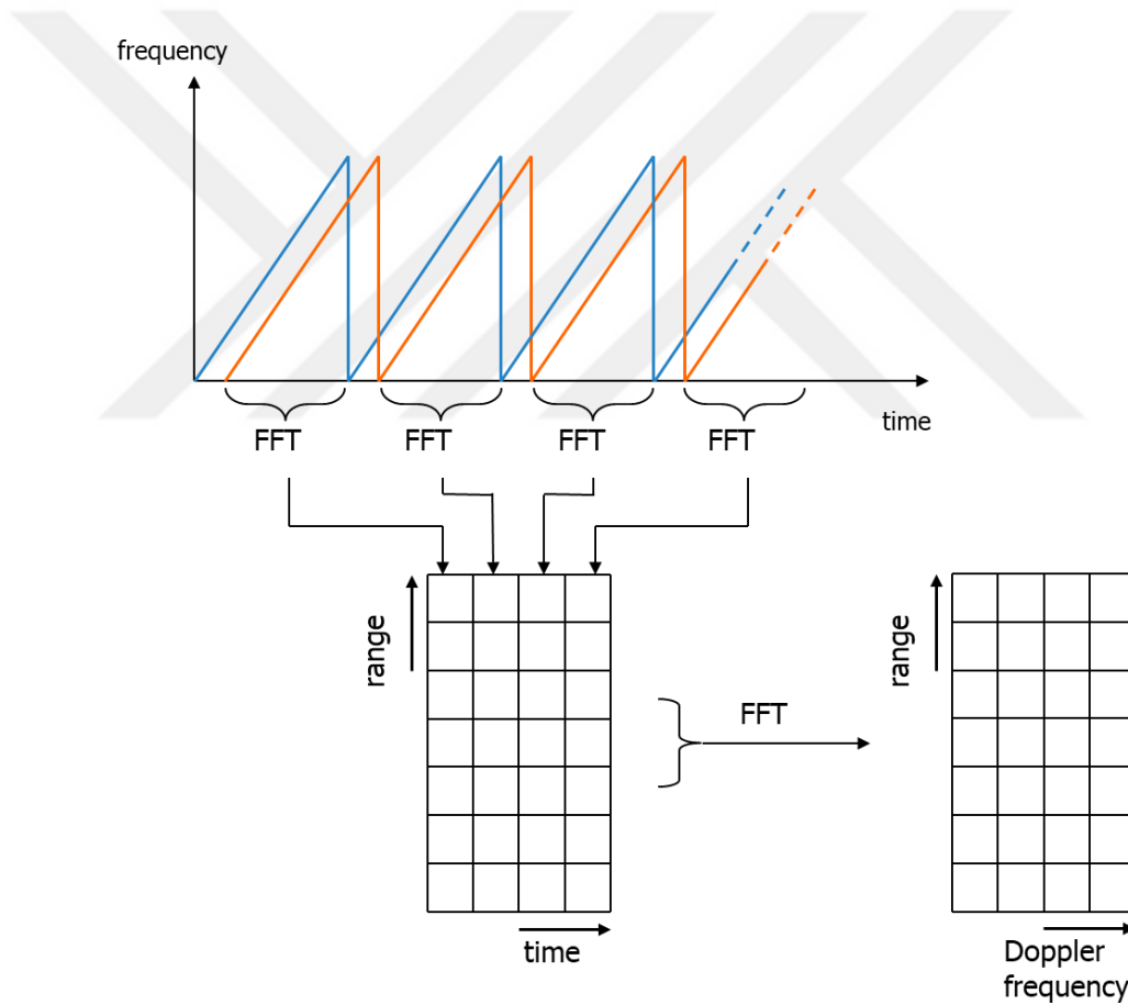
Figure 3.15. FMCW signal processing
