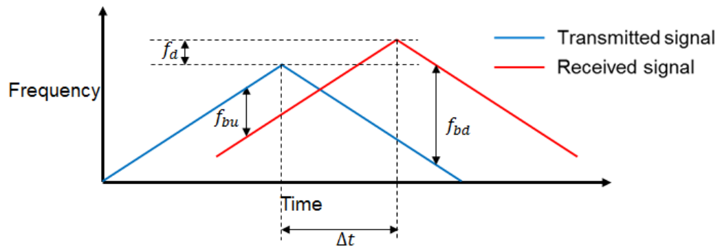
Figure 2.4. FMCW radar triangular sweep
