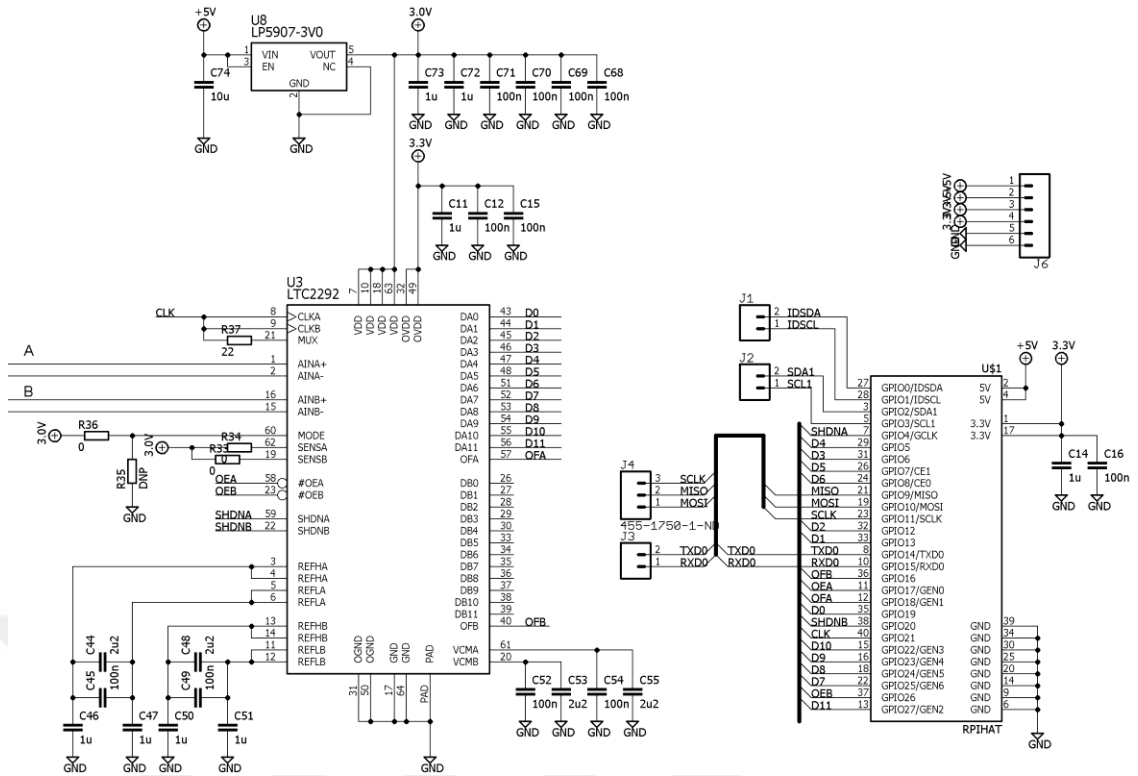
Figure 3.9. ADC interface circuit schematic diagram
