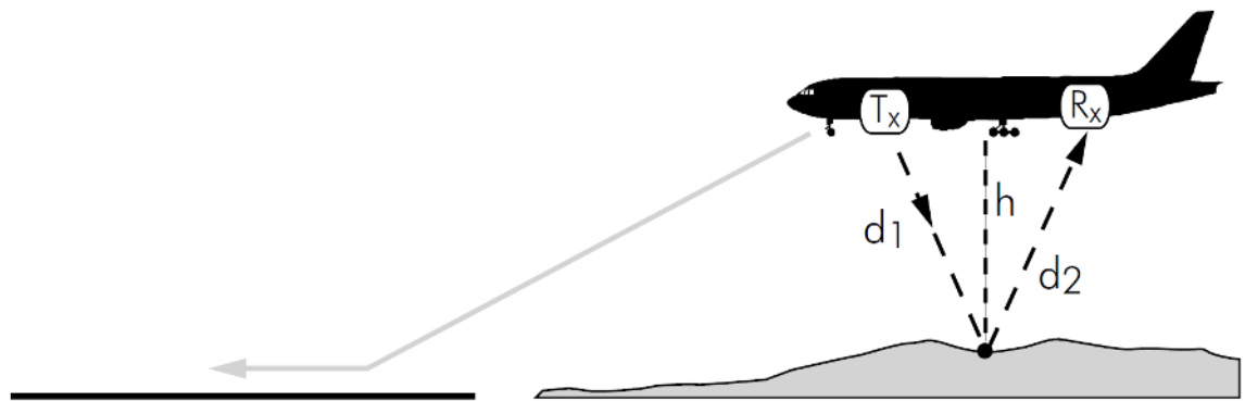
Figure 2.5. Radio altimeter principle
