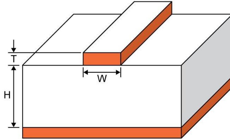
Figure 3.13. Microstrip transmission line structure
