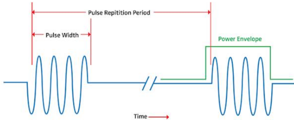
Figure 1.2. Pulse radar waveform
