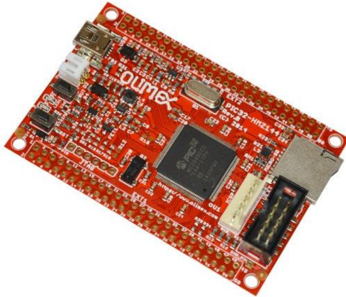
Figure 3.10. PIC32-HMZ144 board
