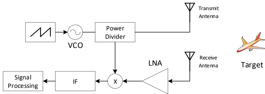
Figure 2.13. FMCW radar block diagram
