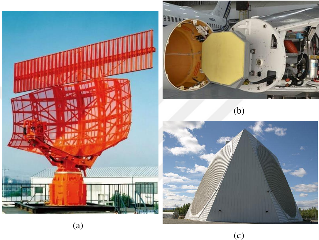
Figure 1.1. Examples of radar systems: (a) ASR-9 air traffic control radar, (b) APG-83 Scalable Agile Beam Radar (SABR) AESA for the F-16, and (c) PAVE PAWS Phased Array Warning System
