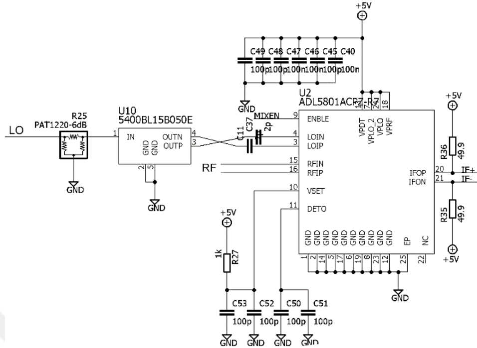
Figure 3.5. Mixer circuit schematic diagram
