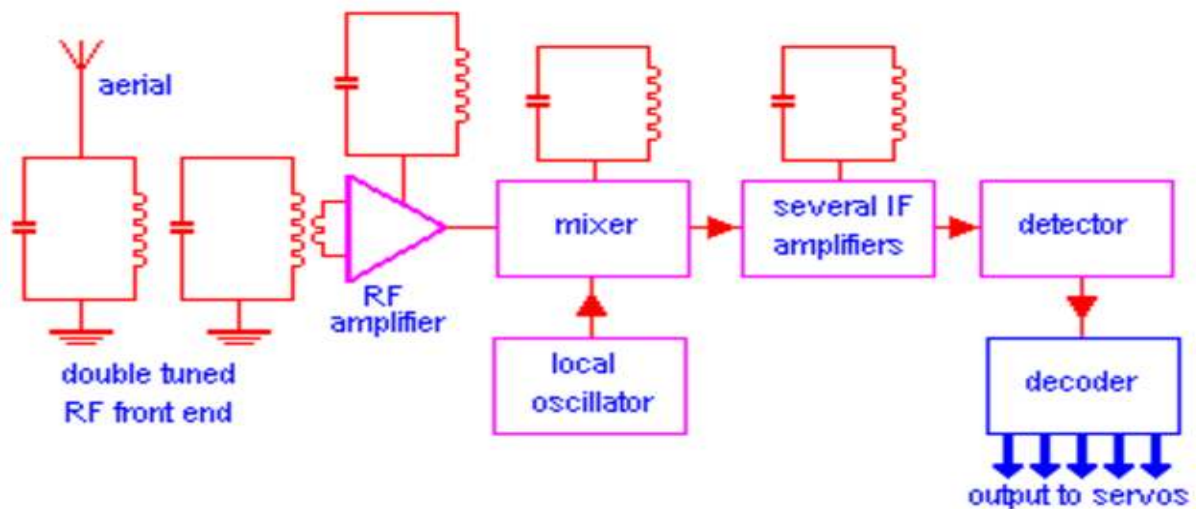
Fig. 5.14 Single conversion superheterodyne receiver
