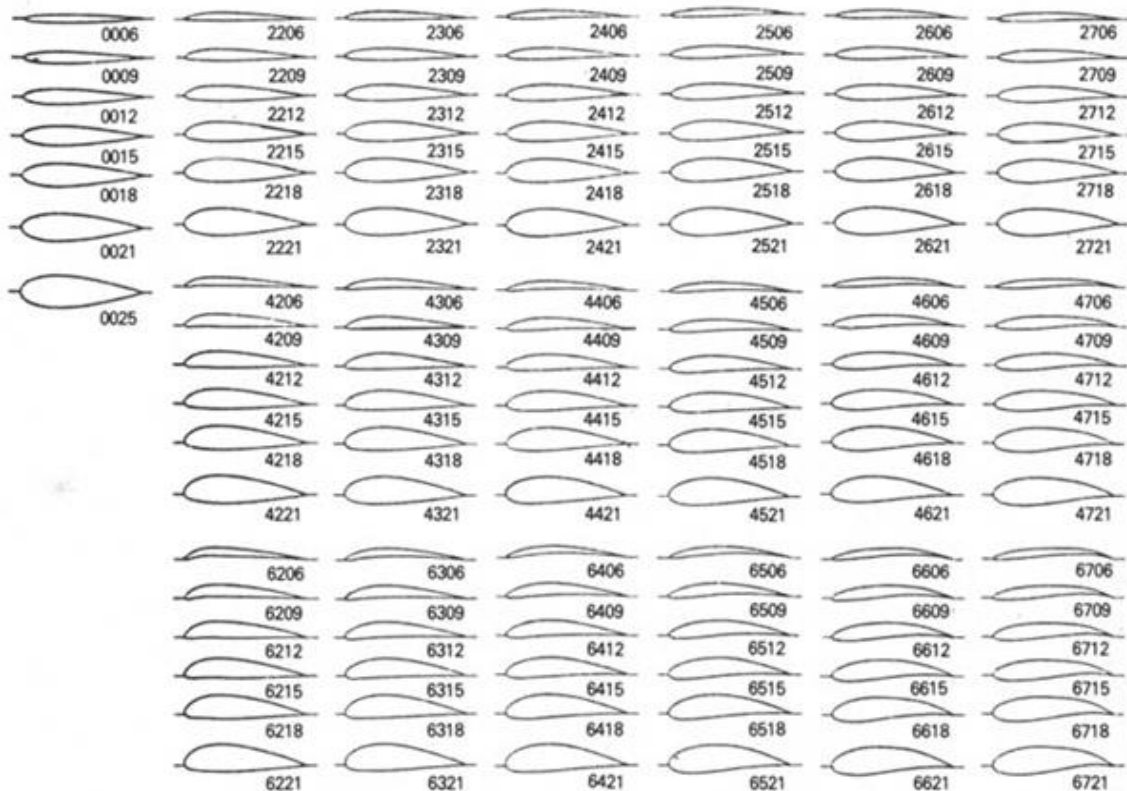
Fig. 3.8 Airfoil families [18]
