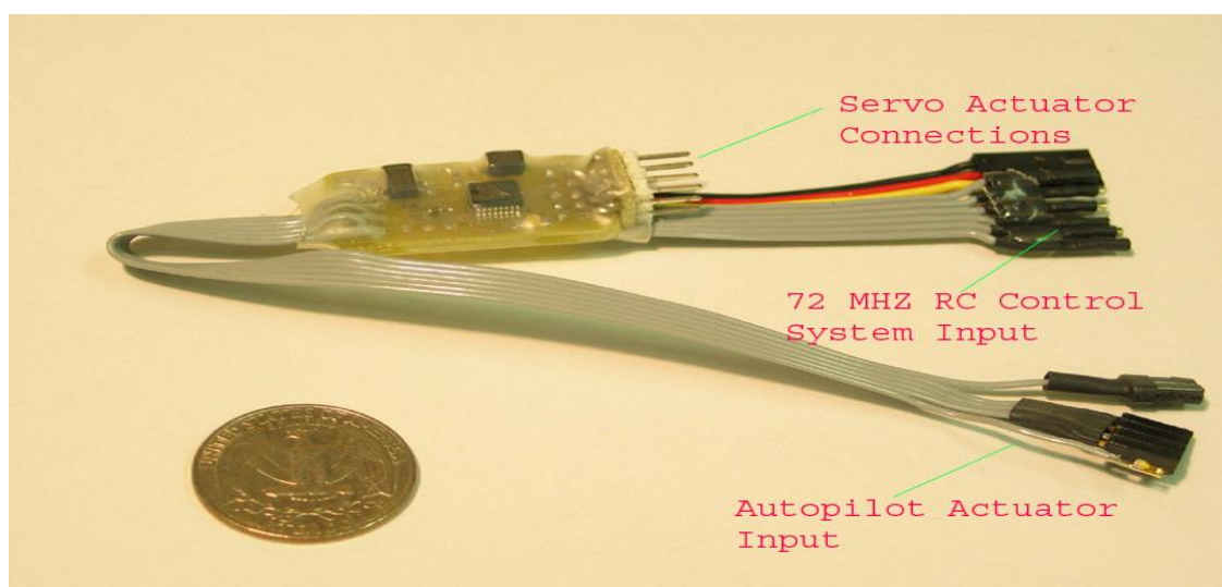
Fig. 7.5 Bypass circuit
