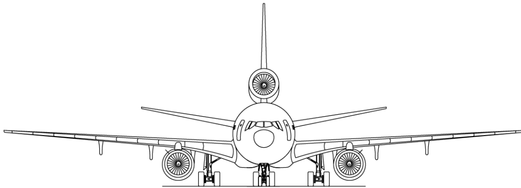
Fig. 3.10 Wing dihedral [25]
