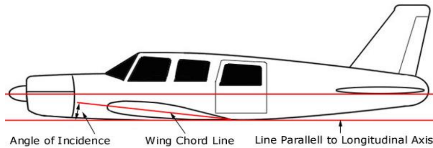
Fig. 3.9 Wing incidence [24]
