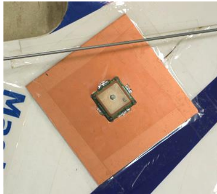
Fig. 7.3 GPS receiver
