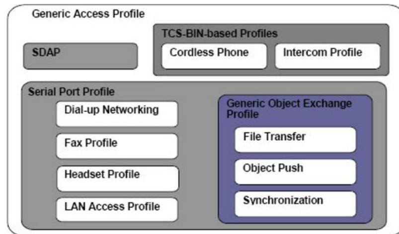
Figure 2.4. Bluetooth profile [4-5]
