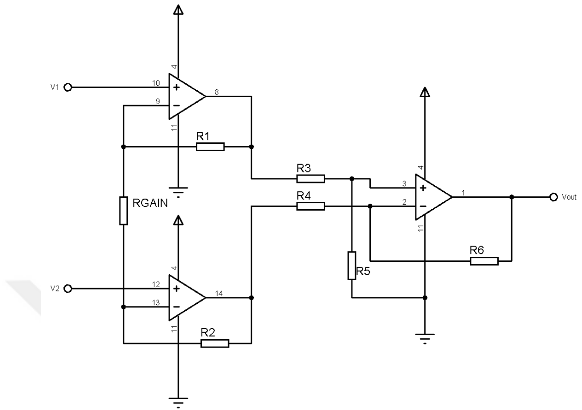
Figure 2.8 Schematic of instrumentation amplifier
