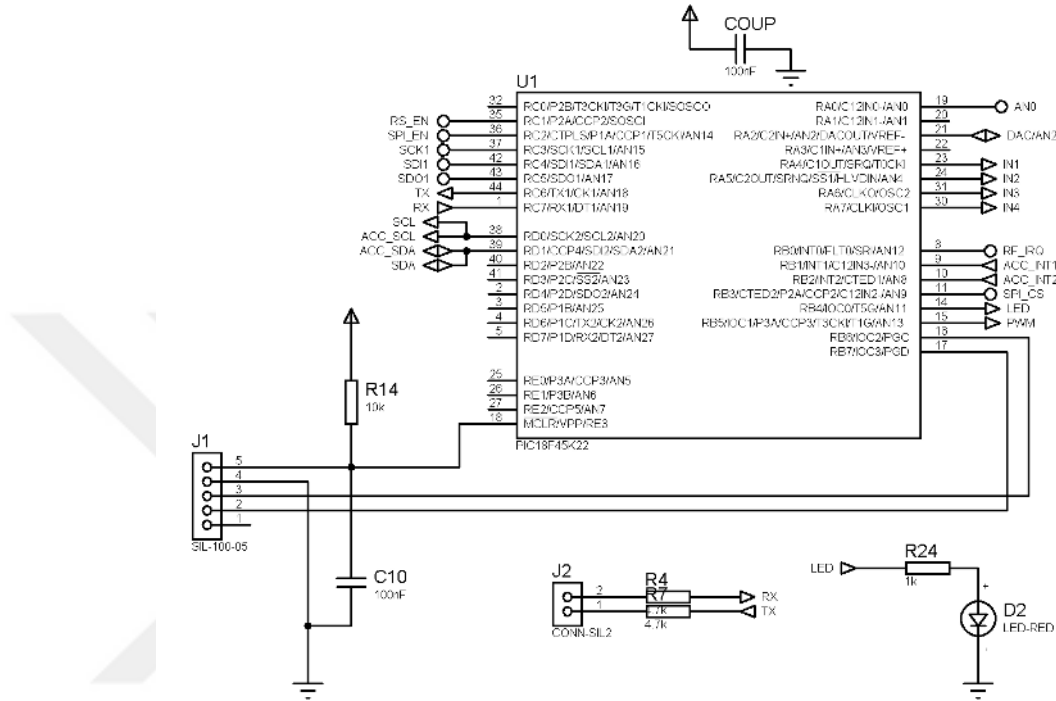
Figure 3.2 Pin layout of microcontroller
