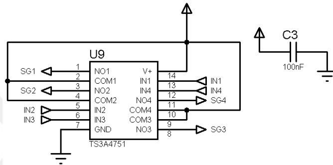
Figure 3.10 Analog switch for powering up strain gauges
