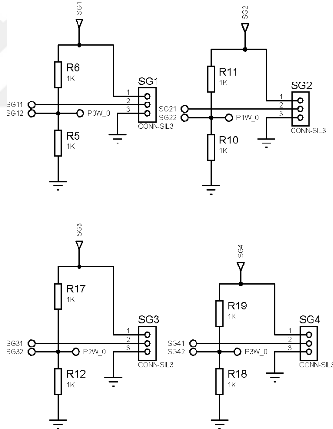
Figure 3.9 Strain gauge inputs
