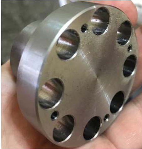
Figure 6.23 The final shape for the pin holder.
