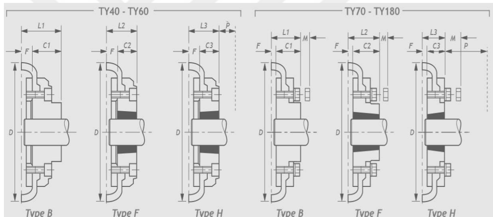
Figure 7.17 Technical drawing for Tyreflex coupling.
