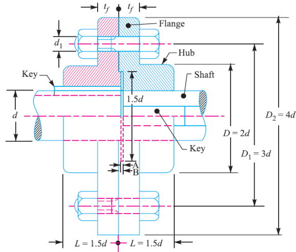
Figure 3.1 Unprotected flange.
