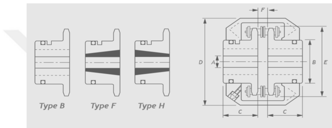
Figure 7.19 Technical drawing for Chainflex coupling.
