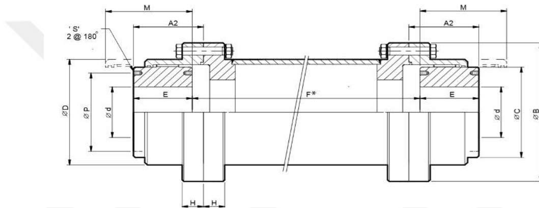
Figure 7.22 ET Spacer Tube coupling technical drawing.
