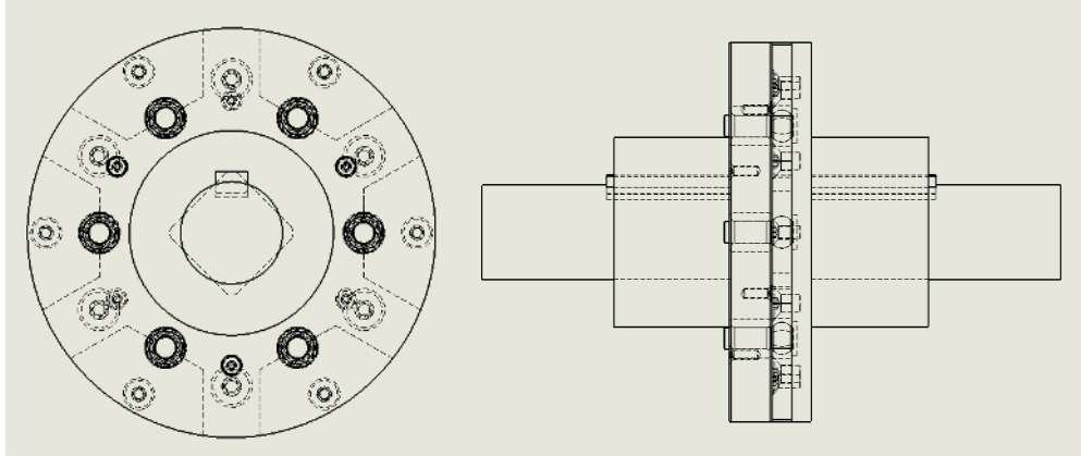
Figure 4.3 Technical drawing of the new coupling.
