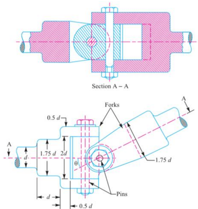
Figure 3.12 Universal coupling.
