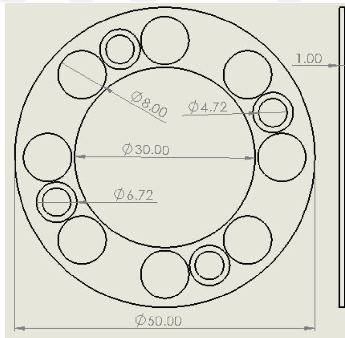
Figure 6.5 Technical drawing of the plate.
