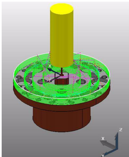
Figure 6.9 CNC milling proccess for middle holder.
