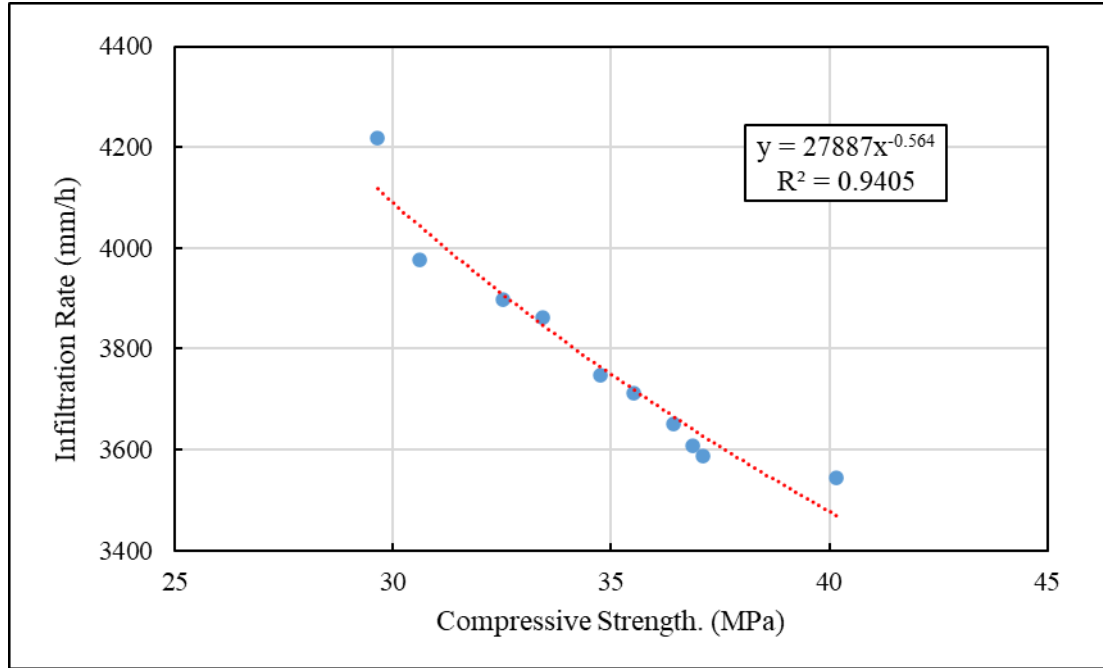
Figure 4.10 Compressive strength and Infiltration Rate
