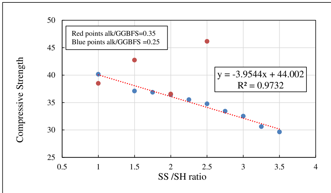
Figure 4.3-a Effect of SS/SH ratio on compressive strength
