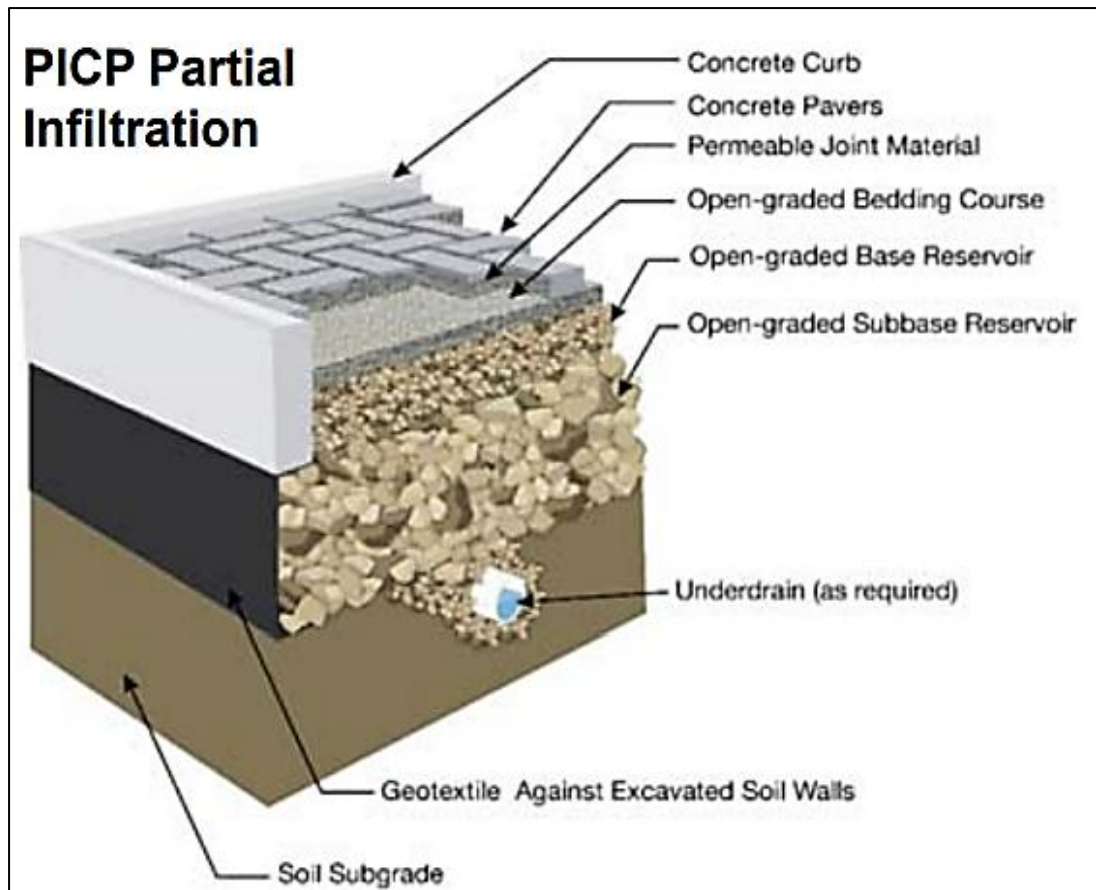
Figure 5.1 Typical cross-section of pervious concrete paver units
