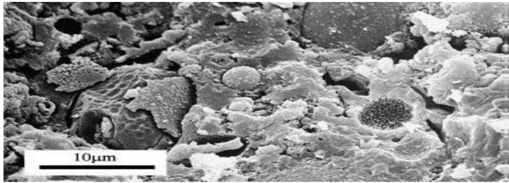
Figure 2.3 Micrographs of alkali-activated PFA geopolymer fracture surface. (Jiminez et al. 2004)
