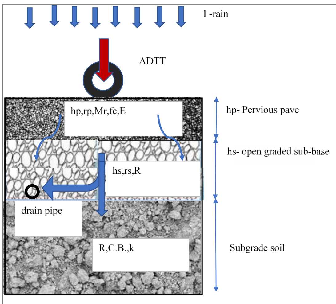
Figure 5.7 Pervious concrete pave design for the study
