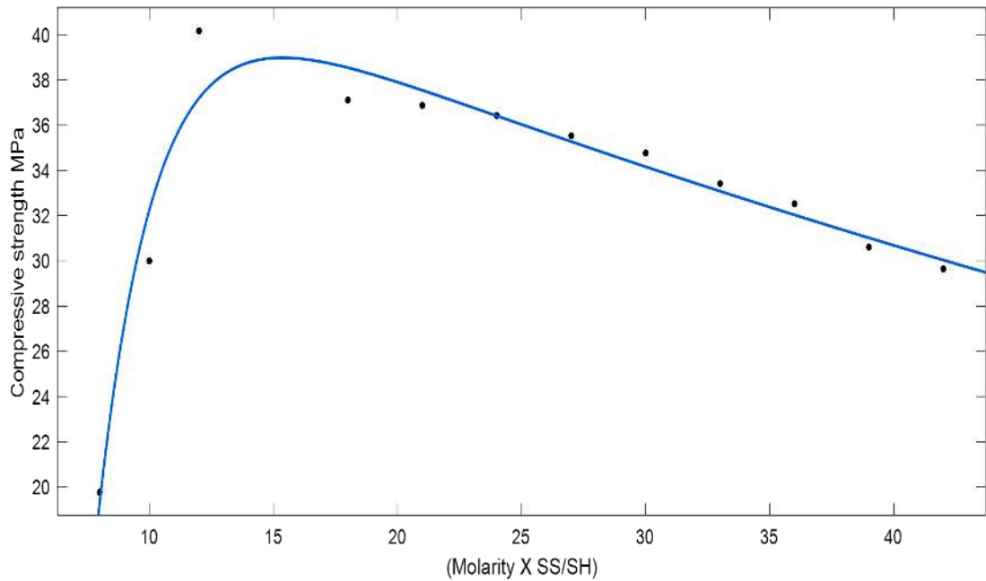
Figure 4.4-a the effect of (Molarity X SS/SH) on the Compressive Strength of GPPC produced with maximum size of 14 mm, Alk/GGBFS ratio of 0.25 and GGBFS content 325 \text{ kg/m}^3
