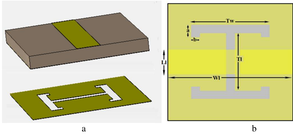
Figure 4.74 (a) 3D view of the T-Shaped DGS resonator. (b) front view
