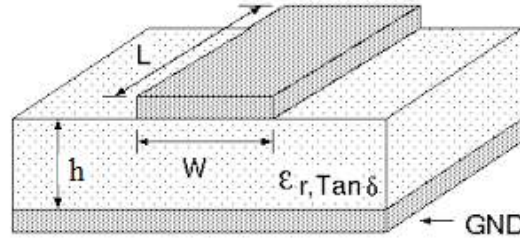
Figure 2.3 Microstrip line
