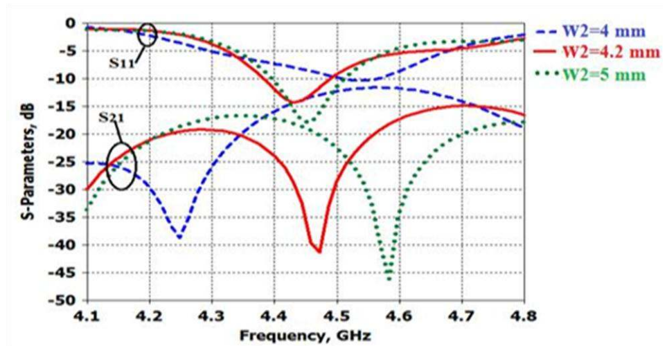
Figure 4.38 S-parameters for various length W2 of LSCW.
