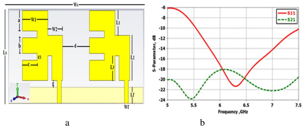
Figure 4.1 a) The proposed MIMO system, b) S-Parameters.
