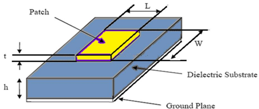
Figure 2.1 Microstrip patch antenna
