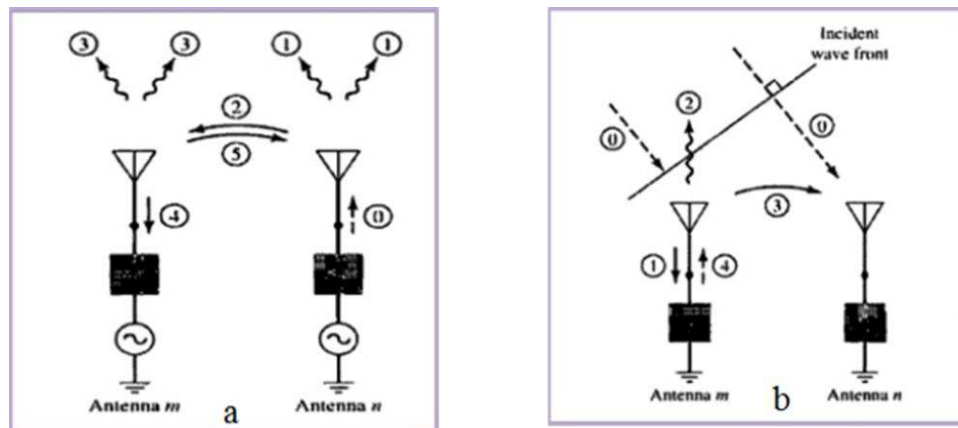
Figure 3.1 Mutual coupling path [45] (a): Coupling paths between antennas m and n at transmitting mode. (b): Coupling paths between antennas m and n at receiving mode.
