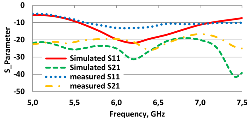
Figure 4.9 Comparison between simulated and measured S-parameters with the CSR matrix of the proposed MIMO system [34].
