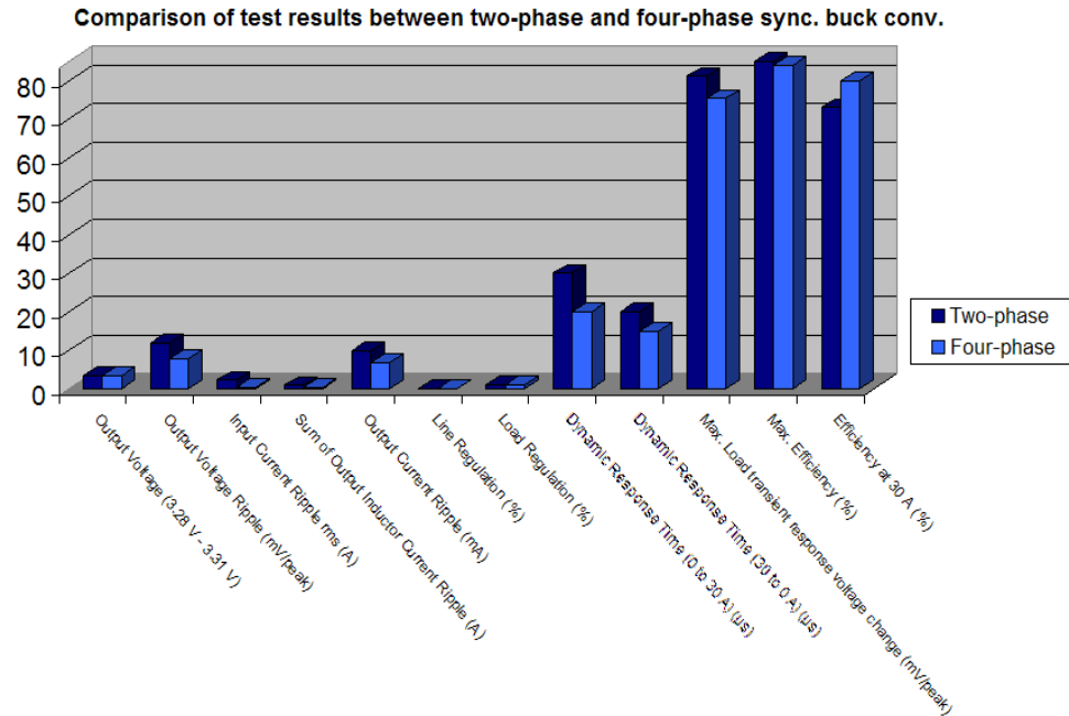
Figure 5.60 Comparison of test results among two-phase and four-phase synchronous buck converter.
