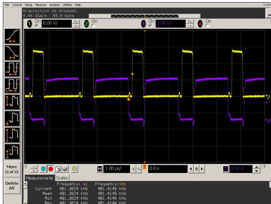
Figure 5.35 High side MOSFET and low side MOSFET PWM signals of third phase.
