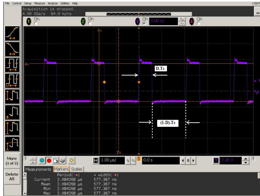
Figure 5.40 Waveform of phase1 inductor voltage during charging and discharging time.
