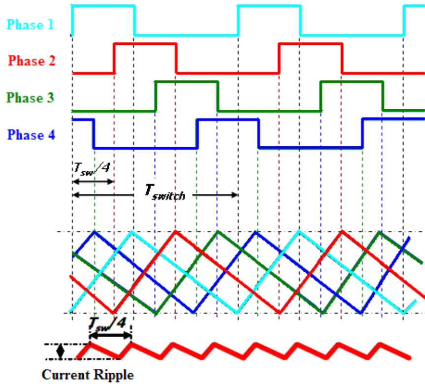
Figure 2.9 Main waveforms of four-phase synchronous buck converter in steady state conditions.
