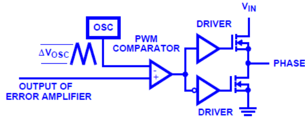
Figure 3.9 The modulator (Mattingly, 2003).
