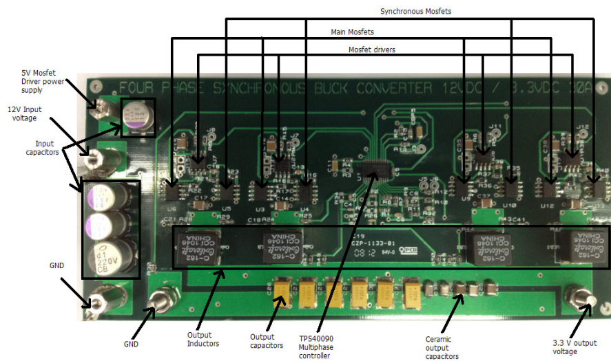
Figure 5.11 General view of the four-phase synchronous buck converter.
