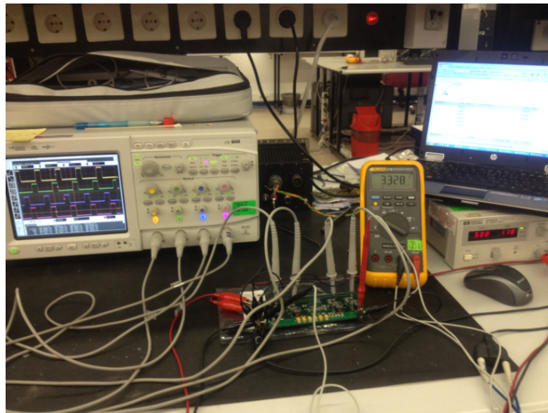
Figure 5.37 Photo of measurement of output voltage without load.
