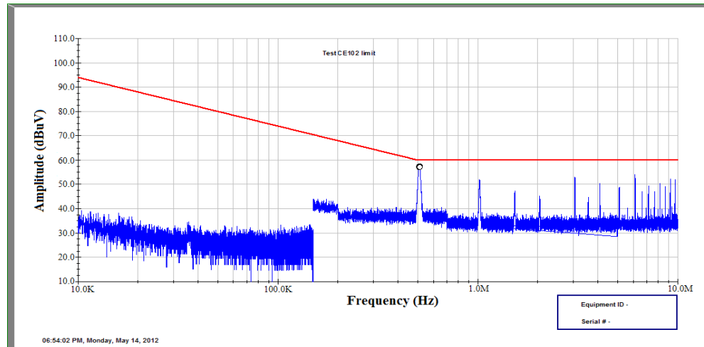
Figure 5.55 CE102 test results for four-phase buck converter (+ power line).
