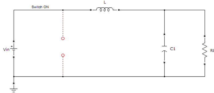
Figure 2.2 Non-synchronous buck converter, when the switch is ON.
