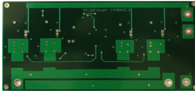
Figure 5.9 Photos of the designed four-phase buck converter PCB (a: component side, b: solder side)
