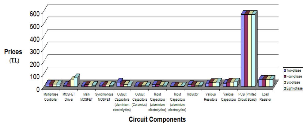
Figure 5.58 Cost comparisons among two-phase, four-phase, six-phase and eight-phase synchronous buck converter circuit components.
