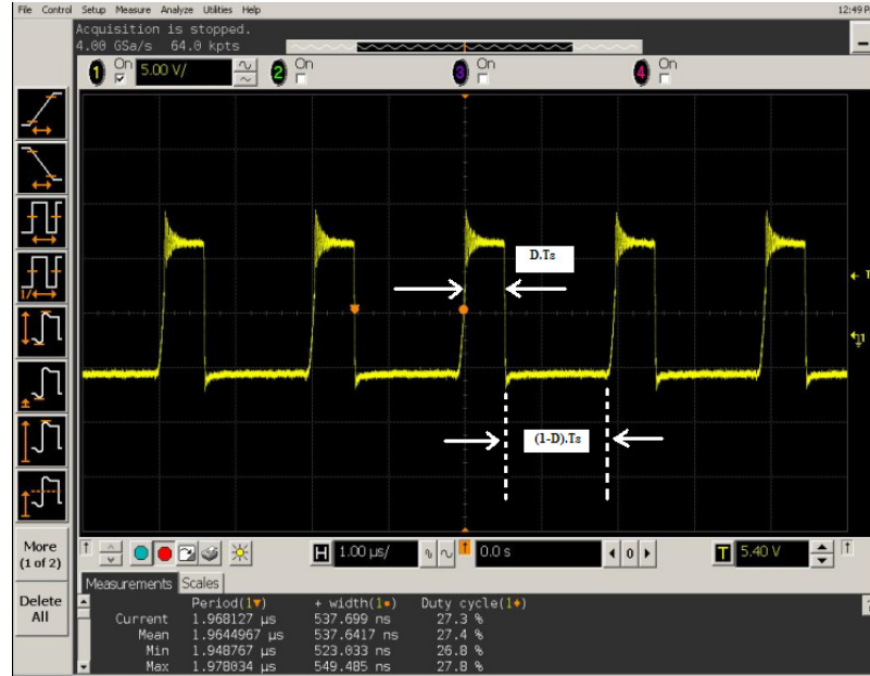
Figure 5.20 Waveform of phase 1 inductor voltage during charging and discharging periods.
