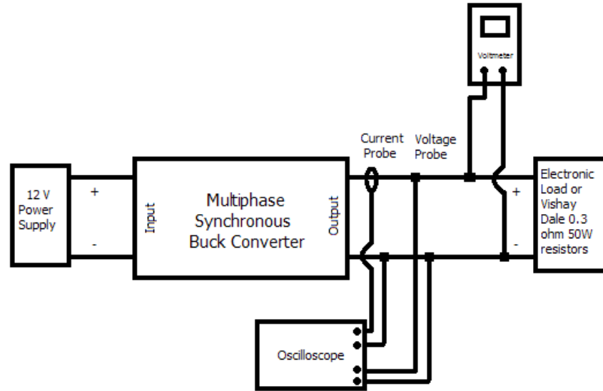
Figure 5.12 Test setup connections.
