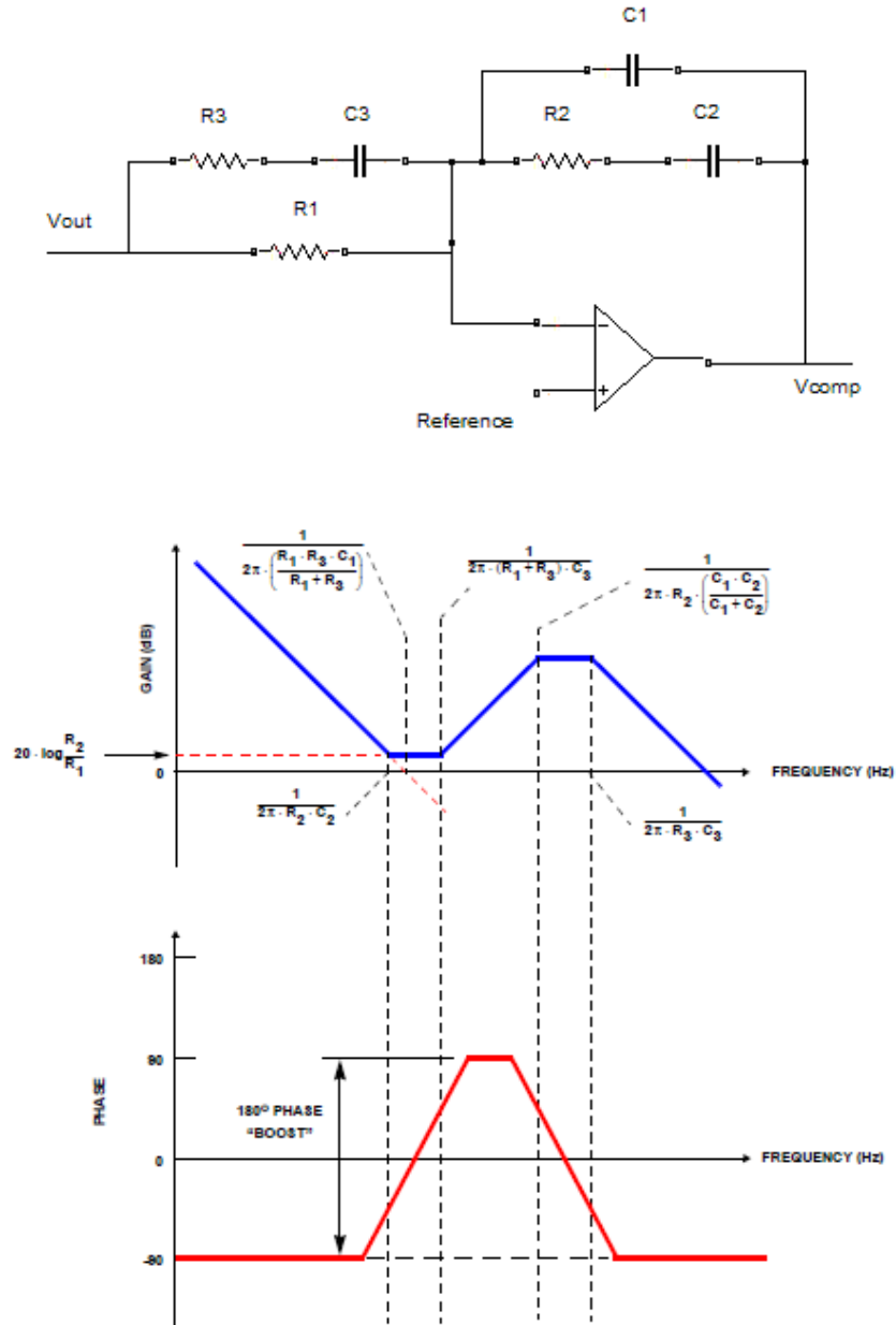
Figure 3.15 Type III compensation network.
