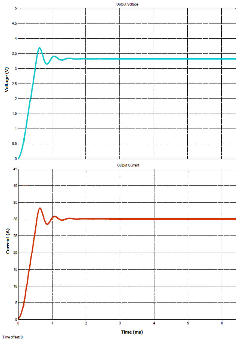
Figure 4.6 Output voltage and output current at full load.
