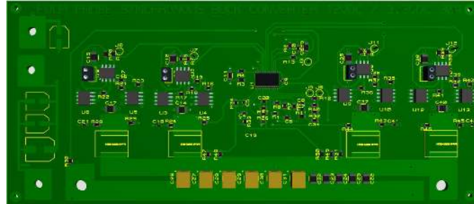
Figure 5.8 3D visualization of the four-phase synchronous buck converter circuit (Protues ARES 7).
