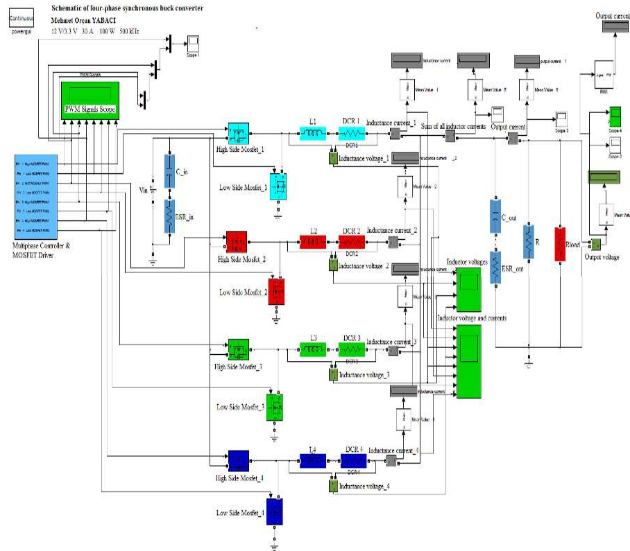
Figure 4.15 Simulation circuit schematic of four-phase synchronous buck converter.
