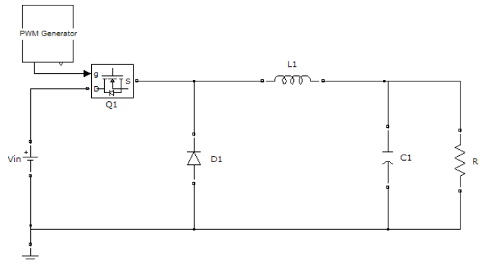
Figure 2.1 Non-synchronous buck converter topology.
