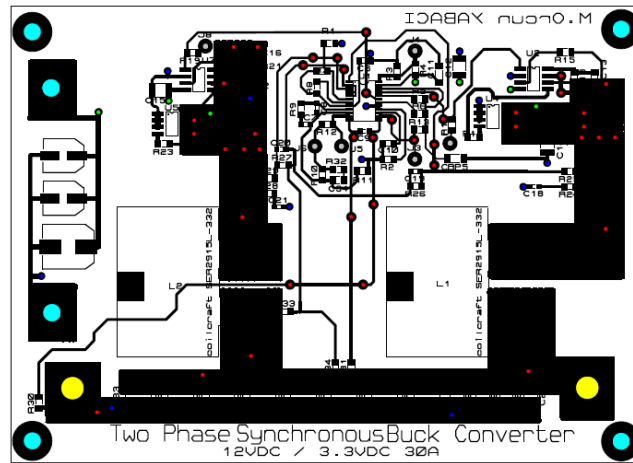
Figure 5.4 Overall layout of the two-phase synchronous buck converter circuit (CAM350 Pro 6).
