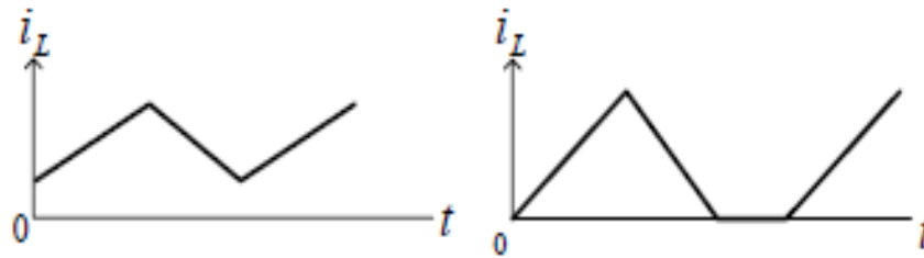
Figure 2.5 (a) Continuous mode. (b) Discontinuous mode.
