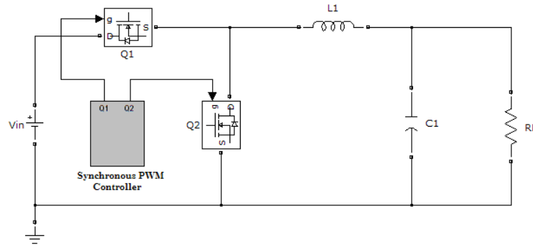
Figure 2.4 Synchronous buck converter topology.
