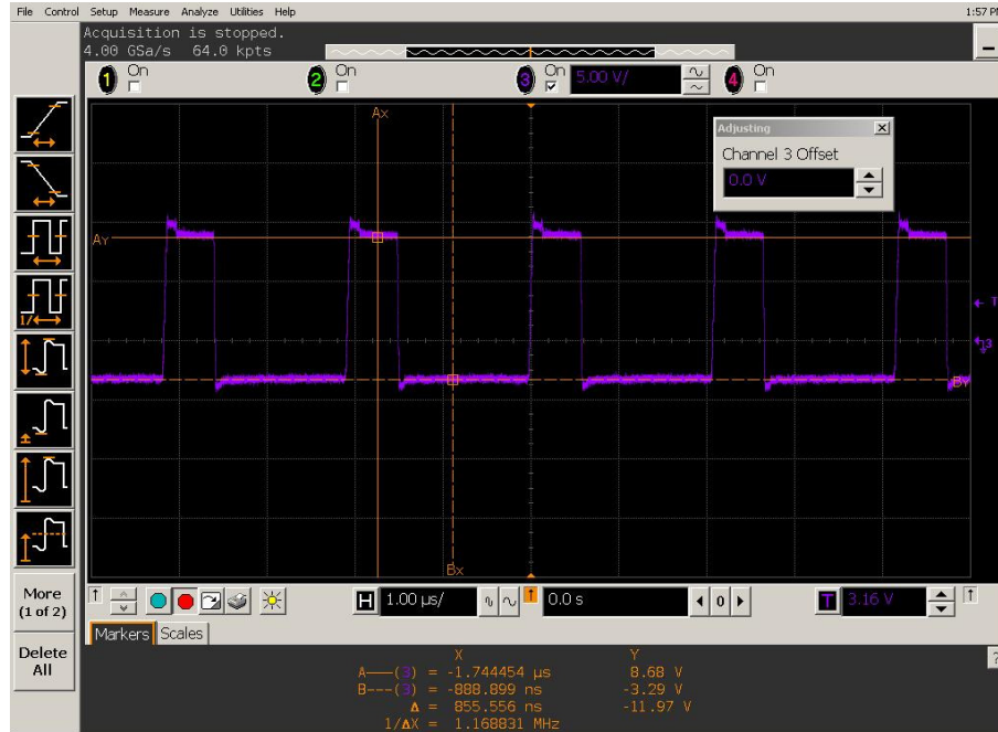
Figure 5.41 Phase 1 inductor voltage waveform.
