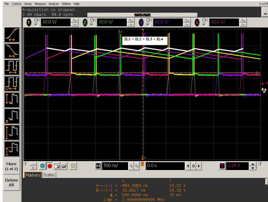
Figure 5.47 Sum of output inductor currents.
