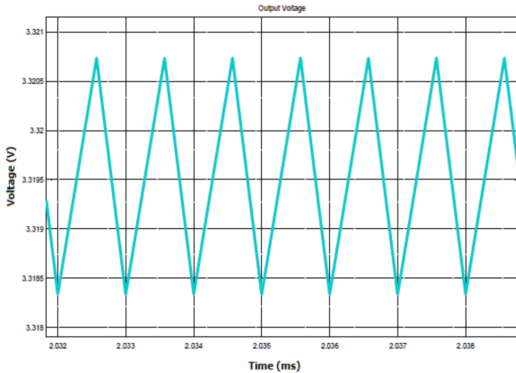
Figure 4.7 Output voltage ripple at full load.
