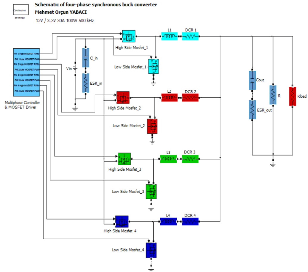
Figure 4.14 Circuit schematic of four-phase synchronous buck converter.
