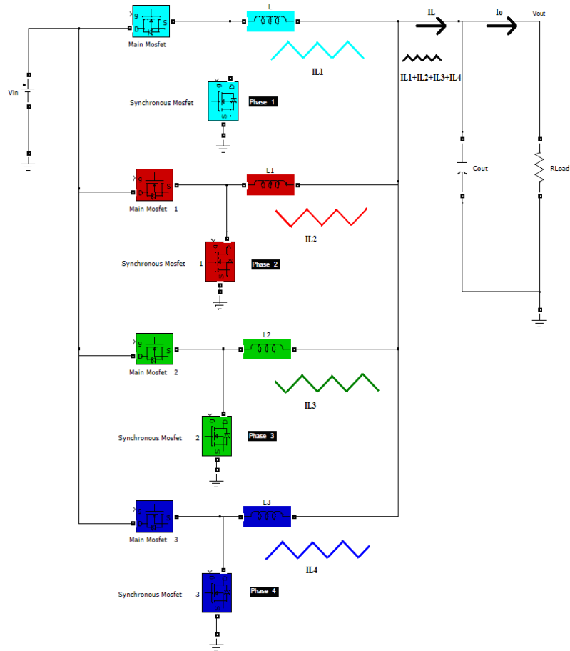
Figure 2.8 Four-phase synchronous buck converter.
