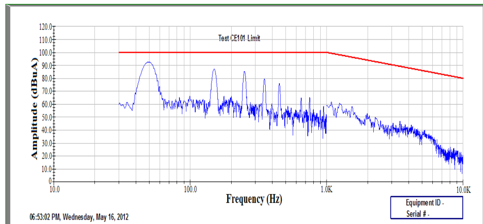
Figure 5.53 CE101 test results for four-phase buck converter (+ power line).
