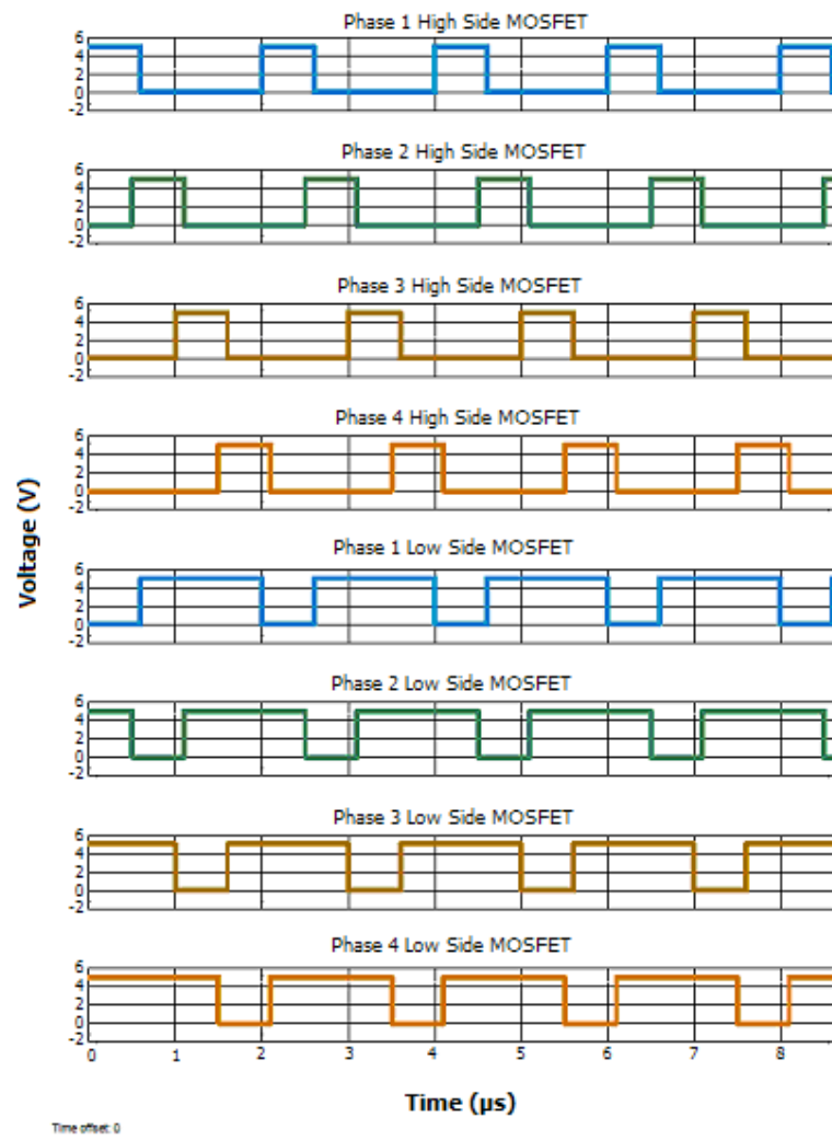
Figure 4.16 PWM signals.
