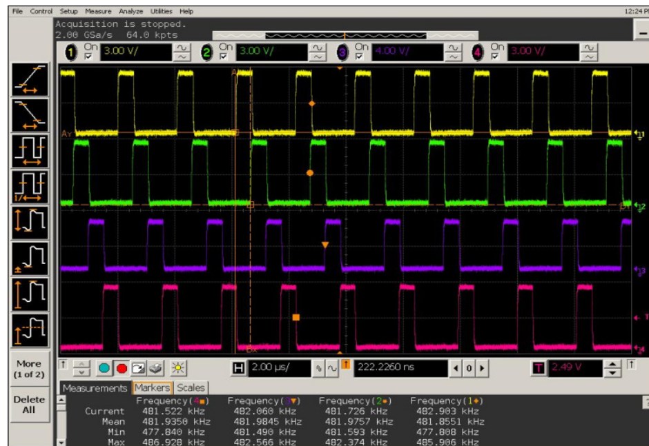
Figure 5.32 PWM signals of four phases generated by TPS40090controller.
