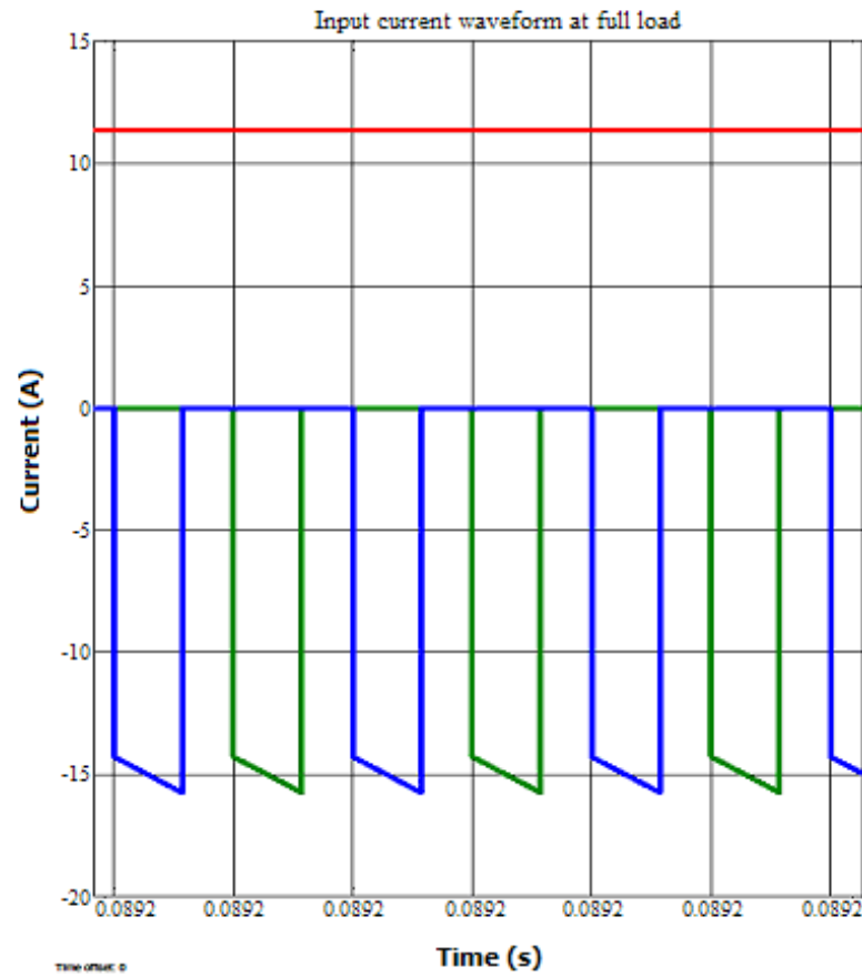
Figure 4.12 Input current waveform at full load.
