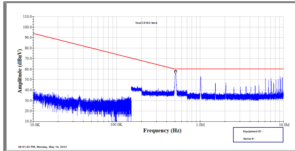
Figure 5.54 CE102 test results for two-phase buck converter (+ power line).
