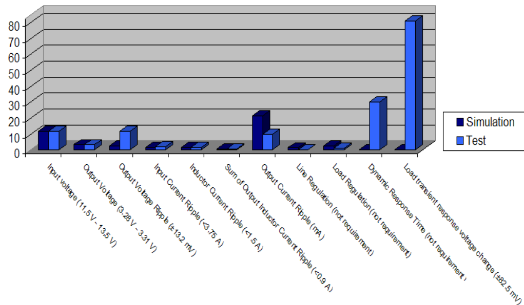
Figure 5.31 Summary of two-phase synchronous buck converter circuit simulation and test results.
