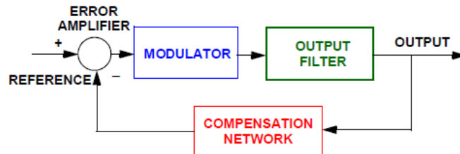
Figure 3.8 Basic block of the buck converter (Mattingly, 2003).
