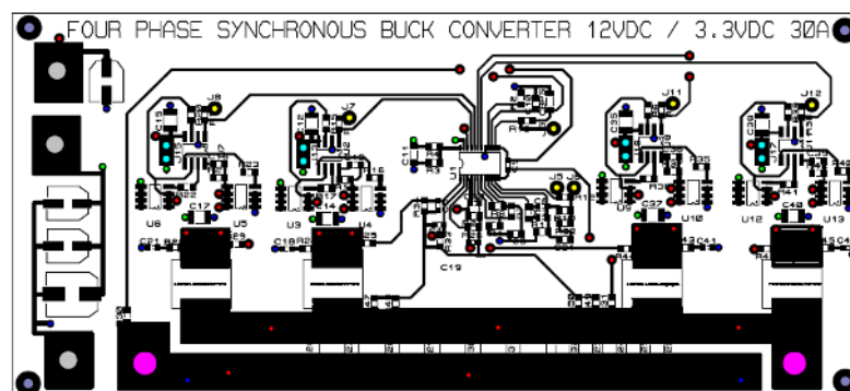
Figure 5.7 Overall layout of the four-phase synchronous buck converter circuit (CAM350 Pro 6).
