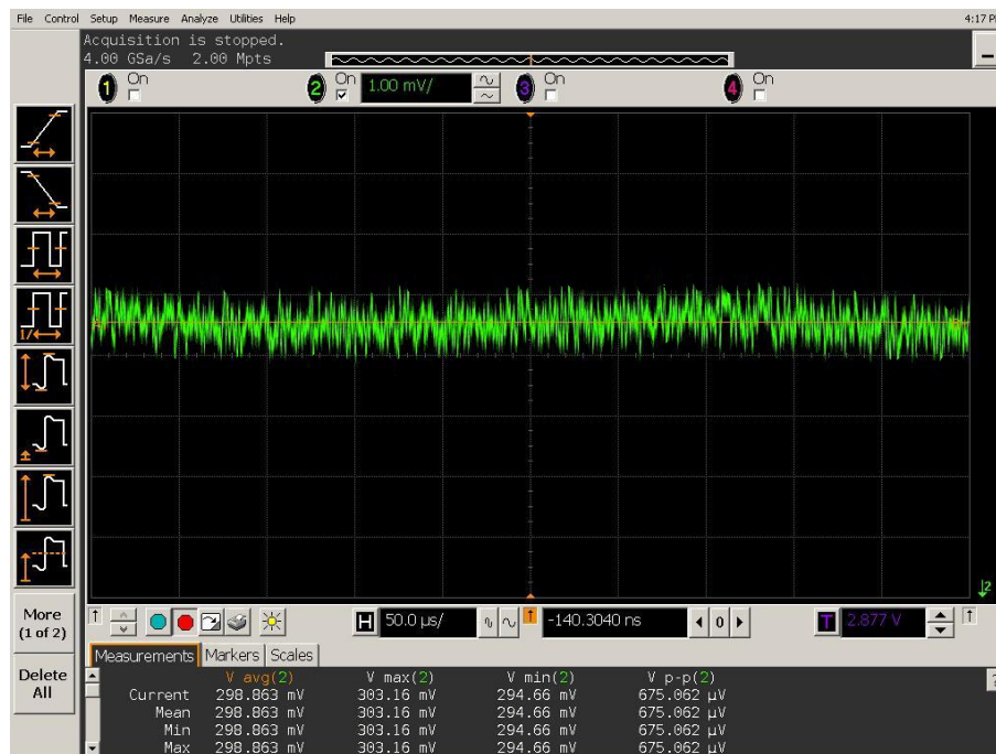
Figure 5.46 Output current waveform at full load (10mV/A).
