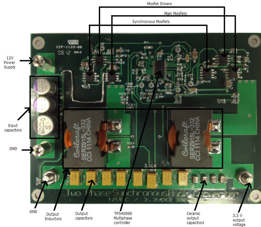
Figure 5.10 General view of the two-phase synchronous buck converter.
