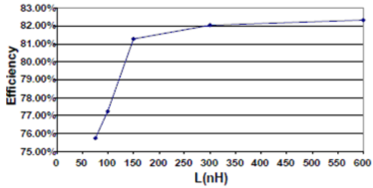
Figure 3.2 Change of efficiency according to phase inductance for multiphase buck converter (Dong, 2009).
