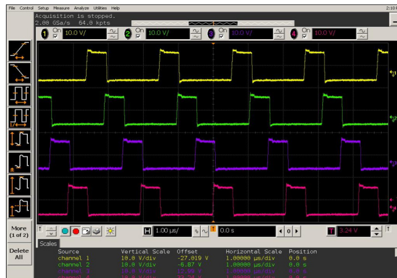
Figure 5.39 Inductor voltage waveforms at full load.
