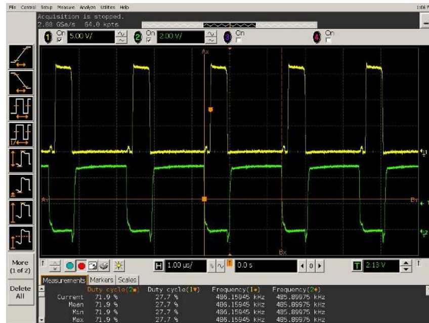
Figure 5.33 High side MOSFET and low side MOSFET PWM signals of first phase.
