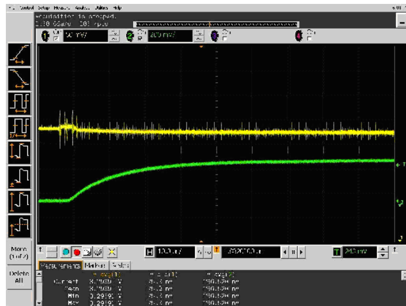
Figure 5.29 Output voltage transient overshoot (0 A to 30 A).
