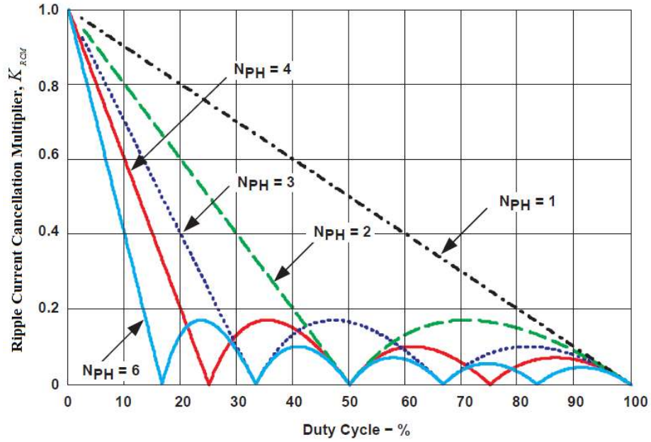
Figure 3.6 Output ripple current cancellation multiplier versus duty cycle.
