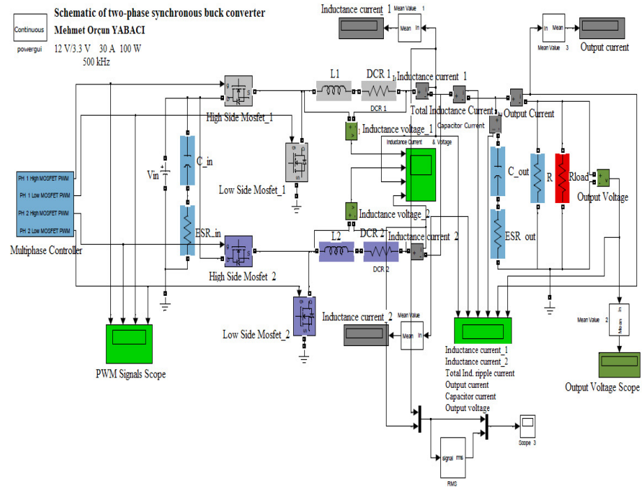
Figure 4.2 Simulation circuit schematic of two-phase synchronous buck converter.
