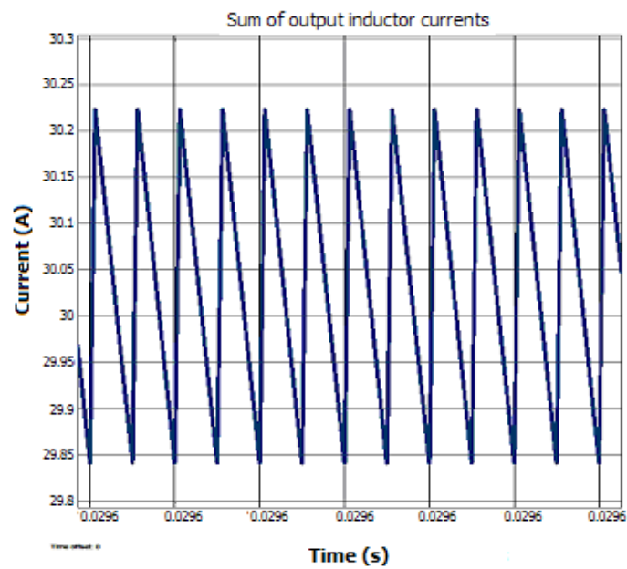
Figure 4.22 Sum of output inductor currents for all four phases at full load.
