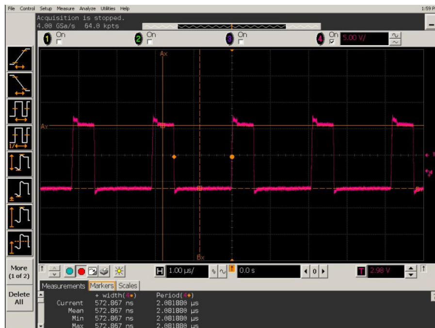
Figure 5.42 Phase 2 inductor voltage waveform.
