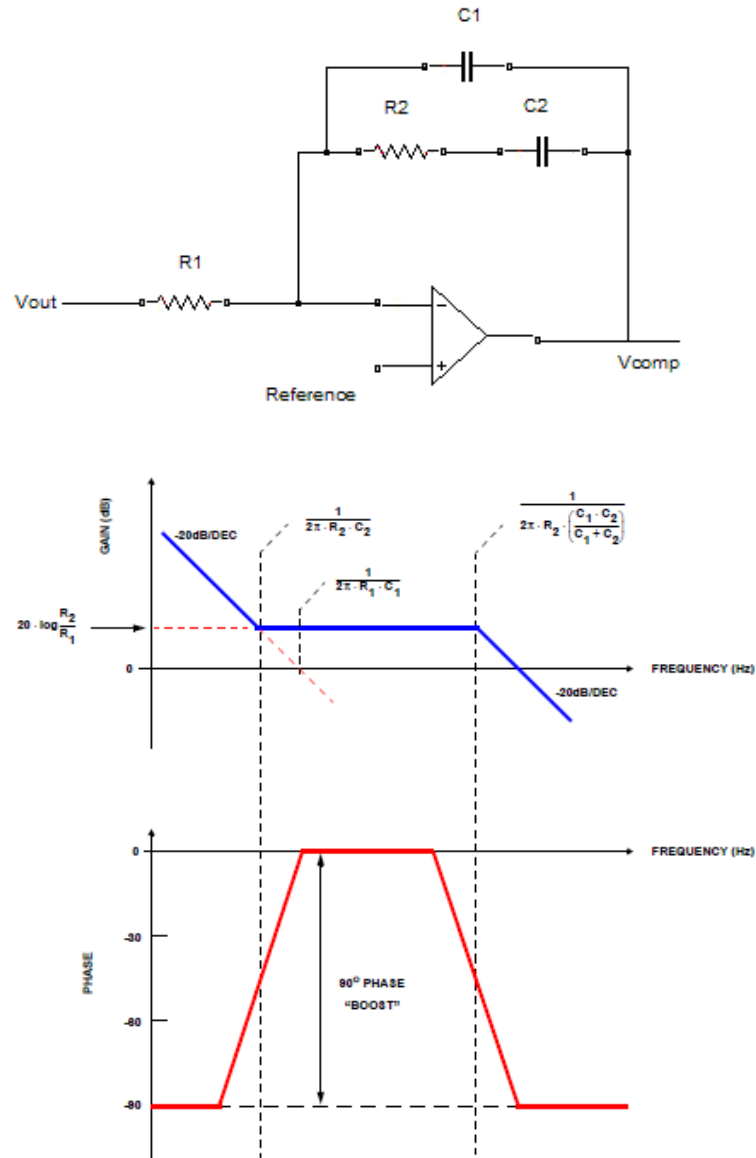
Figure 3.14 Type II compensation network.
