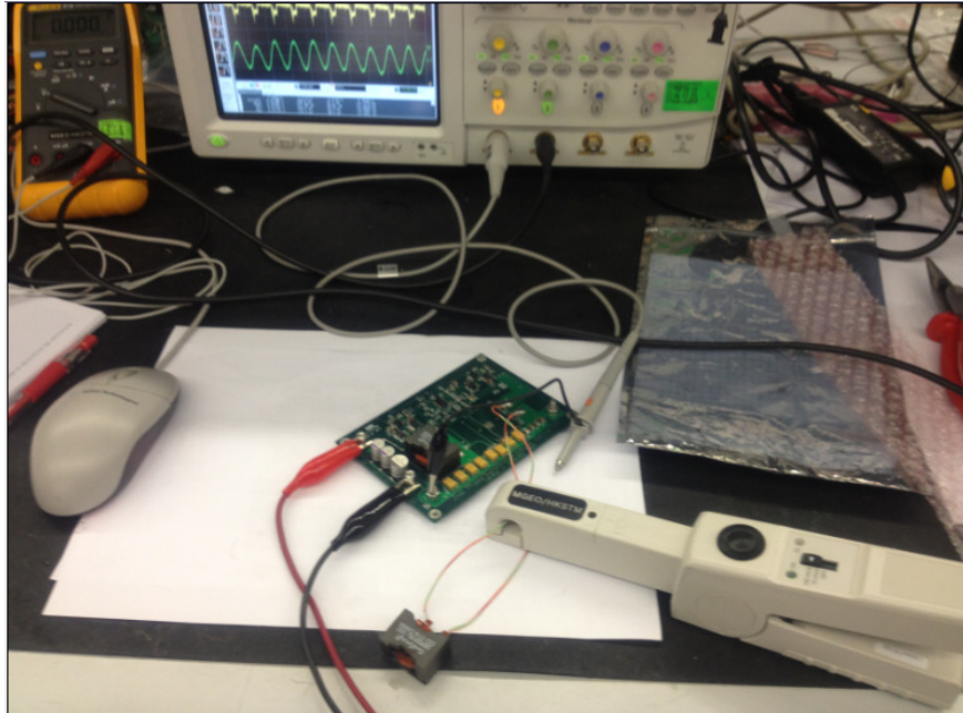
Figure 5.23 Photo of test setup for measurement of inductor current ripples.
