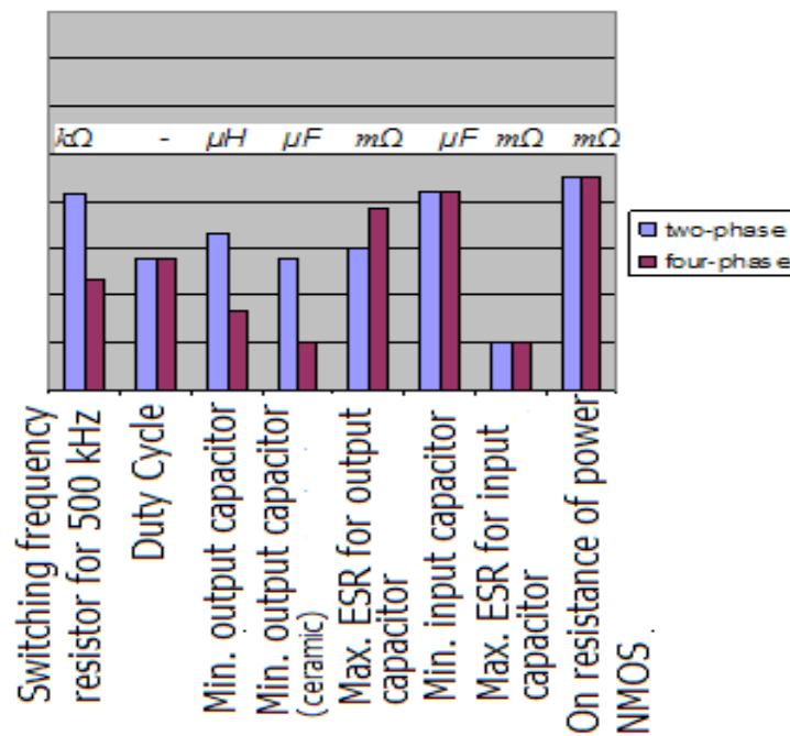
Figure 3.20 Difference between the values of components belonging to two-phase and four-phase synchronous buck converter circuits.
