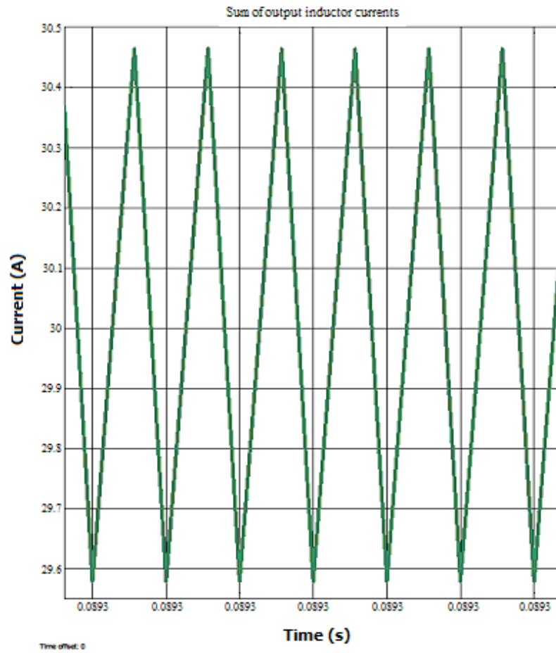
Figure 4.10 Sum of output inductor currents for all two phases at full load.
