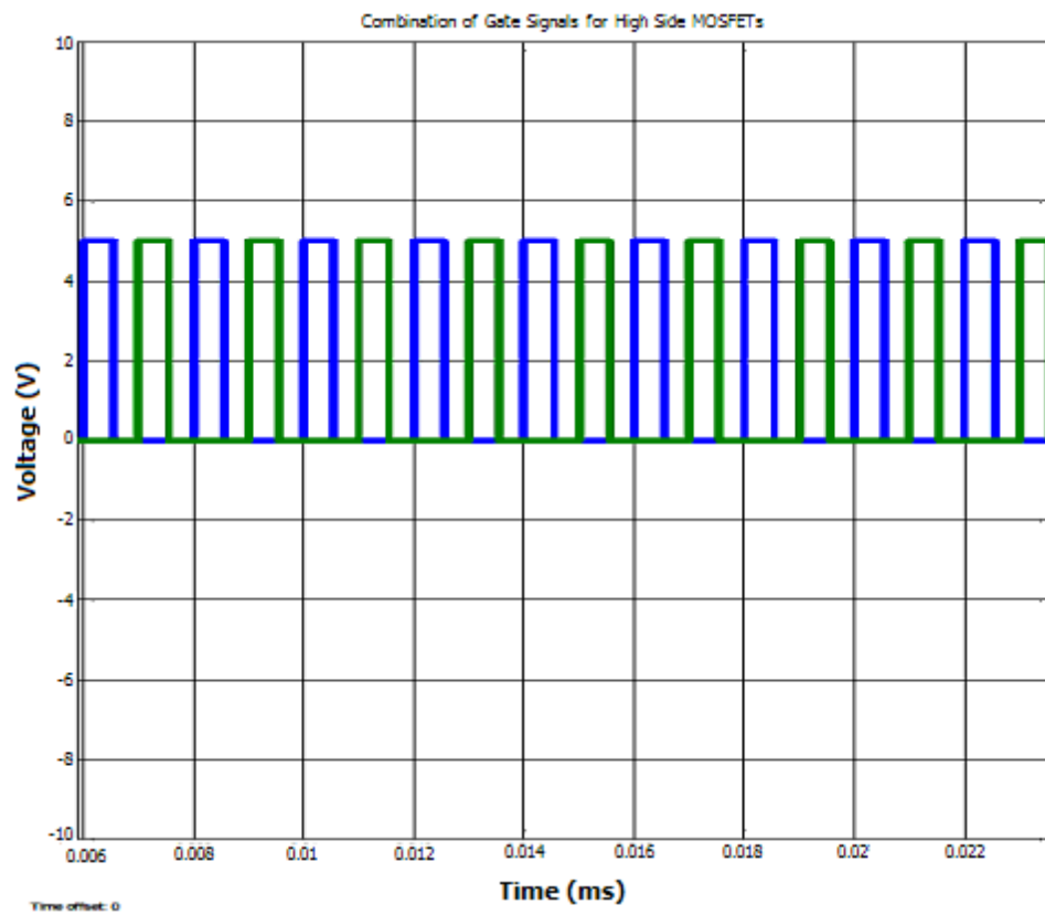
Figure 4.5 Composite of gate signals for high side MOSFETs.
