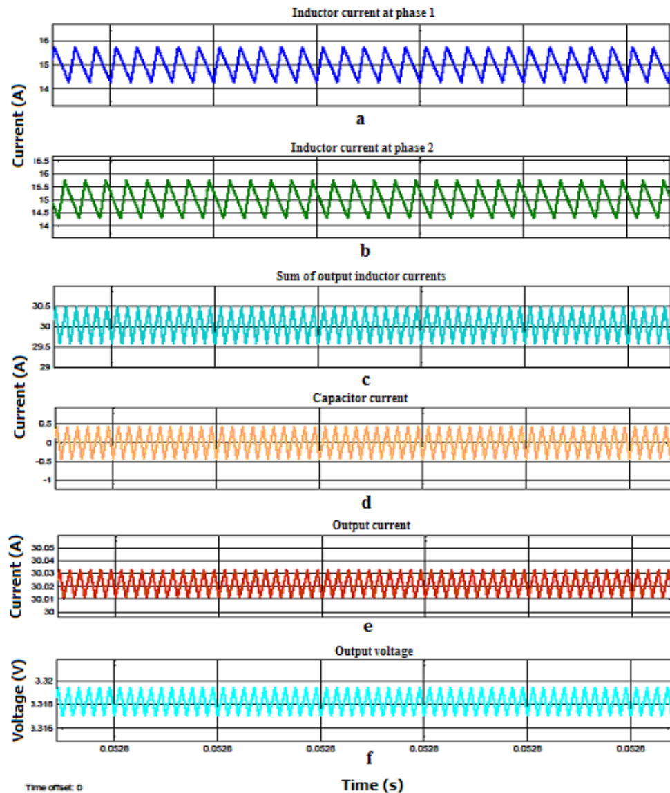
Figure 4.13 All important signals at full load (a: inductor current at phase 1, b: inductor current at phase 2, c: sum of output inductor currents, d: capacitor current, e: output current, f: output voltage).
