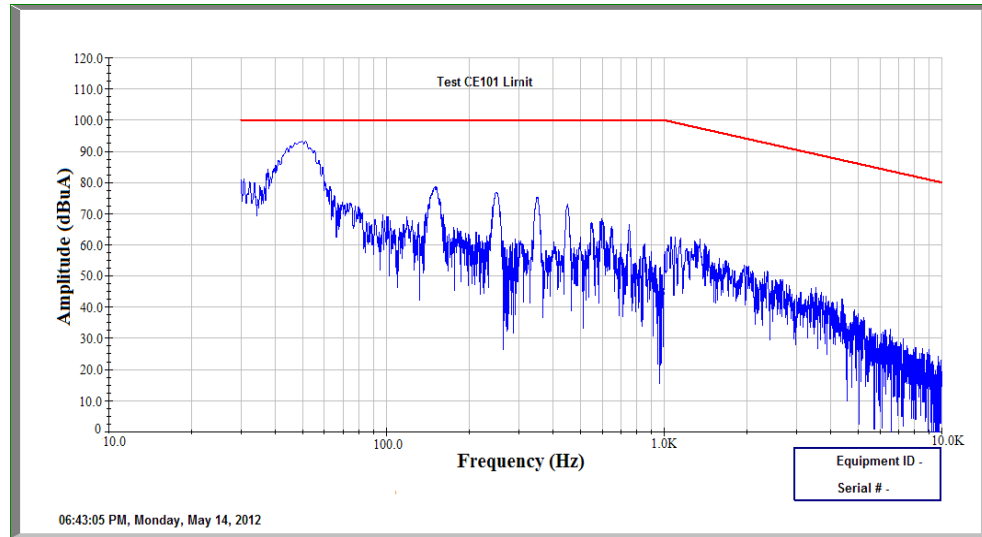
Figure 5.52 CE101 test results for two-phase buck converter (+ power line).
