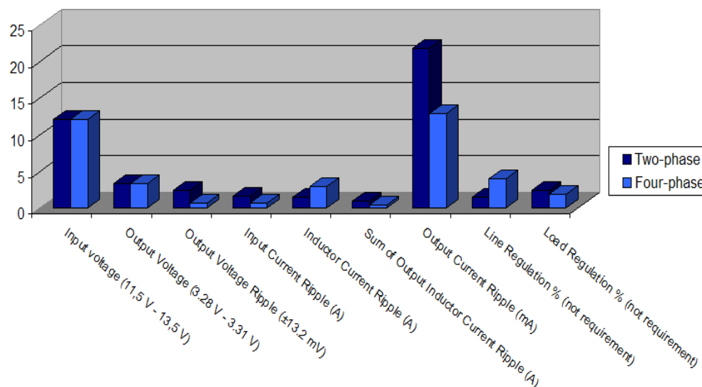
Figure 4.26 Comparison of simulation results between two-phase and four-phase synchronous buck converter.
