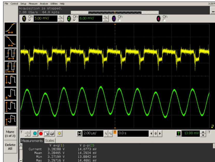
Figure 5.25 Inductor current ripple waveform for phase 2.
