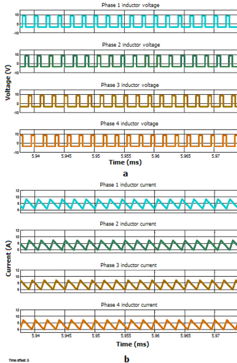
Figure 4.20 Inductor voltages and inductor ripple currents for each phase (a: inductor voltages for each phase, b: inductor currents for each phase).
