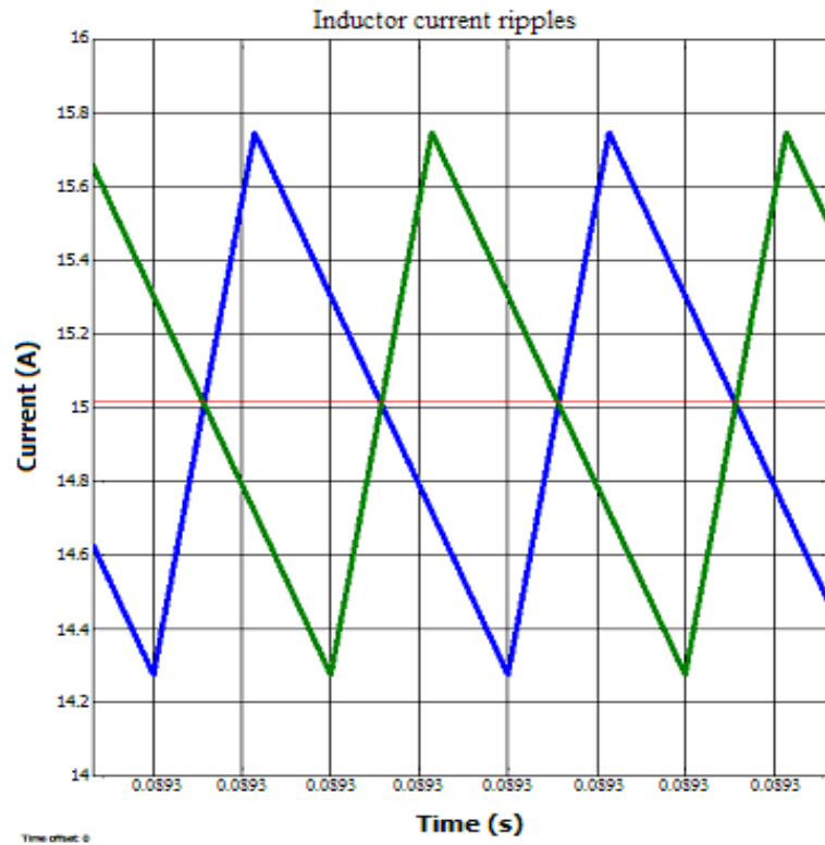
Figure 4.9 Inductor current ripple waveforms at each channel at full load.
