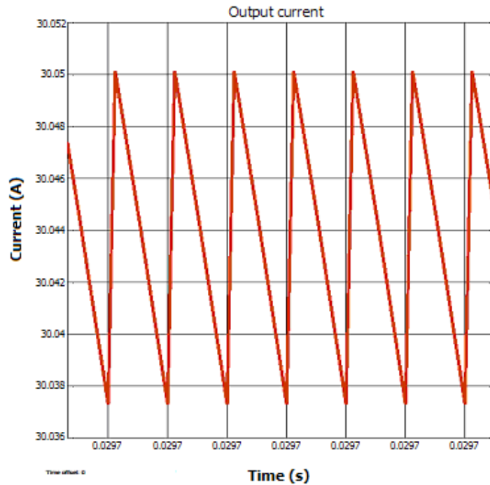
Figure 4.23 Output current at full load.
