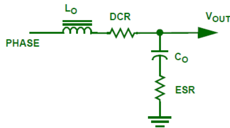
Figure 3.10 The output filter (Mattingly, 2003).
