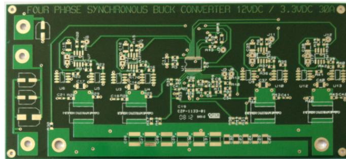
Figure 5.8 3D visualization of the four-phase synchronous buck converter circuit (Protues ARES 7).
