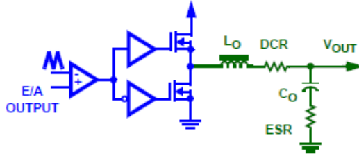
Figure 3.11 The open loop system (Mattingly, 2003).
