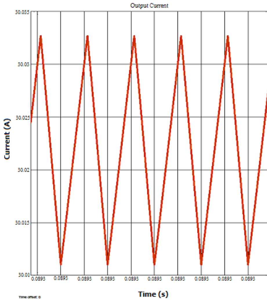
Figure 4.11 Output current at full load.
