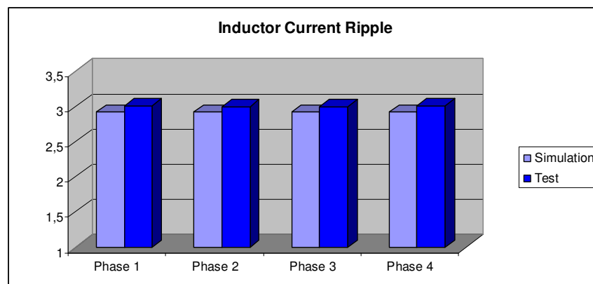
Figure 5.45 Summary of inductor current ripple values.
