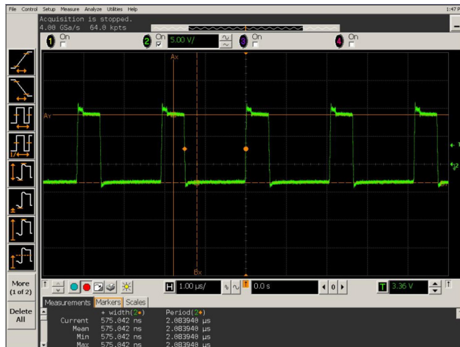
Figure 5.44 Phase 4 inductor voltage waveform.
