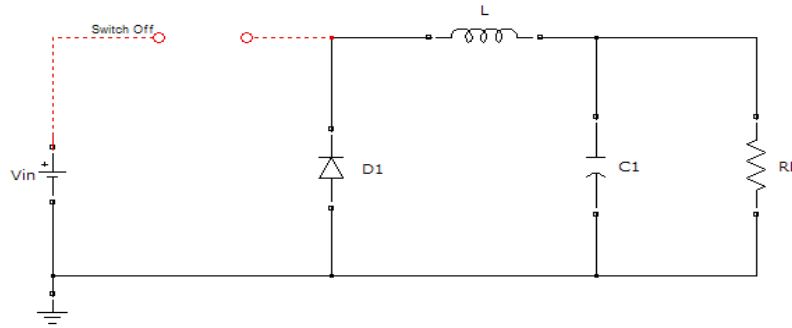
Figure 2.3 Non-synchronous buck converter, when the switch is OFF.
