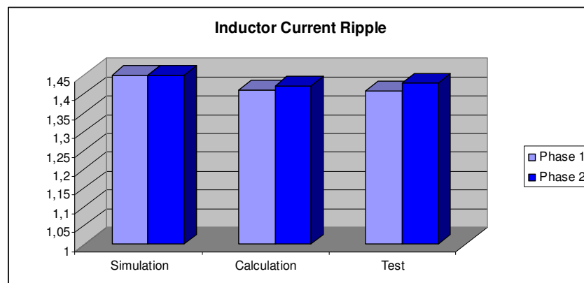
Figure 5.26 Summary of inductor current ripple values.
