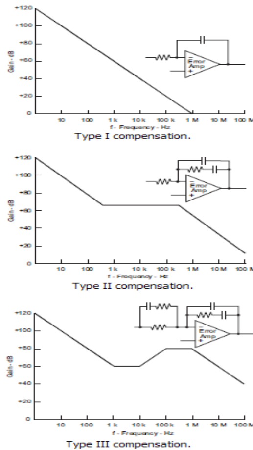
Figure 3.13 Power supply compensation schemes (Day, 2004).
