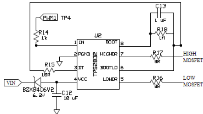
Figure 5.2 Schematic of the gate driver circuit TPS2832.
