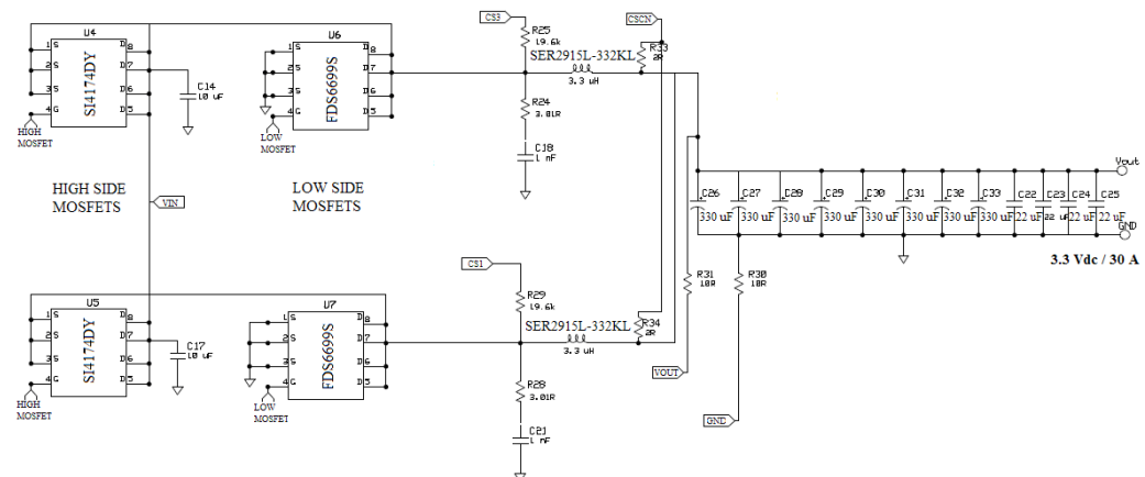
Figure 5.3 Schematic of the power circuit (two-phase).
