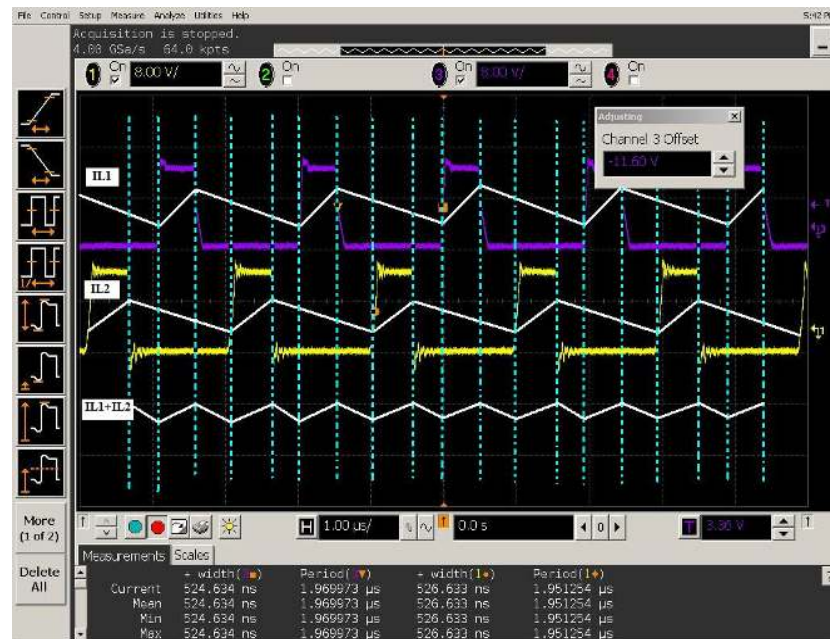
Figure 5.28 Sum of output inductor currents.
