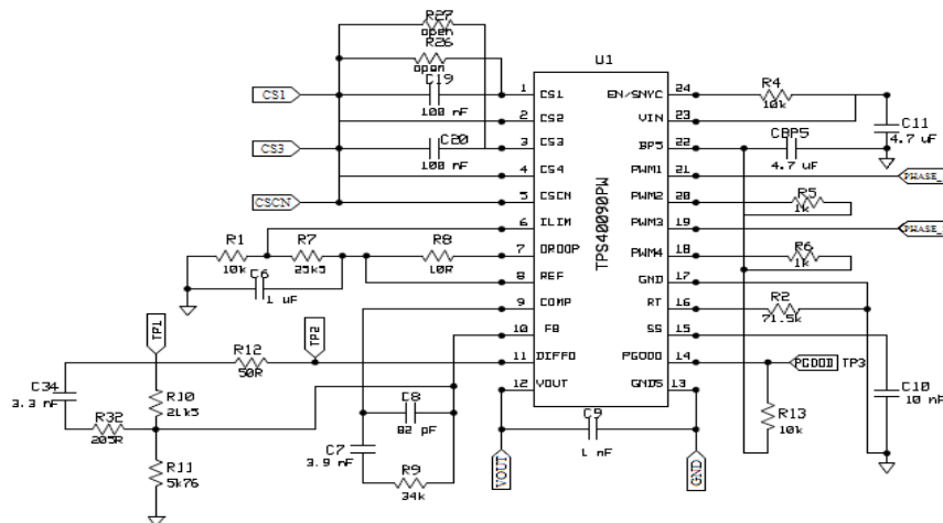
Figure 5.1 Schematic of the multiphase controller TPS40090.
