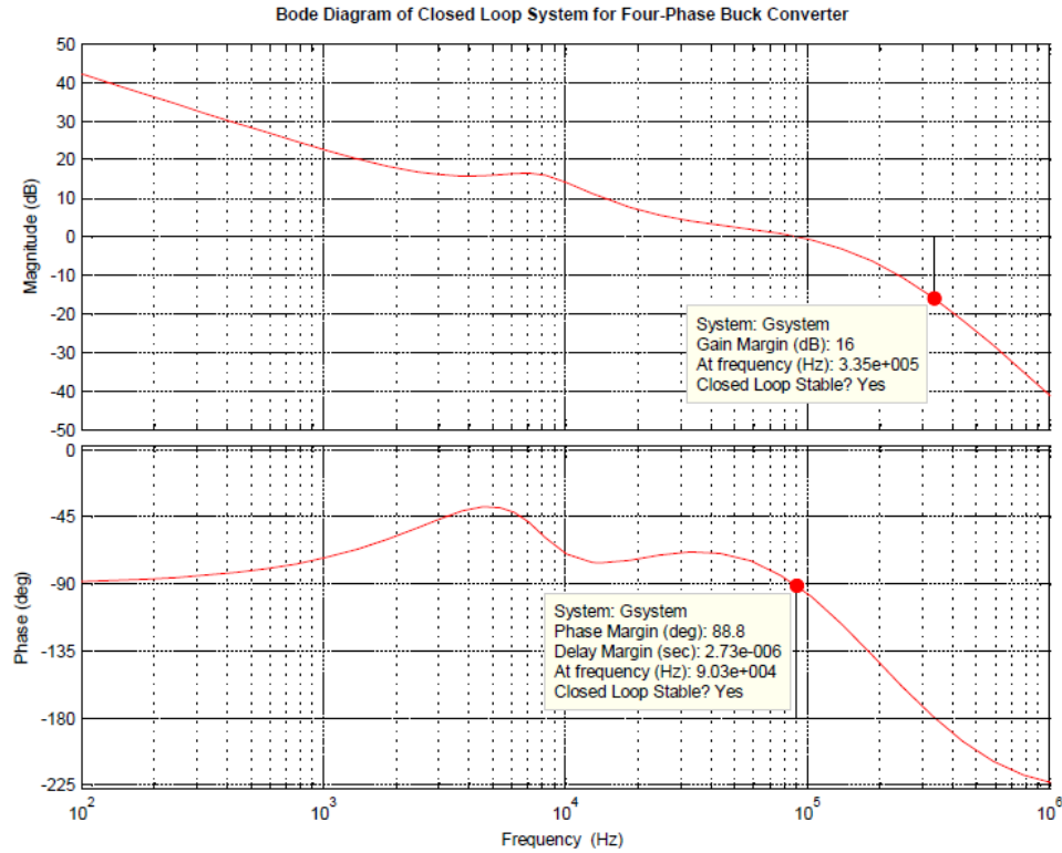
Figure 3.19 Bode diagram of closed-loop system for four-phase buck converter.
