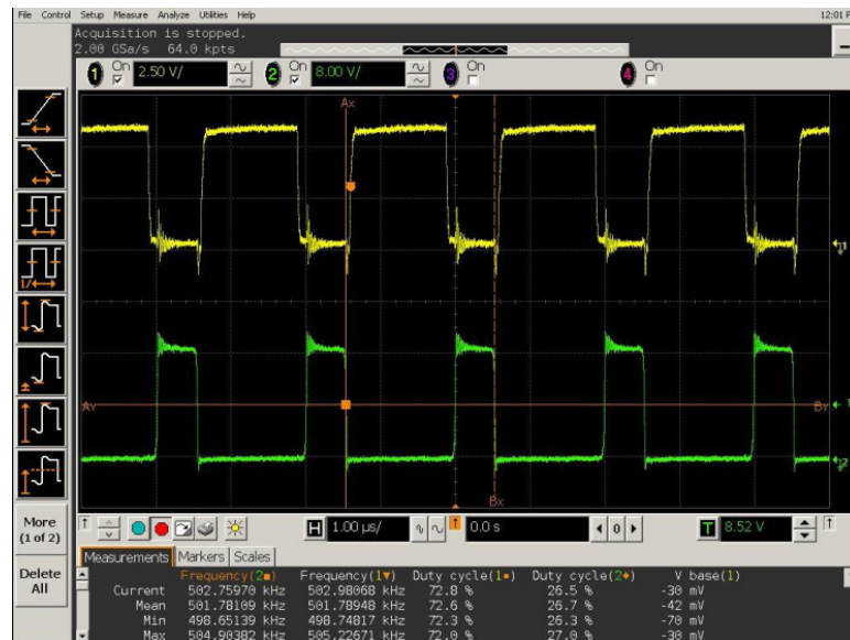
Figure 5.17 High side and low side MOSFETs PWM signals of second phase.
