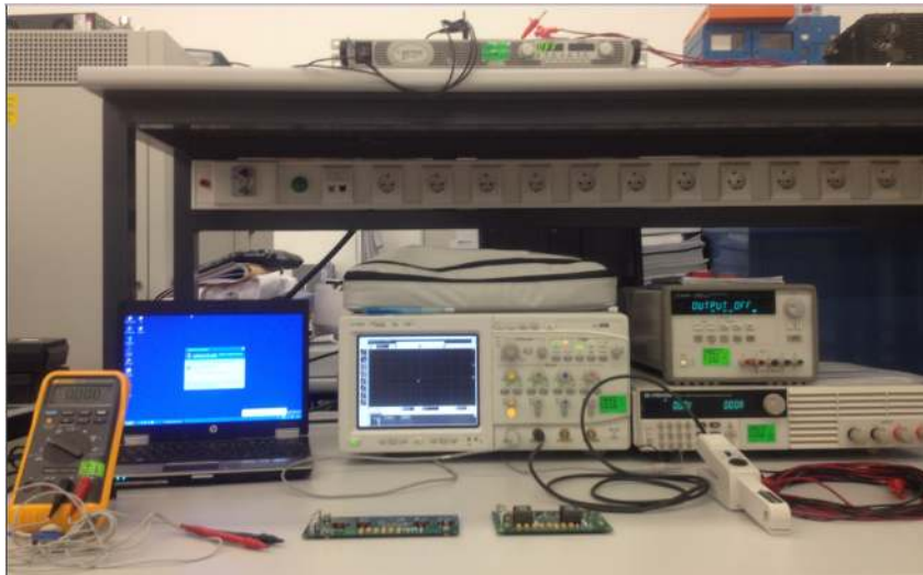
Figure 5.13 Photo of test setup.
