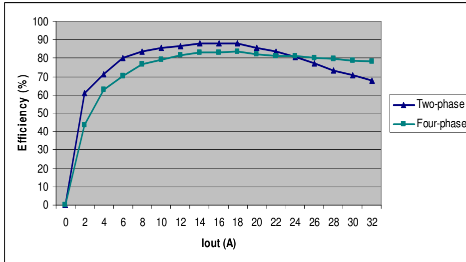
Figure 5.51 Efficiency comparison of between two-phase and four-phase synchronous buck converters.
