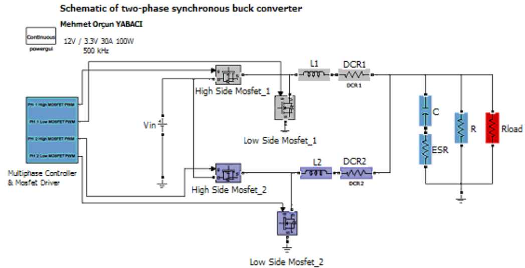
Figure 4.1 Circuit schematic of two-phase synchronous buck converter.
