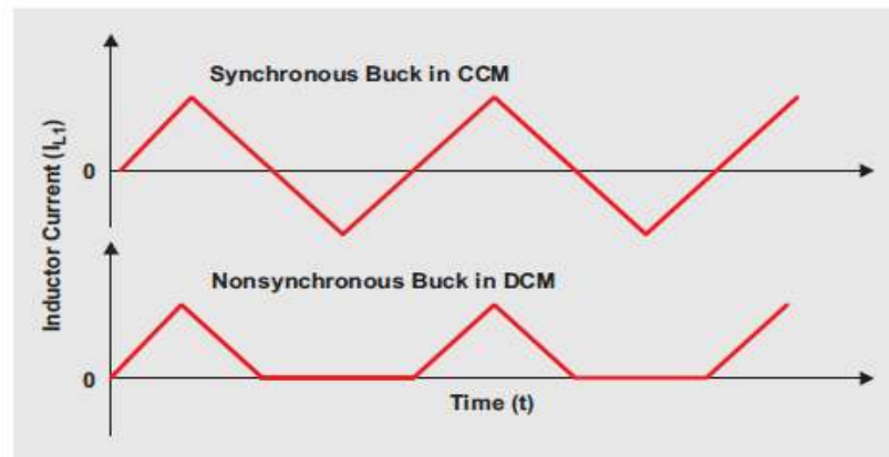
Figure 2.6 Synchronous and non-synchronous buck converter inductor current modes (Nowakowski & Tang, 2009).
