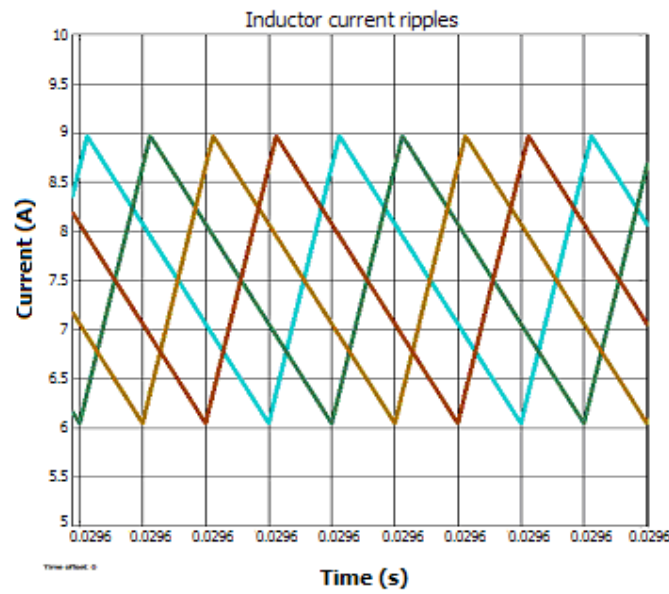
Figure 4.21 Inductor current ripple waveforms at each channel at full load.
