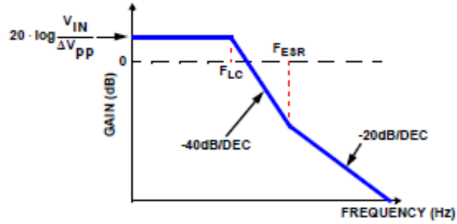
Figure 3.12 The open loop system gain (Mattingly, 2003).
