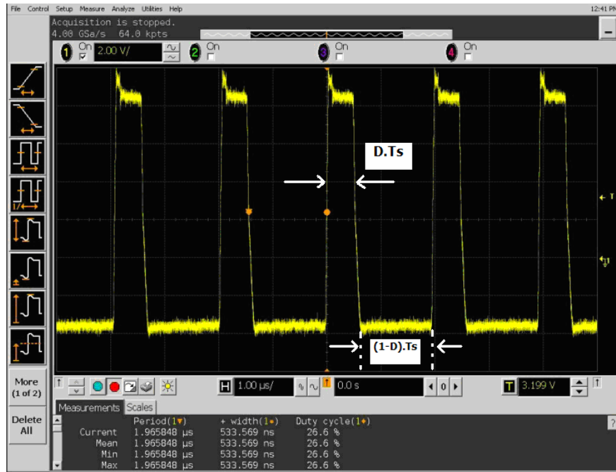
Figure 5.22 Waveform of phase 2 inductor voltage during charging and discharging time.
