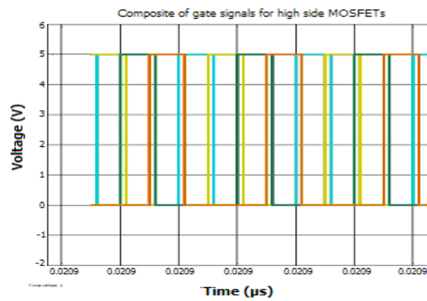
Figure 4.17 Composite of gate signals for high side MOSFETs.
