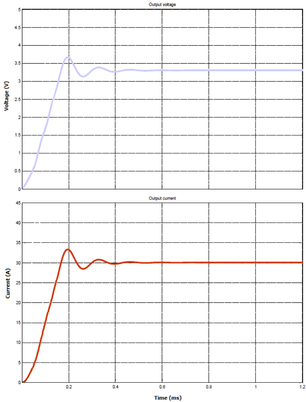
Figure 4.18 Output voltage and output current at full load.
