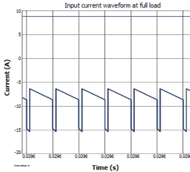
Figure 4.25 Input capacitor current waveform at full load.
