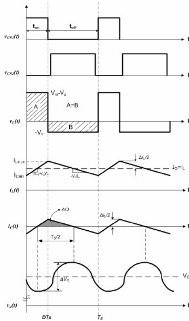
Figure 3.1 The main waveforms of the voltages and currents for a synchronous buck converter (Erdoğan, 2010).
