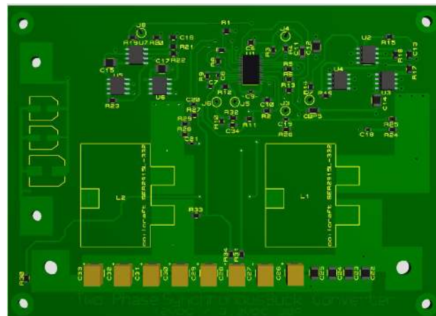
Figure 5.5 3D visualization of the two-phase synchronous buck converter circuit (Protues ARES 7).
