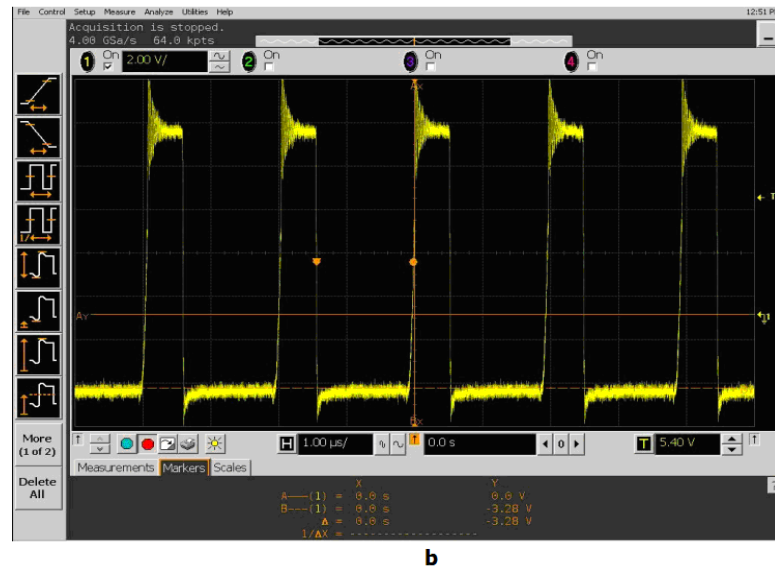
Figure 5.21 Waveform of phase 1 inductor voltage (a: Inductor current rises, b: Inductor current decreases).
