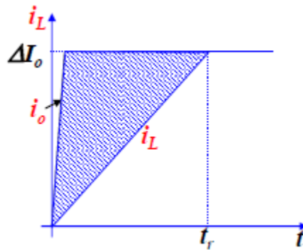
Figure 3.3 The ratio of Multiphase buck converter's inductor and output current slew rates at transient response (Dong, 2009).
