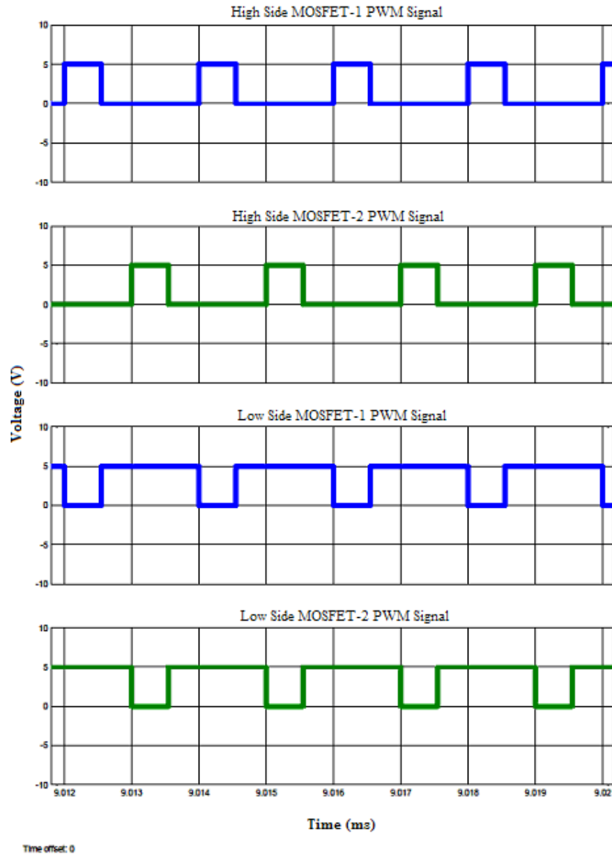
Figure 4.4 PWM signals.
