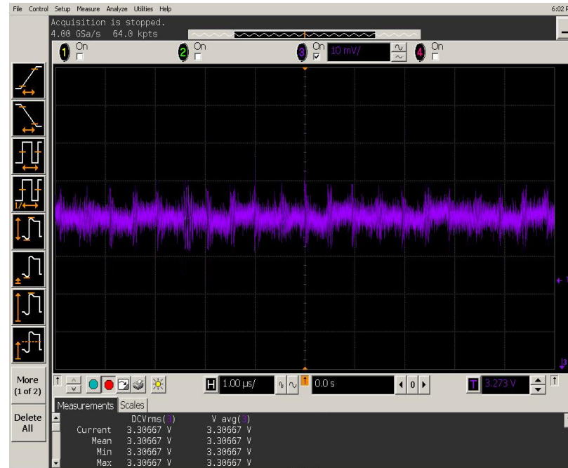
Figure 5.18 Output voltage waveform.
