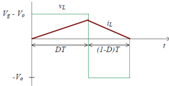
Figure 2.7 CCM/DCM boundary condition.
