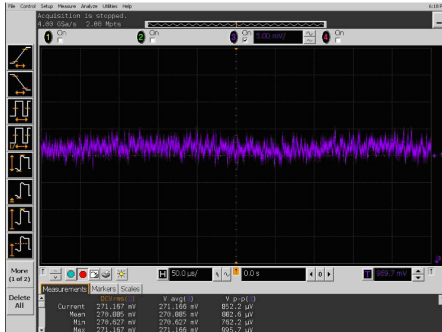
Figure 5.27 Output current waveform at full load.
