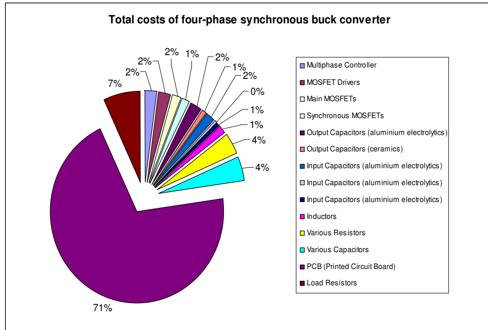
Figure 5.57 Total costs of four-phase synchronous buck converter.
