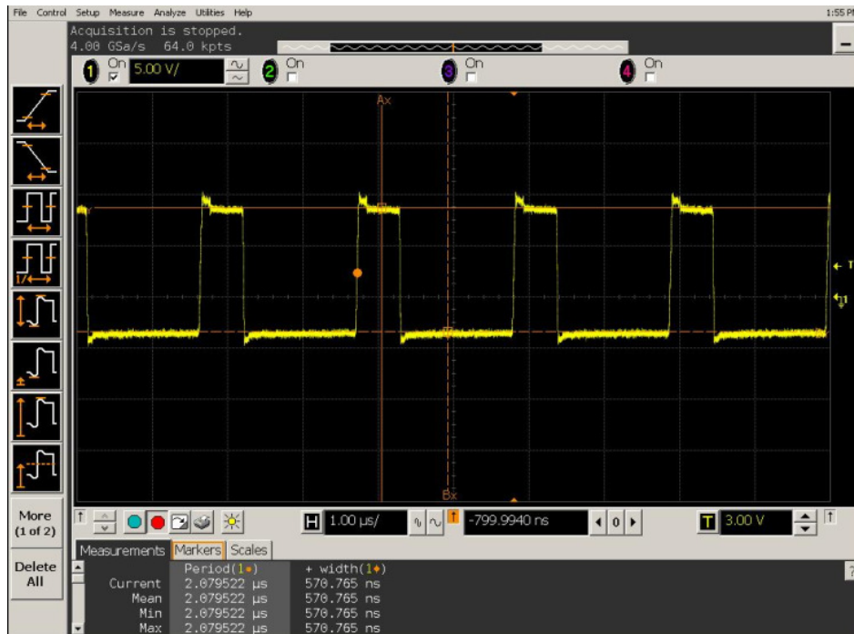
Figure 5.43 Phase 3 inductor voltage waveform.
