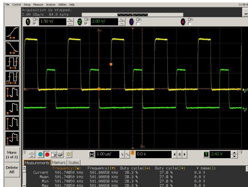
Figure 5.15 PWM signals of TPS40090PW controller IC.
