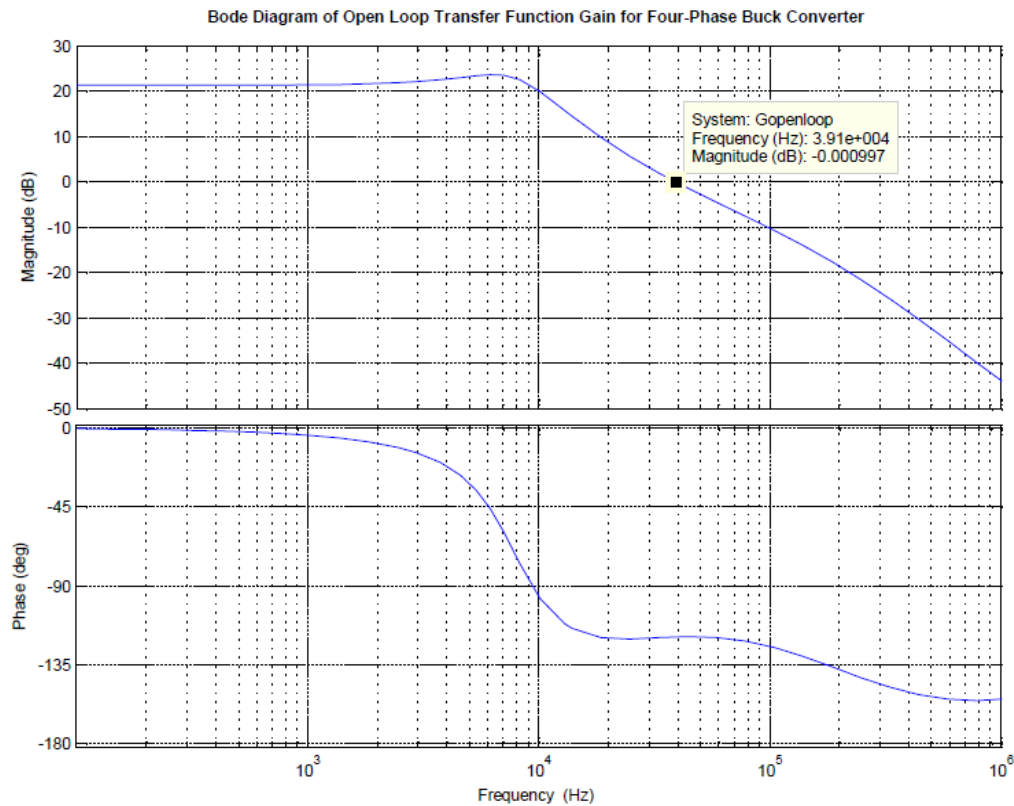
Figure 3.18 Bode diagram of open-loop transfer function gain for four-phase buck converter.
