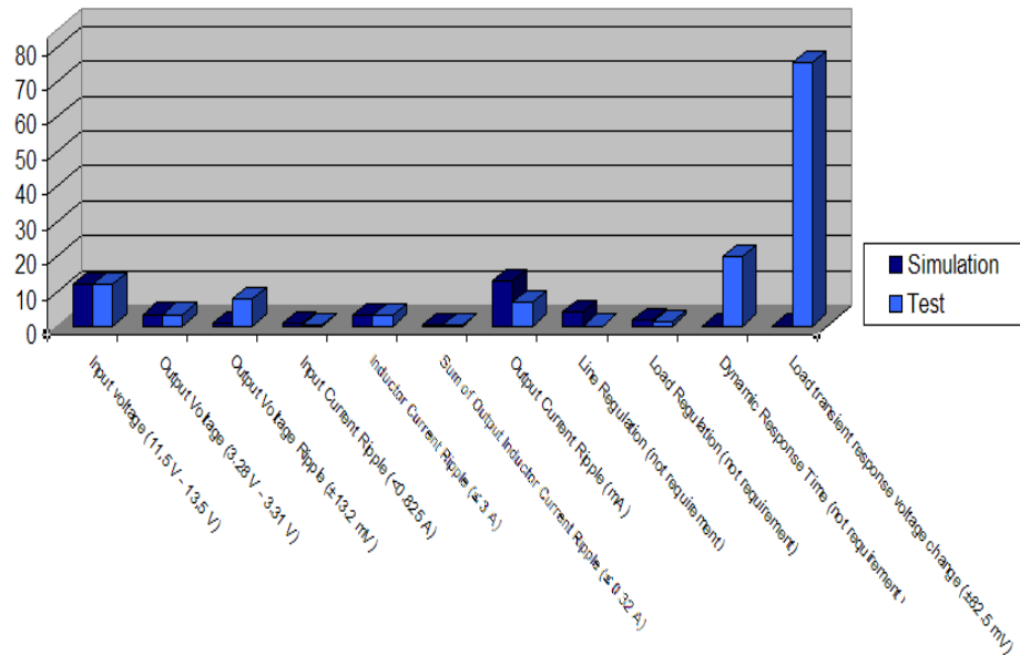
Figure 5.50 Summary of four-phase synchronous buck converter circuit simulation and test results.
