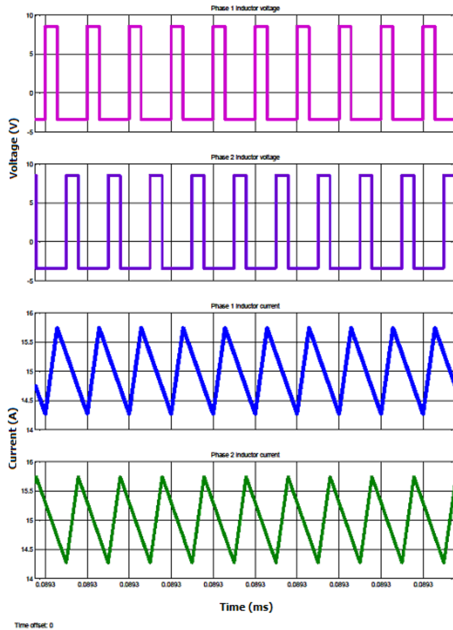
Figure 4.8 Inductor voltages and inductor ripple currents at both two phases.
