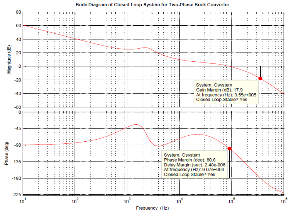
Figure 3.17 Bode diagram of closed-loop system for two-phase buck converter.
