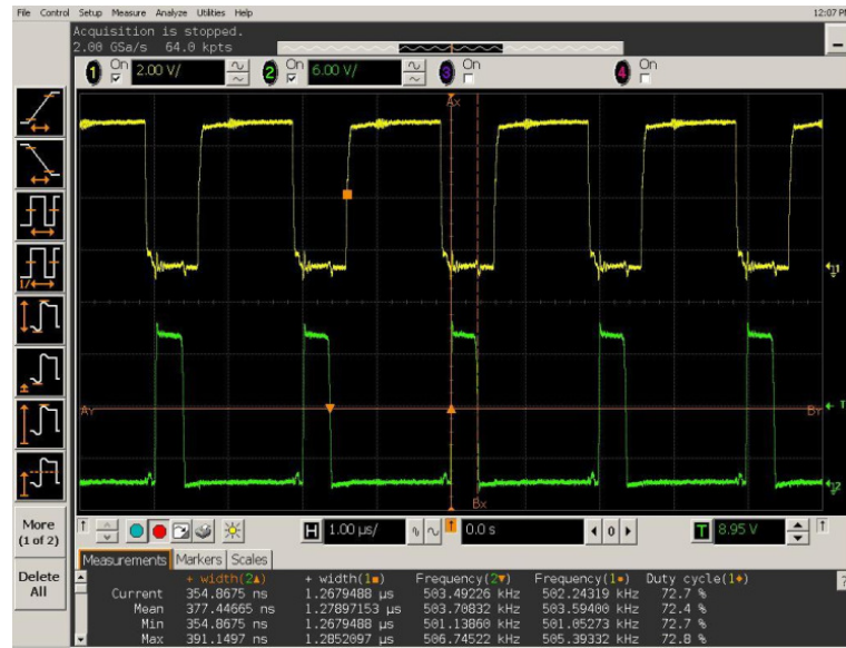
Figure 5.16 High side and low side MOSFETs PWM signals of first phase.
