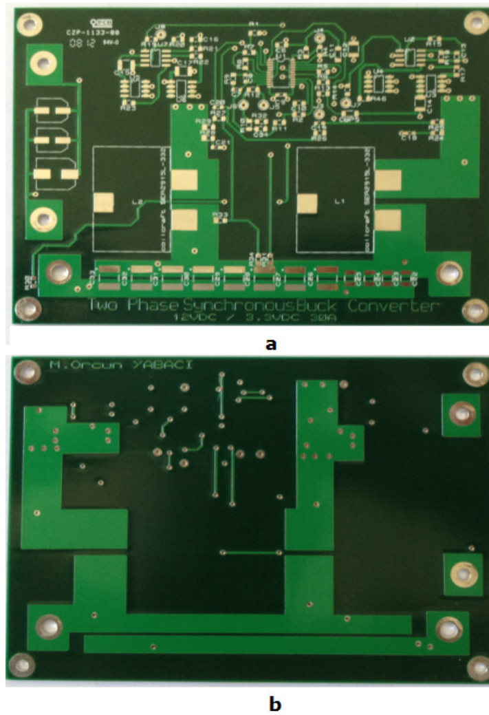
Figure 5.6 Photos of the designed two-phase buck converter PCB (a: component side, b: solder side)
