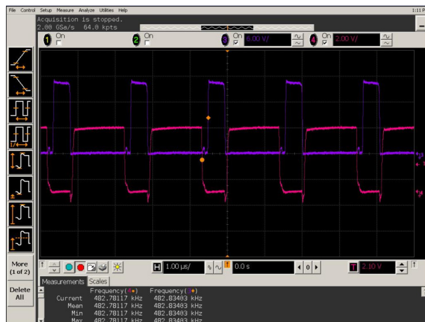
Figure 5.34 High side MOSFET and low side MOSFET PWM signals of second phase.
