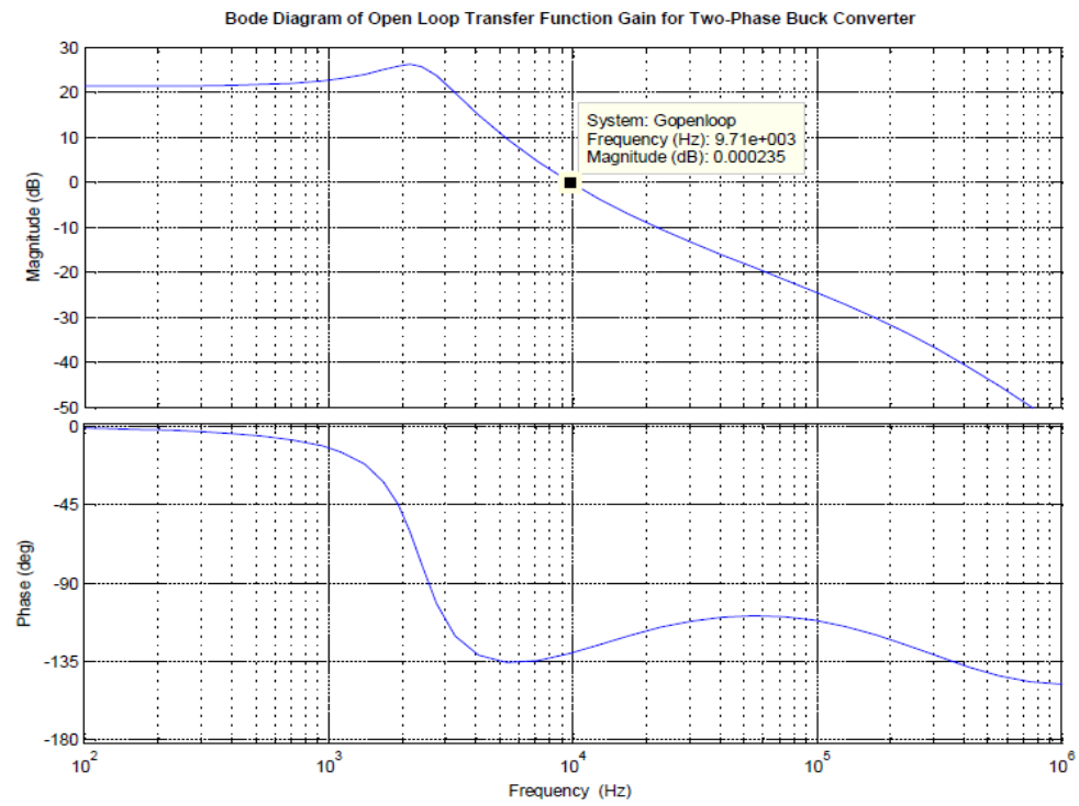
Figure 3.16 Bode diagram of open-loop transfer function gain for two-phase buck converter.
