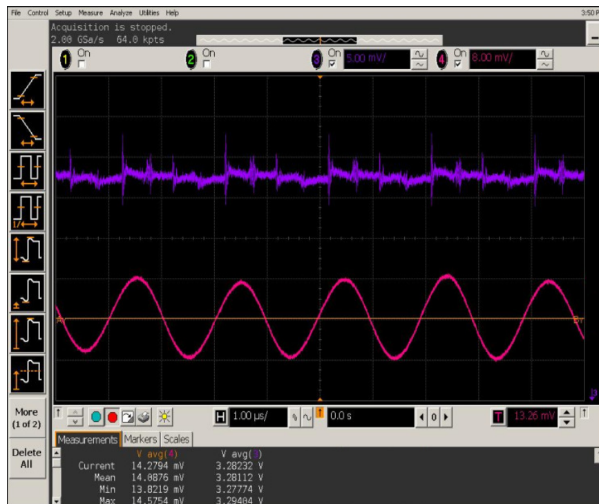
Figure 5.24 Inductor current ripple waveform for phase 1.
