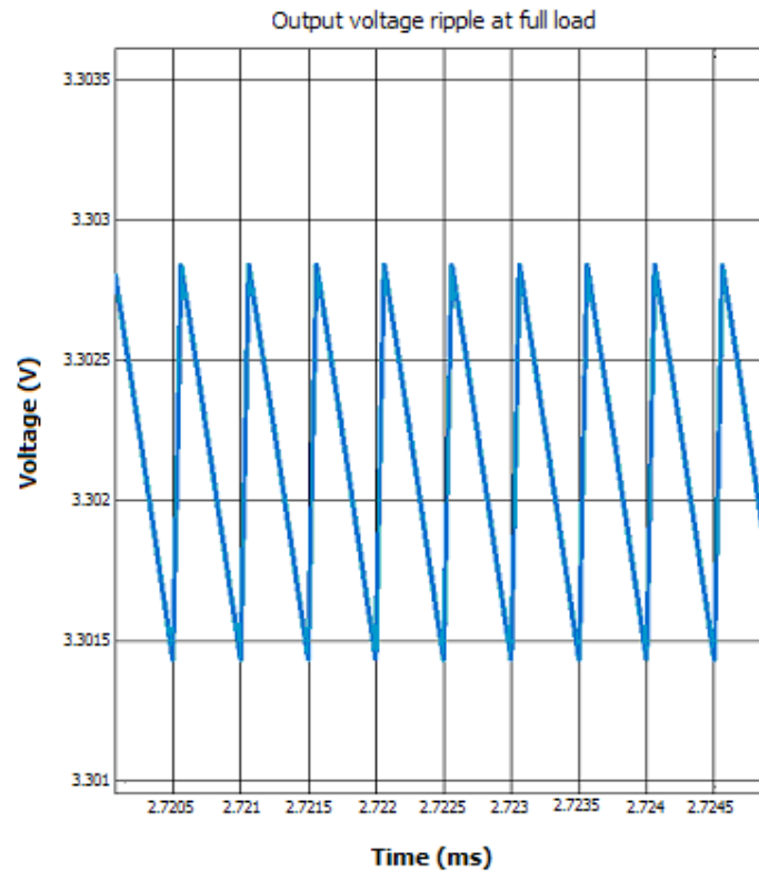
Figure 4.19 Output voltage ripple at full load.
