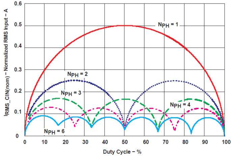
Figure 3.7 Input ripple RMS current versus duty cycle.
