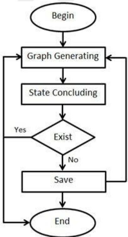
Figure 2.2. The control flow diagram of the forward approach
