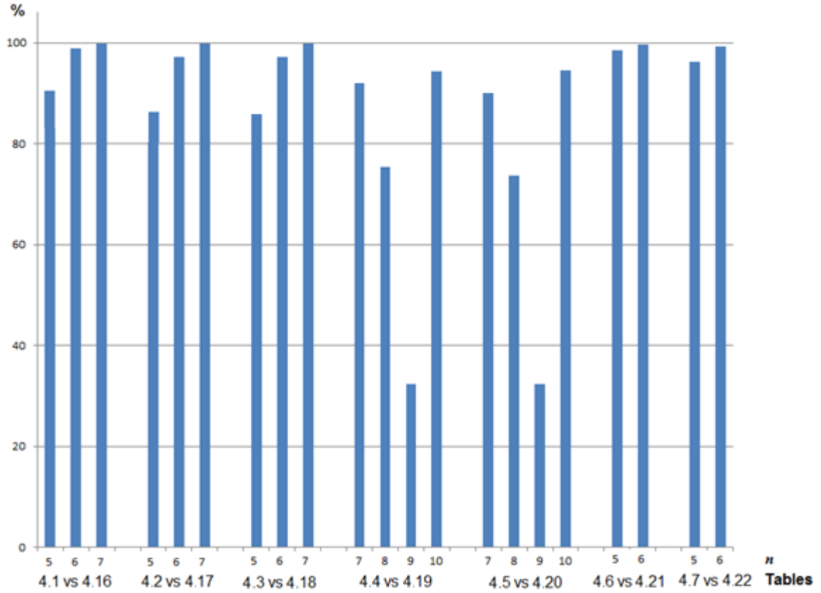
Figure 4.3. The execution time decrease in the optimized backward algorithm comparing to the backward algorithm
