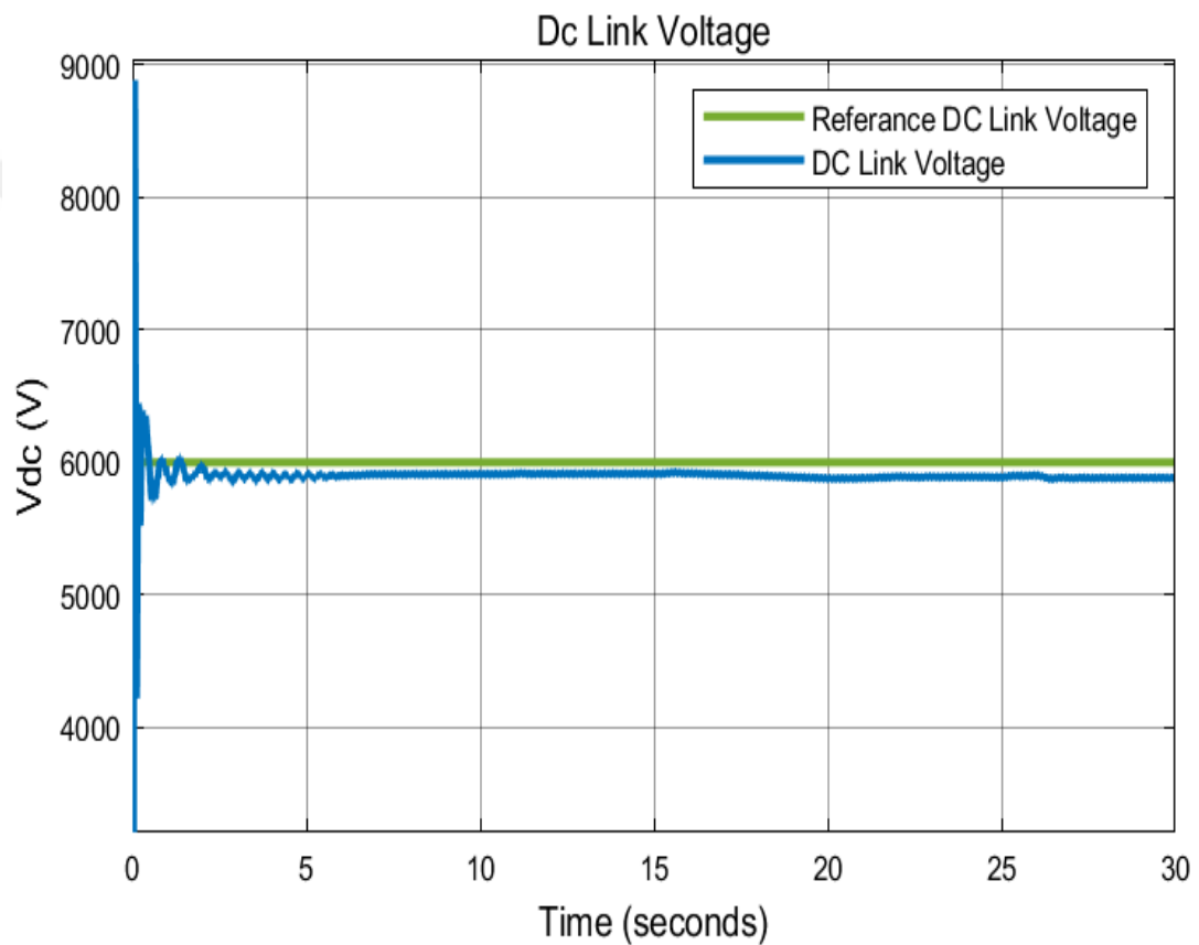
Figure 5.17 The Dc link voltage (Volt). Blue, represent the DC Link voltage of DFIG BTB MMC, Green, represent the reference DC Link Voltage.
