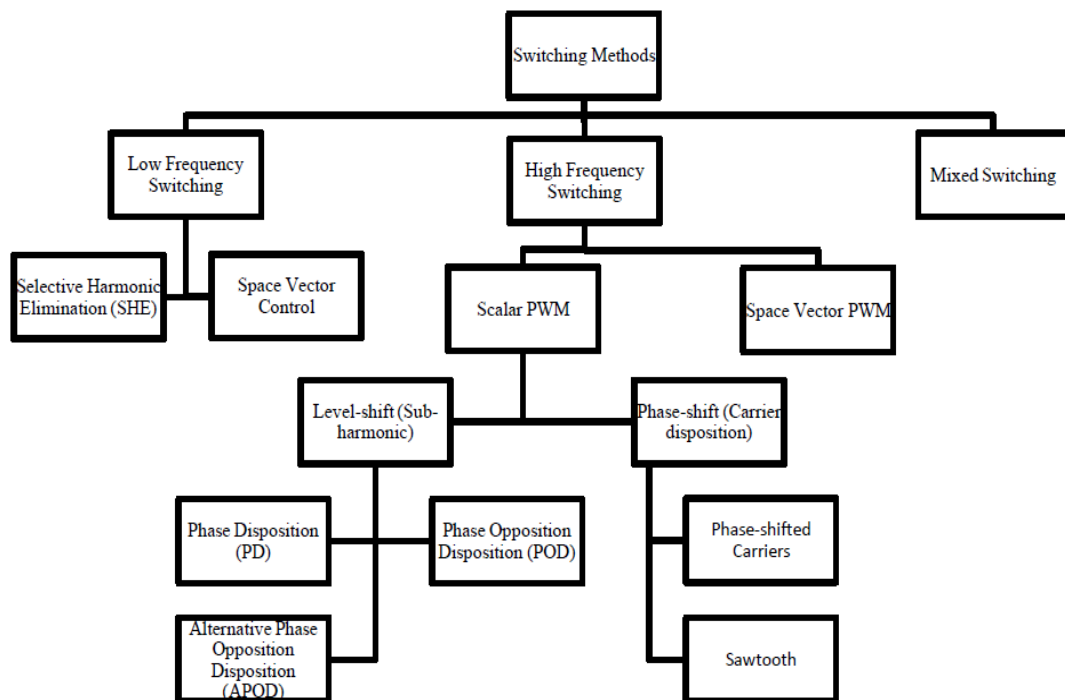
Figure 3.18 Switching methods for modular multilevel converters [106]
