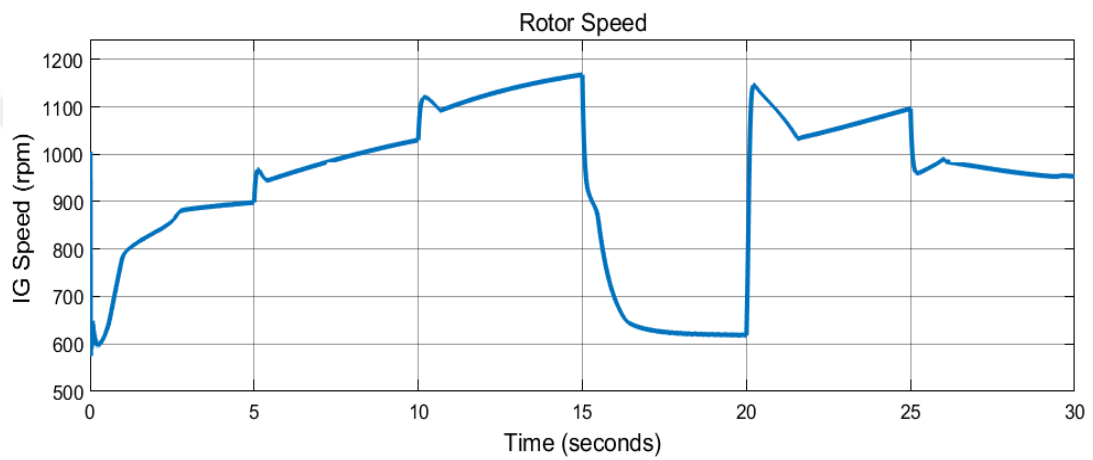
Figure 5.1 IG speed variation wind speed for variable speed of (10, 12, 15, 15, 10) m/sec that changed every 5 second period
