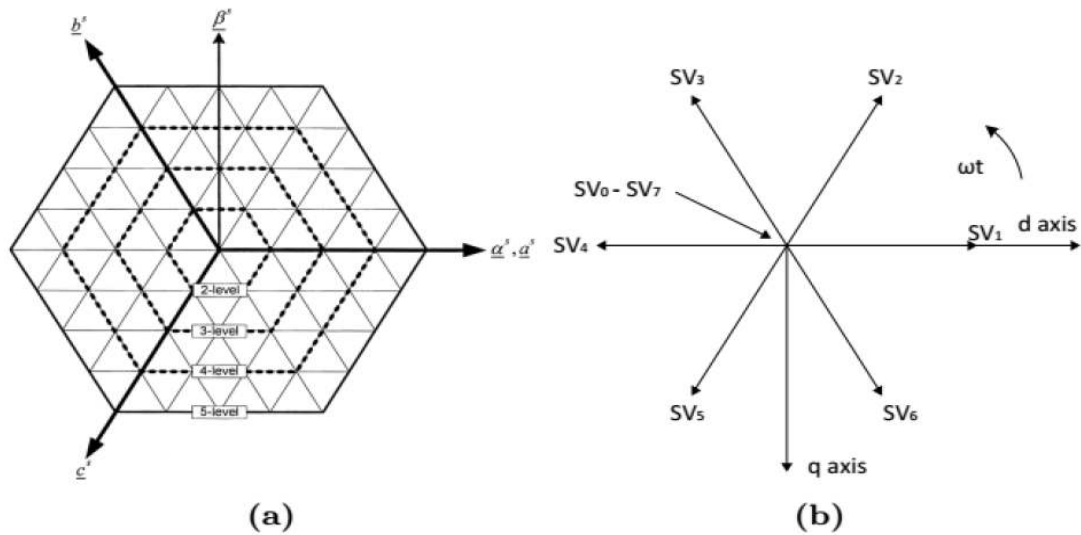
Figure 3.24 The space vector diagram: a) five-level structure; b) two-level SVM [106]
