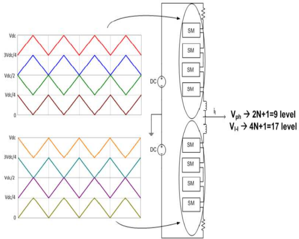
Figure 3.28 Carrier sets for the phase opposition disposition method for 2N+1 levels of phase voltage [106]
