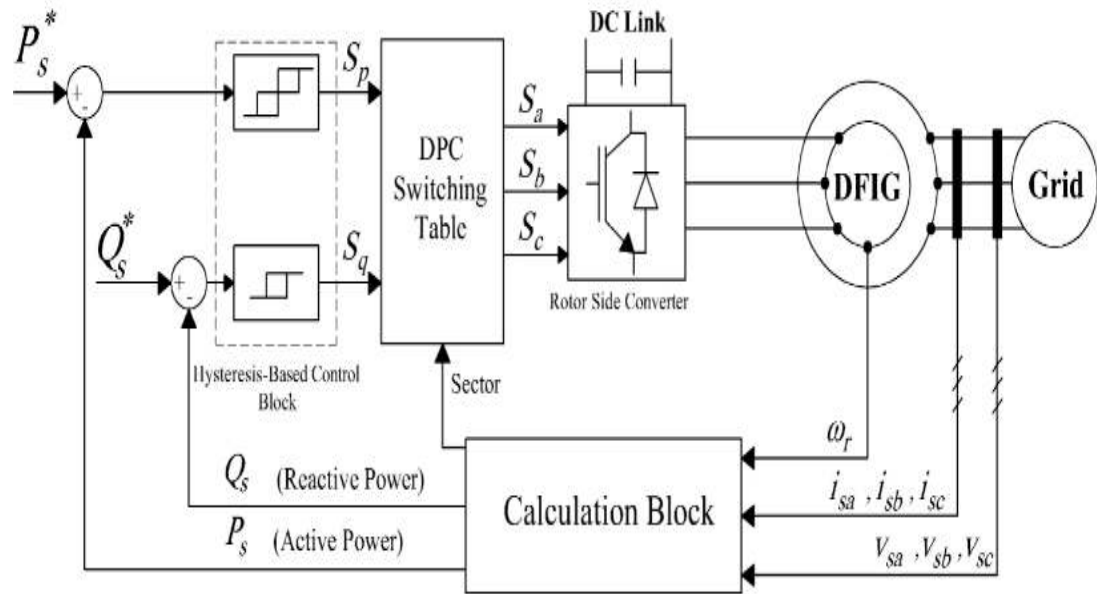
Figure 3.8 Typical block diagram for direct power control [53]
