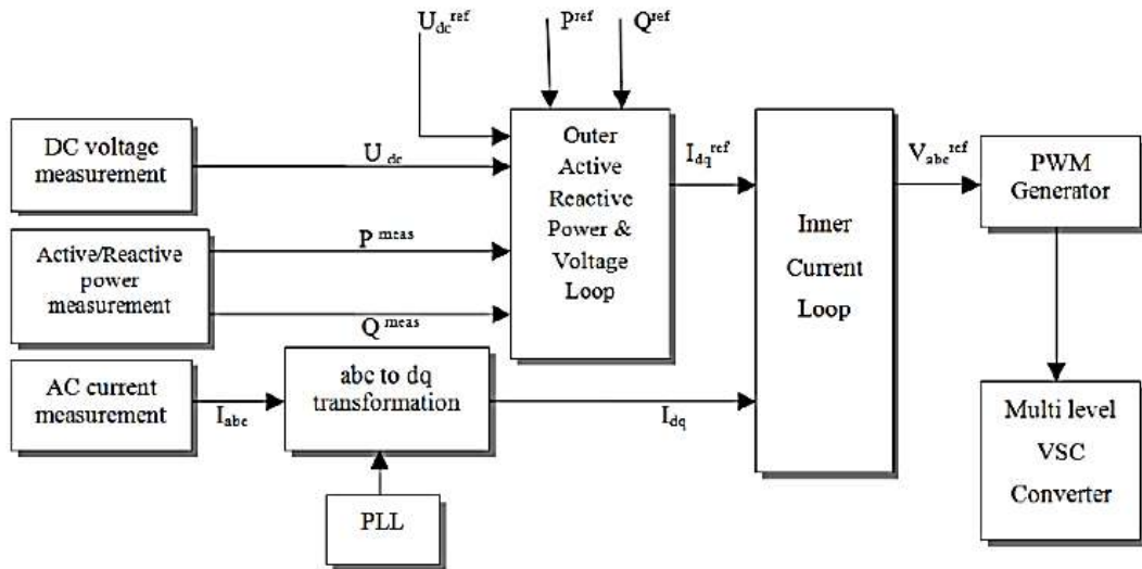
Figure 4.6 Block diagram active and reactive power loop
