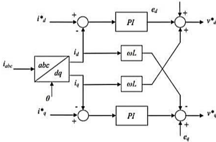
Figure 4.7 Block diagram structure of inner current loop
