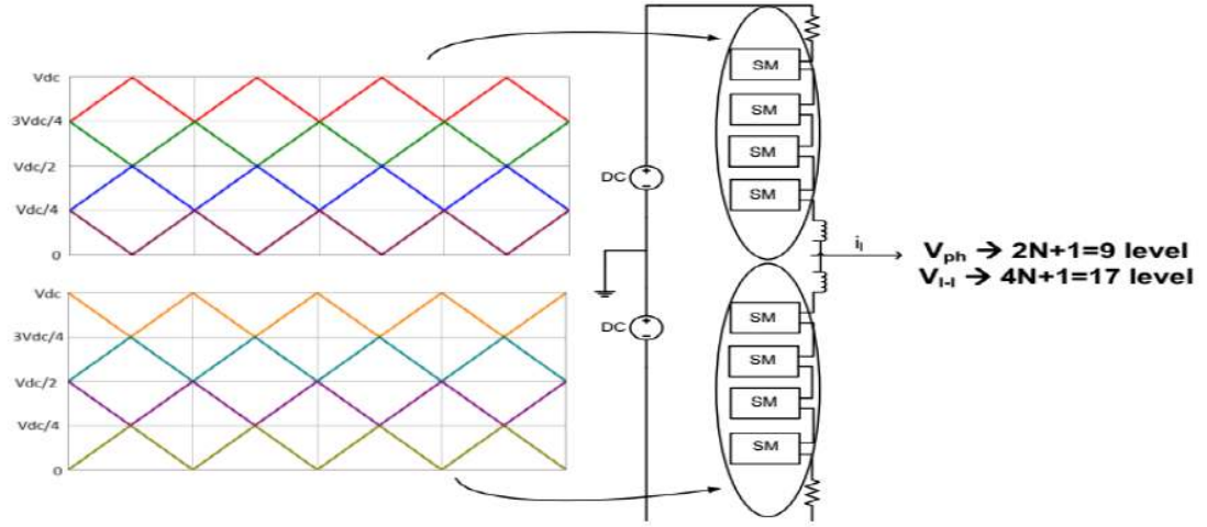
Figure 3.30 Carrier set for the alternative phase opposition disposition method for 2N+1 levels of phase voltage [106]
