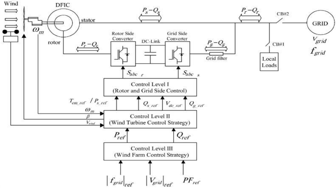
Figure 3.3 Doubly fed induction generator for a wind power system [53]
