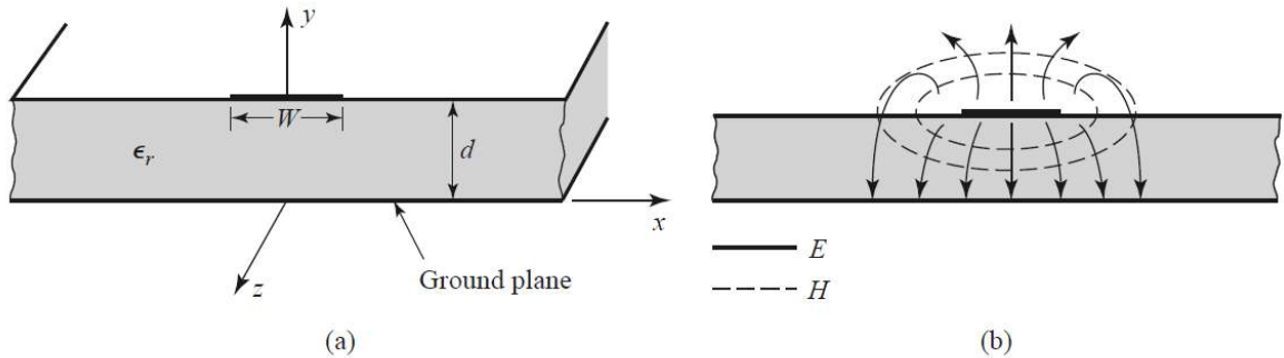
Figure 2. 1 Microstrip transmission line (a) Geometry (b) Electric and magnetic field lines
