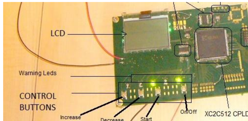
Figure 4.17 Control Buttons.
