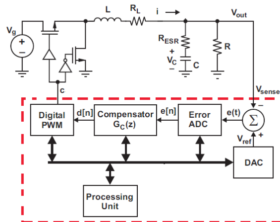
Figure 1.2 PID digital control algorithm in a SMPS.
