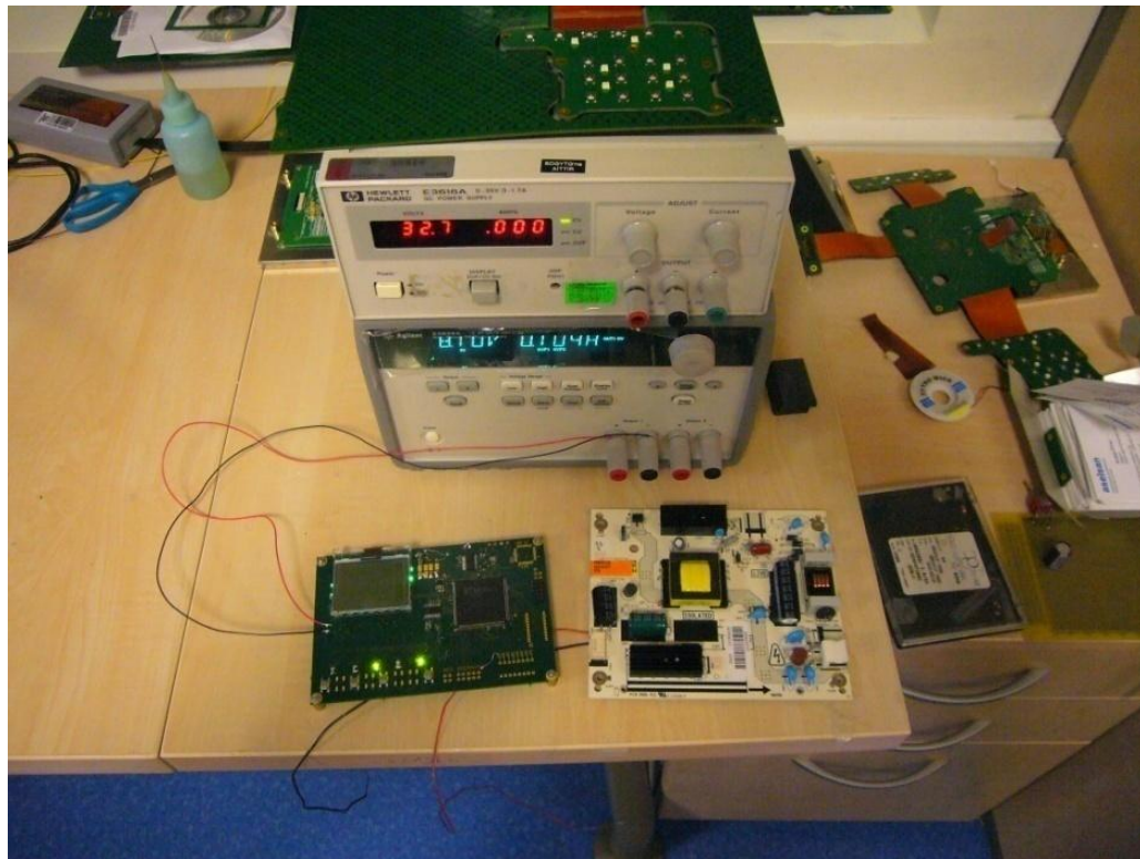
Figure 4.22 A SMPS System available in market is tested with SMPS Transformer Test Device.
