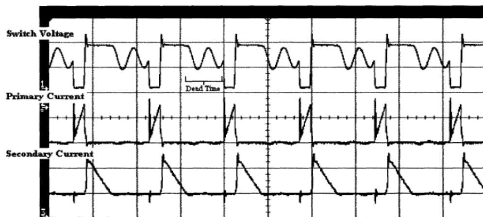
Figure 3.13 An oscilloscope print out of switching elements' waveforms in DCM (Kenia, 2004).
