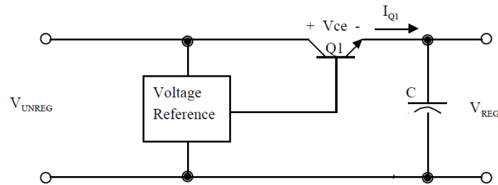
Figure 3.1 Schematic linear voltage regulators (Counsil,2000).
