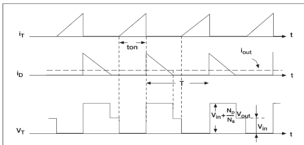
Figure 3.14 Typical Waveforms for DCM operation.(ST electronics, 1999).
