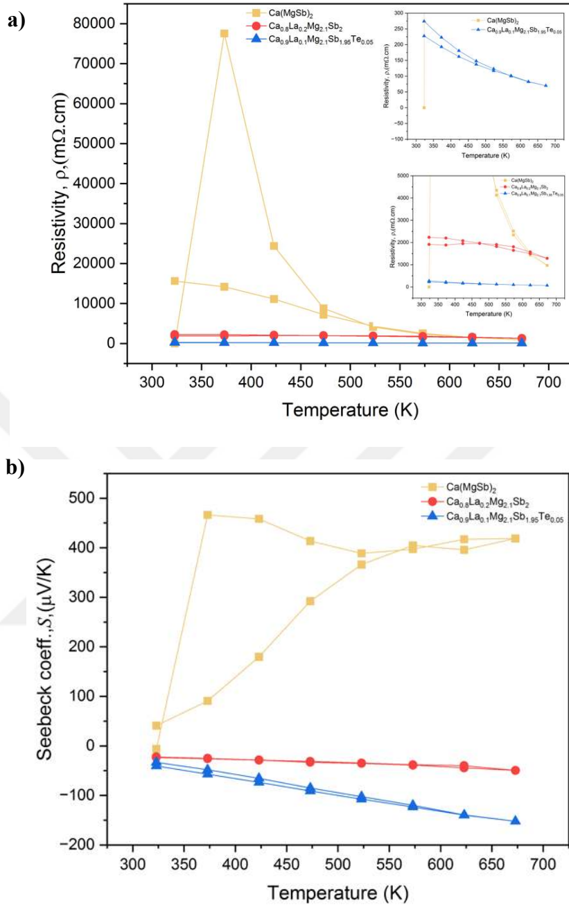
Figure 5. 8 CaMg 2 Sb 2 compounds thermoelectric measurements a) Resistivity and b) Seebeck coefficient as a function of temperature.
