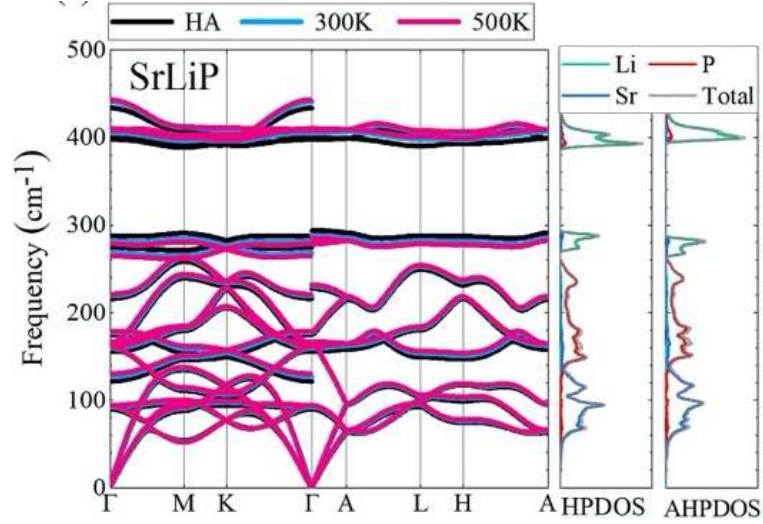
Figure 3. 9 Harmonic phonon dispersion curves and phonon density of states (HPDOS), non-harmonic phonon dispersion curves and phonon density of states (AHPDOS) for SrLiP (41).
