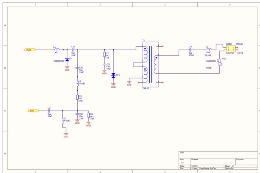
Figure 26 Transformer Circuit
