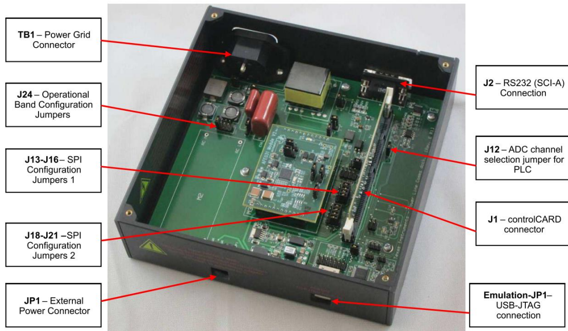
Figure 9 PLC Modem from Texas Instruments[12]
