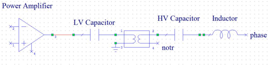
Figure 6 Coupling Circuit[8]
