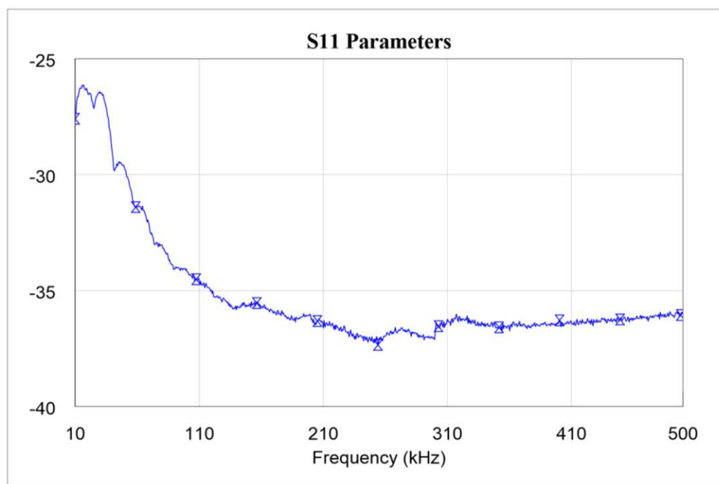
Figure 14 S11 Parameters
