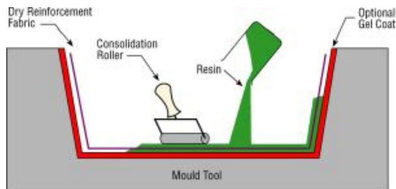
Figure 3.6 Hand lay-up process technique.
