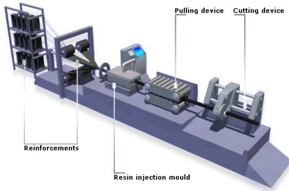
Figure 3.12 Pultrusion technique.
