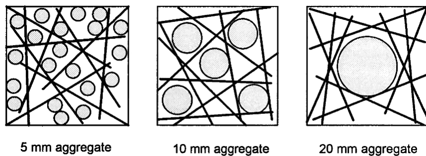
Figure 2.9 Effect of aggregate size on fiber distribution(Chen 1995)
