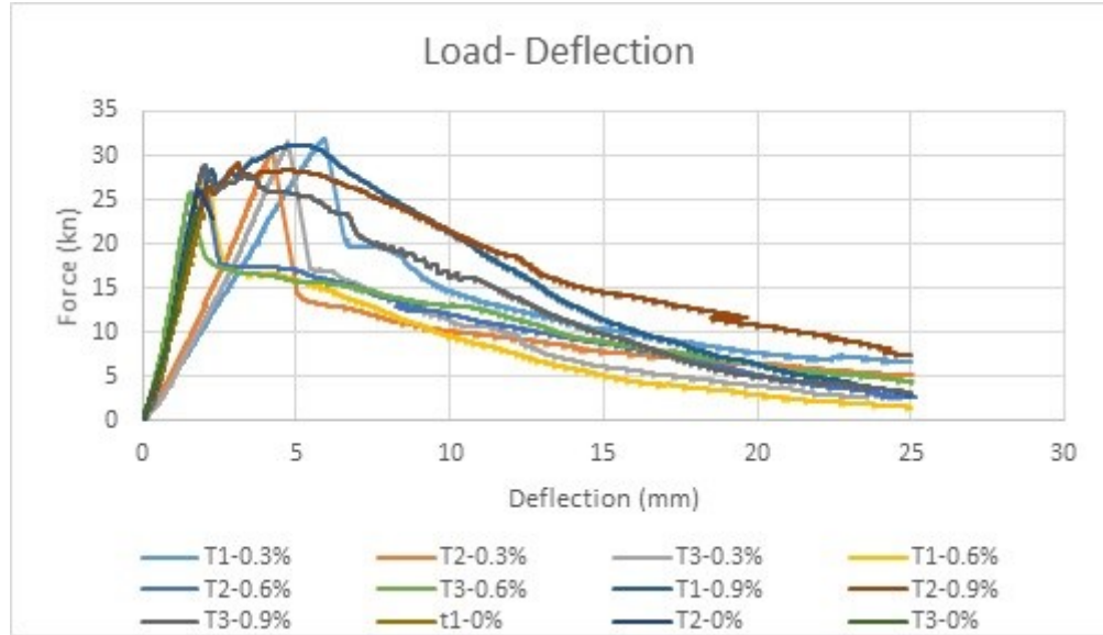
Figure 4.15. Load deflection curves for TPM-80.
