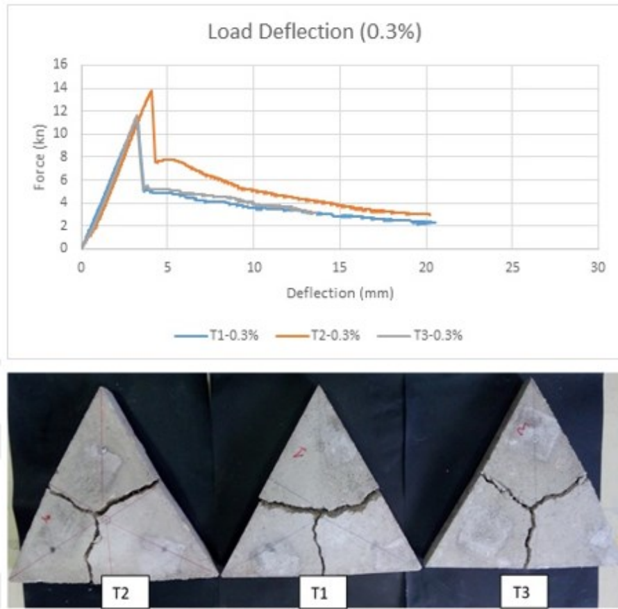
Figure 4.7 Load-deflection garph for Triangular panel 50-(0.3%)
