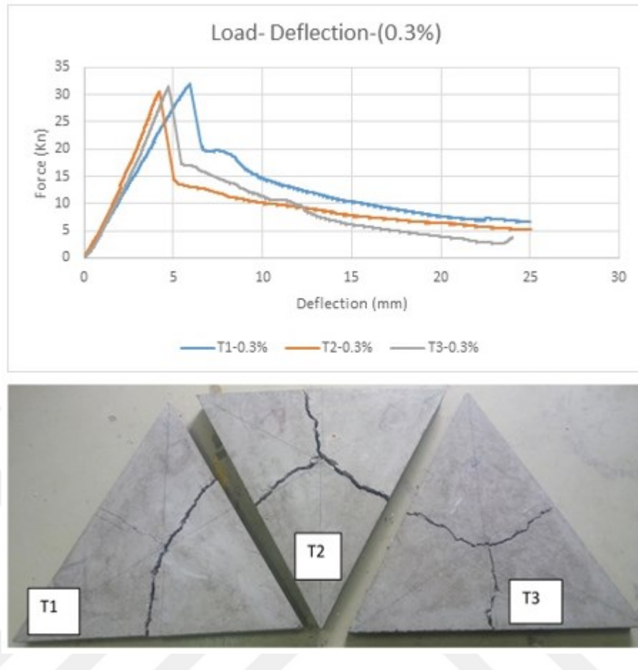
Figure 4.12 Load-deflection and crack pattern garph of Triangular panel 80-(0.3%)
