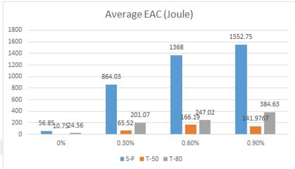
Figure 4.16. Average EAC for Square and Triangular panels.
