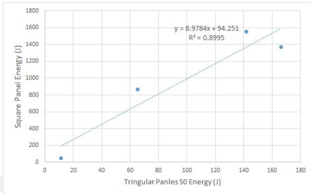
Figure 4.19. The energy relationship obtained from Square panels and Triangular panels -50
