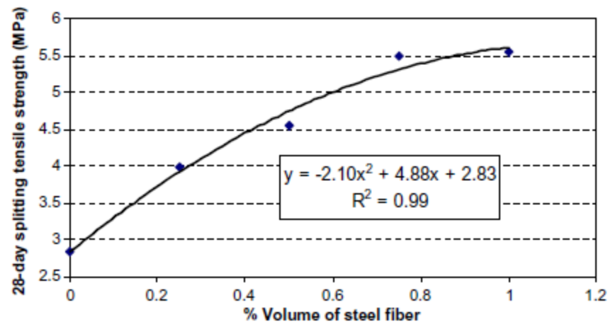
Figure 2.6 Relationship between volume of steel fiber and splitting tensile strength Shafigh et al. (2011).
