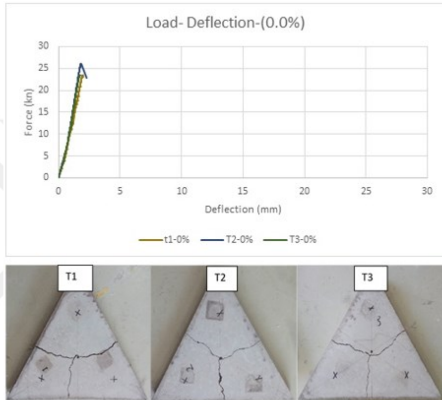
Figure 4.11 Load-deflection and crack pattern garph of Triangular panel 80-(0%)
