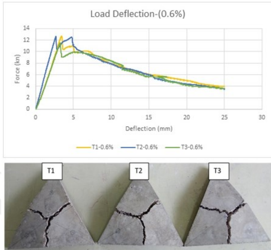
Figure 4.8 Load-deflection and crack pattern garph of Triangular panel 50-(0.6%)
