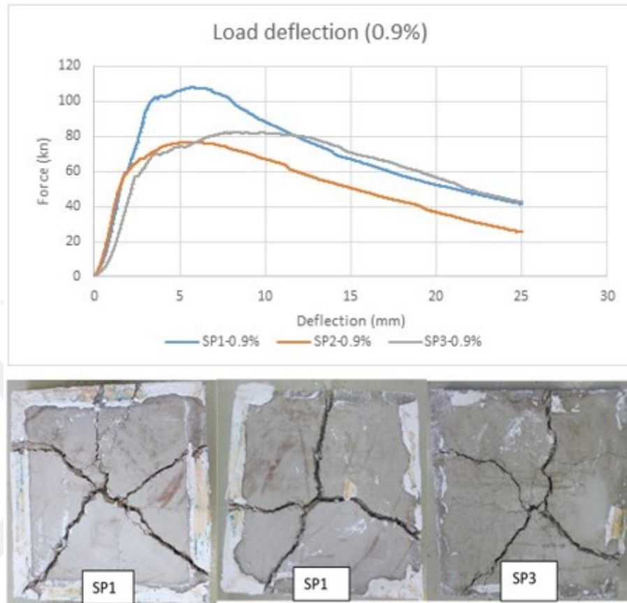
Figure 4.4 Load-deflection and crack pattern garph of Square panel-(0.9%)
