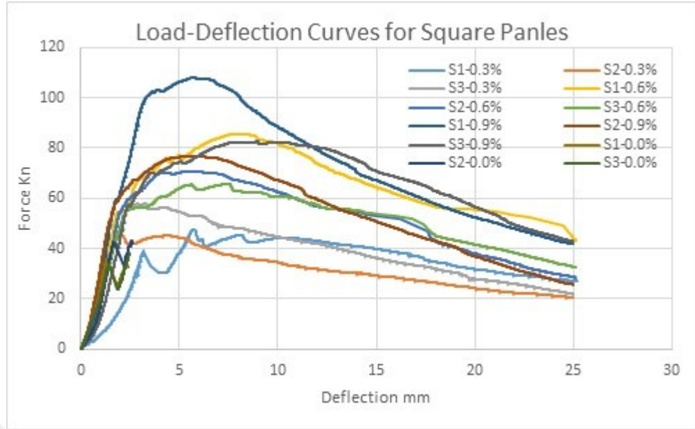
Figure 4.5. Load-deflection curves for square panels.
