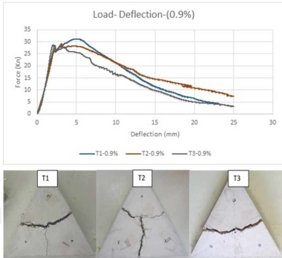
Figure 4.14 Load-deflection and crack pattern garph of Triangular panel 80-(0.9%)
