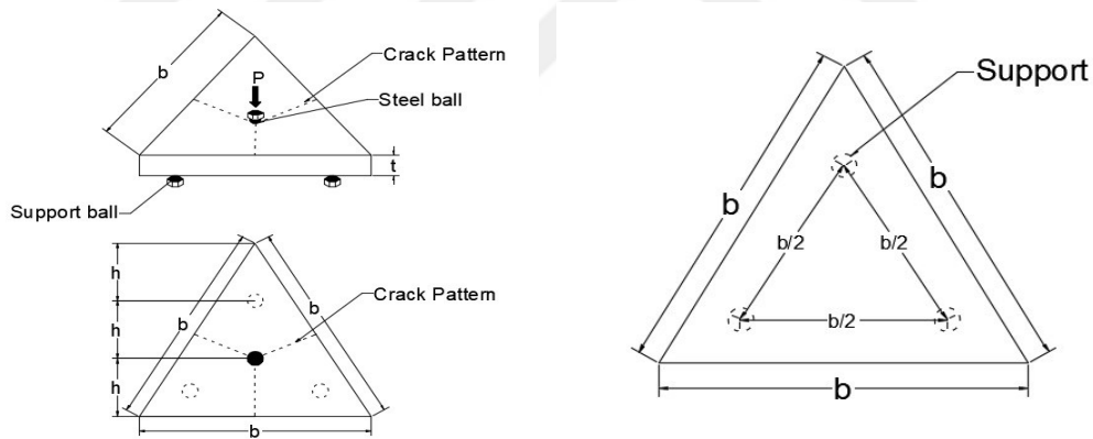
Figure 2.13 Geometry of the traingular plate specimen and support layout.
