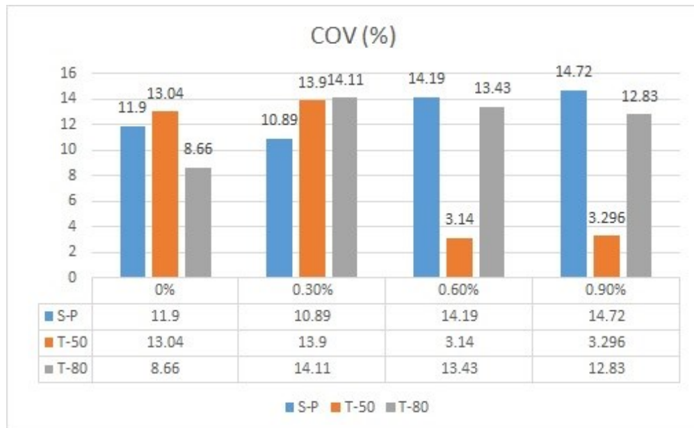
Figure 4.17. Coefficient of variation for square and triangular panels
