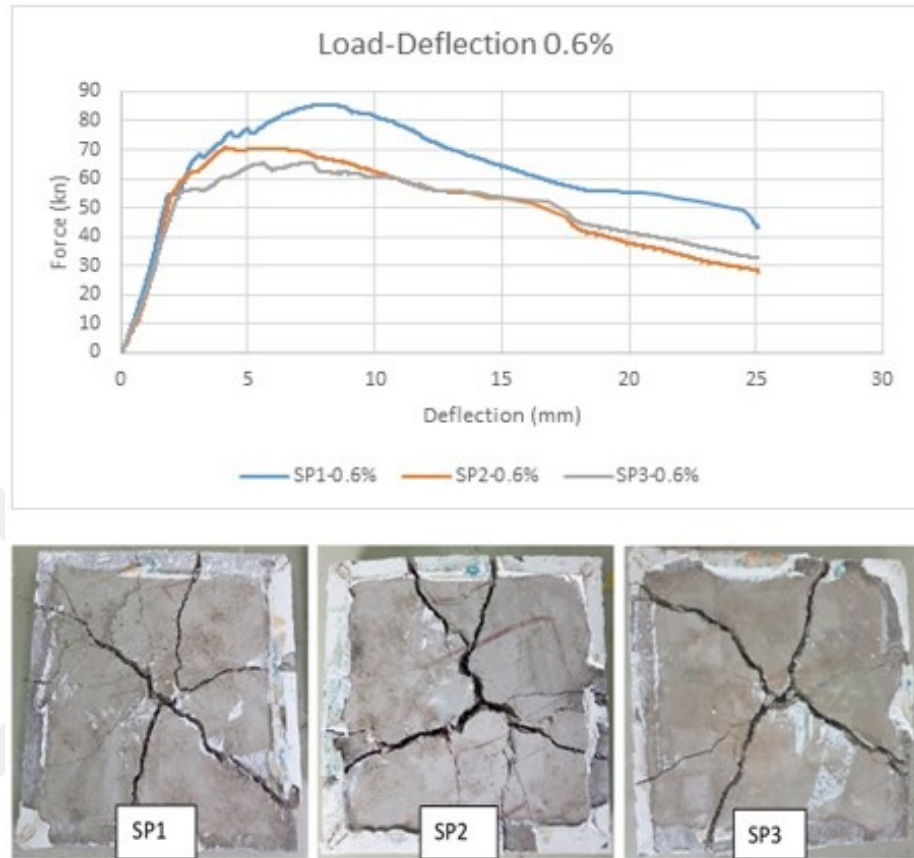
Figure 4.3 Load-deflection and crack pattern garph of Square panel-(0.6%)
