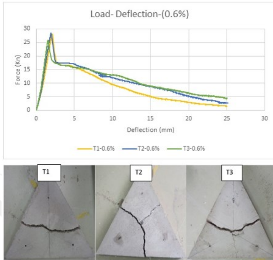
Figure 4.13 Load-deflection and crack pattern garph for Triangular panel 80-(0.6%)
