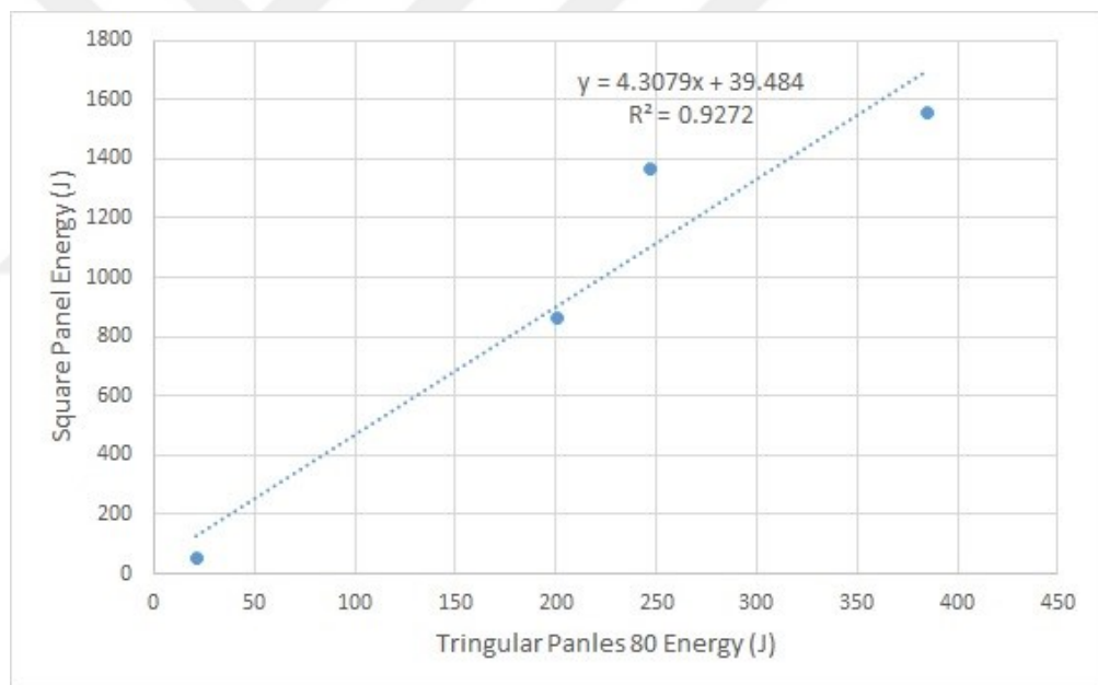
Figure 4.18. The energy relationship obtained from Square panels and Triangular panels -80
