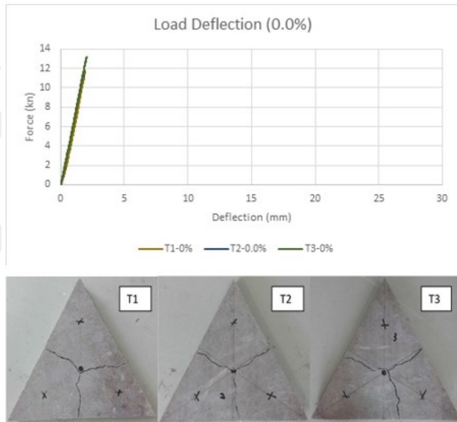
Figure 4.6 Load-deflection and crack pattern garph of Triangular panel 50-(0.0%).
