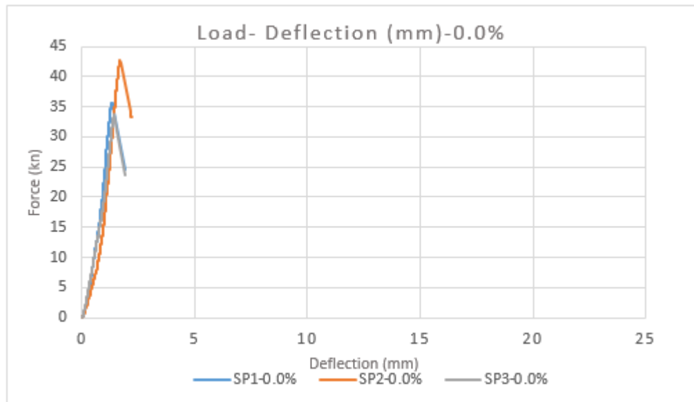
Figure 4.1 Load-deflection garph for control Square panel-(0.0%)
