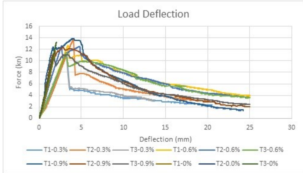
Figure 4.10. Load deflection curves for TPM-50.
