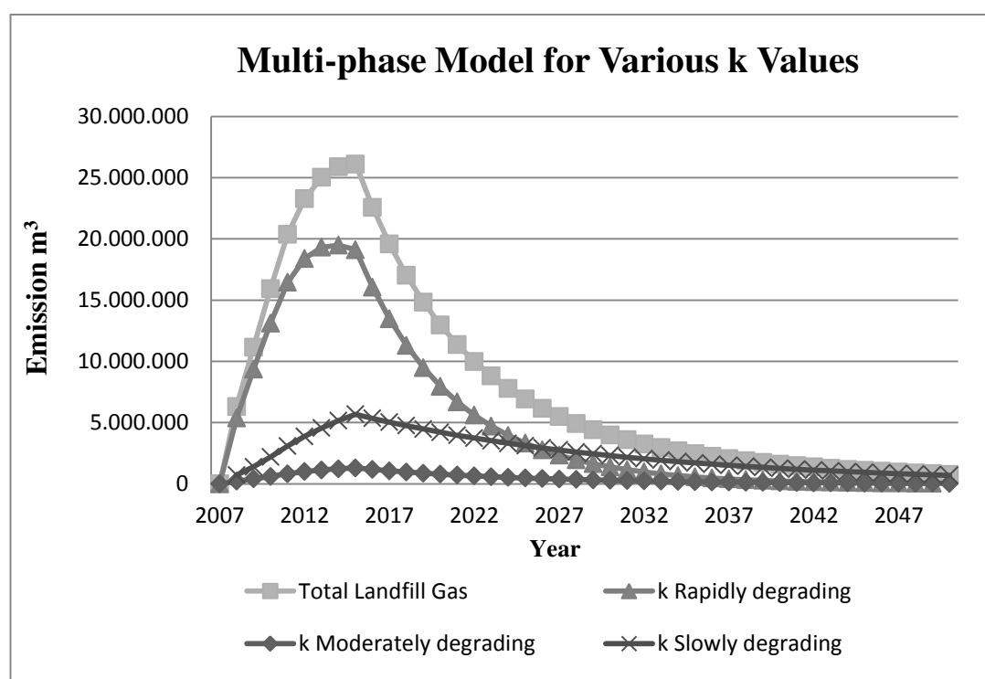
Figure 5.4 Emission Estimations by Multi-phase Model for Various k Values . That is shown total LFG generation and under the LFG generation, slowly degrading, moderately degrading and rapidly degrading organic waste decomposition
