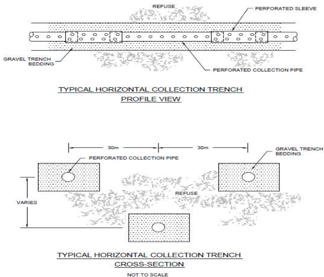
Figure 2.5 Shows the construction of a typical horizontal LFG extraction trench. (Handbook For The Preparation Of Landfill Gas To Energy Projects World Bank 2003)
