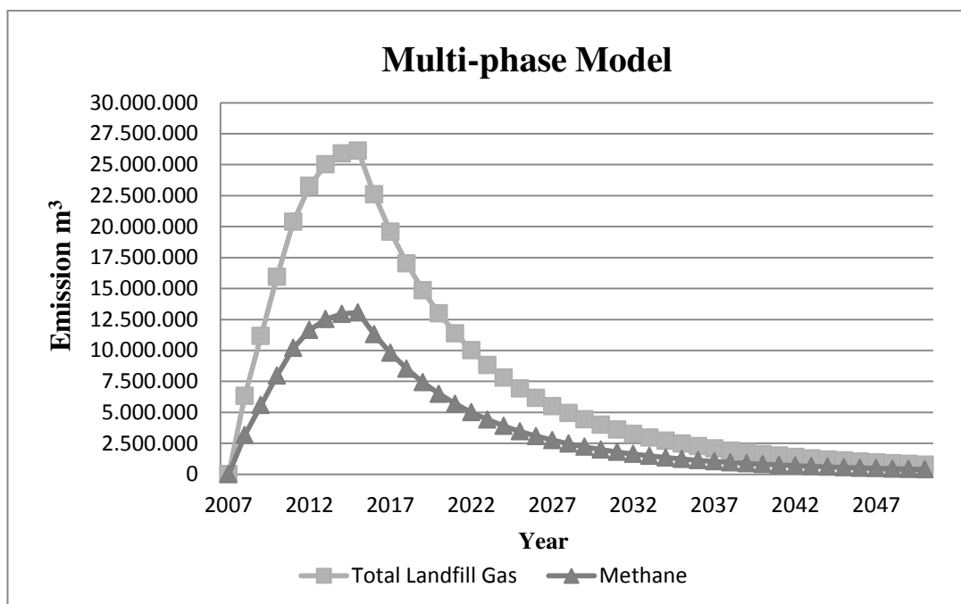
Figure 5.3 Emission Estimations by Multi-Phase Model, x axial is represented year and y axial is represented Total LFG \text{m}^3
