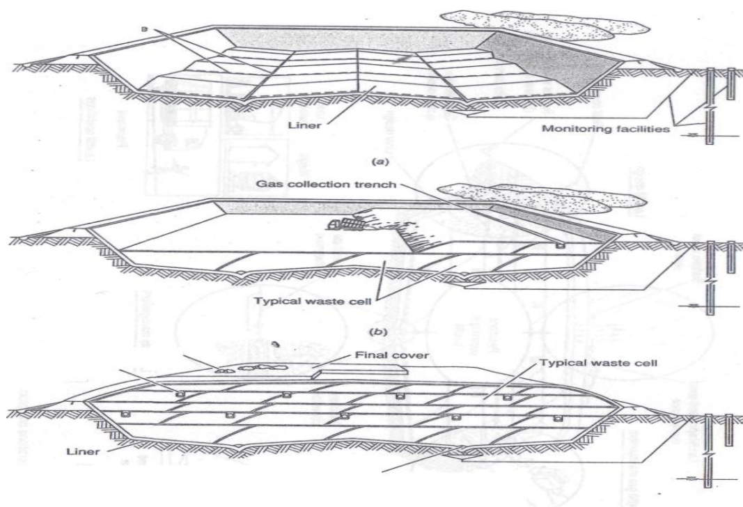
Figure 2.3 Development and completion of a solid waste landfill: (a) excavation and installation of landfill liner, (b) placement of solid waste in landfill, and (c) cutaway through completed landfill.
