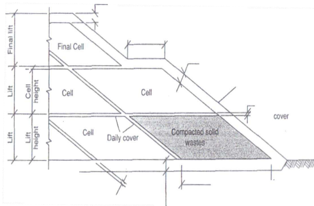
Figure 2.1 Sectional view through a landfill (Tchobanoglou, Theisen, & Vigil, 1993)
