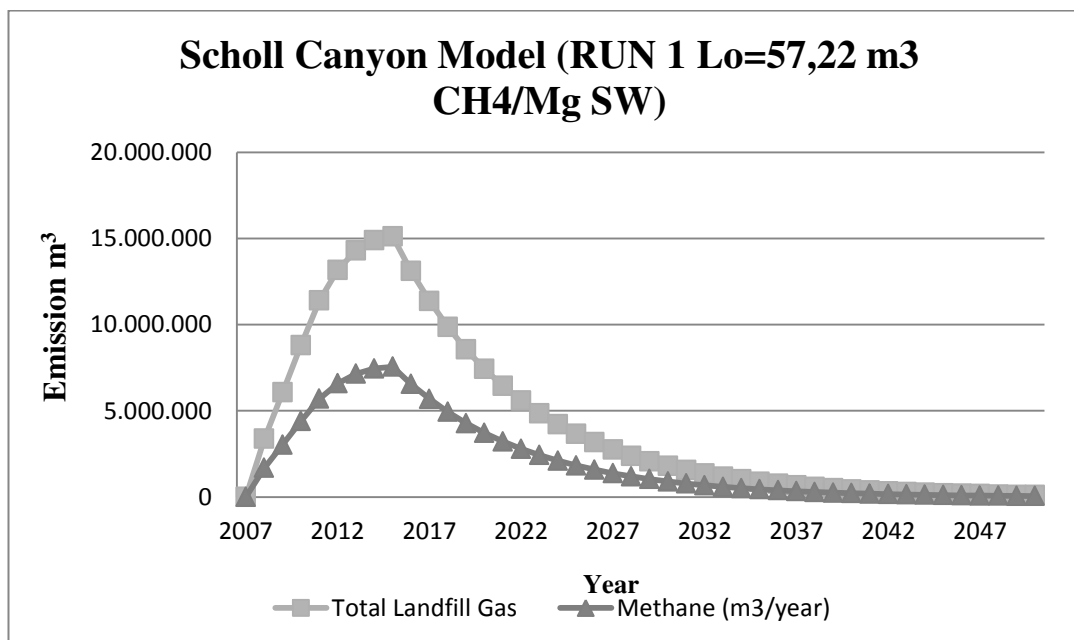
Figure 5.6 Emission Estimations by Scholl Canyon Model (RUN 1 Lo=57,22 m3 CH4/Mg SW)x axial is represented year and y axial is represented LFG m3.
