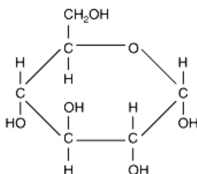
Figure 5.3: Molecular structure of glucose [Url-22].
