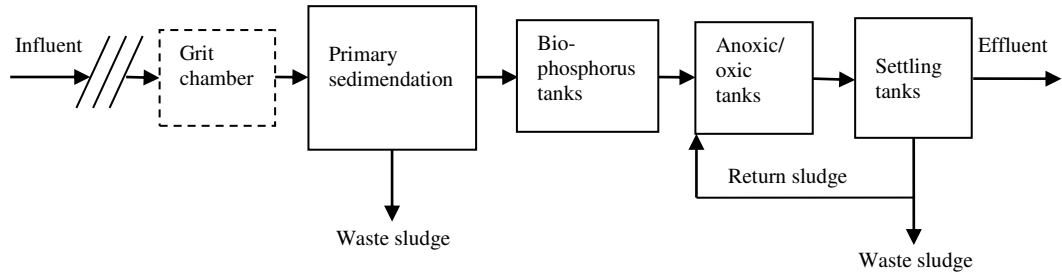
Figure 3.5 A simple flow diagram of Cigli WWTP
