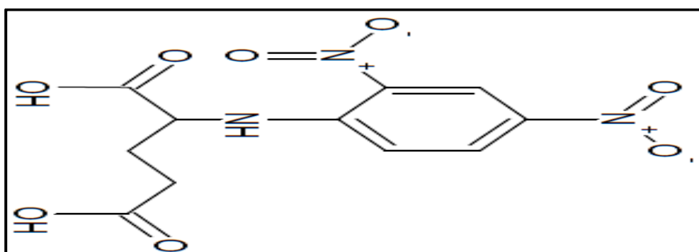
Figure 14: The Chemical Structure of MSG derivative using (DNFB) Reagent.
