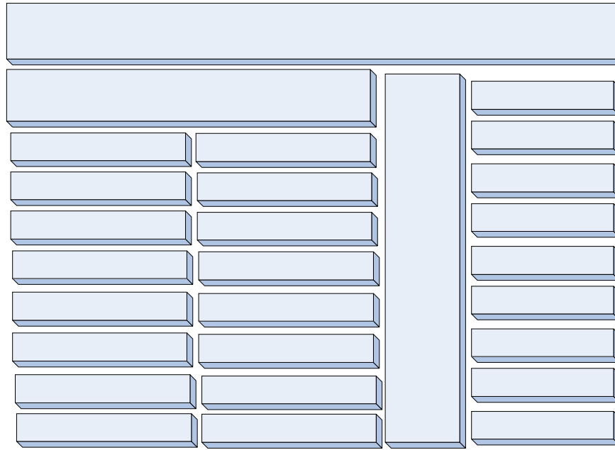
Figure 98 - Primitive system
