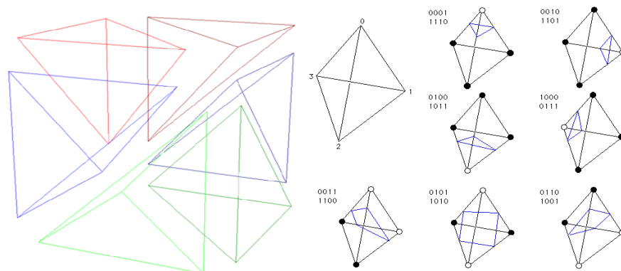
Figure 115 - Six tetrahedrons of a voxel (left) and mesh configuration for one tetrahedron (Right)
