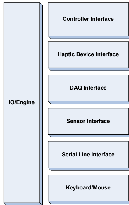
Figure 158 - I/O Engine Architecture
