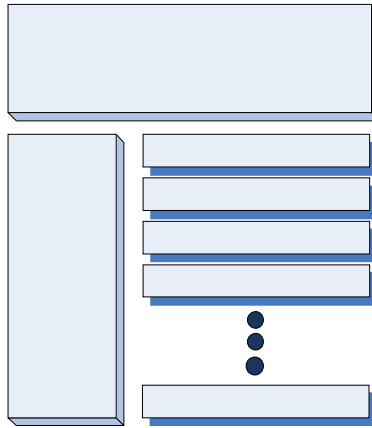
Figure 95 - Vertex system
