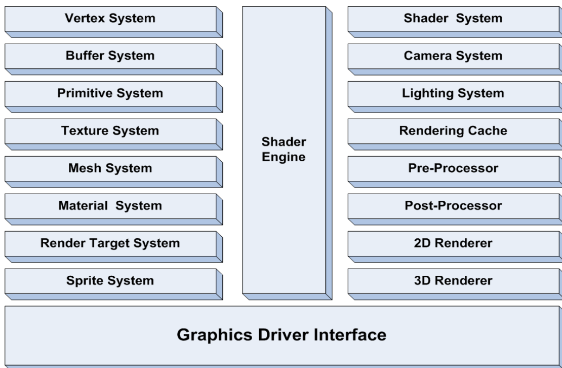
Figure 94 - DMRenderer architecture
