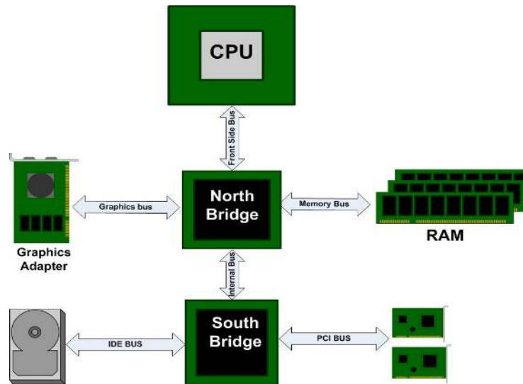
Figure 93 - Computer architecture
