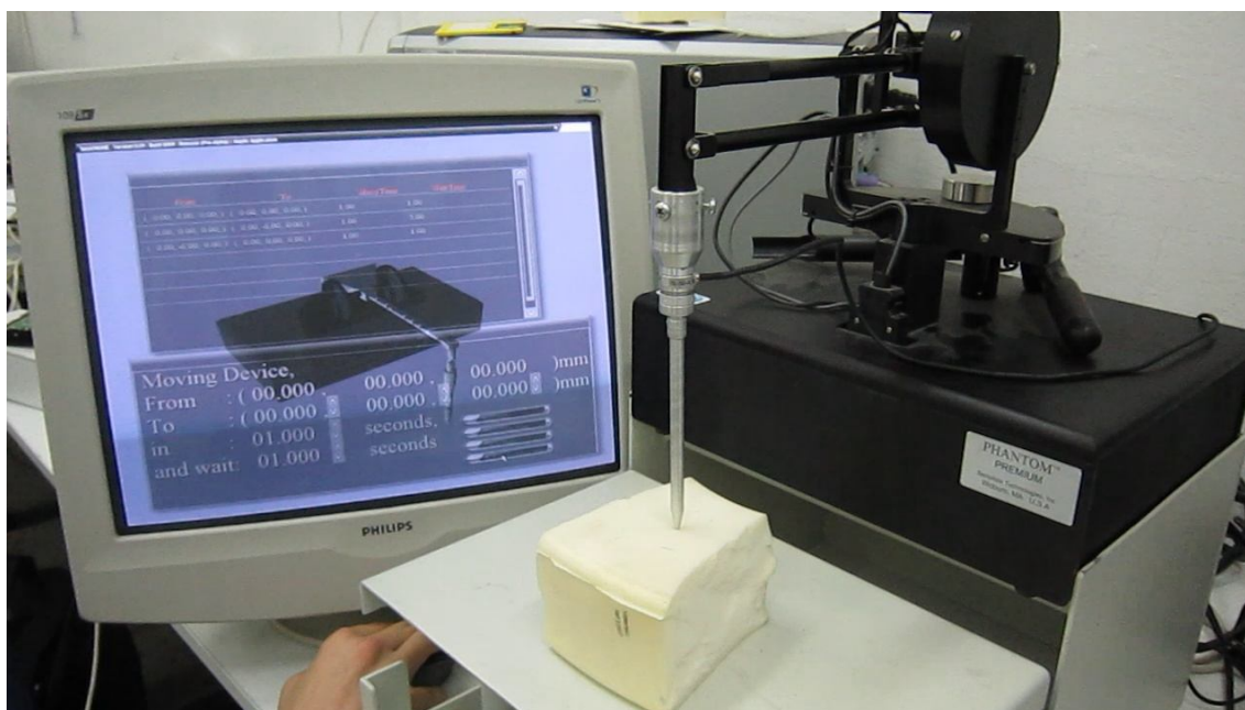
Figure 169 – Path planning
