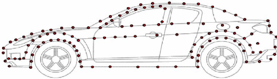
Figure 51 - Sampled vertices
