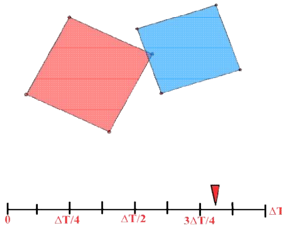
Figure 83 - Final collision positions found; Collision report will be created.
