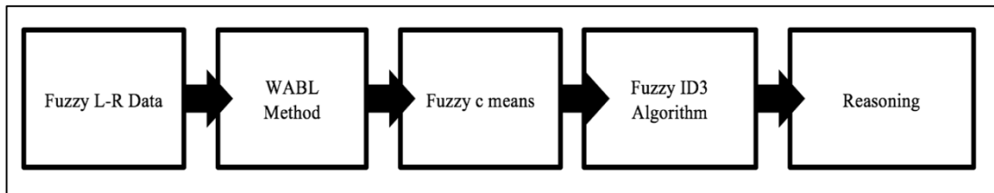
Figure 4.1 The process of fuzzy decision tree induction based on linguistic data by using WABL defuzzification method.
