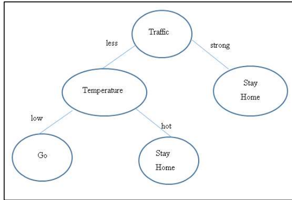
Figure 2.3 Example of classical decision tree.
