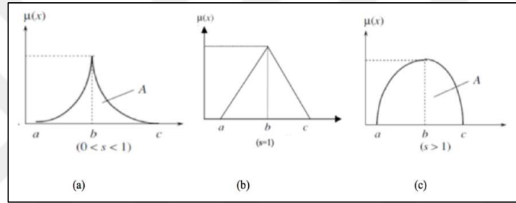
Figure 2.1 Forms of parametric triangular fuzzy numbers (a) 0 < s < 1 (b) s=1 (c) s > 1 .
