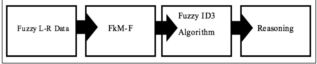
Figure 5.2 The process of fuzzy decision tree induction based on linguistic data by using WABL defuzzification method.
