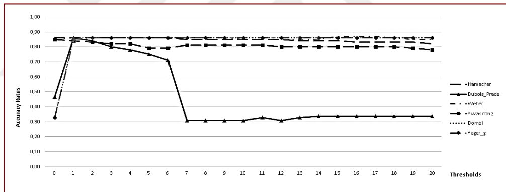
Figure 6.7 Accuracy rates handled from different parametric operators Range =(0-20) and \theta_r=0.75 .
