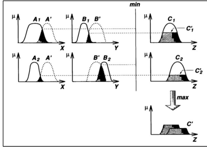
Figure 2.6 Fuzzy reasoning for multiple rules with multiple antecedents.
