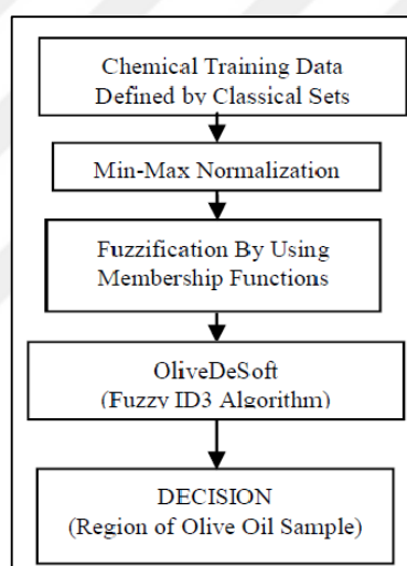
Figure 6.2 Classification Procedure by using fuzzy ID3.
