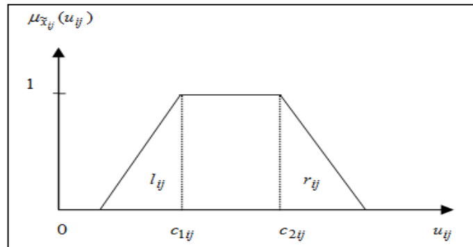
Figure 5.1 Trapezoidal membership function.
