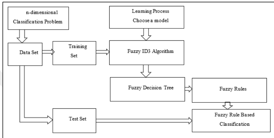
Figure 2.7 A classification problem with Fuzzy ID3 algorithm combined with FRBC
