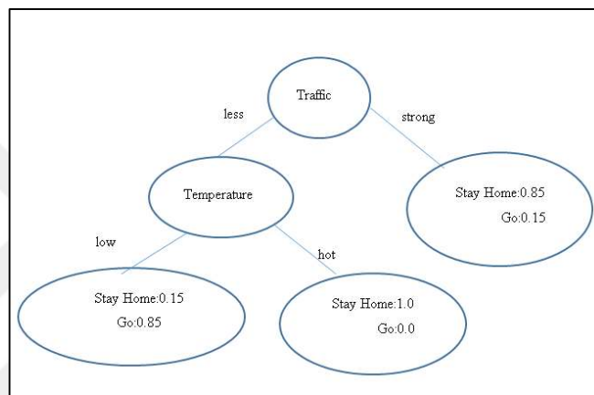
Figure 2.4 Example of fuzzy decision tree.
