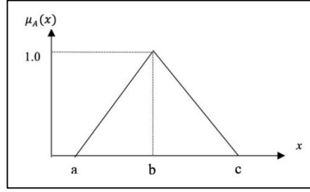
Figure 2.2 Triangular Membership function characterized by three parameters \{a, b, c\} .
