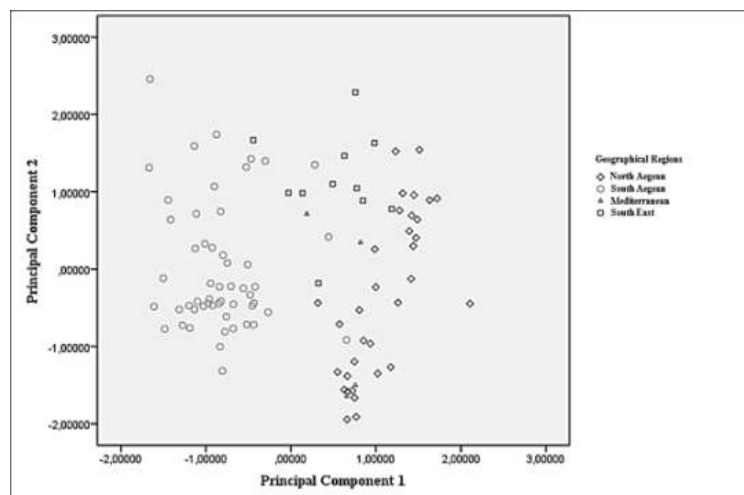
Figure 6.6 The Principal components plot on the virgin olive oil sample.
