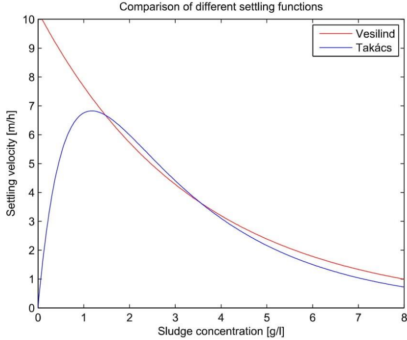
Figure 2.6 Comparison of different settling functions [16]
